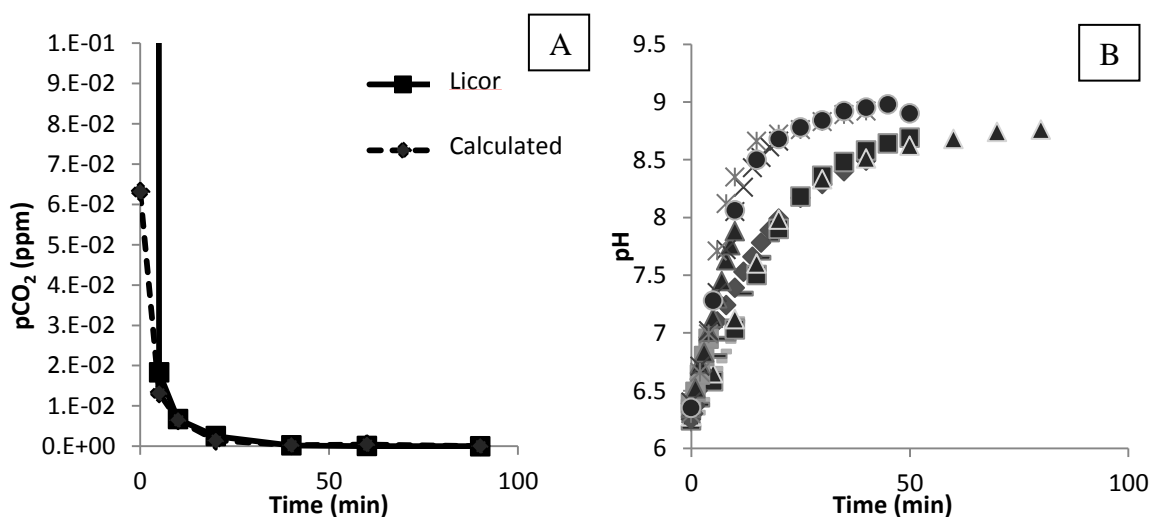
Figure II-15 A. Evolution of calculated \text{pCO}_2 and measured. B. Evolution of pH for low pH experiments at high flow rate and low flow rate. The point correspond to the sampling at different time step.
