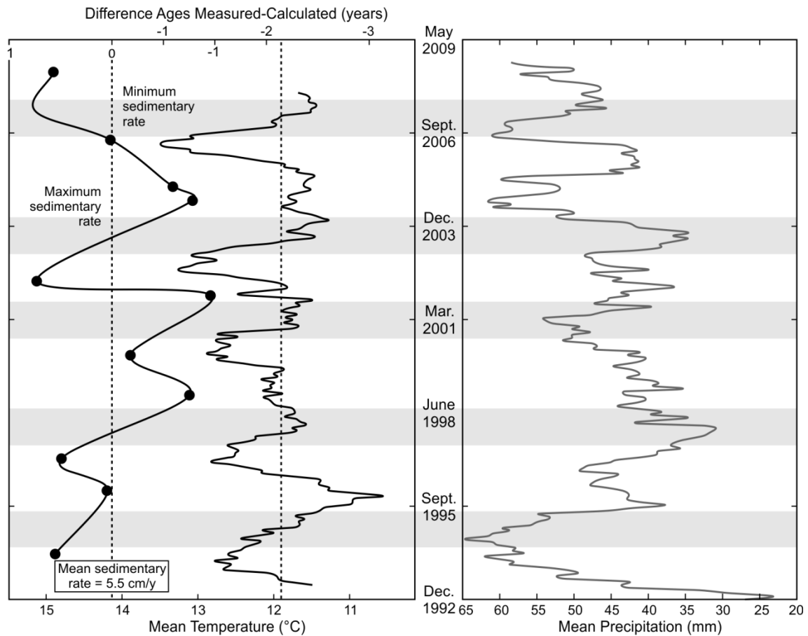
Figure I-16 (A) The difference between measured age obtained with the ^{210}\text{Pb}/^{226}\text{Ra} method and the calculated age with the linear trend compare to the variation of mean temperature. There is correlation between the high temperature and the high accumulation rate. The dashed line corresponds to the difference of measured ages and calculated one with a mean value of 5.5 \text{ cm}\cdot\text{yr}^{-1} . And the black line is the mean temperature value measured in Aulnat (French Massif Central, Météo France). (B) The difference between measured ages obtained with the ^{210}\text{Pb}/^{226}\text{Ra} method and the calculated age with the linear trend compare to the variation of mean rain.
