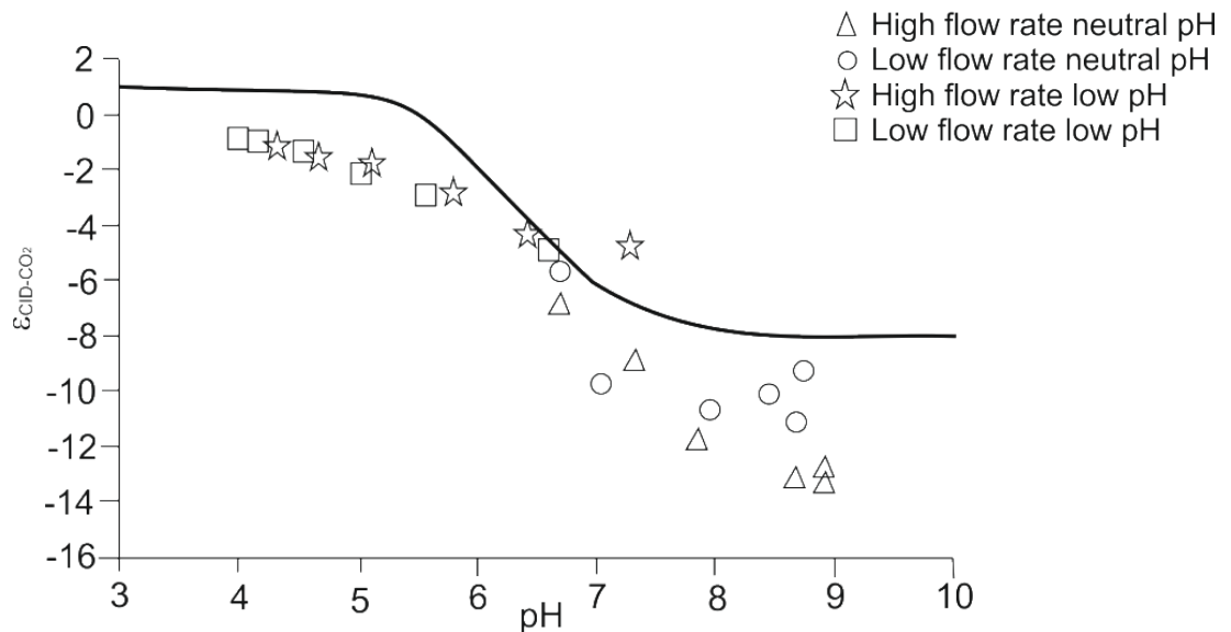
Figure II-20 Evolution of the fractionation factor between DIC and CO 2
