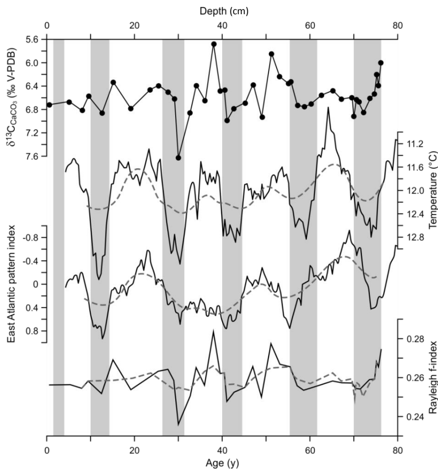
Figure I-20 \delta^{13}\text{C} of travertine with the Rayleigh distillation associated correlate with the East Atlantic pattern (component of the North Atlantic Oscillation) and the temperature in Aulnat (French Massif Central) vs. time. The bands are the climatic cycles of 3 or 5 years, the dashed lines correspond to the range mean.
