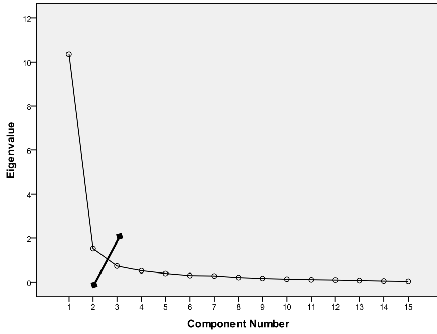
Scree Plot
