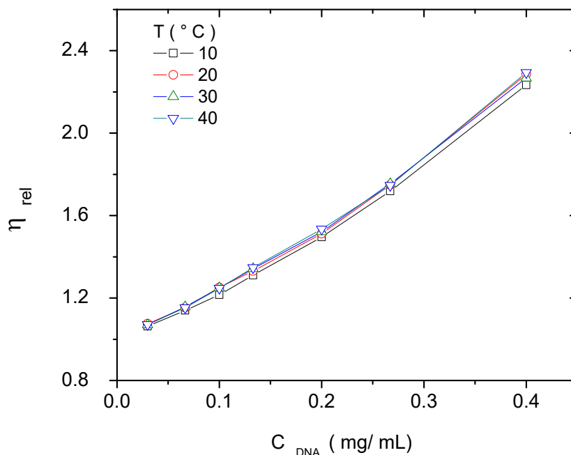
Figure 2.15. Relative viscosity dependence with DNA concentration measured at several temperatures.
