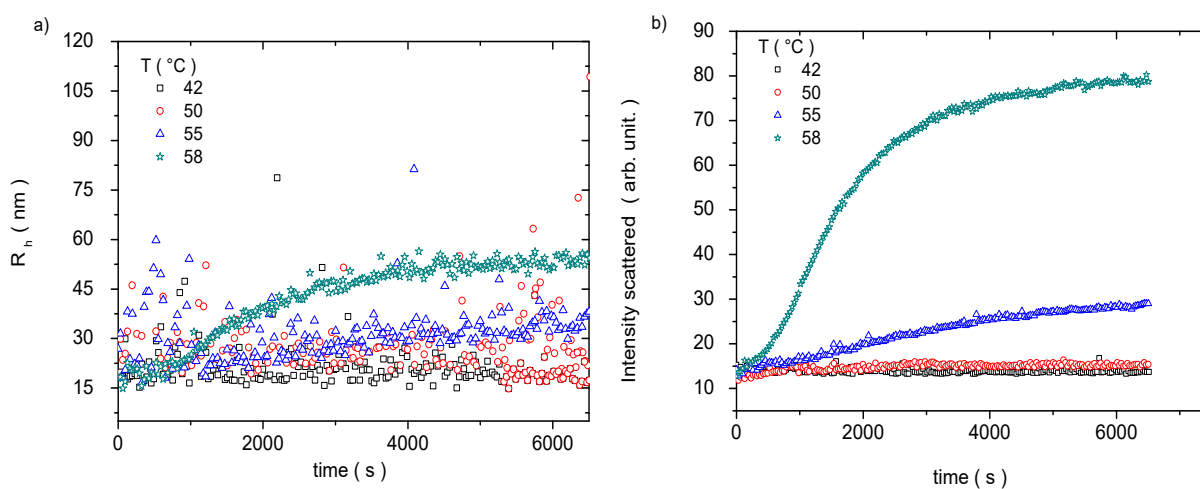
Figure 4.9. a) Hydrodynamic radius and b) scattering light intensity as a function of time for a P104 solution with a concentration of 20 mg/mL after the temperature jump from T_1 = 38\text{ }^\circ\text{C} to the temperatures of 42, 50, 55 and 58 ^\circ\text{C} .
