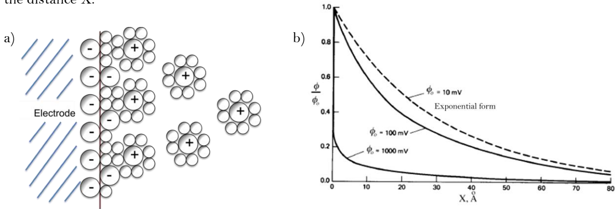
Figure 3.3 a) Schematic representation of Gouy-Chapman model and b) Potential profiles through the diffuse layer for a solution 10^{-2} M in a 1:1 electrolyte at 25^\circ C [22].
