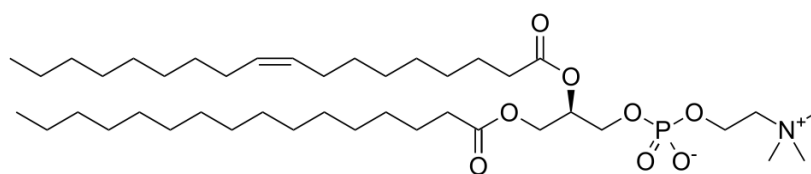
Figure 5.1. Chemical structure of L- \alpha -Phosphatidylcholine [27].
