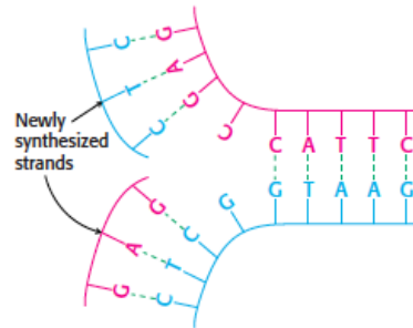
Figure 1.1. DNA replication, as suggested by Watson and Crick [4].
