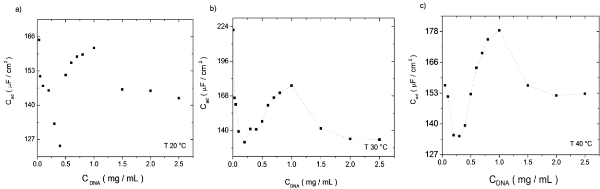
Figure 3.19. Adsorption capacitance, C_{ads} , as a function of DNA concentration at the temperatures of a) 20, b) 30 and c) 40 °C.
