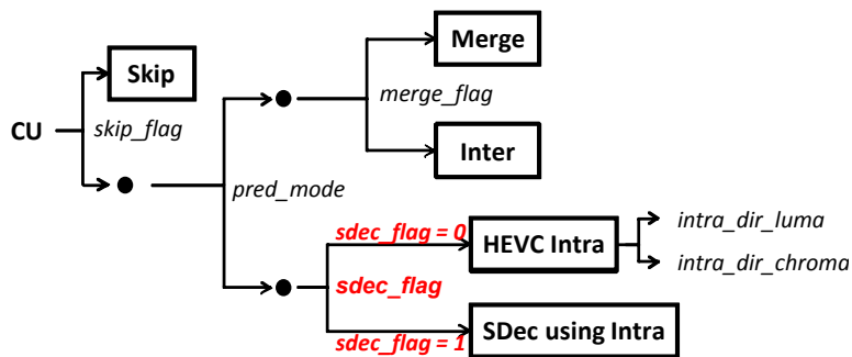
Figure 3.2 – Signaling scheme for the introduced SDec syntax elements in the SDec scheme using Intra coding mode
