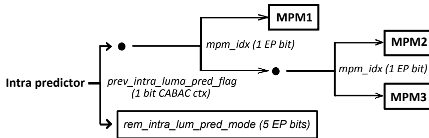
Figure 1.5 – Intra MPM signaling scheme.
