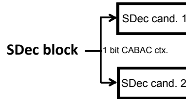
Figure 3.8 – Signaling of sdec_ref in case of 2 candidates for the SDec reference.
