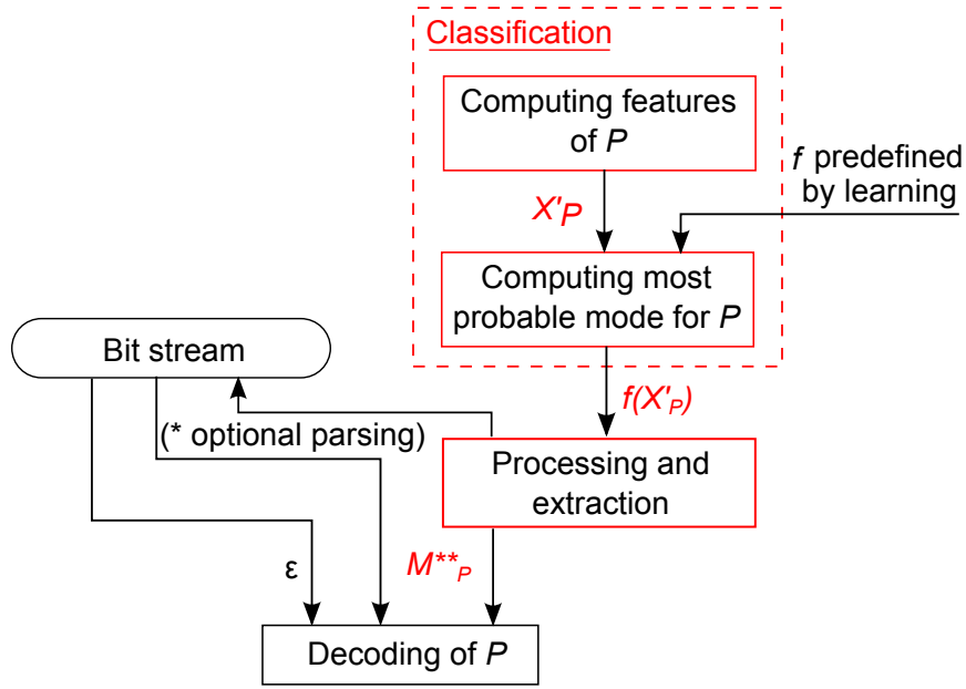
Figure 8.7 – Proposed decoder scheme based on machine learning.
