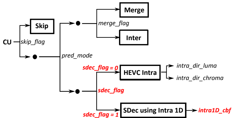
Figure 4.8 – Signaling scheme for the introduced SDec syntax elements in the SDec scheme using Intra 1D mode.
