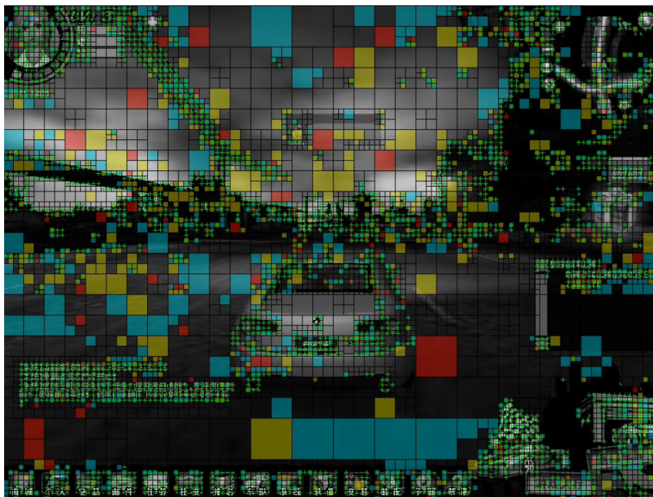
Figure 3.10 – Sequence "ChinaSpeed_1024×768" with blocks encoded in SDec mode highlighted in yellow, blue and red for exploiting respectively the first, the second and the third block candidate to be the SDec reference - AI configuration.
