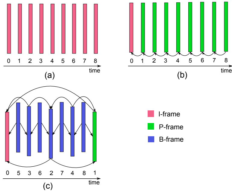
Figure 1.2 – GOP structures with different types of frame highlighted in colors. Arrows indicate references of a frame. The number under each frame indicates its order of processing. (a) AI. (b) LP. (c) RA.
