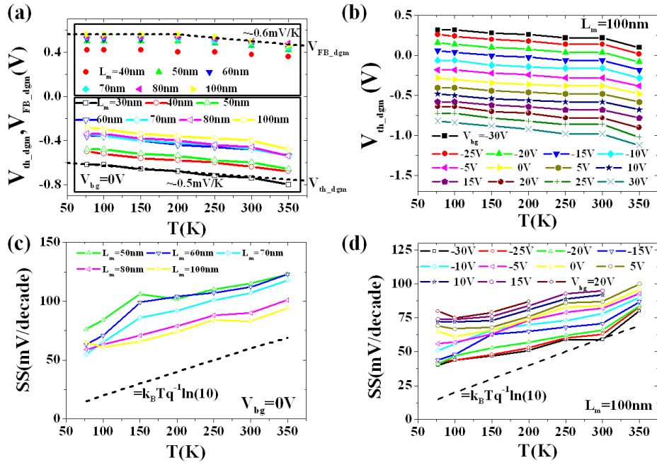
Figure 9 (a) The temperature dependence of V_{th,dgm} and V_{FB,dgm} versus L_m and (b) that of V_{bg} dependence in L_m=100 nm JLT. (c) The temperature behavior of SS at V_{bg}=0 V with respect to L_m and (d) that of V_{bg} reliance in L_m=100 nm JLT.
