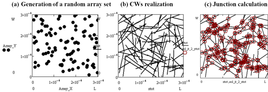
Figure 3-5 One example ( L_{\text{mask}}=W_{\text{mask}}=3\mu\text{m} with \rho_{\text{CW}}=10/\mu\text{m}^2 ) of (a) generation of a random array set of center position ( x_i, y_i ), (b) CWs realization based on ( x_i, y_i, l_i, \theta_i ), and (c) junction calculation.
