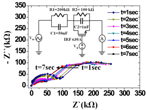
Figure A-3 The transient impedance measurements for the two R//C circuits with a commercial N-type MOS-FET (metal-oxide-semiconductor field-effect transistor), IRF630A, to simulate the change of the total resistance of the second R//C circuit. As the gate voltage varied, the total resistance of the second circuit changed, shifting the second semicircle to the left. Inset: The electrical model for a DUT ( R_1=200\text{k}\Omega//C_1=50\text{nF} and R_2=100\text{k}\Omega//C_2=1\text{nF} // IRF630A (NMOS))
