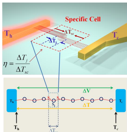
Figure 7-5 Definition of a specific cell (top), and a schematic of the specific cell in one ideal path (bottom), where the whole film composed of such numerous identical cells. Thus, the total TEP is obtained from the contribution of TEP from each cell.
