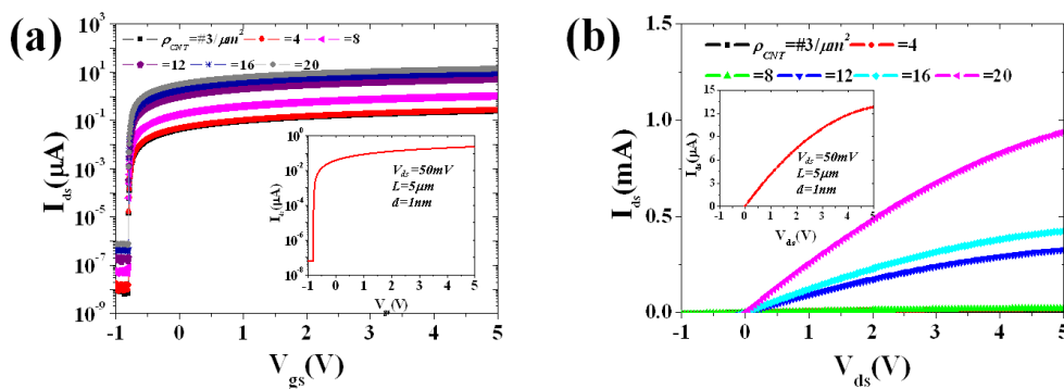
Figure 6-10 SPICE simulation results of (a) transfer curves I_{ds}(V_{gs}) and (b) output characteristics depending on different \rho_{\text{CNT}} based on L_d . ( L_{\text{mask}} = W_{\text{mask}} = 3 \mu\text{m} )
