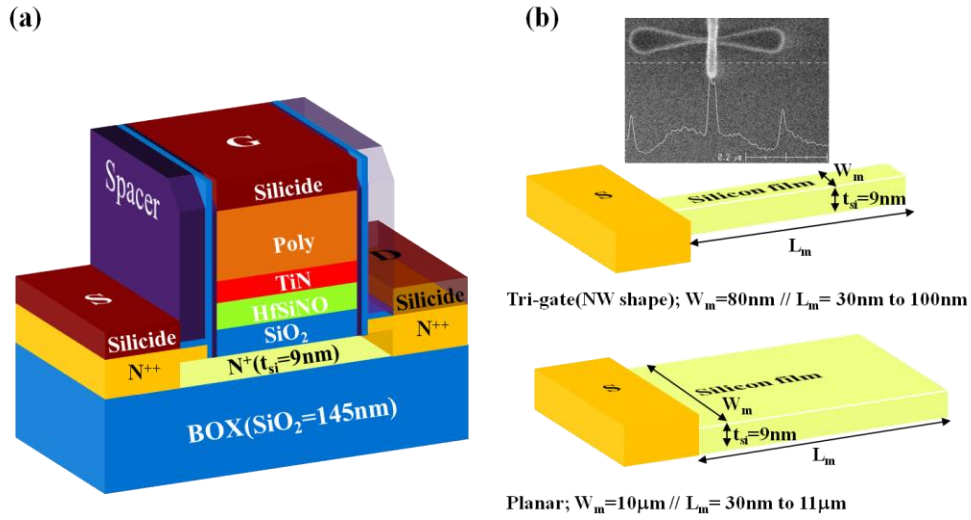
Figure 4-3 (a) Simplified three-dimensional device structure and (b) on-mask splits ( L_m and W_m ) for planar and nanowire(NW) shape of JLTs with a representative SEM (Scanning Electron Microscope) image of NW JLT
