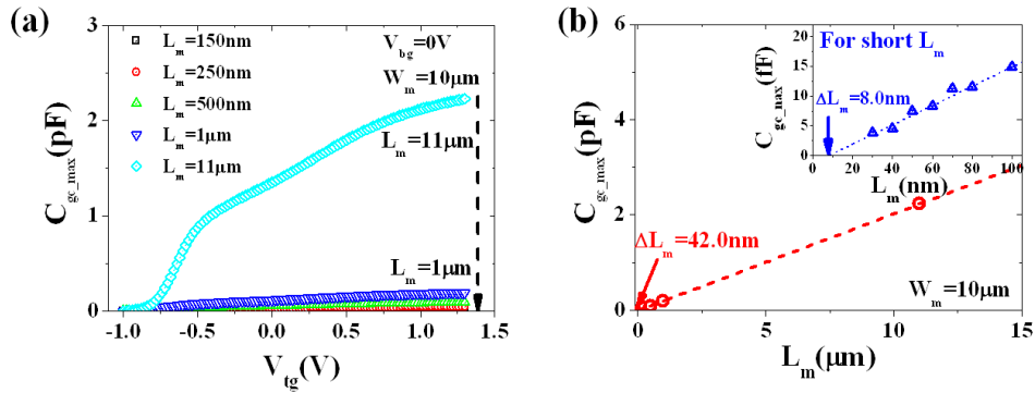
Figure 4-4 (a) Representative C_{gc\_max}(V_{tg}) curves for N-type JLTs ( L_m=150\text{nm} to 11\mu\text{m} with fixed W_m=10\mu\text{m} ). (b) C_{gc\_max} versus L_m for extraction of \Delta L_m ( \approx 42\text{nm} ). (Inset: Same data procedures in short channel JLTs ( L_m \leq 100\text{nm} ) for \Delta L_m ( \approx 8\text{nm} ) evaluation).
