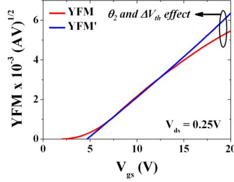
Figure 2-10 Comparison between YFM and YFM' after consideration of \theta_2 and \Delta V_{th} .
