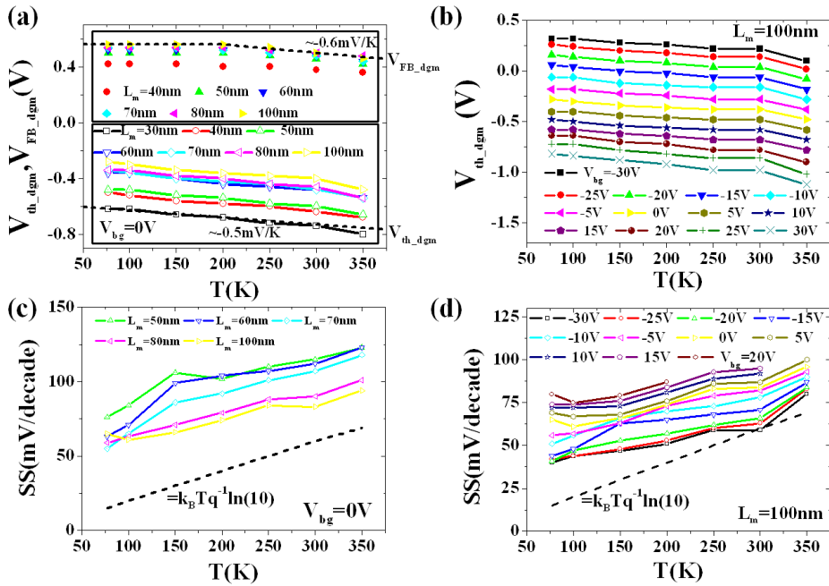
Figure 4-8 (a) The temperature dependence of V_{th,dgm} and V_{FB,dgm} versus L_m and (b) that of V_{bg} dependence in L_m=100\text{nm} JLT. (c) The temperature behavior of SS at V_{bg}=0\text{V} with respect to L_m and (d) that of V_{bg} reliance in L_m=100\text{nm} JLT.
