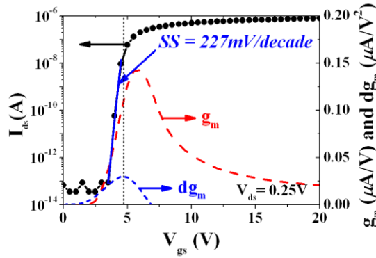
Figure 2-8 Subthreshold characteristic of PMMA passivated \text{SnO}_2 FET.
