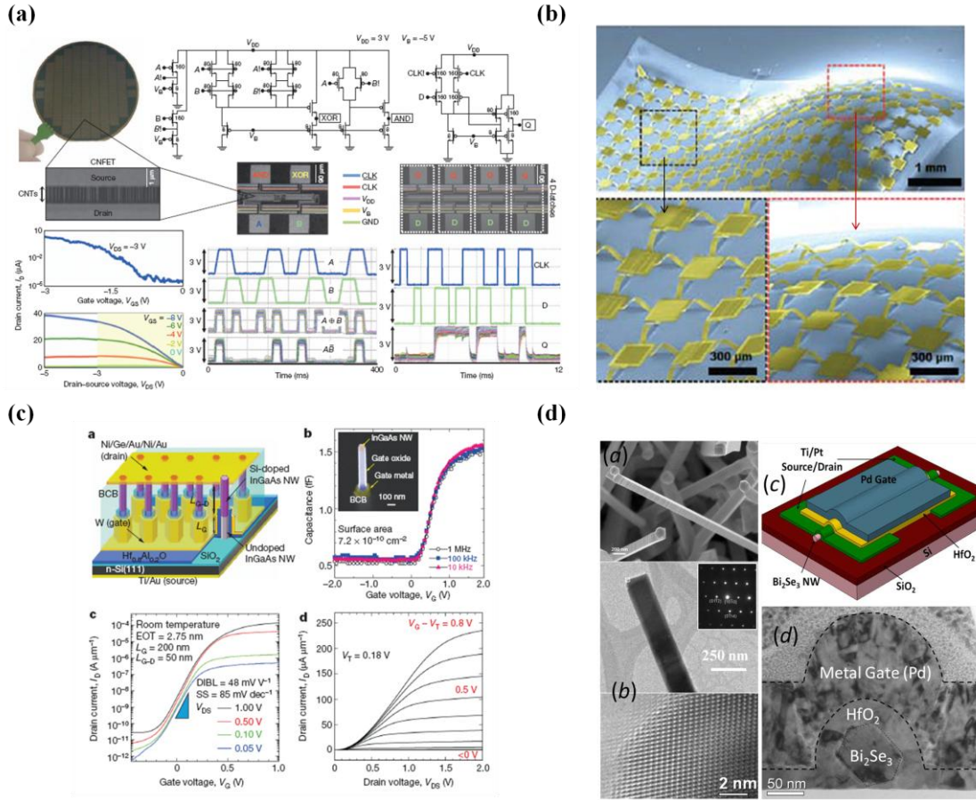
Figure 1-14 (a) Characteristics of CNT-FET subcomponents operating circuit for CNT computer[26] (b) Stretchable logic inverters based on \text{SnO}_2 semiconducting nanowires[27] (c) A III-V nanowire channel on silicon for high-performance vertical transistors[30] (d) Topological insulator \text{Bi}_2\text{Se}_3 nanowire for high performance FETs[32].
