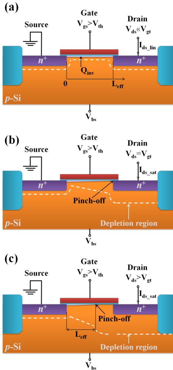
Figure 2-2 Cross-section view of an n-type MOSFET (a) in linear with very small V_{ds} , (b) at onset of saturation (or weak inversion), and (c) deep saturation regime.
