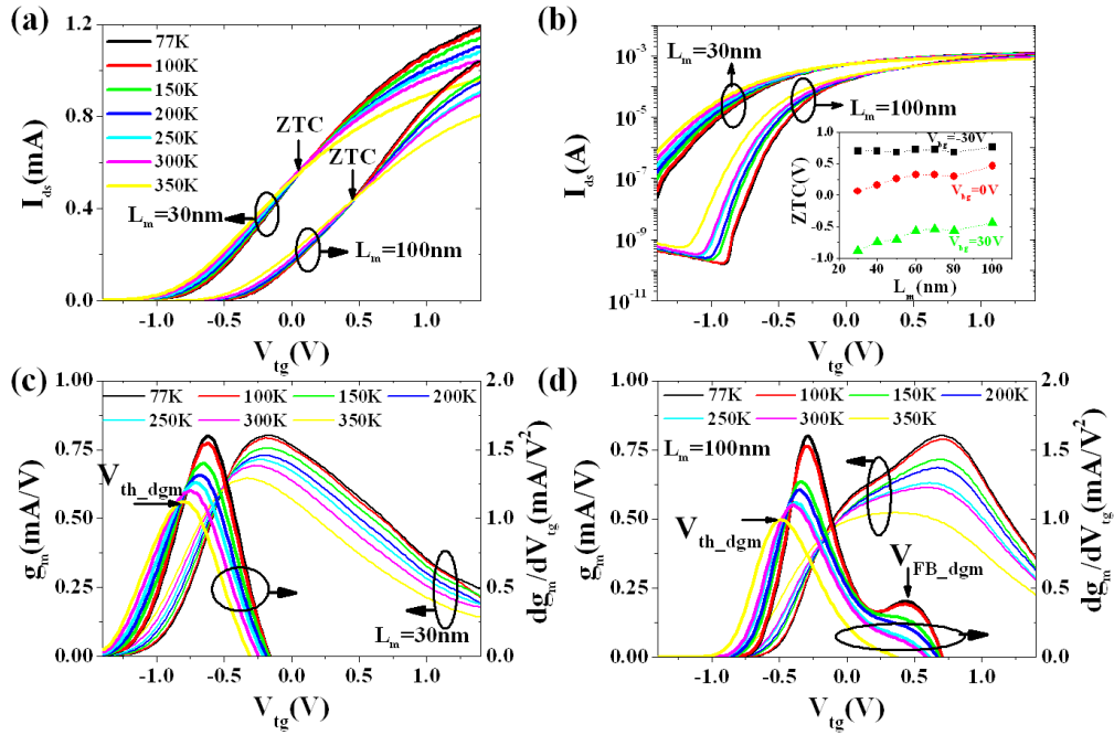
Figure 4-6 The representative (a) linear and (b) log scaled transfer curves in L_m=30\text{nm} and 100\text{nm} JLTs with varying T (77K to 350K). (Inset: ZTC versus L_m depending on V_{bg} ) The temperature dependence of g_m (left axis) and dg_m/dV_{tg} (right axis) of (c) L_m=30\text{nm} and (d) L_m=100\text{nm} JLTs, respectively.
