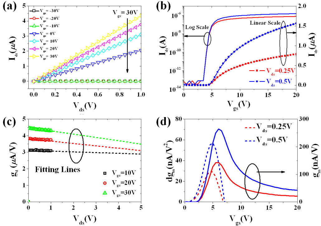
Figure 2-3 Representative examples of (a) output characteristics, (b) transfer curves, (c) drain conductance ( =\partial I_{ds}/\partial V_{ds} ), and (d) transconductance curves ( =\partial I_{ds}/\partial V_{gs} ) of fabricated n-type long channel \text{SnO}_2 FET. Detailed electrical analysis will be presented in Chap. 5.
