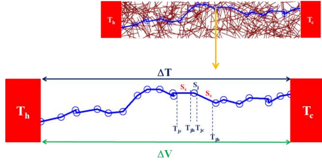
Figure 7-4 A representative random network generated by a numerical simulation (top) and one of dominant paths in s-SWCNT network for TEP calculation (bottom).
