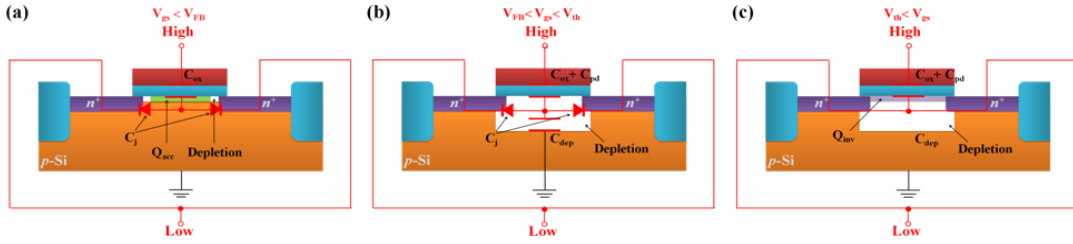
Figure 2-12. Equivalent circuit models for C_{gc} measurement depending on the conduction regimes, (a) accumulation, (b) depletion, and (c) inversion, respectively.[7]
