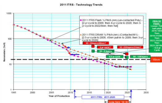
Figure 1-2 2011 International Technology Roadmap of Semiconductors (ITRS)-Dynamic Random Access memory (DRAM) and Flash memory half pitch trends. [ http://www.itrs.net/ ]
