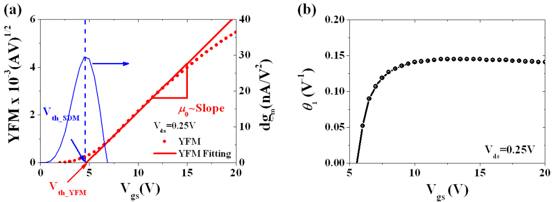
Figure 2-9 (a) YFM and dg_m , and (b) \theta_1 curves of PMMA passivated SnO_2 FET as a function of V_{gs} .
