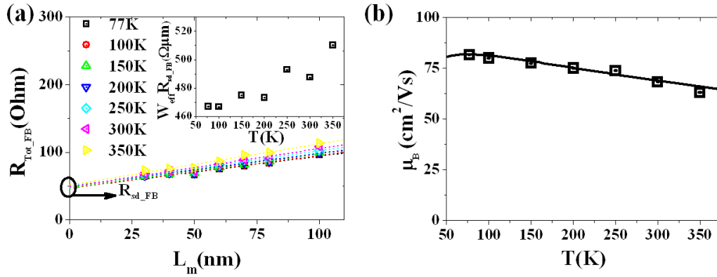
Figure 4-9 (a) The temperature dependence of R_{tot\_FB} with respect to L_m . Fitting curves (dotted lines) are plotted together with data (symbols). (Inset: The temperature dependence of W_{eff} normalized R_{sd\_FB} ) (b) The temperature dependence of \mu_B and corresponding fitting curve with account for various mobility fitting components ( \mu_{ph} , \mu_C , \mu_{neu} , and \gamma )
