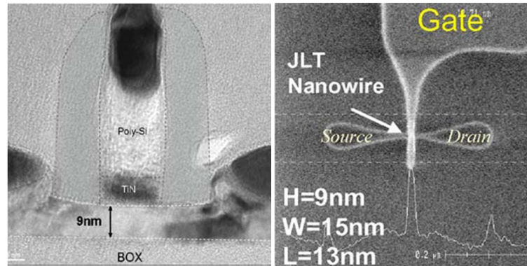
Figure 4-2 Representative (a) TEM and (b) SEM images of cross-sectional tri-gate nanowire JLTs.[3]
