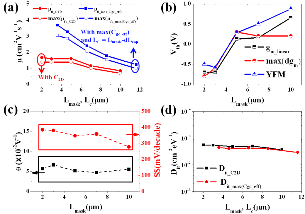
Figure 19 (a) \mu_0 extracted from C 2D with L_{mask} (red lines) and \mu_{fe} from \max(C_{gc\_eff}) with L_c (blue lines), respectively (b) V_{th} versus L_{mask} based on various V_{th} evaluation techniques (c) \theta (circle) and SS (rectangular) with respect to different L_{mask} (d) D_{it} extracted from C 2D with L_{mask} (rectangular) and \max(C_{gc\_eff}) with L_c (circle), respectively.
