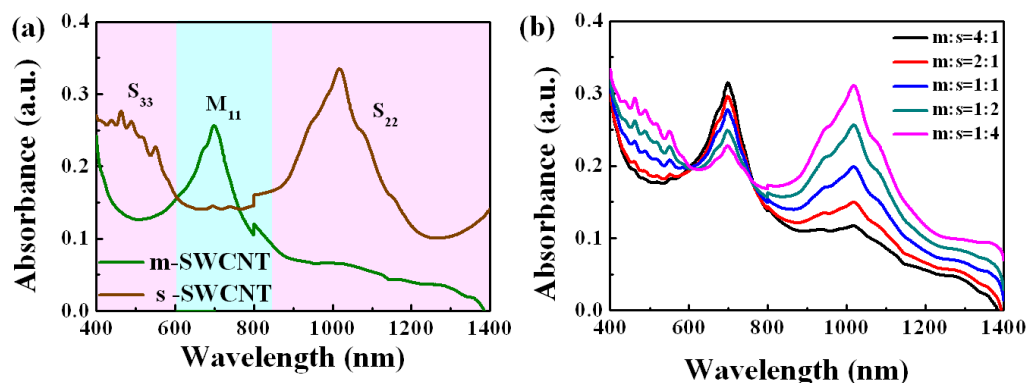
Figure 7-2 (a) The UV-vis-NIR absorbance of the type separated m- and s-SWCNT dispersions and (b) that of the mixtures with varying m:s ratio.
