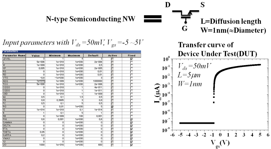
Figure 6-9. Various electrical parameter list of N-type silicon semiconducting NW in P-Spice simulator and its corresponding representative transfer curves. ( V_{ds} = 50 \text{ mV} , silicon channel length and width are 5 \mu\text{m} and 1 \text{ nm} , respectively.)
