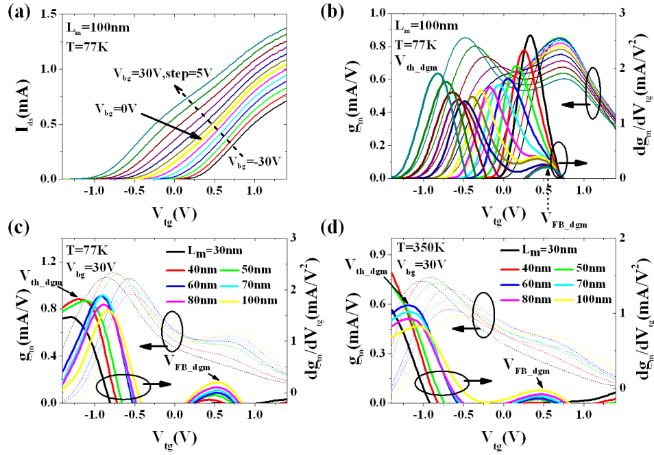
Figure 8 (a) Various transfer curves of L_m=100\text{nm} JLT at T=77\text{K} depending on different V_{bg} (b) g_m (left axis) and dg_m/dV_{tg} (right axis) curves. Same graphs at V_{bg}=30\text{V} with (c) T=77\text{K} and (d) T=350\text{K} with respect to L_m , respectively.
