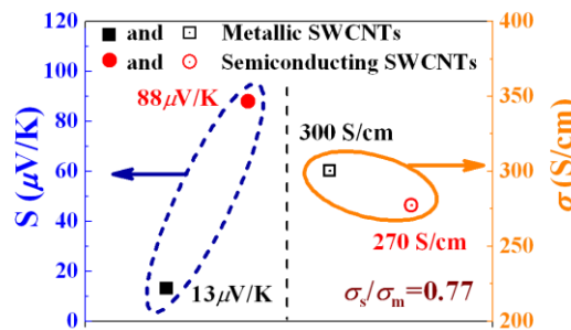
Figure 7-3 The measured TEP and electrical conductivity of the type separated m- and s-SWCNT thin films.
