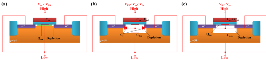
Figure 2-13. Equivalent circuit models for C_{tot} measurement depending on the conduction regimes, (a) accumulation, (b) depletion, and (c) inversion, respectively.[7]
