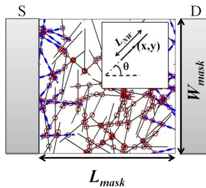
Figure 3-4 A representative realized array set of a 2D RN-CWs with L_{mask} = W_{mask} = 3\mu m with \rho_{CW} = 10/\mu m^2 . [10]
