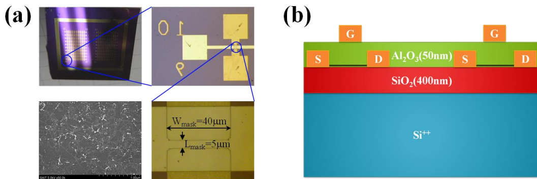
Figure 16 (a) Optical images of RN-TFTs and a representative SEM image of synthesized single-walled CNTs. (b) A simplified cross section view of fabricated top-gate RN-TFTs.
