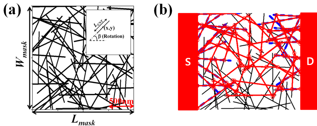
Figure 21 (a) A representative randomly generated set of 2D RN-TFTs (in case of L_{mask}=W_{mask}=2\mu m , \rho_{CNT}=20/\mu m^2 and L_{CNT}=1\mu m ) (b) Visualized all possible optimal pathways (red lines) from CNTs directly connected to S to D electrode (blue dotted line) in the case of Fig. 21(a). (Junction points between CNTs: small red circles)
