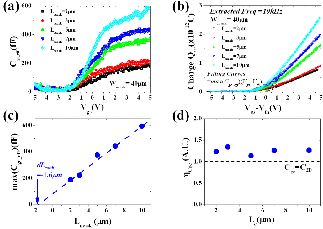
Figure 18 (a) C_{gc\_eff}(V_{gs}) curves of a top-gate RN-TFTs at f=10kHz (b) Q_{acc}(V_{gs}) (symbols) with linear fitting lines ( \approx \max(C_{gc\_eff}) \times (V_{gs} - V_{th}) , dotted lines) (c) \max(C_{gc\_eff}) and (d) \eta_{Cgc} verses L_{mask} and L_C , respectively.
