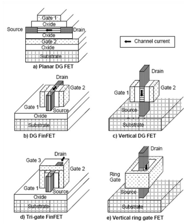
Figure 1-11 Several types of multi-gate MOSFETs structure.[17]
