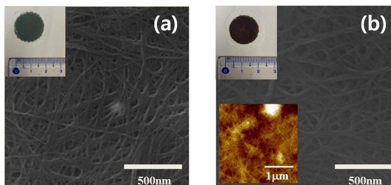
Figure 7-1 Representative SEM images of high-purity (a) m-SWCNT (b) and s-SWCNT thin films, respectively. Insets show their photographs after filtration. Additionally, atomic force microscope image of s-SWCNTs also presented in inset (b).
