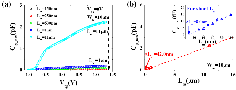
Figure 5 (a) Representative C_{gc\_max}(V_{tg}) curves for N-type JLTs ( L_m=150nm to 11μm with fixed W_m=10μm ). (b) C_{gc\_max} versus L_m for extraction of \Delta L_m (≈42nm). (Inset: Same data procedures in short channel JLTs ( L_m \leq 100nm ) for \Delta L_m (≈8nm) evaluation).
