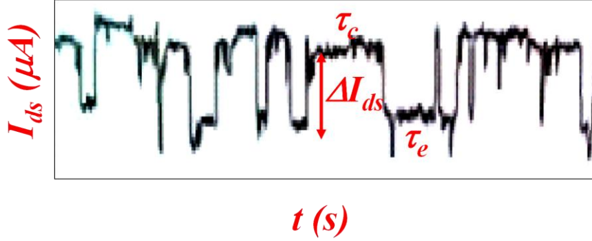
Figure 2-20 Typical I_{ds} as a function of time for RTS noise pattern in JLT. ( W_m=L_m=100\text{nm} )
