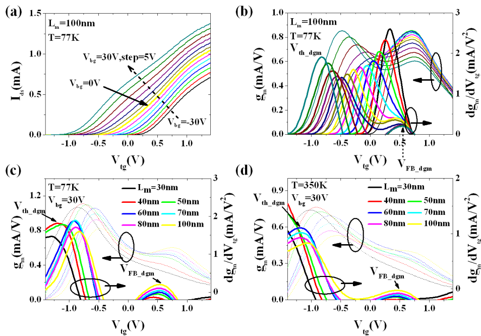
Figure 4-7 (a) Various transfer curves of L_m=100\text{nm} JLT at T=77\text{K} depending on different V_{bg} (b) g_m (left axis) and dg_m/dV_{tg} (right axis) curves. Same graphs at V_{bg}=30\text{V} with (c) T=77\text{K} and (d) T=350\text{K} with respect to L_m , respectively.
