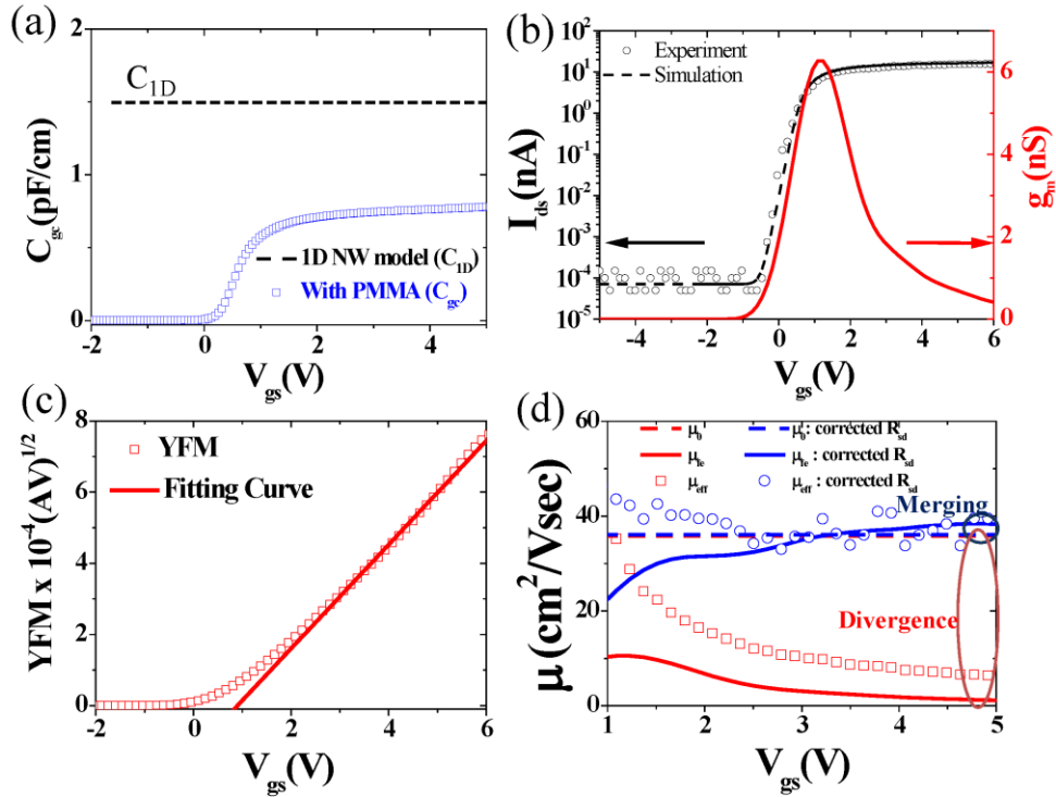
Figure 14 (a) Comparison capacitance values between the C_{1D} and simulated C_{gc}(V_{gs}) (open rectangular) respect to back-gate bias. (b) I_{ds}(V_{gs}) (open circle) and g_m(V_{gs}) (line) of SnO 2 NW-FET at V_{ds}=0.25V . Simulated I_{ds}(V_{gs}) (dotted circle) is added for comparison. (c) YFM( V_{gs} ) curve with linear fitting line. (d) Comparison of various mobility ( \mu_0 , \mu_{fe} , \mu_{eff} ) before and after R_{sd} correction.
