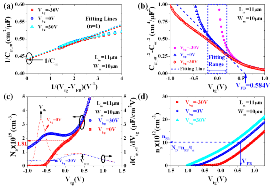
Figure 4-5 (a) 1/C_{gc\_eff} of N-type JLTs ( L_m=11\mu\text{m} with W_m=10\mu\text{m} ) with respect to V_{bg} (-30V to 30V) for C_{ox} and corresponding CET extraction in high V_{tg} regime. (b) 1/C_{gc\_eff}^2 - 1/C_{ox}^2 of N-type of JLTs for V_{FB} evaluation in partially depleted region (c) N_D based on Eq. (4-4) (left axis) and dC_{gc\_eff}/dV_{tg} (right axis) curves of N-type of JLTs. (d) n_s versus V_{tg} curves for N_D estimation with account for the position of V_{FB} .
