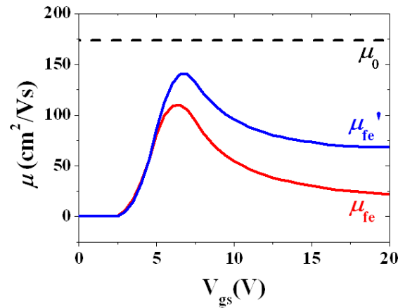
Figure 2-5 Comparison of various mobility values ( \mu_0 , \mu_{fe} , and \mu_{fe}' ) in PMMA passivated \text{SnO}_2 FET.
