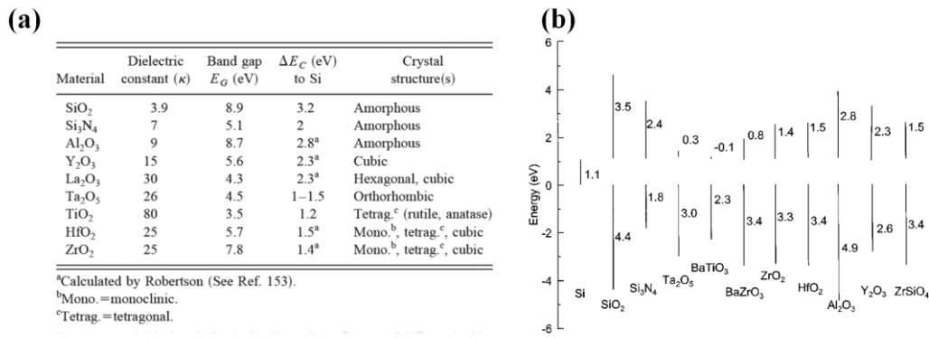
Figure 1-12 (a) Comparison table of relevant properties of potential candidates of high- \kappa dielectric materials and (b) corresponding band offset calculation result.[21]
