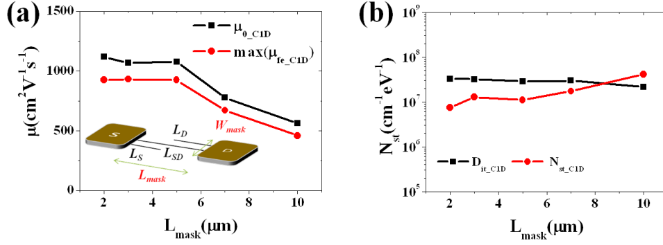
Figure 6-11 \mu_0 and \mu_{fe} extracted from C_{1\text{D}} (inset: simplified device configuration of RN-TFTs for the split CV measurements) (b) Recalculated N_{\text{st}} and D_{\text{it}} with C_{1\text{D}} versus L_{\text{mask}} , respectively.
