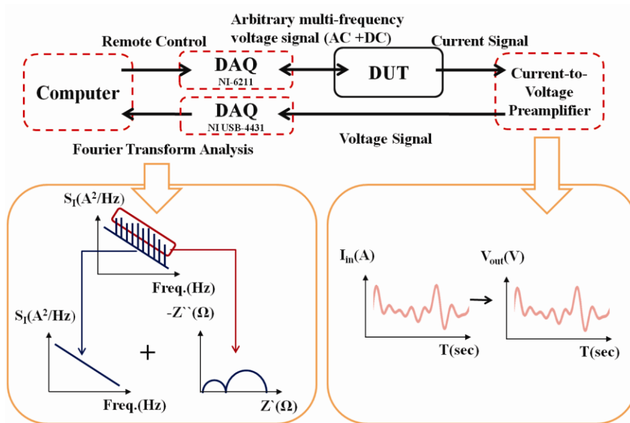
Figure A-1 The simplified schematic of an in-situ Nyquist and electrical noise meter for transient measurements: Two DAQ system can be integrated into one DAQ. The signals of the noise or the impedance can be extracted and optimized by tuning the amplification factors and the measurement range
