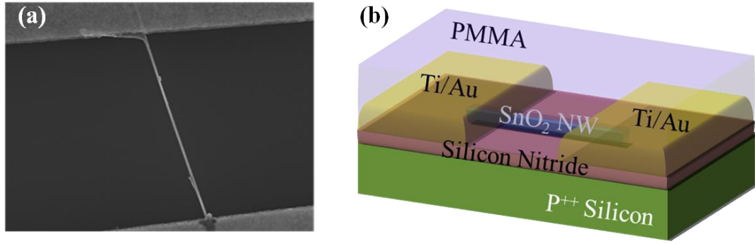
Figure 13 (a) FESEM image of SnO 2 NWs and (b) a simplified 3D structure of PMMA passivated SnO 2 NW-FET.
