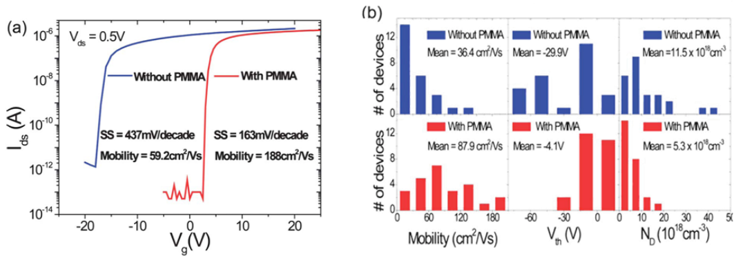
Figure 5-1 (a) Representative transfer curves of SnO 2 NW-FETs and (b) histogram of field effect mobility, V_{th} , and carrier concentration for with and without PMMA passivation layer at V_{ds}=0.5 V.[15]
