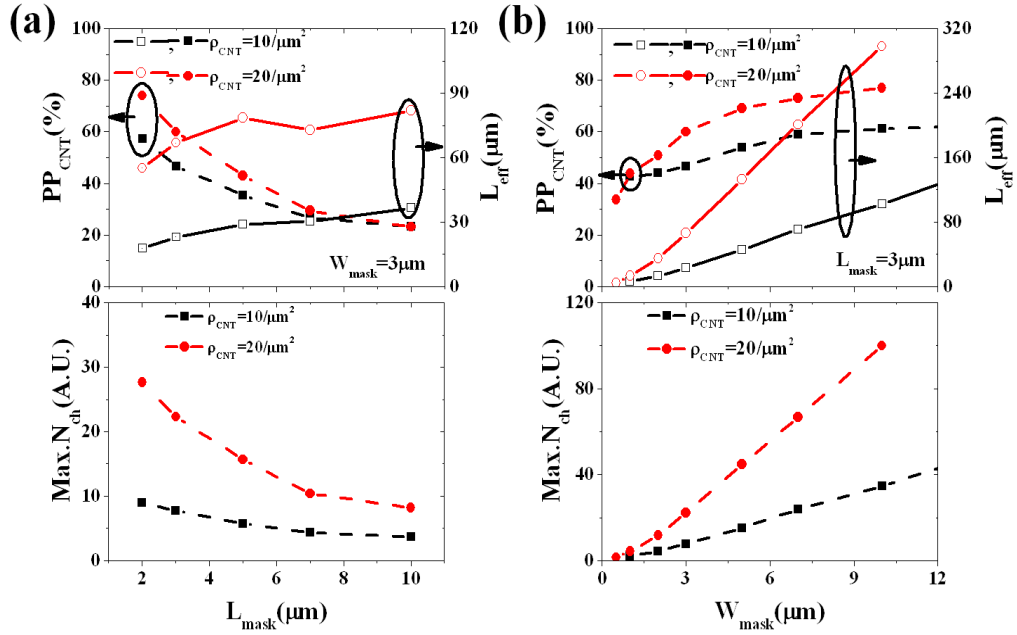
Figure 22 (a) PR CNT and corresponding L eff (top), and Max.N ch (bottom) depending on L mask with fixed W mask = 3 μm (b) Same parameters depending on W mask with fixed L mask = 3 μm.
