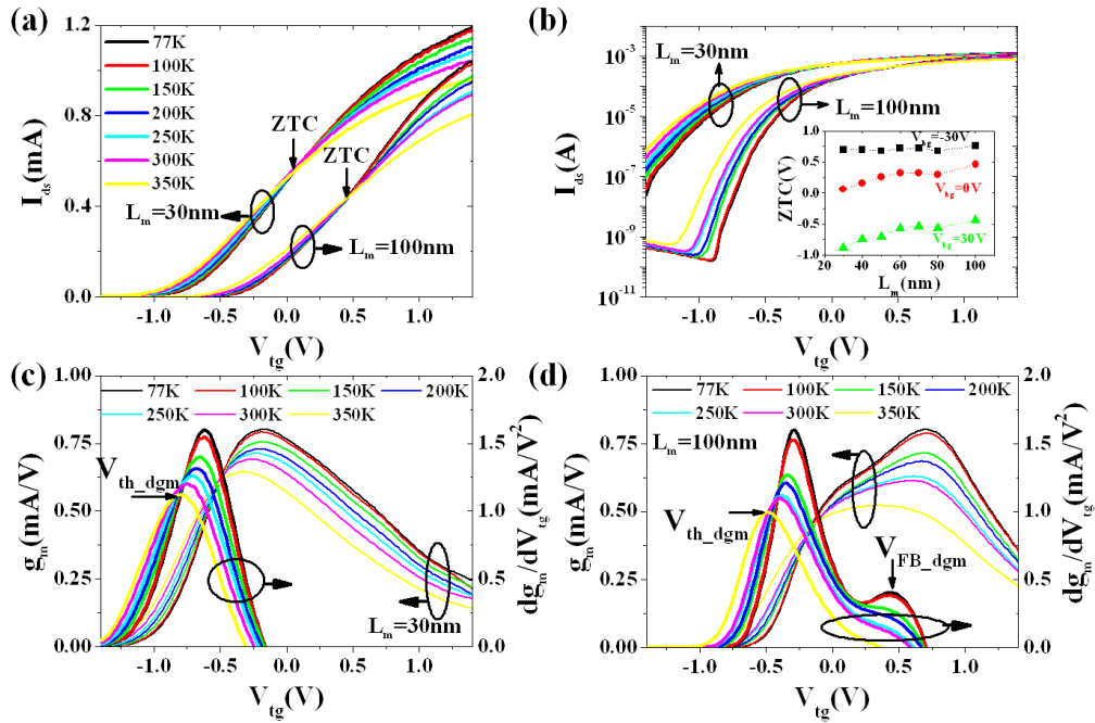
Figure 7 The representative (a) linear and (b) log scaled transfer curves in L_m=30nm and 100nm JLTs with varying T (77K to 350K). (Inset: ZTC versus L_m depending on V_{bg} ) The temperature dependence of g_m (left axis) and dg_m/dV_{tg} (right axis) of (c) L_m=30nm and (d) L_m=100nm JLTs, respectively.
