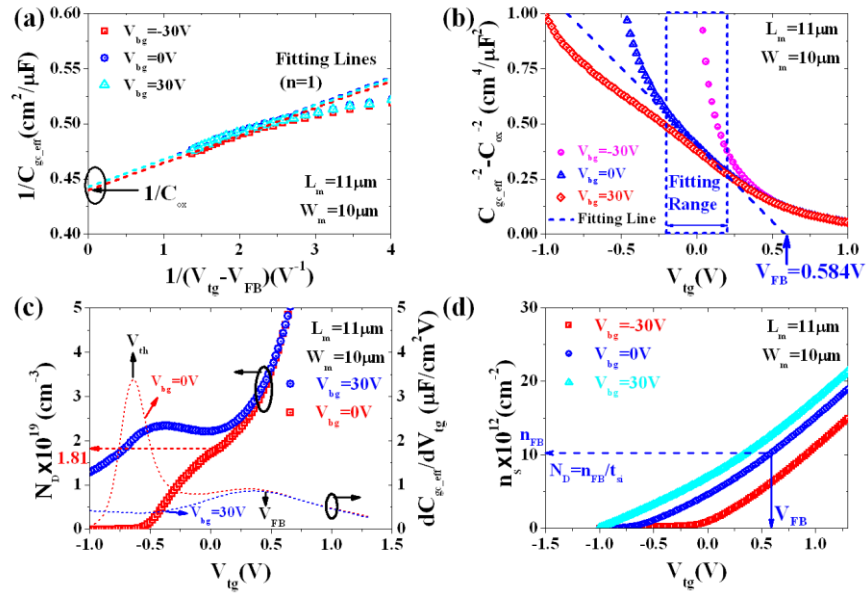
Figure 6 (a) 1/C_{gc\_eff} curves ( L_m=11\mu m with W_m=10\mu m ) with respect to V_{bg} (-30V to 30V) for C_{ox} determination (b) C_{gc\_eff}^{-2} - C_{ox}^{-2} behaviors for V_{FB} extraction in partially depleted region (c) N_D estimation based on Maserjian's function (left axis) and dC_{gc\_eff}/dV_{tg} (right axis) curves (d) n_s versus V_{tg} curves for N_D evaluation at V_{FB}
