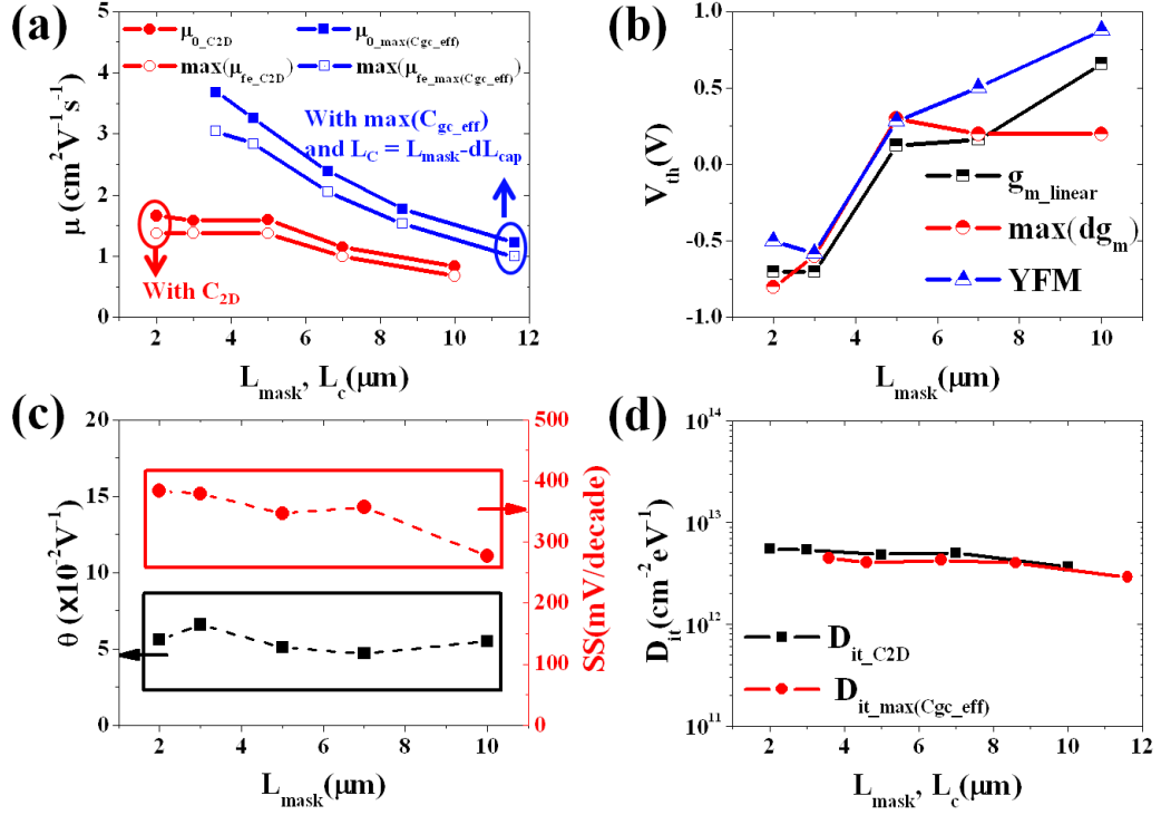
Figure 6-4 (a) \mu_0 extracted from C_{2D} with L_{\text{mask}} (red lines) and \mu_{fe} from \max(C_{gc\_eff}) with L_c (blue lines), respectively (b) V_{th} versus L_{\text{mask}} based on various V_{th} evaluation techniques (c) \theta (circle) and SS (rectangular) with respect to different L_{\text{mask}} (d) D_{it} extracted from C_{2D} with L_{\text{mask}} (rectangular) and \max(C_{gc\_eff}) with L_c (circle), respectively.
