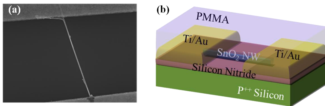
Figure 5-2 (a) FE-SEM image of \text{SnO}_2 NWs and (b) a simplified 3D structure of PMMA passivated \text{SnO}_2 NW-FET.
