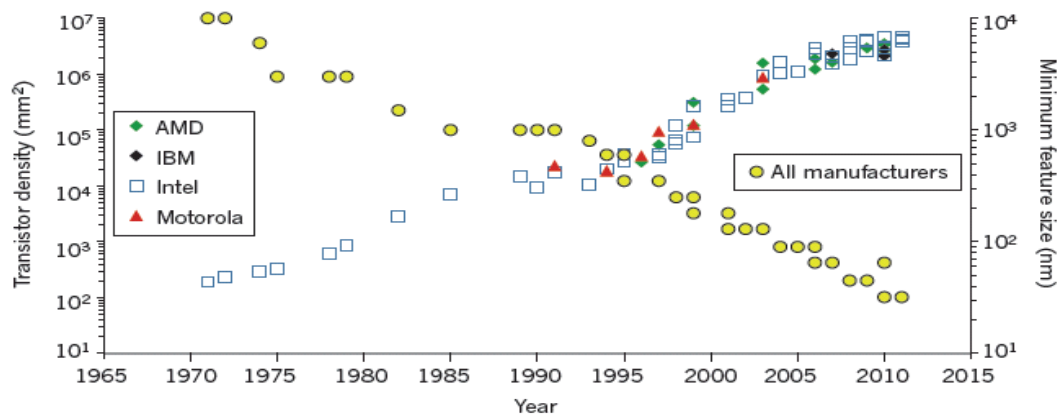
Figure 1 Trend of the gate length miniaturization and the density of transistors in microprocessors over time [1]
