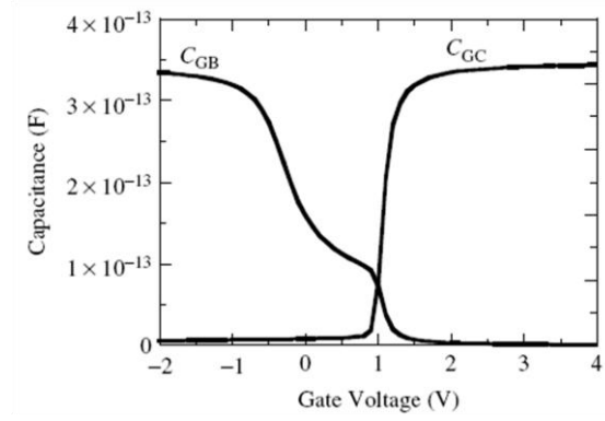
Figure 2-14 Typical split CV ( C_{gb} and C_{gc} ) curves as a function of V_{gs} . [5]
