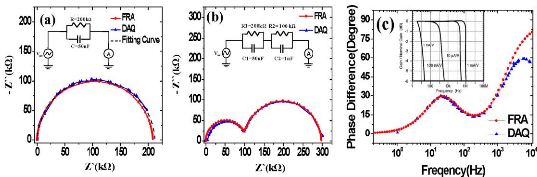
Figure A-2 The Nyquist plots obtained using various methods (FRA(circle), DAQ (triangle)) with (a) a parallel RC circuit and with (b) two different series parallel RC circuits. Inset: The test circuit for one R/C circuit (a) R=200k\Omega/C=50nF and two R/C circuits (b) R1=200k\Omega/C1=50nF and R2=100k\Omega/C2=1nF . (c) The frequency dependence of the phase difference in case of (b) (inset: the frequency dependence of gain of the SR570 preamplifier)
