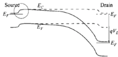
Figure 1-5 Energy-band diagrams at the semiconducting surface from source to drain, for (a) long and (b) short channel MOSFET, respectively.[9]
