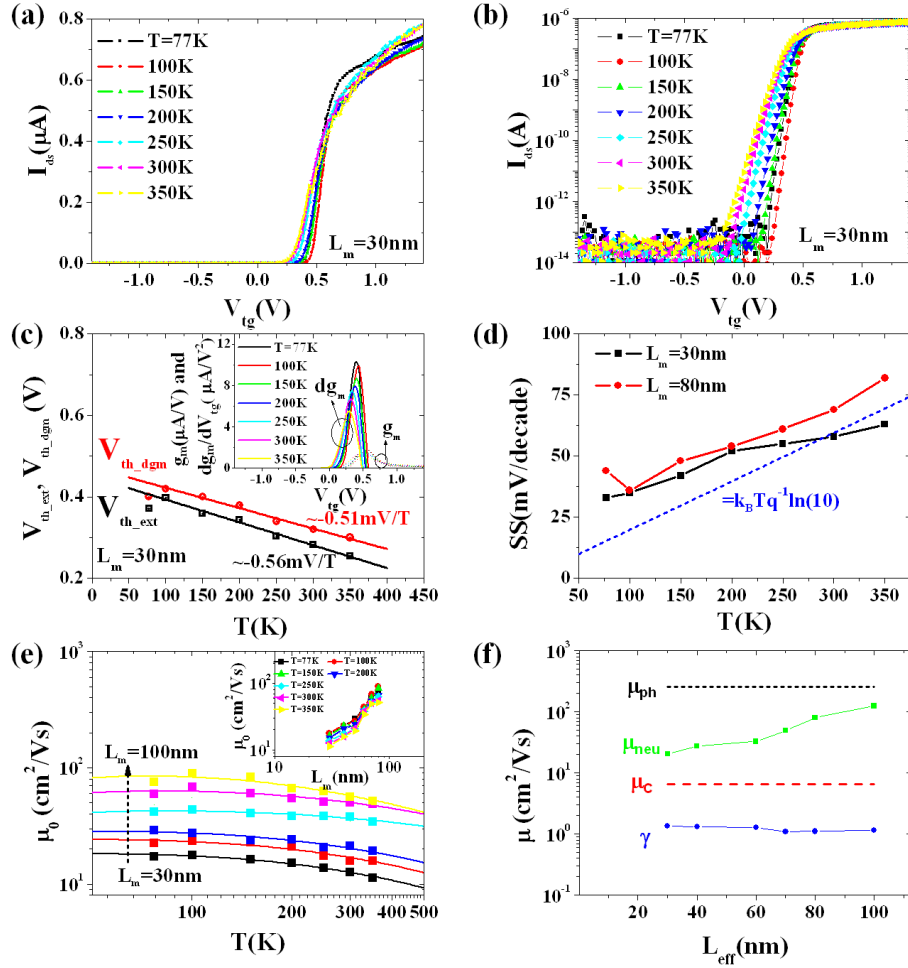
Figure 4-11 The representative (a) linear and (b) log scaled transfer curves as a function of V_{tg} in L_m=30\text{nm} tri-gate NW shape JLTs with varying T (77K to 350K). (c) The temperature dependence of V_{th\_dgm} and V_{th\_ext} . (Inset: g_m and dg_m/dV_{tg} curves) (d) The temperature behavior of SS (e) \mu_0 extracted from YFM as a function of T depending on L_m (Inset: \mu_0 versus L_m with varying T ) (f) Various mobility fitting components ( \mu_{ph} , \mu_C , \mu_{neu} , and \gamma ) for \mu_0 depending on L_m .
