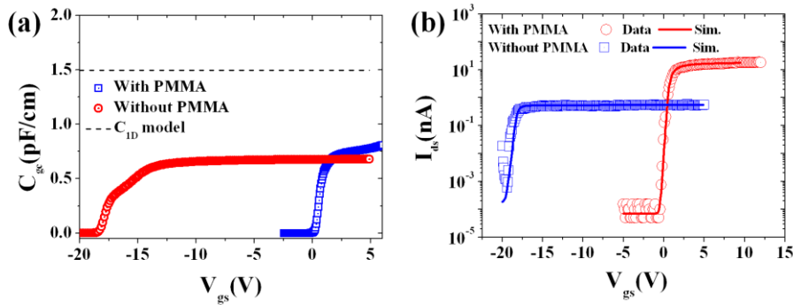
Figure 5-4 (a) Comparison capacitance values between the C_{1D} and simulated C_{gc}(V_{gs}) with and without PMMA passivation layer respect to back-gate bias. (b) I_{ds}(V_{gs}) of \text{SnO}_2 NW-FET with and without PMMA passivation layer at V_{ds}=0.25\text{V} .
