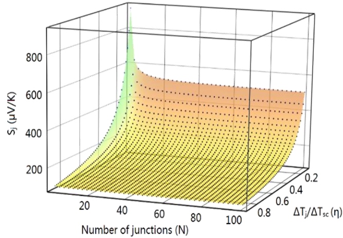
Figure 7-6 The calculated junction TEP as a function of the number of junctions (N) and factor \eta
