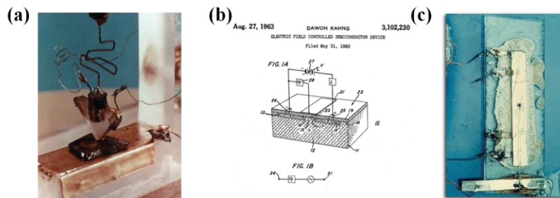
Figure 1-1 Photographs of the firstly developed (a) BJT (in 1947), (b) MOSFET (in 1960), and (c) IC (in 1961), respectively.
