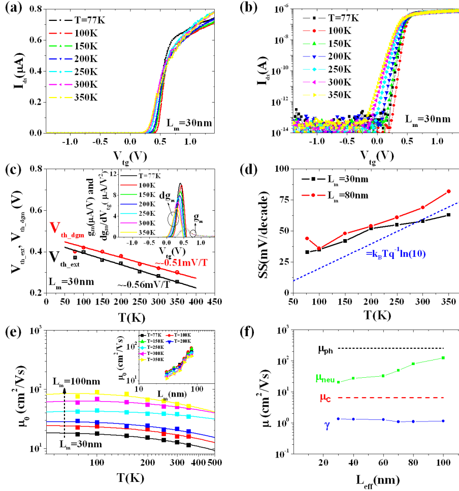
Figure 12 The representative (a) linear and (b) log scaled transfer curves as a function of V_{tg} in L_m=30\text{nm} tri-gate NW shape JLTs with varying T (77K to 350K). (c) The temperature dependence of V_{th\_dgm} and V_{th\_ext} . (Inset: g_m and dg_m/dV_{tg} curves) (d) The temperature behavior of SS (e) \mu_0 extracted from YFM as a function of T depending on L_m (Inset: \mu_0 versus L_m with varying T ) (f) Various mobility fitting components ( \mu_{ph} , \mu_c , \mu_{neu} , and \gamma ) for \mu_0 depending on L_m .
