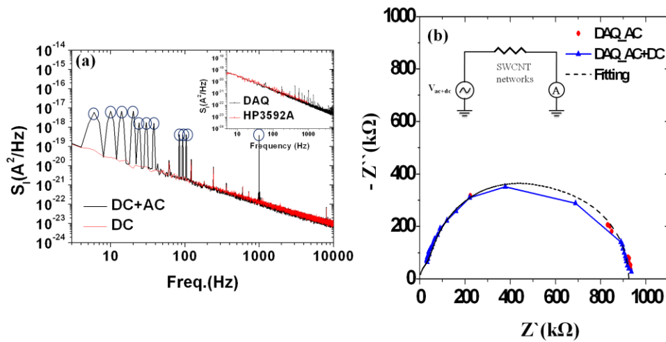
Figure A-4 (a) Comparison of the current power spectra obtained from SWCNT-FET with only DC (2V) bias or both AC and DC (2V). The dark open circles corresponded to the applied AC frequencies for getting the Nyquist plot. The inset shows the noise spectra obtained by each single noise meas-
