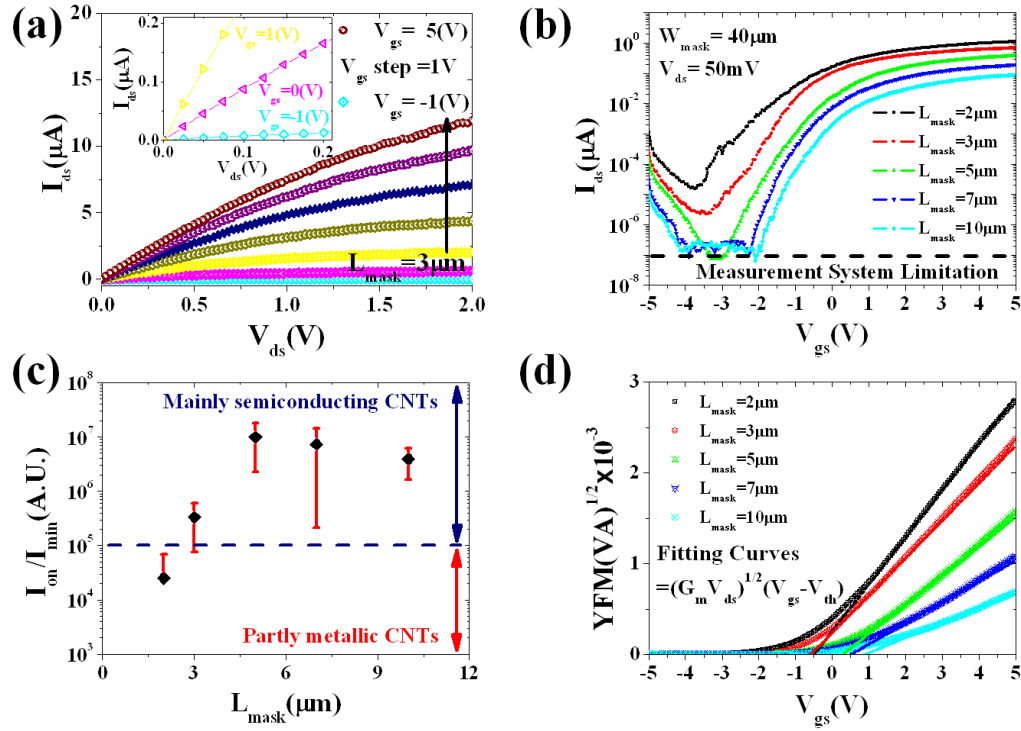
Figure 6-2 (a) Representative output characteristic I_{ds}(V_{ds}) curves of RN-TFTs depending on V_{gs} (from V_{gs}=-1V to 5V with V_{gs}=1V step) in case of L_{mask}=3\mu m . (inset: the magnification view of small V_{ds} region) (b) Typical transfer I_{ds}(V_{gs}) curves with respect to different L_{mask} at V_{ds}=50mV (c) I_{on} and I_{min} ratio versus L_{mask} (d) YFM(V_{gs}) (symbols) and corresponding fitting curves (dotted lines) with respect to L_{mask} .
