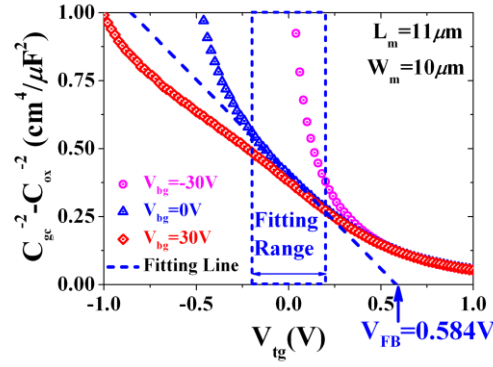
Figure 2-16 C_{gc}(V_{tg})^{-2} - C_{ox}^{-2} curves of N-type JLT depending on V_{bg} .
