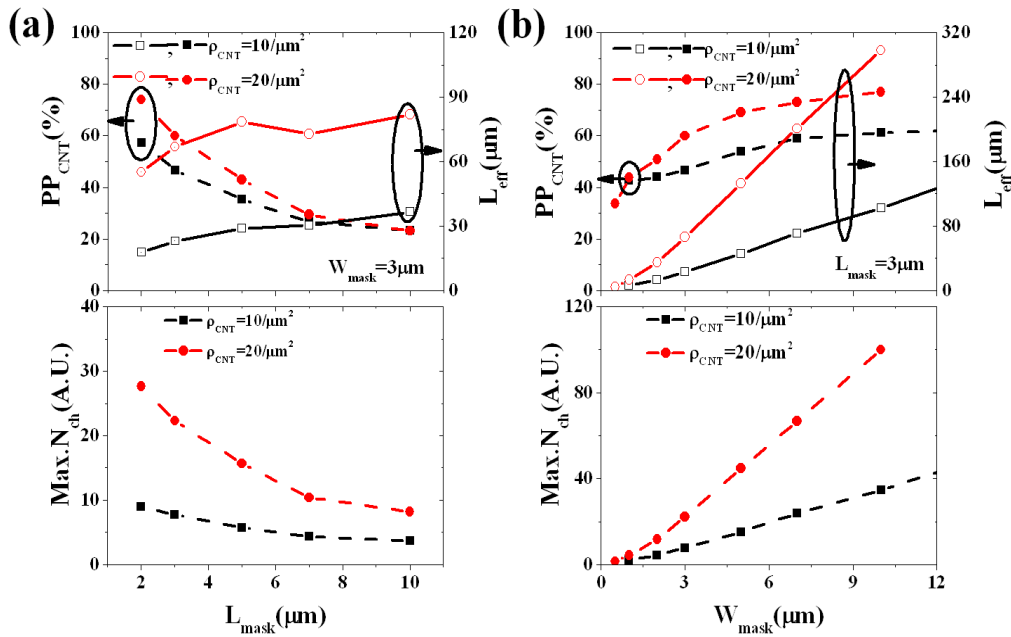
Figure 6-7 (a) \text{PR}_{\text{CNT}} and corresponding L_{\text{eff}} (top), and \text{Max.N}_{\text{ch}} (bottom) depending on L_{\text{mask}} with fixed W_{\text{mask}} = 3 \mu\text{m} (b) Same parameters depending on W_{\text{mask}} with fixed L_{\text{mask}} = 3 \mu\text{m} .
