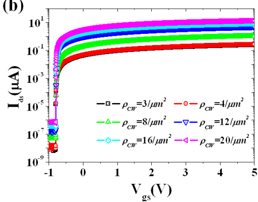
Figure 3-10. SPICE simulation results of output characteristics I_{ds}(V_{ds}) and transfer curve I_{ds}(V_{gs}) curves depending on different \rho_{cw} ( L_{mask}=W_{mask}=3\mu m )
