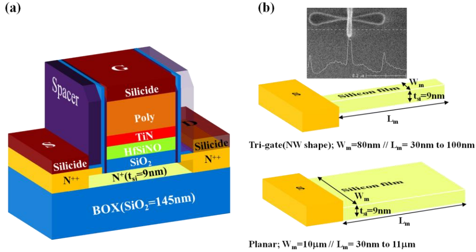
Figure 4 (a) Simplified three-dimensional device structure and (b) on-mask splits ( L_m and W_m ) for planar and nanowire(NW) shape of JLTs with a representative SEM (Scanning Electron Microscope) image of NW JLT
