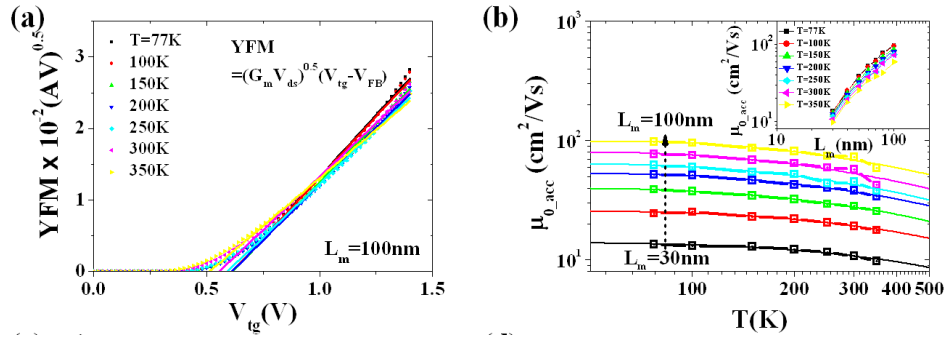
Figure 11 (a) T dependence of YFM in accumulation regime in the case of L_m=100\text{nm} JLT. (b) \mu_{0\_acc} as a function of T depending on L_m (Inset: \mu_{0\_acc} versus L_m with varying T)
