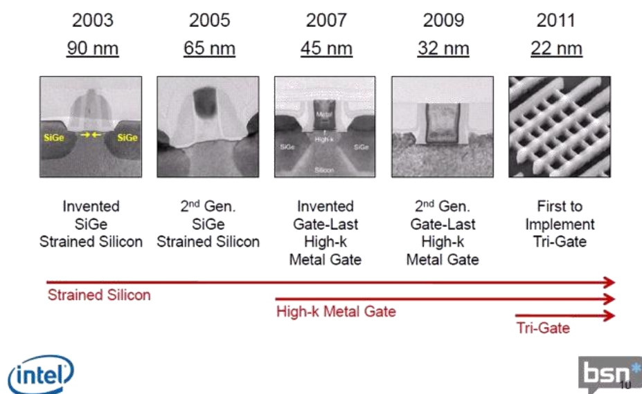
Figure 2-1 Intel's Transistor Leadership over generations: 90nm, 65nm, 45nm, 32nm and 22nm. Three major inventions: SiGe, HKMG (High- \kappa metal gate) and Tri-Gate structure. [ http://www.intel.com , http://www.brightsideofnews.com ]
