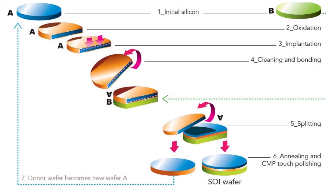
Figure 1-10 Fabrication process of manufacturing ultrathin SOI via Smart Cut process [ http://www.soitec.com/en/technologies/smart-cut/ ]
