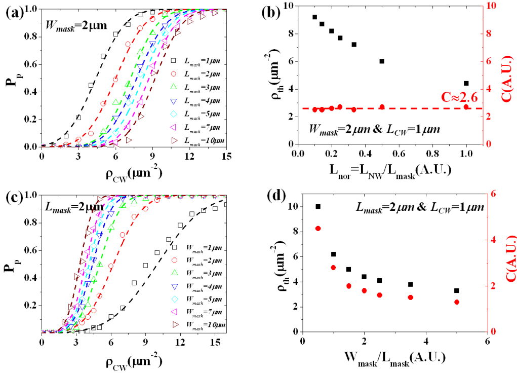
Figure 3-8 Percolation probability ( P_p ) variation with \rho_{CW} as a function of L_{mask} for fixed W_{mask}=2\mu m , and (b) corresponding erf fitting parameters. Figs (c) and (d) are the same figure as a function of W_{mask} with fixed L_{mask}=2\mu m . [10]
