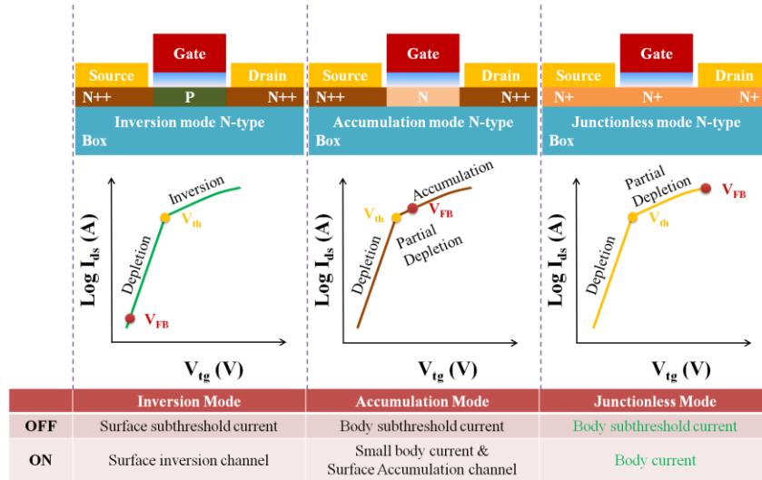
Figure 4-1 Comparison of conduction mode of advance MOS transistors (Left: Inversion mode, Middle: Accumulation mode, Right: Junctionless mode)
