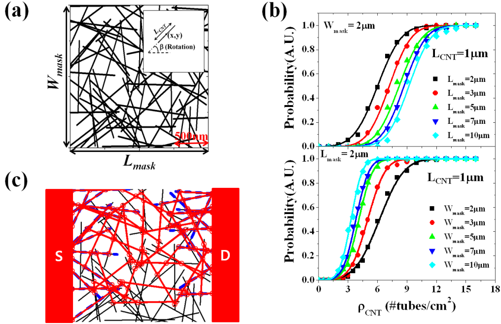
Figure 6-6 (a) A representative randomly generated set of 2D RN-TFTs (in case of L_{mask}=W_{mask}=2\mu m , \rho_{CNT}=20/\mu m^2 and L_{CNT}=1\mu m ) (b) P dependency on \rho_{CNT} as a function of L_{mask} for fixed W_{mask}=2\mu m (top) and P as a function of W_{mask} for fixed L_{mask}=2\mu m (bottom) (c) Visualized all possible optimal pathways (red lines) from CNTs directly connected to S to D electrode (blue dotted line) in the case of Figure 6(a). (Junction points between CNTs: small red circles)
