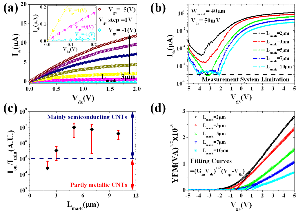
Figure 17 (a) Representative output characteristic I_{ds}(V_{ds}) curves of RN-TFTs depending on V_{gs} in case of L_{mask}=3\mu m . (inset: the magnification view of small V_{ds} region) (b) Typical transfer I_{ds}(V_{gs}) curves with respect to different L_{mask} at V_{ds}=50mV (c) I_{on} and I_{min} ratio versus L_{mask} (d) YFM( V_{gs} ) (symbols) and corresponding fitting curves (dotted lines) with respect to L_{mask} .
