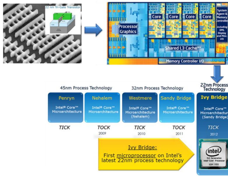
Figure 1-3 Intel's 22nm technology for FinFET structure and Intel core i7-3770K (22nm Ivy Bridge) [http://newsroom.intel.com/docs/DOC-2032]
