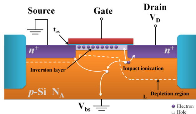
Figure 1-7 Illustration of impact ionization near drain region in N-type MOSFET.
