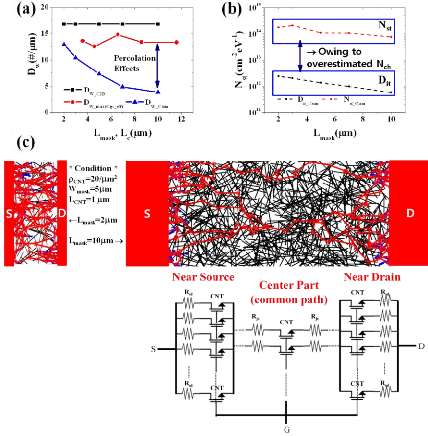
Figure 23 (a) D_W based on C_{2D} , \max(C_{gc\_eff}) , and C_{Sim} (b) N_{st} and D_{it} extracted from C_{Sim} (c) Comparison the effective D_{W\_Csim} between L_{\text{mask}} = 2 \mu\text{m} and L_{\text{mask}} = 10 \mu\text{m} with fixed W_{\text{mask}} = 5 \mu\text{m} in random network system. (Simplified electrical equivalent circuit was displayed)
