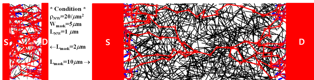
Figure 3-1 A representative numerical percolation simulation result for comparison between L_{\text{mask}}=2\mu\text{m} and L_{\text{mask}}=10\mu\text{m} with fixed W_{\text{mask}}=5\mu\text{m} with the fixed nanowire density ( \rho_{\text{NW}}=20/\mu\text{m}^2 ) in random network system.[9]
