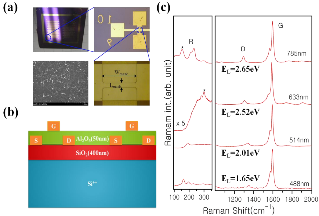
Figure 6-1 (a) Optical images of RN-TFTs and a representative SEM image (Hitachi, S-5500) of synthesized single-walled CNTs (b) A simplified cross section view of fabricated top-gate RN-TFTs. (c) Raman spectra of active channel areas of single-walled CNTs obtained with four different laser excitations ( 1.65\text{eV} < E_L < 2.65\text{eV} ). The peaks labeled with * are found to be instrumental artifacts.
