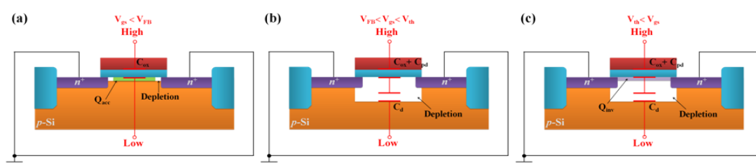
Figure 2-11. Equivalent circuit models for C_{gb} measurement depending on the conduction regimes, (a) accumulation, (b) depletion, and (c) inversion, respectively.[7]
