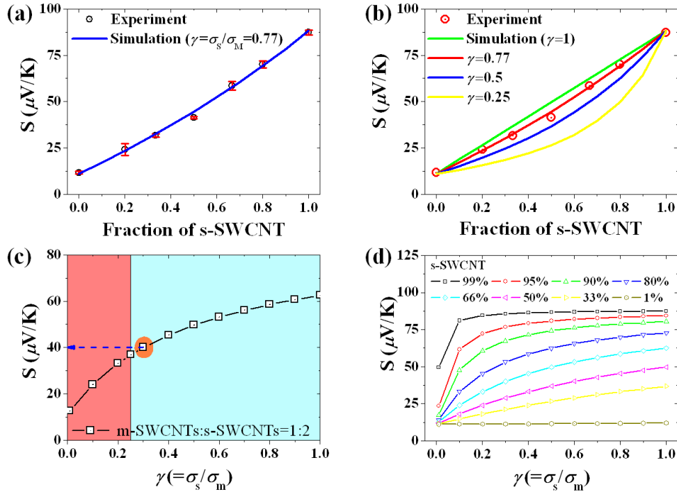
Figure 7-7 (a) The experimental and calculated TEP as a function of the s-SWCNT fraction in the mixed thin films (b) The fitting curves of the TEP in the mixed SWCNT films depending on \gamma=(\sigma_s/\sigma_m) (c) Example of the simulated TEP for a SWCNT film with a m:s ratio equal to 1:2 as a function of \gamma , (d) and the corresponding fitting curves of TEP versus \gamma for different fractions of s-SWCNTs in the films.
