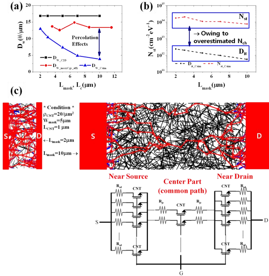
Figure 6-8 (a) D_w based on C_{2D} , \max(C_{gc\_eff}) , and C_{Sim} (b) N_{st} and D_{it} extracted from C_{Sim} (c) Comparison the effective D_{W\_Csim} between L_{mask}=2\mu m and L_{mask}=10\mu m with fixed W_{mask}=5\mu m in random network system. (Simplified electrical equivalent circuit was displayed)
