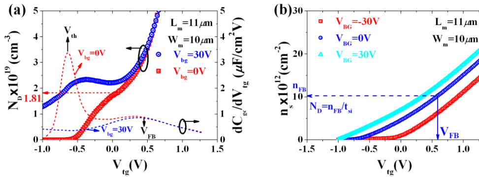
Figure 2-17 (a) N_D based on Eq. (2-25) and dC_{gc}/dV_{tg} (right axis) curves of n-type of JLTs. (b) n_s versus V_{tg} curves for N_D estimation with account for the position of V_{FB} .
