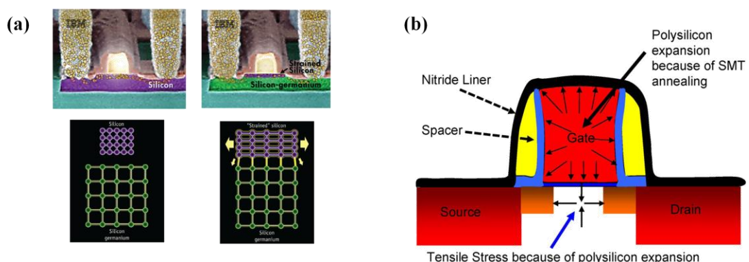
Figure 1-9 Illustration of (a) straining of silicon by means of silicon germanium and (b) mechanism of gate stress memorization technique [17, 18]
