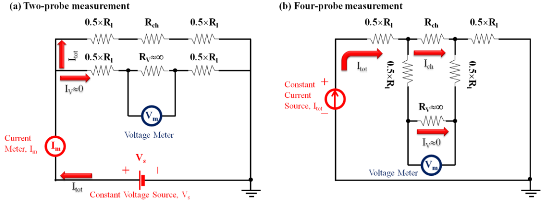
Figure 2-6 (a) Two-terminal and (b) four-probe measurement configurations.
