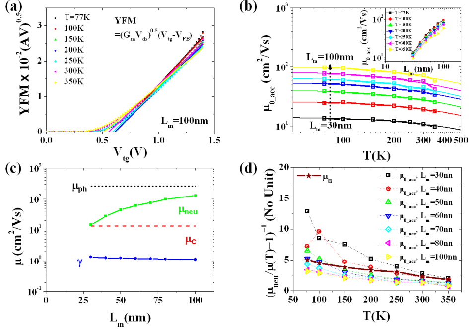
Figure 4-10 (a) The temperature dependence of YFM in accumulation regime in the case of L_m=100\text{nm} JLT. (b) \mu_{0\_acc} as a function of T depending on L_m (Inset: \mu_{0\_acc} versus L_m with varying T ) (c) Various mobility fitting components ( \mu_{ph} , \mu_c , \mu_{neu} , and \gamma ) for \mu_{0\_acc} depending on L_m . (d) The relative ratio of effective \mu_{neu} contribution to \mu_B and \mu_{0\_acc} .
