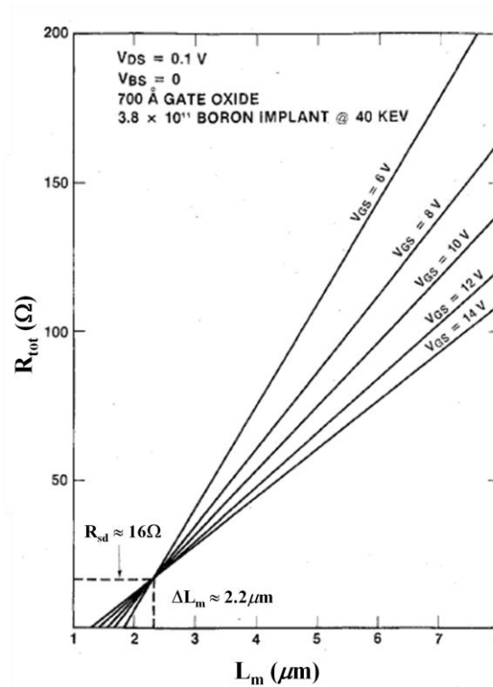
Figure 2-7 Measured total resistance R_{tot} as a function of L_m depending on different V_{gs} values for a set of poly silicon gate n-channel MOSFETs with fixed mask width W_m=200\mu m with 70nm SiO_2 MOSFET.[34]
