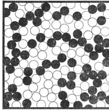
Figure 3-2 Mixture of conducting (black disc) and non-conducting (white disc) grains.[26]
