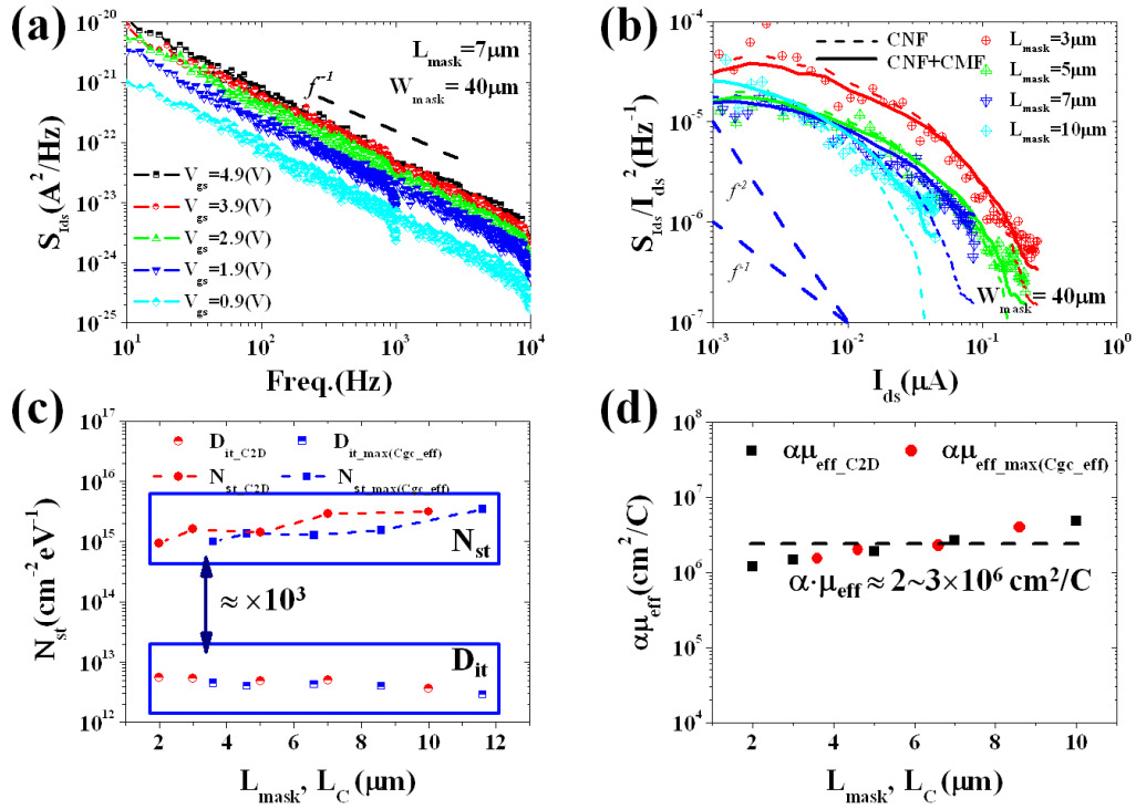
Figure 20 (a) LFN-PSD for different V_{gs} at V_{ds}=50mV ( L_{mask}=7\mu m ) (b) I_{ds} normalized LFN-PSD at f=10Hz (symbols) with CNF (dotted lines) and CNF-CMF (lines) fitting curves (c) Comparison of N_{st} and D_{it} versus L_{mask} and L_c , respectively (d) \alpha \cdot \mu_{eff} depending on different L_{mask} and L_c , respectively.
