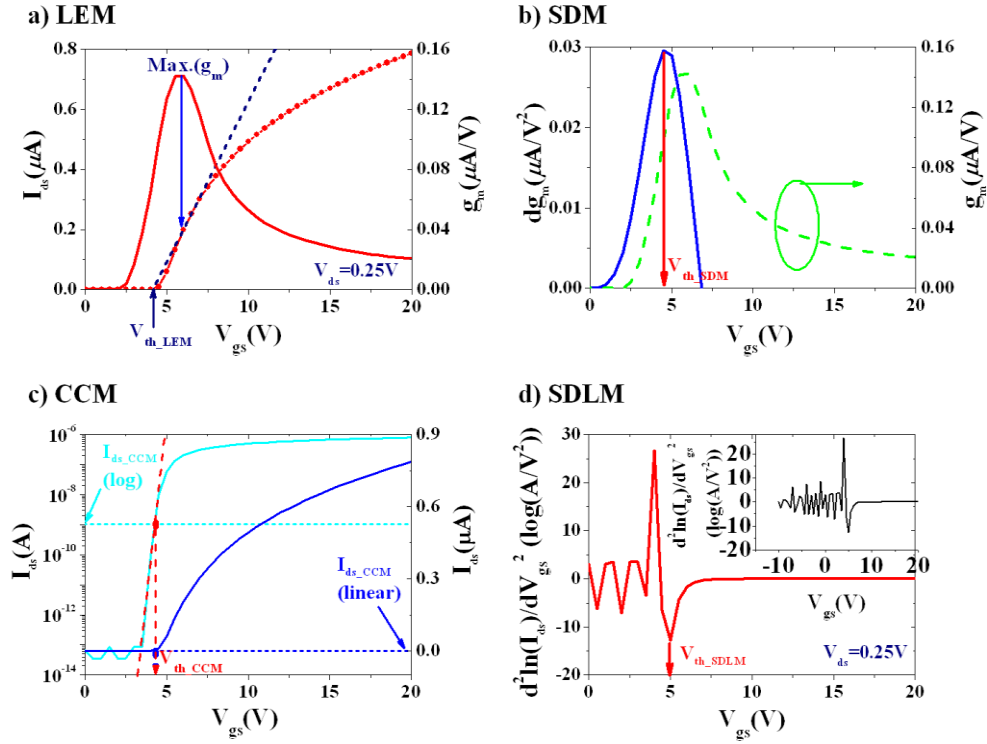
Figure 2-4 Various V_{th} extraction methods for PMMA (polymethyl methacrylate) passivated \text{SnO}_2 FET ( W_{eff}=42\text{nm} and L_{eff}=4.02\mu\text{m} on 150\text{nm} \text{Si}_3\text{N}_4 layer) by using (a) LEM, (b) SDM, (c) CCM, and (d) SDLM
