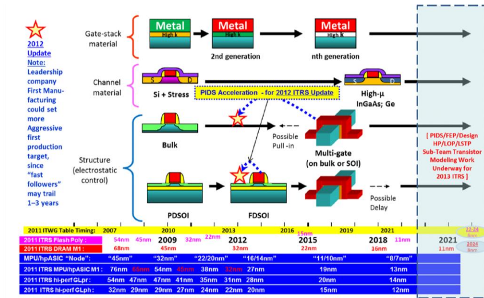
Figure 1-8 2012 ITRS "Equivalent Scaling" process technologies timing Overall Roadmap Technology Characteristics (ORTC) microprocessor unit (MPU)/High-performance ASIC half pitch and gated length trends and timing, and industry "Nodes". [ http://www.itrs.net/ ]
