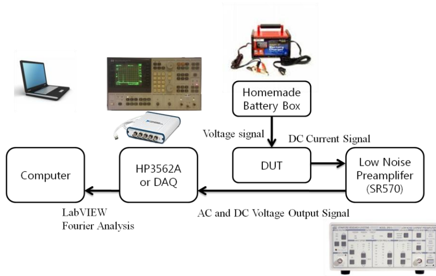
Figure 5-3 The LFN measurement system
