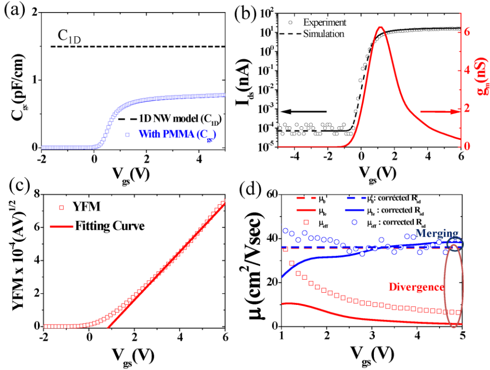
Figure 5-5 (a) Comparison capacitance values between the C_{1D} and simulated C_{gc}(V_{gs}) (open rectangular) respect to back-gate bias. (b) I_{ds}(V_{gs}) (open circle) and g_m(V_{gs}) of SnO 2 NW-FET at V_{ds}=0.25V . Simulated I_{ds}(V_{gs}) (dotted circle) is added for comparison. (c) YFM( V_{gs} ) curve with linear fitting line. (d) Comparison of various mobility ( \mu_0 , \mu_{fe} , \mu_{eff} ) before and after R_{sd} correction.
