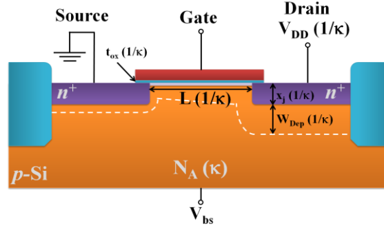
Figure 1-4 Illustration of scaling parameter of MOSFET.
