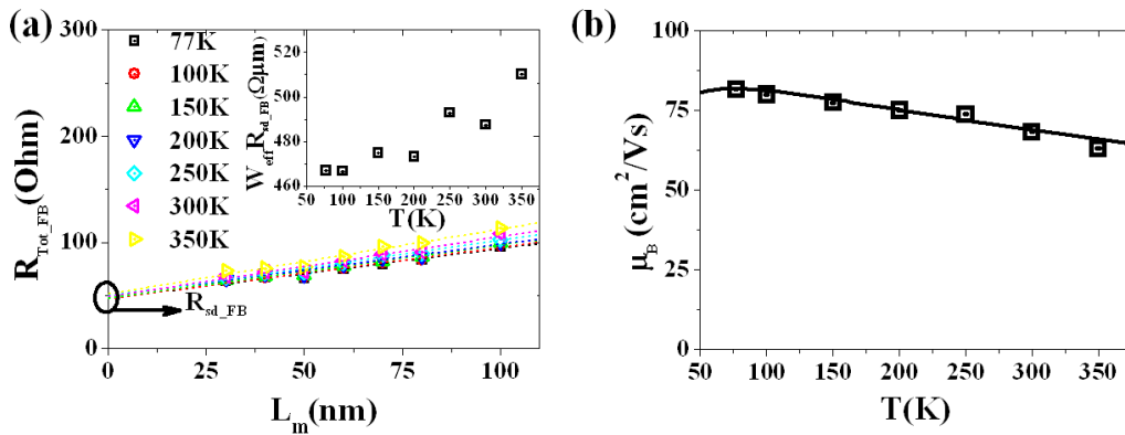
Figure 10 (a) The temperature dependence of R_{tot,FB} with respect to L_m . Fitting curves (dotted lines) are plotted together with data (symbols). (Inset: The temperature dependence of W R_{sd,FB} / R_{sd,FB} ) (b) The temperature dependence of \mu_B and corresponding fitting curve with account for various mobility fitting components ( \mu_{ph} , \mu_C , \mu_{neu} , and \gamma )
