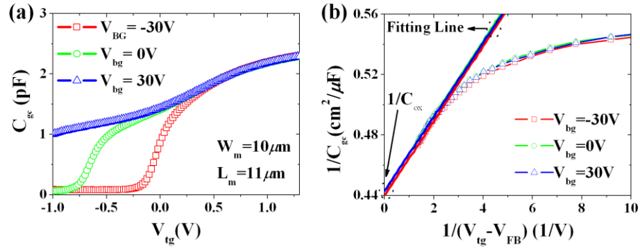
Figure 2-15 (a) C_{gc}(V_{tg}) curves of N-type JLT ( L_m=11\mu\text{m} with W_m=10\mu\text{m} ) depending on V_{bg} , V_{tg} and V_{bg} are top and back gate induced bias respectively and (b) corresponding 1/C_{gc}(V_{tg}) curves for C_{ox} and corresponding CET extraction in high V_{tg} regime.
