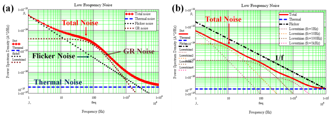
Figure 2-19 (a) Various PSD source for total LFN characteristics and (b) the superposition of four different Lorentzian curves.
