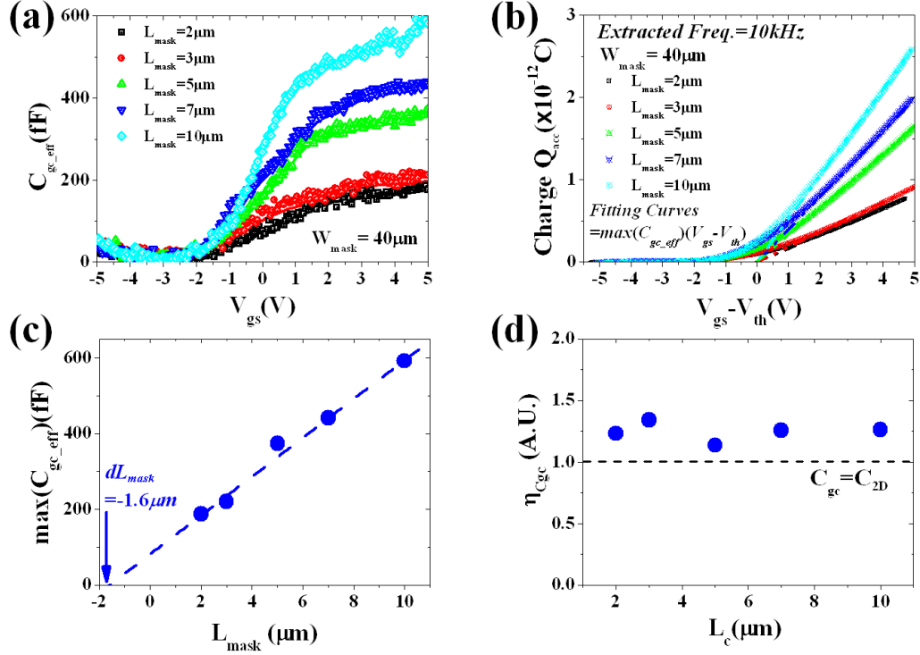
Figure 6-3 (a) C_{gc\_eff}(V_{gs}) curves of a top-gate RN-TFTs at f=10kHz (b) Q_{acc}(V_{gs}) (symbols) with linear fitting lines ( \approx \max(C_{gc\_eff}) \times (V_{gs} - V_{th}) , dotted lines) (c) \max(C_{gc\_eff}) and (d) \eta_{Cgc} verses L_{mask} and L_c , respectively.
