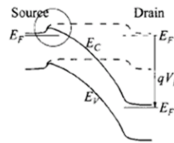
Figure 1-5 Energy-band diagrams at the semiconducting surface from source to drain, for (a) long and (b) short channel MOSFET, respectively.[9]
