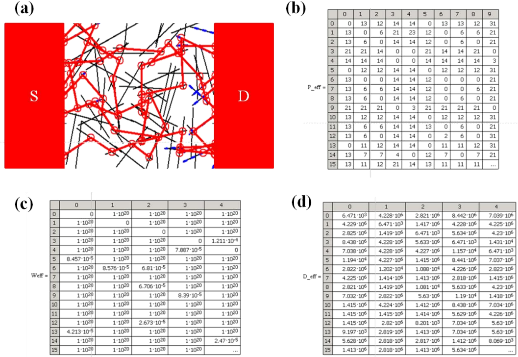
Figure 3-7 (a) Optimal pathways from S to D in a test set of Fig. 3-5, and corresponding (b) P, (c) W, and (d) D matrix, respectively.
