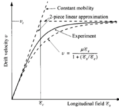
Figure 1-6 Drift velocity ( v_d ) curves as a function of E for silicon and semiconductor.[9]
