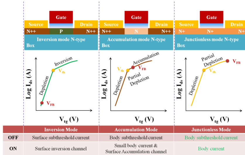
Figure 3 Comparison of conduction mode of advance MOS transistors (Left: Inversion mode, Middle: Accumulation mode, Right: Junctionless mode)
