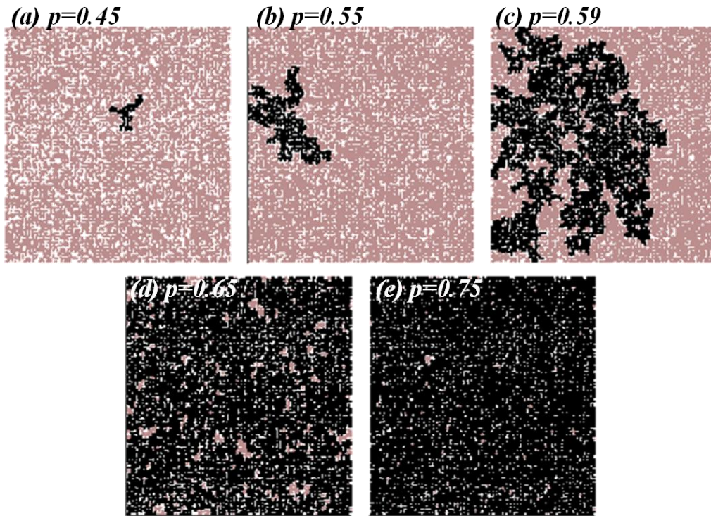
Figure 3-3 Percolation in square lattice with system size L \times L = 150 \times 150 . Occupation probability (a) p=0.45 , (b) 0.55 , (c) 0.59 , (d) 0.65 , and (e) 0.75 , respectively. From p=0.59 , the cluster which percolates from top-to-bottom is observed.[27]
