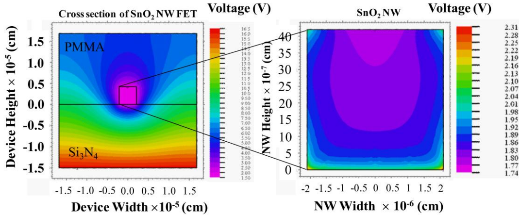
Figure 5-7 Simplified cross-section view of the effective V_{gs} contour in PMMA passivated \text{SnO}_2 NW-FET with back-gate configuration (left) and its magnified view in \text{SnO}_2 -NW region (right) at high V_{gs} .
