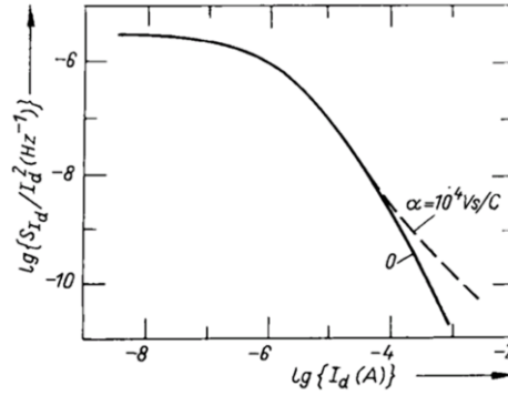
Figure 2-22 Theoretical variation of the I_{ds} normalized PSD in the case of \alpha_C \approx 0 and \alpha_C \approx 10^4 V_s/C , respectively.[17]
