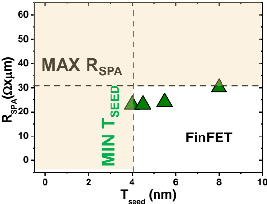
Figure 2.58: FinFET low temperature junction figure of merit: R_{SPA} - T_{SEED} MIN trade-off for.
