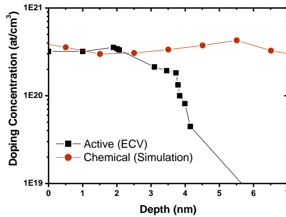
Figure 3.20 : Active doping profile obtained by ECV technique in comparison to chemical profile (simulation).
