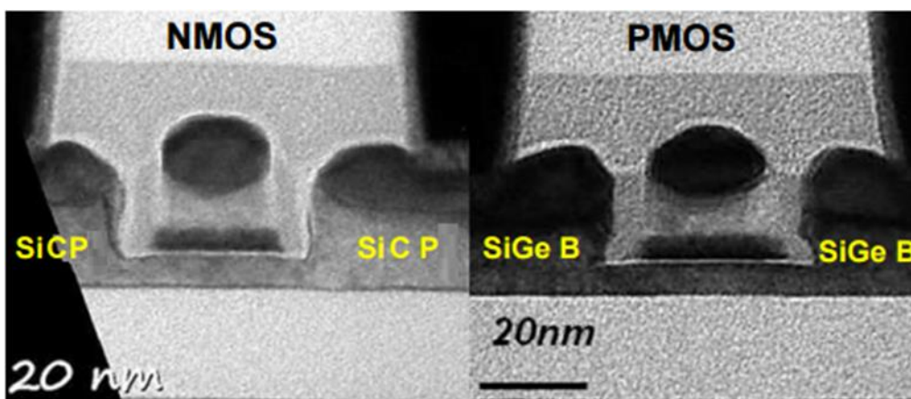
Figure 3.2: TEM cross section images for nMOS and pMOS fabricated with the POR process 14nm FDSOI [Weber 15].
