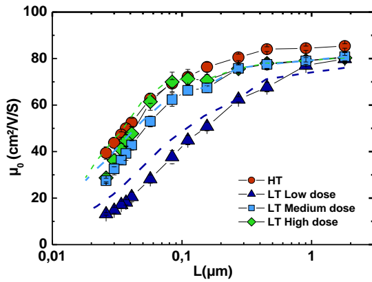
Figure 2.30: Carriers mobility at low electric field for different gate lengths. High temperature devices and low temperature devices with medium and high dose show similar behaviors after \Delta L correction. Strong degradation is shown for low temperature device with low dose split.
