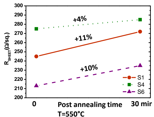
Figure 1.16: Sheet resistance percentage variation after post annealing of 30 minutes at 550°C.
