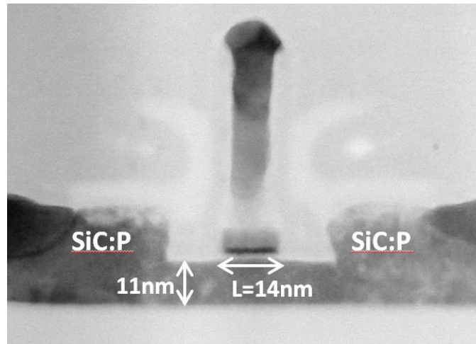
Figure 4.35: TEM observation of an n-type TriGate device fabricated with the process flow illustrated in Figure 4.32.
