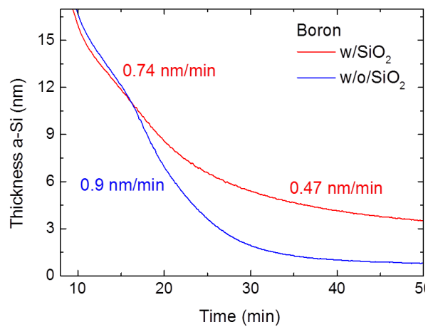
Figure 1.33: In-situ ellipsometry 450 °C annealing of B implanted samples with (w/SiO 2 ) and without (w/o/SiO 2 ) the oxide layer.
