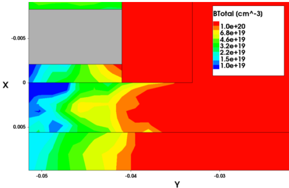
Figure 4.17: Total boron concentration after heated implantation for the first simulated condition. It has been considered unsatisfying since high dopant concentration is present into the channel region.
