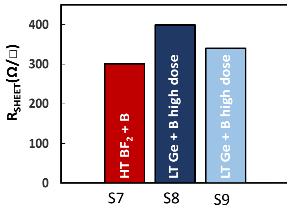
Figure 1.18: Sheet resistance values measured on samples reported in Table 1.2 for p-type doping.
