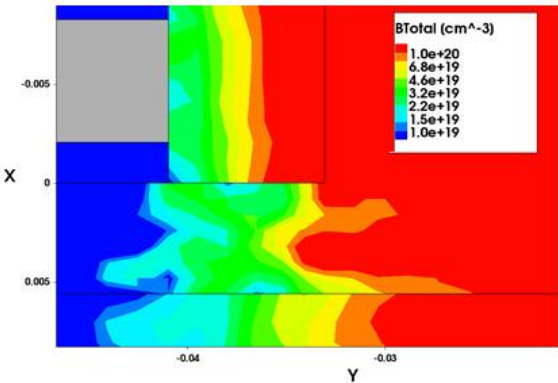
Figure 4.18: Total boron concentration after heated implantation for the second simulated condition. The dopant concentration below the spacer appears satisfying (around 5 \times 10^{19} at/cm 3 ) concentration below 10^{19} at/cm 3 is present into the channel. This condition is the one chosen for the electrical device.
