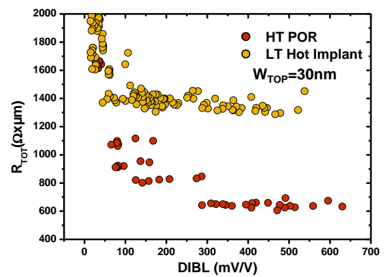
Figure 4.41: R_{TOT} -DIBL trade-off for low temperature devices with hot implantation in comparison with high temperature POR. Same DIBL is shown while total resistance degradation is observed for hot implant split.
