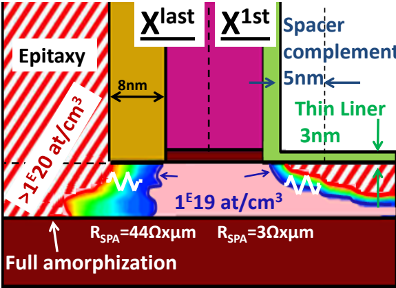
Figure 2.47: KMC simulation of junction profile for extension last and extension first integration.
