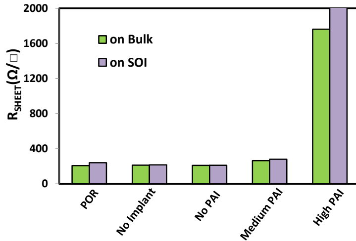
Figure 3.31: R_{\text{SHEET}} measurement on Bulk and SOI unsalicyded structures for splits described in Table 3.1.
