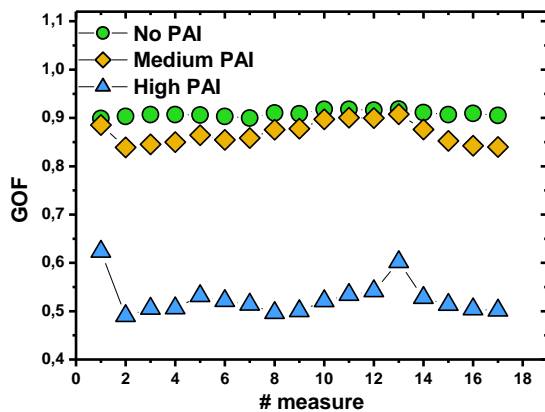
Figure 3.27: GOF ellipsometry measurement post SiGe:B epitaxy on SiGeOI structures.
