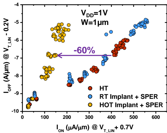
Figure 4.21: I_{ON} - I_{OFF} trade-off performance for hot implant split with respect to high temperature devices and low temperature devices with RT implant.
