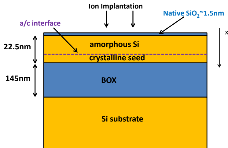
Figure 1.5: Scheme of full sheet SOI sample used for SPER analysis.
