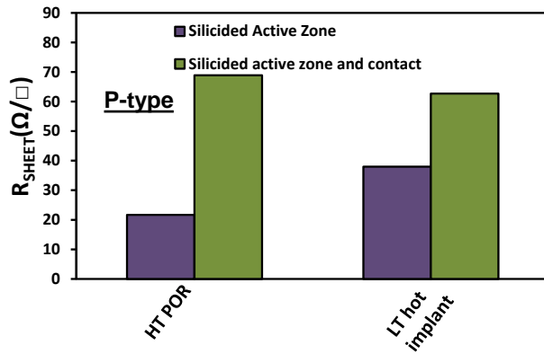
Figure 4.40: Sheet resistance measurements on silicided active zone with and without contact resistance for hot implant split and POR.
