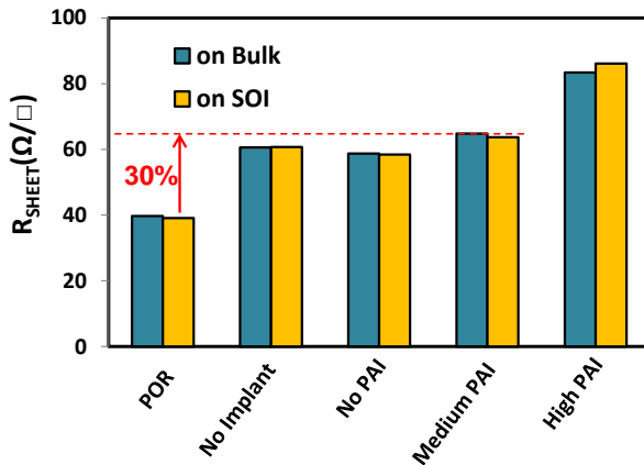
Figure 3.43: R_{SHEET} measurements on bulk and SOI salicided p-type structures for splits detailed in in Table 3.2.
