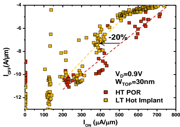
Figure 4.46: I_{ON} - I_{OFF} trade-off for n-type low temperature devices with hot implantation in comparison with high temperature POR.
