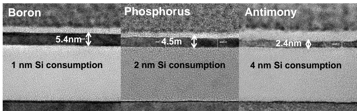
Figure 4.32: Silicon consumption after nitride removal, for samples subjected to heated implantation.
