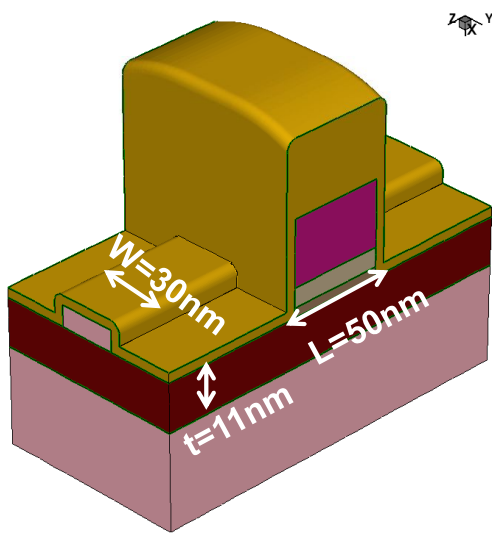
Figure 4.36: Simulated structure of TriGate device.
