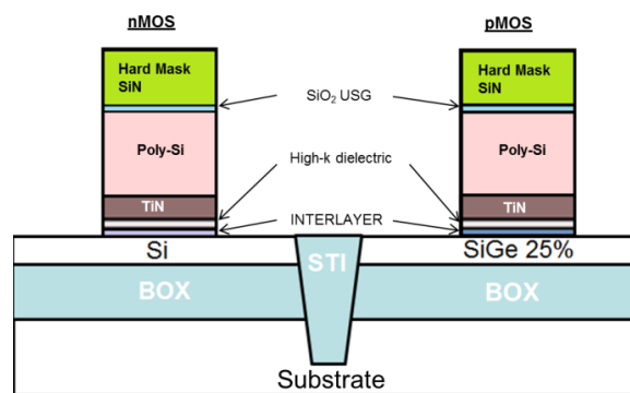
4) Lithography
