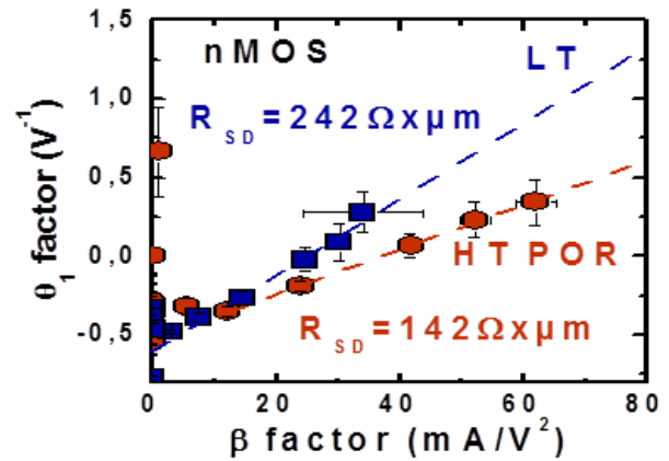
Figure 2.54: Experimental extraction of access resistance for high temperature and low temperature TriGate devices.
