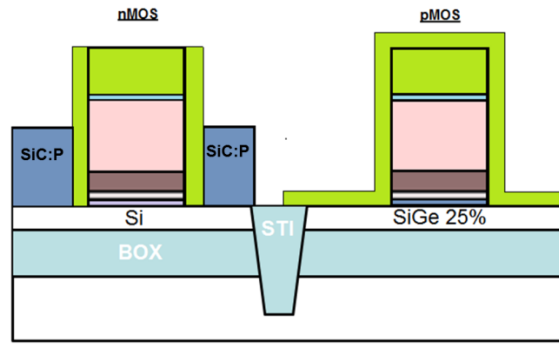
8) First spacer p etching + Raised Source Drain Epitaxy p (SiGe:B)
