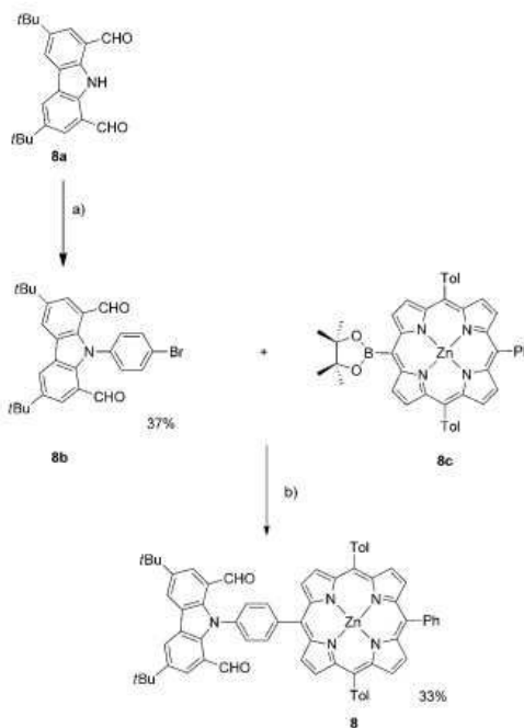
Scheme 5. Synthesis of N -carbazole porphyrin 8 . a) 1,4-Dibromobenzene, CuI, \text{K}_2\text{CO}_3 , 18-C-6, nitrobenzene, reflux, 5 h; b) NaI, \text{Cs}_2\text{CO}_3 , [\text{PdCl}(\text{tBu-C}_6\text{H}_4)_2] , \text{PPh}_3 , toluene/DMF, 80 °C, 24 h.
