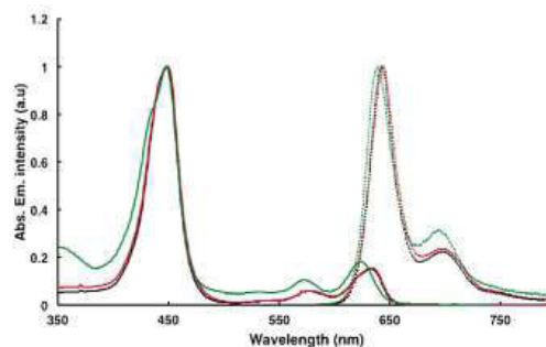
Figure 1. Absorption (solid line) and emission (dashed line) spectra of 1a (red), 1b (black) and 9 (green) in \text{CH}_2\text{Cl}_2 solution.
