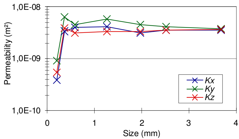
Figure 1.b: Dependency of K^{\text{eff}} estimates with sample size.
