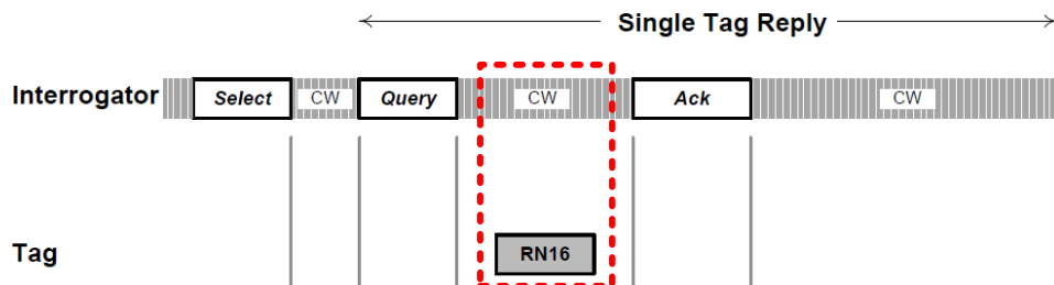
Figure 3.2: Frames timing in forward and return link [57].
