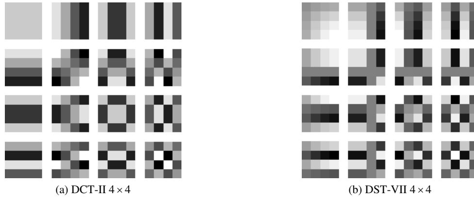
Figure 2.2.1 – Transforms used in HEVC for 4 × 4 blocks
