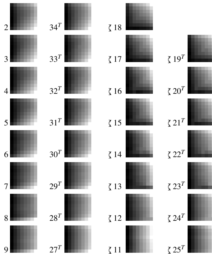
Figure 6.4.4 – Average 8 \times 8 residual profiles showing imposed symmetries with transposition and horizontal mirroring
