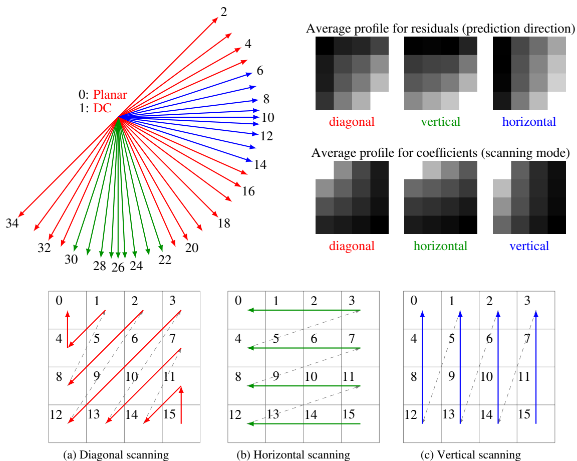
Figure 1.3.3 – HEVC Intra Prediction Modes referred to their scanning patterns together with some average residual examples in the transform domain for 4 \times 4 TUs
