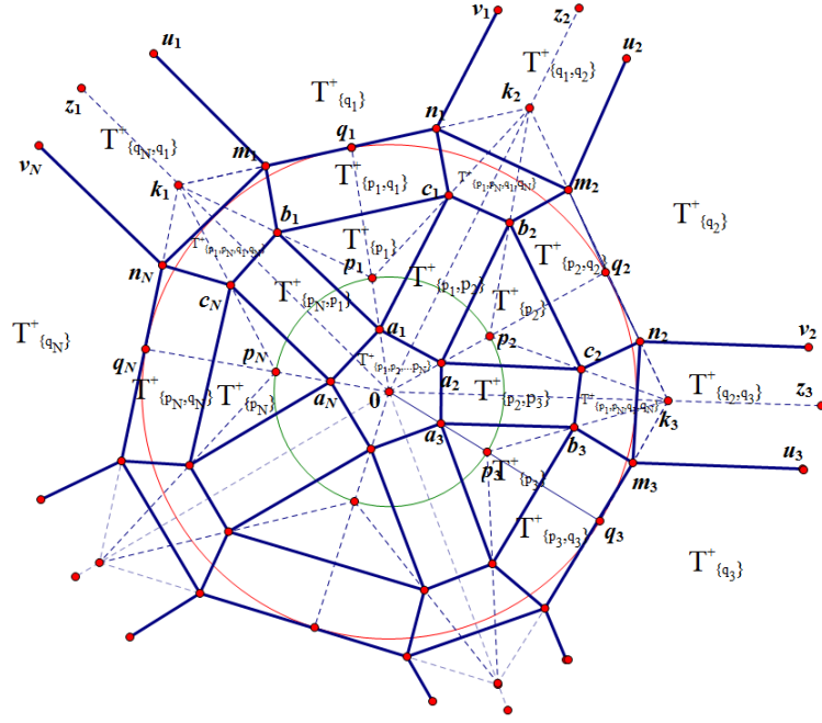
Figure 3.14: The function w^+
