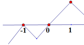
Figure 1.2: Illustration m^-(f, \Omega)
