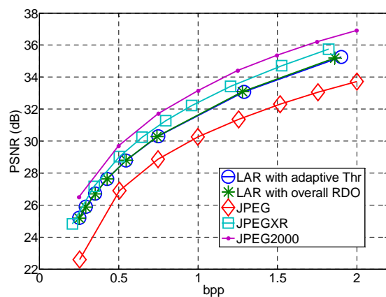
FIGURE 3.45 – PSNR of “bike crop”.
