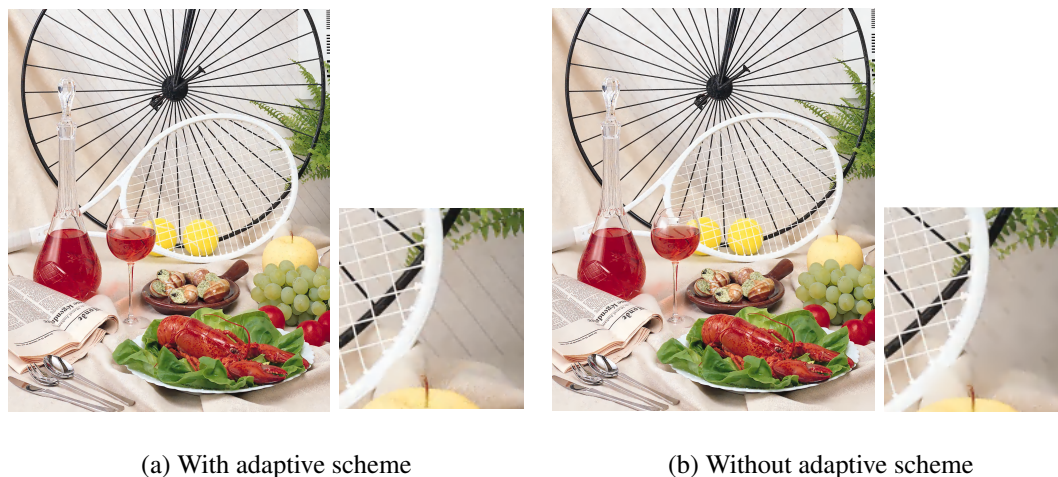
FIGURE 3.36 – Comparison of the decoded images in quqp = 45 . (a) MSSIM = 0.9898 (39.8670 dB), bitrate :0.841 bpp ; (b) MSSIM = 0.9875 (38.0621 dB), bitrate :0.836 bpp.
