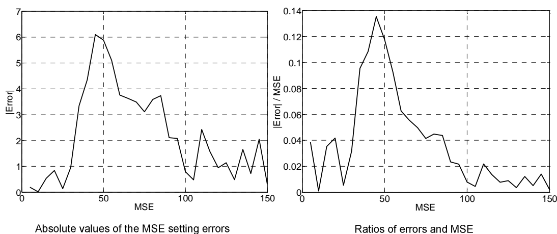
FIGURE 3.29 – Comparison between errors and MSE set for “leaves”
