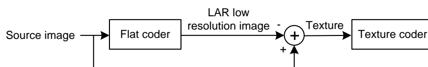
FIGURE 2.1 – Two-layer LAR coder
