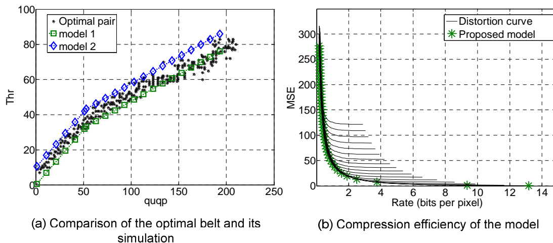
FIGURE 3.8 – Performance of the RDO model for “bike crop”
