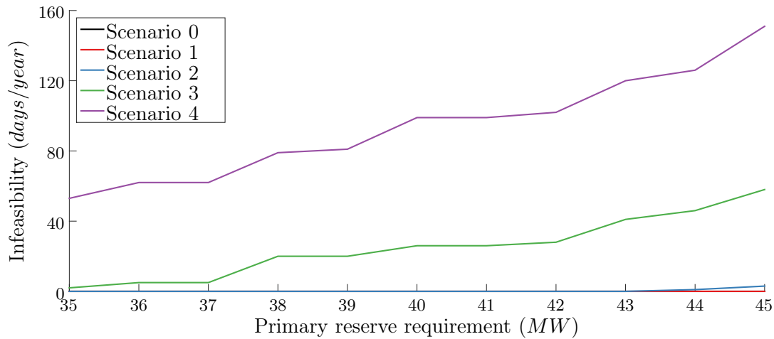
Figure 4.3: Instances where the security constraint is violated (model \mathfrak{M}_1 )
