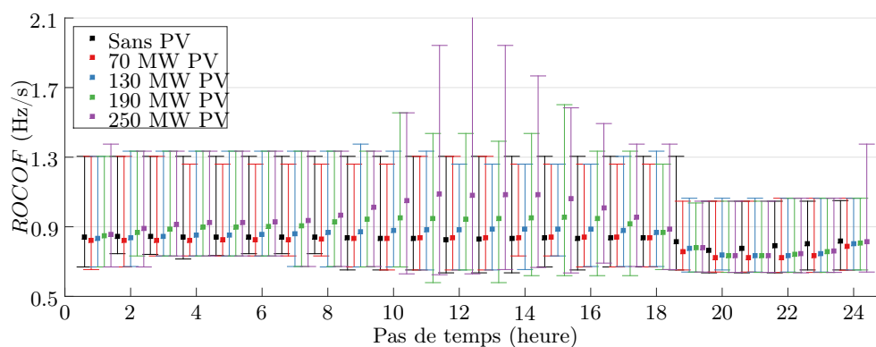
Figure 12: ROCOF
