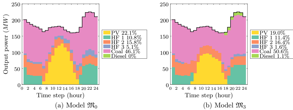
Figure 4.12: Dispatch change for improved dynamic response (Scenario 4)
