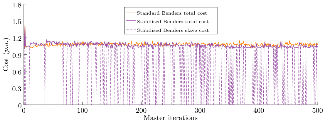
Figure 5.25: Comparison of the total cost of the master candidate solutions
