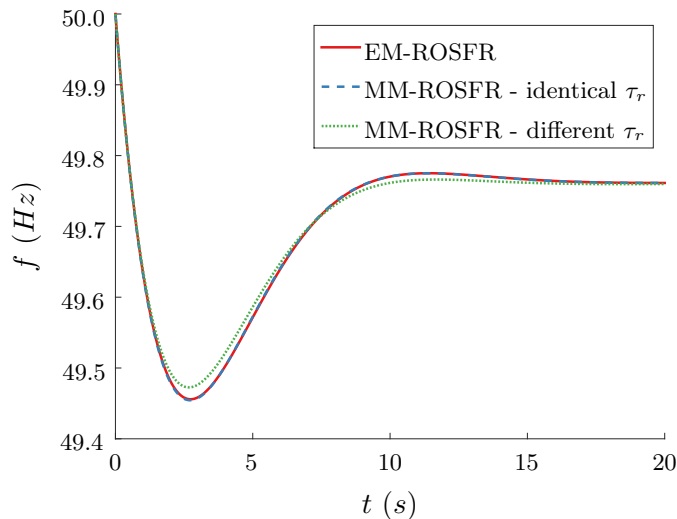
Figure C.1: Frequency for different ROSFR models
