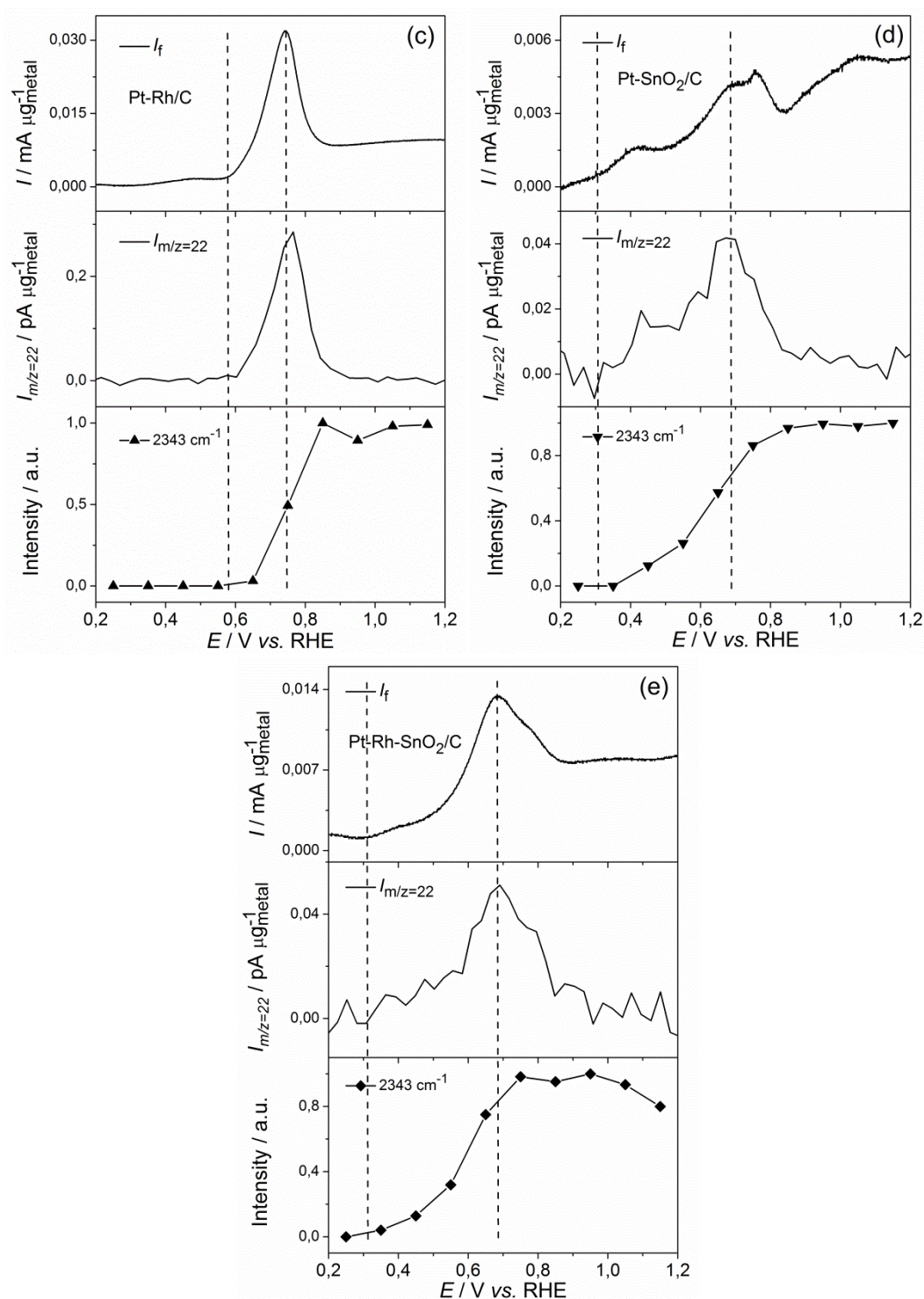
Fig. 31. CO-stripping CV in 0.5 M \text{H}_2\text{SO}_4 , corresponding MS signal m/z = 22 and \text{CO}_2 band intensity (from Fig. 30) on (a) Pt/C, (b) Rh/C, (c) Pt-Rh/C, (d) Pt- \text{SnO}_2 /C and (e) Pt-Rh- \text{SnO}_2 /C; \nu = 10 \text{ mV s}^{-1} ; T = 25^\circ\text{C} .
