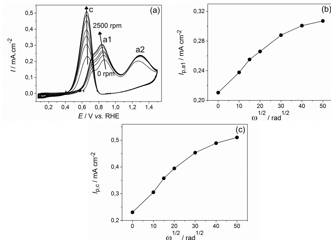
Fig. 14. (a) CV in 0.5 M H 2 SO 4 + 0.1 EtOH on Pt/C (metal loading: 9.9 \mu\text{g} ) on a RDE at different rotation speeds: 0, 100, 225, 400, 900, 1600, 2500 rpm; Evolution of the peak current between (b) E = 0.3 and 1 V vs. RHE ( I_{p,a1} ) and between (c) E = 0.8 and 0.4 V vs. RHE ( I_{p,c} ) against the rotation speed; v = 10 \text{ mV s}^{-1} ; T = 25^\circ\text{C} .
