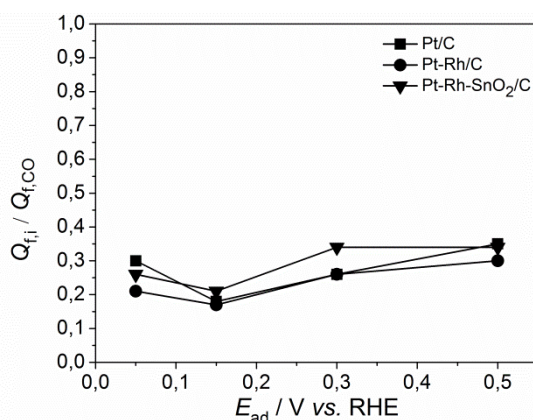
Fig. 74. Relative coverage of Pt/C, Pt-Rh/C and Pt-Rh-SnO 2 /C electroactive surface by “strong acetaldehyde adsorbates” (oxidizing at E > 0.9 V vs. RHE) adsorbed at E_{\text{ad}} = 0.05 , 0.15 , 0.3 and 0.5 V vs. RHE deduced from faraday charges.
