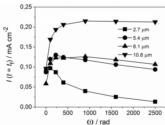
Fig. 20. Evolution of the potentiostatic current (CA at E = 0.7 \text{ V vs. RHE} ) recorded at t_f = 630 s against the rotation speed.
