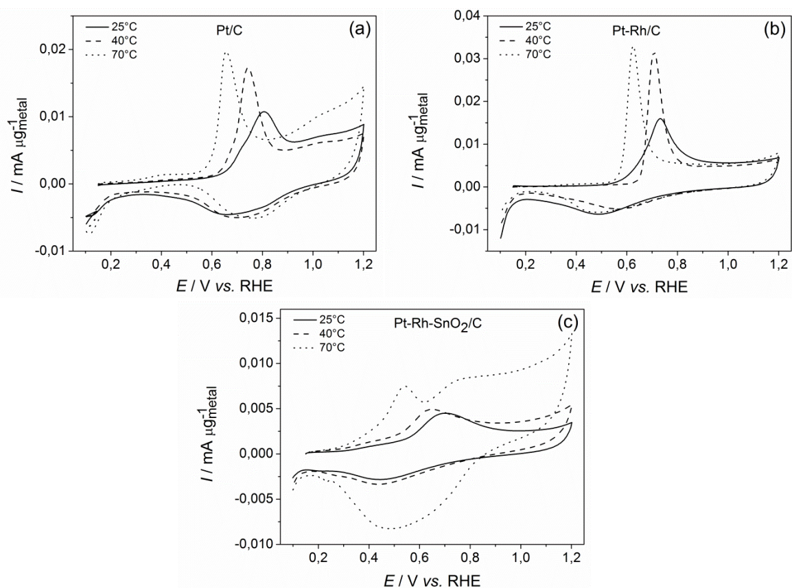
Fig. 78. CO-stripping CV in 0.5 M H 2 SO 4 on (a) Pt/C, (b) Pt-Rh/C and (c) Pt-Rh-SnO 2 /C; T = 25^{\circ}\text{C} (full), 40^{\circ}\text{C} (dash) and 70^{\circ}\text{C} (dots); \nu = 10 \text{ mV s}^{-1} .
