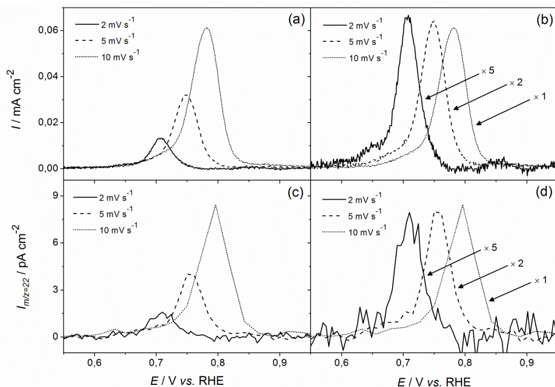
Fig. 21. Subtracted (a) non-amplified and (b) amplified CO-stripping CVs in 0.5 M H 2 SO 4 on Pt/C (metal loading: 9.9 μg) and corresponding (c) non-amplified and (d) amplified MSCVs for mass-to-charge ratio m/z = 22 multiplied by a number indicated in brackets; T = 25^{\circ}\text{C} .
