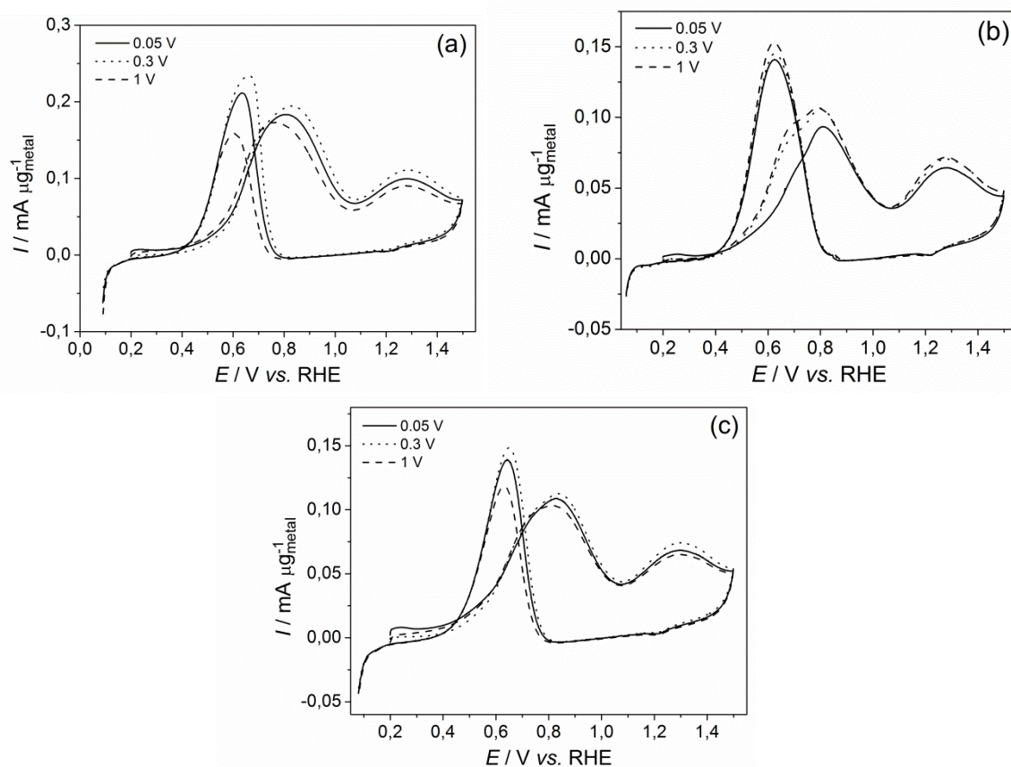
Fig. 43. CV of the EOR in 0.5 M \text{H}_2\text{SO}_4 + 0.1 M EtOH after adsorption at E_{\text{ad}} = 0.05 (solid), 0.3 (dots) and 1 V vs. RHE (dash) on (a) Pt-Rh/C, (b) Pt-SnO 2 /C and (c) Pt-Rh-SnO 2 /C; \nu = 10 \text{ mV s}^{-1} ; T = 25^\circ\text{C} .
