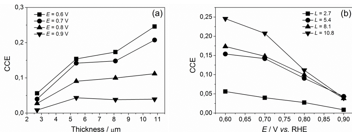
Fig. 16. Evolution of the EOR \text{CO}_2 current efficiency (CCE) against (a) the electrocatalyst thickness and (b) the applied potential calculated from cyclic voltammeteries run in 0.5\text{ M H}_2\text{SO}_4 + 0.1\text{ M EtOH} (represented in Fig. 15a) and corresponding MSCVs (Fig. 15b) on Pt/C.
