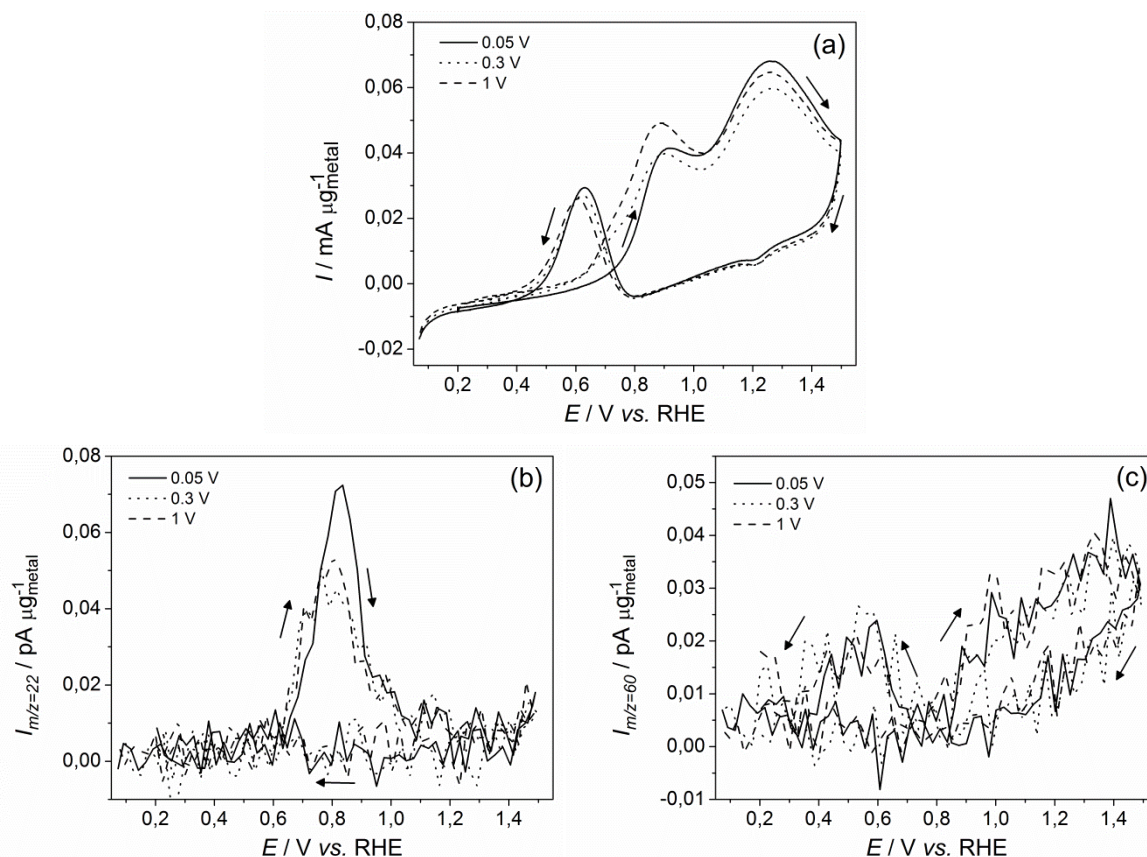
Fig. 53. (a) CV of the EOR in 0.5 M H 2 SO 4 + 0.1 M acetaldehyde after adsorption at E_{ad} = 0.05 (solid), 0.3 (dots) and 1 V vs. RHE (dash) and corresponding MSCV for mass-to-charge ratio (b) m/z = 22 and (c) m/z = 60 on Pt-Rh-SnO 2 /C; \nu = 10 \text{ mV s}^{-1} ; T = 25^\circ\text{C} .
