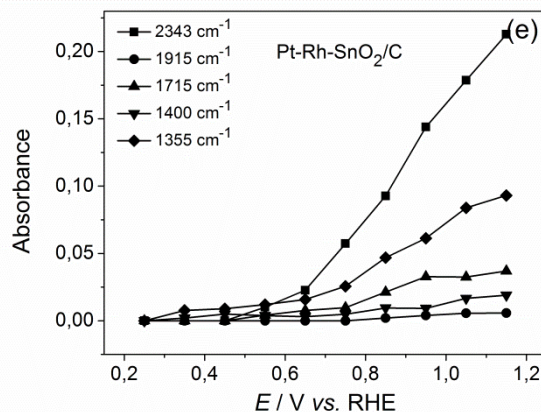
Fig. 35. Evolution of band intensities (at 2343, 1915, 1715, 1400, 1355 \text{cm}^{-1} ) against applied potential on (a) Pt/C (b) Rh/C, (c) Pt-Rh/C, (d) Pt-SnO 2 /C and (e) Pt-Rh-SnO 2 /C.
