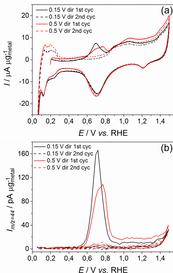
Fig. 60. (a) CV of the electrooxidation of ethanol adsorbates in 0.5 M \text{H}_2\text{SO}_4 after adsorption at (black) E_{\text{ad}} = 0.15 V vs. RHE and (red) E_{\text{ad}} = 0.5 V vs. RHE and the corresponding MSCV for mass-to-charge ratio (b) m/z = 44 on Pt/C; \nu = 10 mV \text{s}^{-1} ; T = 25^\circ\text{C} .
