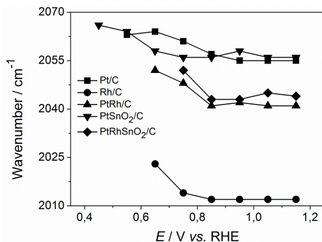
Fig. 29. Variation of the \text{CO}_{\text{L}} band wavenumber versus potential, measured during the CO stripping in 0.5 M \text{H}_2\text{SO}_4 on Pt/C, Rh/C, Pt-Rh/C, Pt-SnO 2 /C and Pt-Rh-SnO 2 /C; T = 25^\circ\text{C} .
