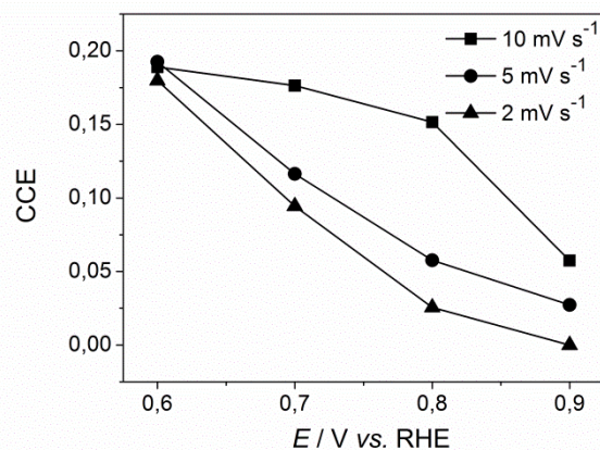
Fig. 23. CO 2 current efficiency (CCE) values calculated from cyclic voltammeteries run in 0.5 M H 2 SO 4 + 0.1 M EtOH (represented in Fig. 22a) at v = 2, 5 and 10 \text{ mV s}^{-1} and corresponding MSCVs (Fig. 22b) on Pt/C.
