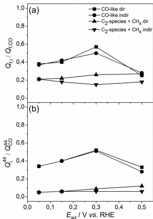
Fig. 58. Relative coverage of the Pt/C surface by ethanol adsorbates adsorbed at E_{ad} = 0.05, 0.15, 0.3 and 0.5 V vs. RHE deduced from (a) faraday charges and (b) ionic charges from the mass-to-charge signal m/z = 44 .
