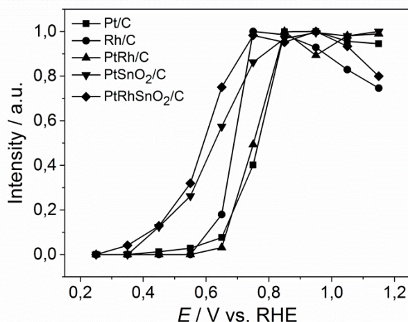
Fig. 30. (a) CO stripping in 0.5 M H 2 SO 4 - CO 2 band intensity against potentials on Pt/C, Rh/C, Pt-Rh/C, Pt-SnO 2 /C and Pt-Rh-SnO 2 /C; T = 25^{\circ}\text{C} .
