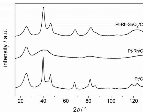
Fig. 75. XRD pattern of 10wt.% carbon supported Pt/C, Pt-Rh/C and Pt-Rh-SnO 2 /C electrocatalysts prepared by the polyol method.
