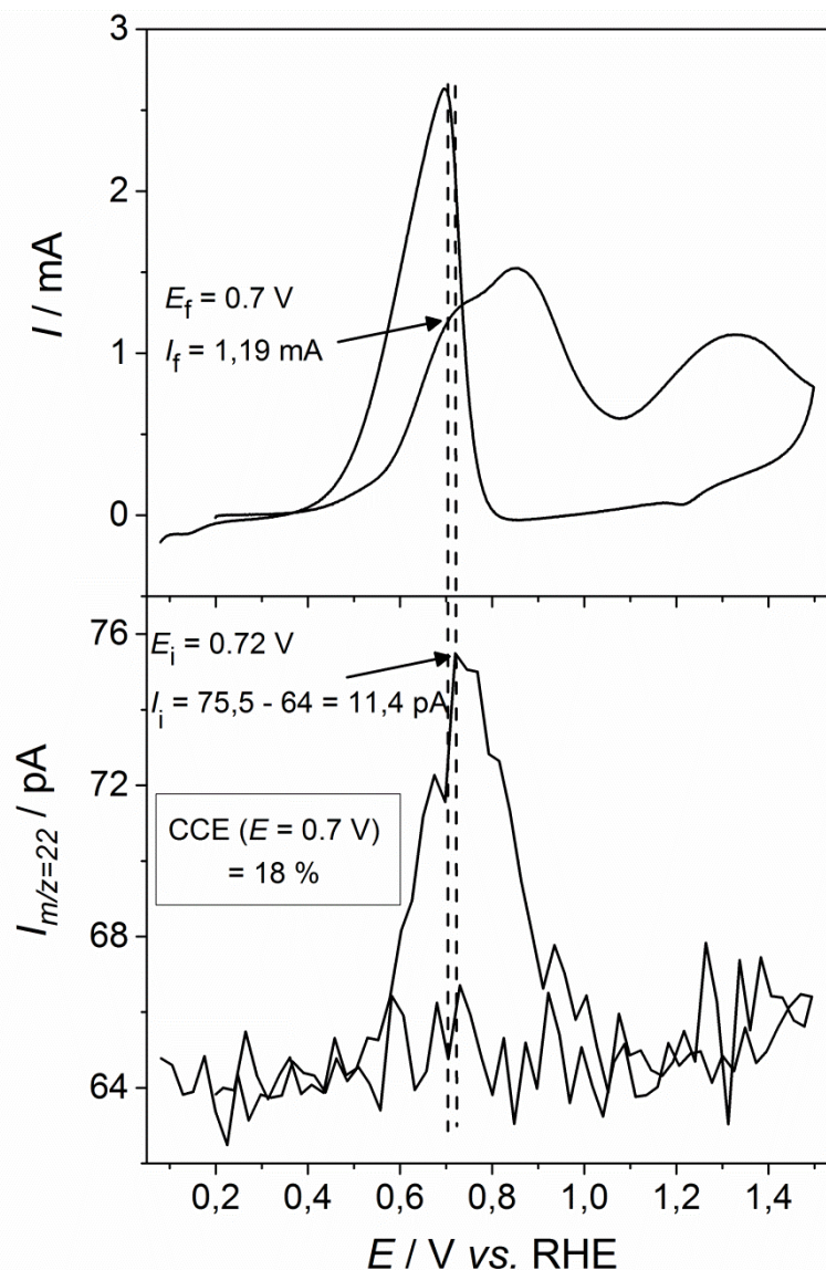
Fig. 12. EOR CCE calculation at E = 0.7 \text{ V vs. RHE} in 0.5 \text{ M H}_2\text{SO}_4 + 0.1 \text{ M EtOH} .
