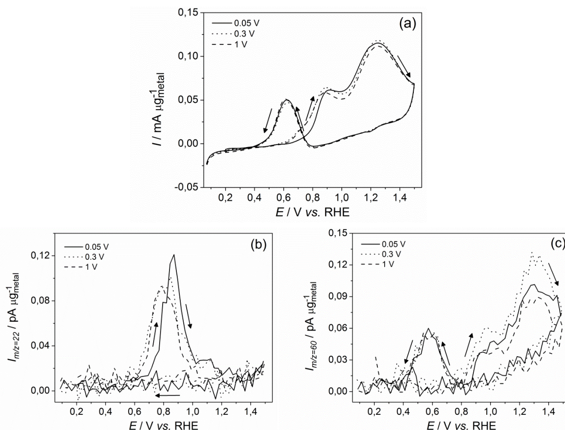
Fig. 49. (a) CV of the EOR in 0.5 M \text{H}_2\text{SO}_4 + 0.1 M acetaldehyde after adsorption at E_{\text{ad}} = 0.05 (solid), 0.3 (dots) and 1 V vs. RHE (dash) and corresponding MSCV for mass-to-charge ratio (b) m/z = 22 and (c) m/z = 60 on Pt/C; v = 10 \text{ mV s}^{-1} ; T = 25^\circ\text{C} .
