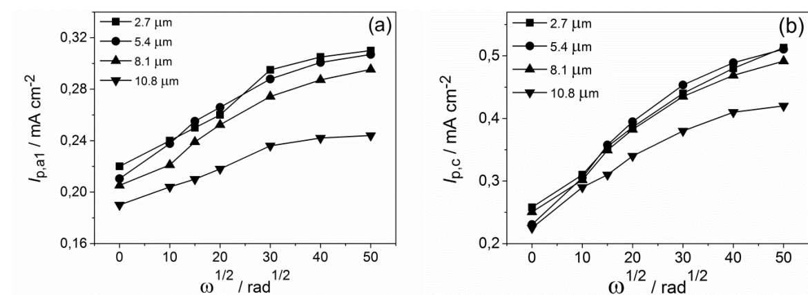
Fig. 18. Evolution of the peak current between (a) E = 0.3 and 1 \text{ V vs. RHE} and (b) E = 0.8 and 0.4 \text{ V vs. RHE} against the rotation speed.
