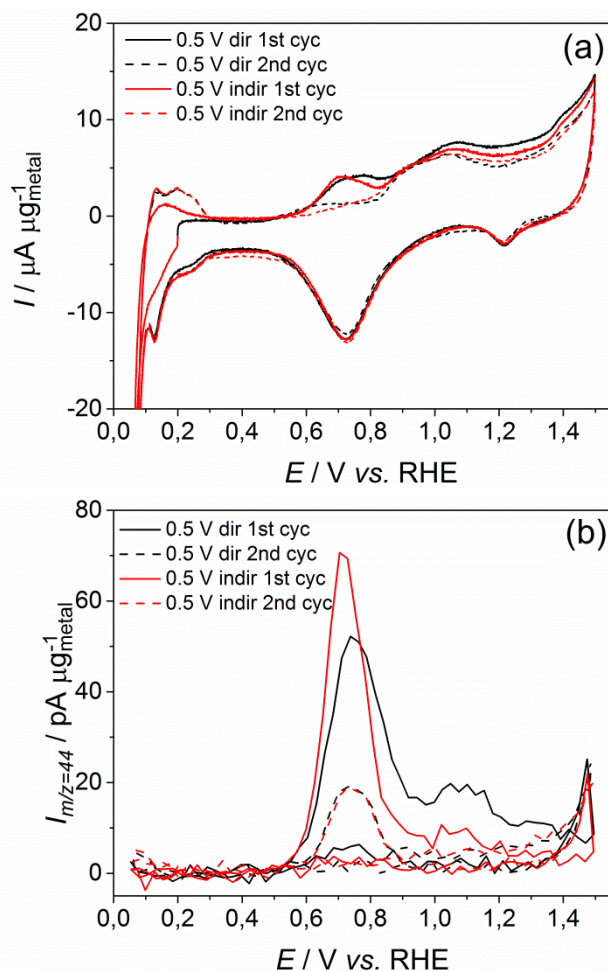
Fig. 65. (a) CV of the electrooxidation of acetaldehyde adsorbates in 0.5 M \text{H}_2\text{SO}_4 after adsorption at E_{\text{ad}} = 0.5 V vs. RHE (black) without and (red) with a first reduction scan and the corresponding MSCV for mass-to-charge ratio (b) m/z = 44 on Pt/C; \nu = 10 \text{mV s}^{-1} ; T = 25^\circ\text{C} .
