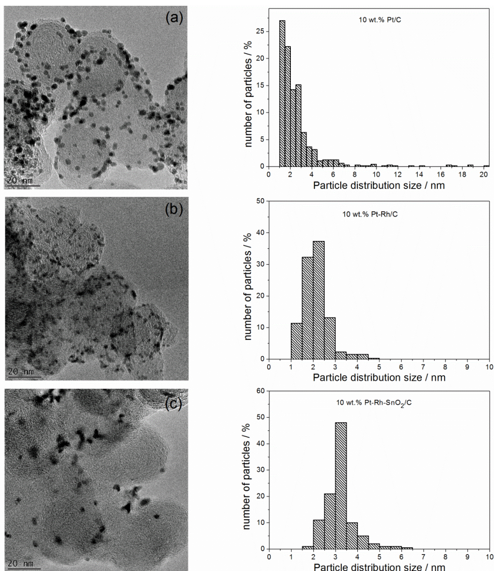
Fig. 76. Typical TEM images and associated particle size distribution of the 10 wt. % (a) Pt/C, (b) Pt-Rh/C and (c) Pt-Rh-SnO 2 /C electrocatalysts.
