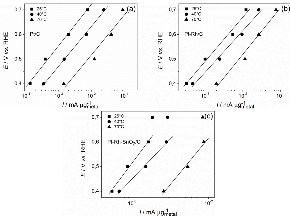
Fig. 80. Tafel plots of potentiostatic currents recorded after 900 s at potentials from 0.4 to 0.7 V vs. RHE (0.1 V step) in 0.5 M H 2 SO 4 + 0.1 M EtOH on (a) Pt/C, (b) Pt-Rh/C and (c) Pt-Rh-SnO 2 /C at 25°C, 40°C and 70°C.
