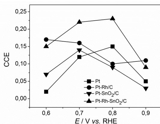
Fig. 37. (a) EOR CO 2 current efficiency (CCE) values calculated from cyclic voltammeteries run in 0.5 M H 2 SO 4 + 0.1 M EtOH (represented in Fig. 33 and Fig. 36) and corresponding MSCVs (in Fig. 33 and Fig. 36) on Pt/C, Pt-Rh/C, Pt-SnO 2 /C and Pt-Rh-SnO 2 /C.
