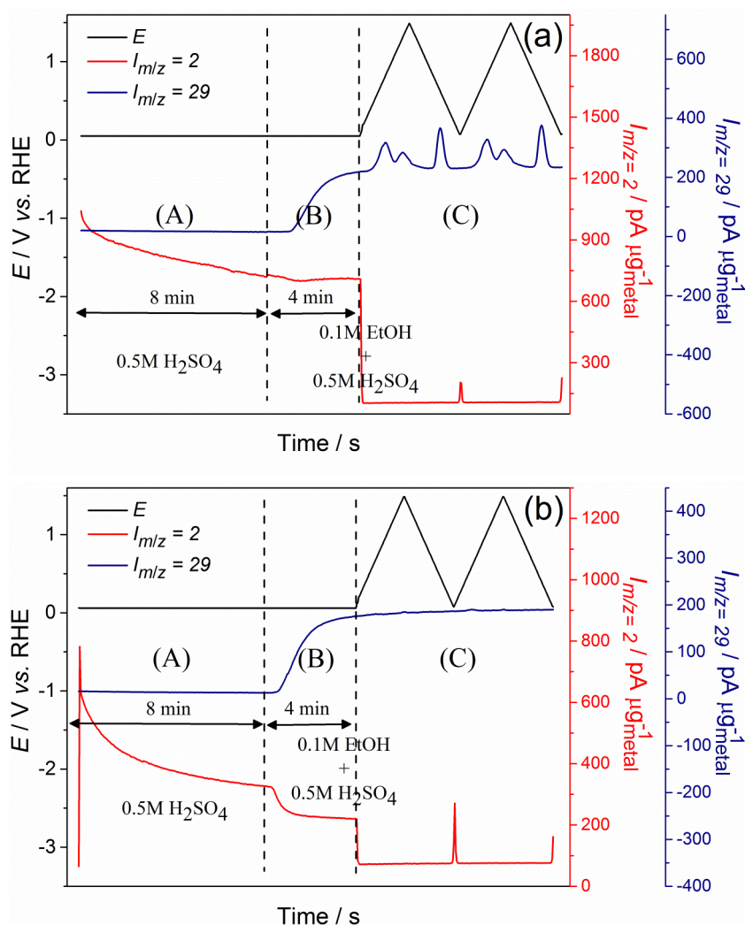
Fig. 47. Evolution of the potential and mass-to-charge ratio signals m/z = 2 and m/z = 29 vs. time on (a) Pt/C and (b) Rh/C during three consecutive steps: (A) hydrogen adsorption in 0.5 M H 2 SO 4 at E_{ad} = 0.05 V vs. RHE, (B) the solution change in 0.5 M H 2 SO 4 + 0.1 M EtOH and (C) the potentiodynamic ethanol oxidation reaction starting at E = 0.2 V vs. RHE.
