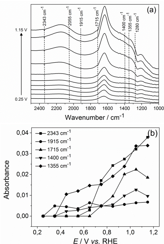
Fig. 32. (a) In situ infrared spectra recorded in 0.5M H 2 SO 4 + 1M EtOH on Pt/C at room temperature and (b) band intensities evolution (at 2343, 1915, 1715, 1400 and 1355 cm -1 ) against the applied potential; R ref = 0.15 V vs. RHE. Potential range: E = 0.25 and 1.15 V vs. RHE; Potential step: E = 0.1 V.
