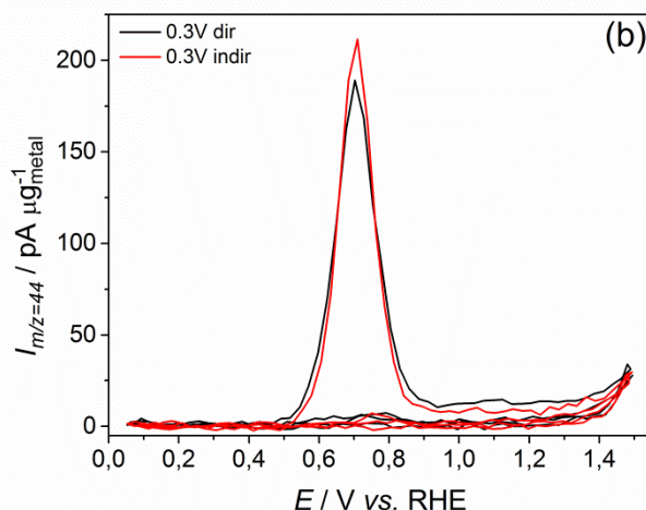
Fig. 59. (a) CV of the electrooxidation of ethanol adsorbates in 0.5 M H 2 SO 4 after adsorption at E_{\text{ad}} = 0.3 V vs. RHE (black) without and (red) with a first reduction scan and the corresponding MSCV for mass-to-charge ratio (b) m/z = 44 on Pt/C; \nu = 10 mV s -1 ; T = 25^\circ\text{C} .
