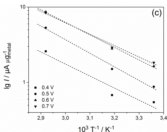
Fig. 81. Arrhenius plots of the of potentiostatic currents recorded after 900 s at potentials from E = 0.4 to 0.7 V vs. RHE (0.1 V step) in 0.5 M H_2SO_4 + 0.1 M EtOH on (a) Pt/C, (b) Pt-Rh/C and (c) Pt-Rh-SnO 2 /C.
