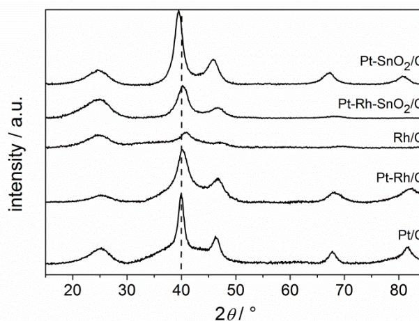
Fig. 24. XRD pattern of carbon supported 20 wt.% Pt/C, Rh/C, Pt-Rh/C, Pt-SnO 2 /C and Pt-Rh-SnO 2 /C electrocatalysts prepared by Polyol method.
