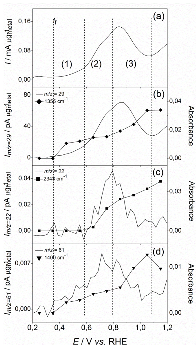
Fig. 33. (a) EOR cyclic voltammetry (in 0.5 M H 2 SO 4 + 0.1 M EtOH) and corresponding MSCV associated with EOR infrared bands (from Fig. 32b): (b) m/z = 29 + 1355 \text{ cm}^{-1} , (c) m/z = 22 + 2343 \text{ cm}^{-1} and (d) m/z = 61 + 1400 \text{ cm}^{-1} on Pt/C; \nu = 10 \text{ mV s}^{-1} ; T = 25^\circ\text{C} .
