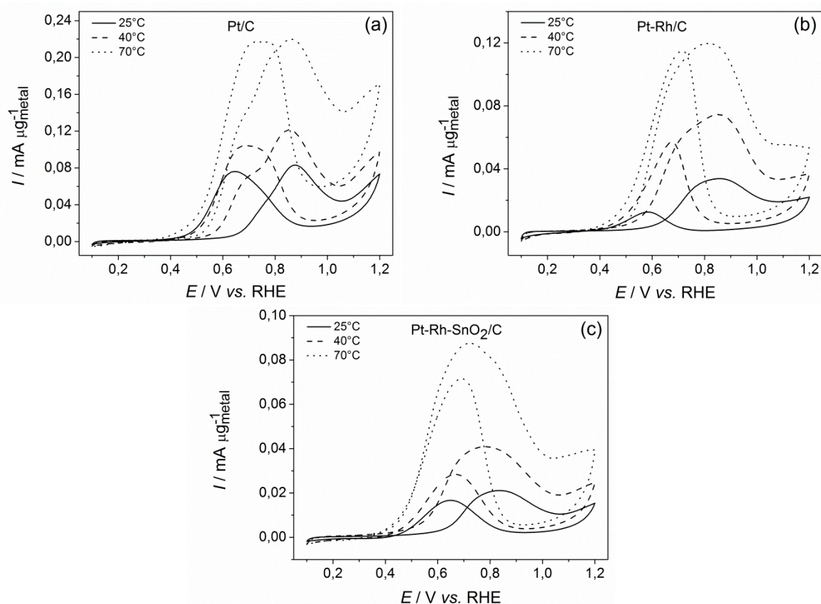
Fig. 79. CV in 0.5 M H 2 SO 4 + 0.1 M EtOH of the EOR on (a) Pt/C, (b) Pt-Rh/C and (c) Pt-Rh-SnO 2 /C; T = 25^{\circ}\text{C} (solid), 40^{\circ}\text{C} (dash) and 70^{\circ}\text{C} (dots); \nu = 10 \text{ mV s}^{-1} .
