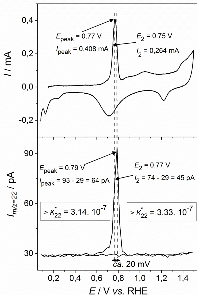
Fig. 11. K_{22}^* calibration using a CO-stripping CV in 0.5 M H_2SO_4 on Pt/C and its associated mass-to-charge signal m/z = 22 .
