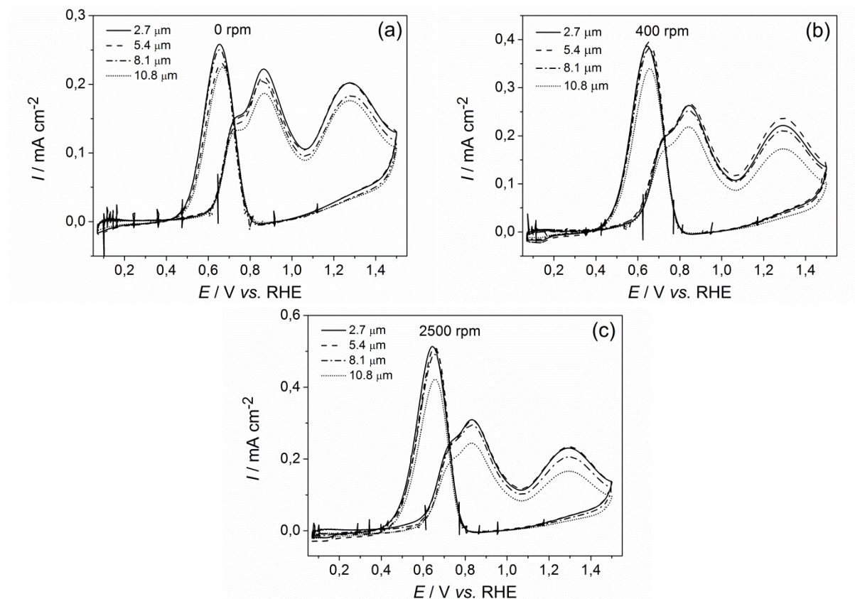
Fig. 17. CV in 0.5 M H 2 SO 4 + 0.1 EtOH on Pt/C ( L = 2.7, 5.4, 8.1 and 10.8 \mu\text{m} ) on a RDE at different rotation speeds: \omega = (a) 0, (b) 400 and (c) 2500 rpm; v = 10 \text{ mV s}^{-1} ; T = 25^\circ\text{C} .
