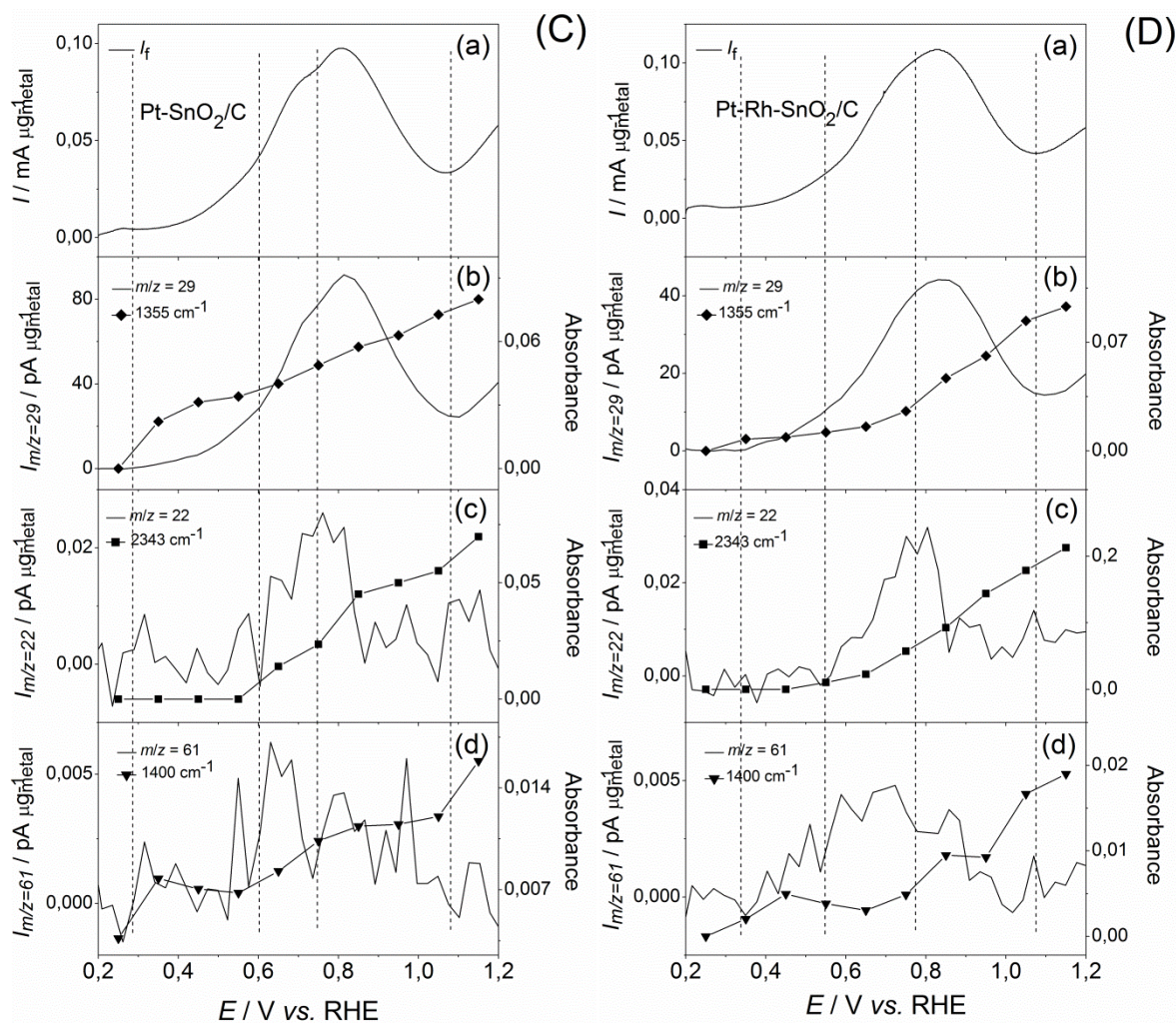
Fig. 36. (a) EOR cyclic voltammetry (in 0.5 M \text{H}_2\text{SO}_4 + 0.1 M EtOH) on (A) Rh/C, (B) Pt-Rh/C, (C) Pt-SnO 2 /C and (D) Pt-Rh-SnO 2 /C and corresponding MSCVs associated with EOR IR-bands (from Fig. 35): (b) m/z = 29 + 1355 \text{ cm}^{-1} , (c) m/z = 22 + 2343 \text{ cm}^{-1} and (d) m/z = 61 + 1400 \text{ cm}^{-1} on Pt/C; \nu = 10 \text{ mV s}^{-1} ; T = 25^\circ\text{C} .
