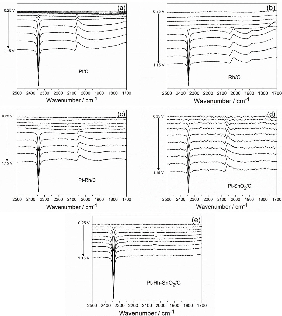
Fig. 28. In situ infrared spectra recorded during CO stripping in 0.5 M H 2 SO 4 on (a) Pt/C, (b) Rh/C, (c) Pt-Rh/C, (d) Pt-SnO 2 /C and (e) Pt-Rh-SnO 2 /C; T = 25°C.
