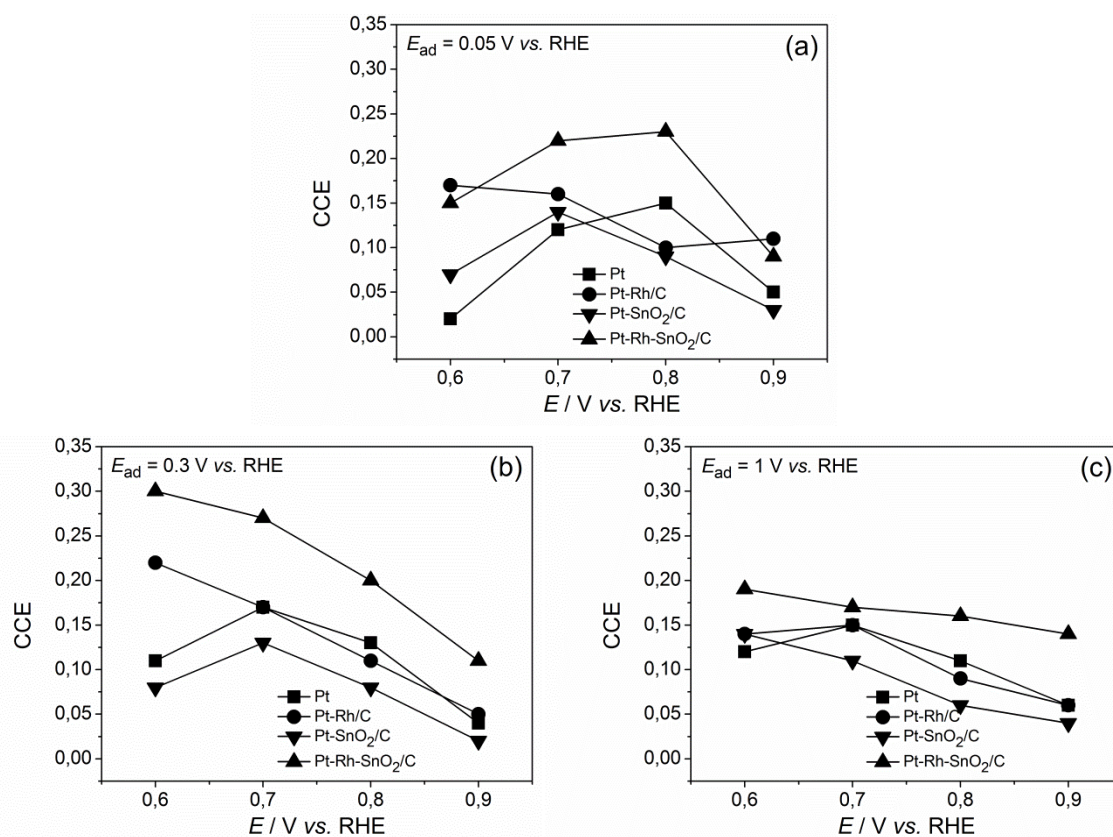
Fig. 46. Potentiodynamic EOR CO_2 current efficiency (CCE) values deduced from cyclic voltammeteries in 0.5 M H_2SO_4 + 0.1 M EtOH on Pt/C, Pt-Rh/C, Pt- SnO_2/C and Pt-Rh- SnO_2/C preceded by CA at E_{ad} = (a) 0.05, (b) 0.3 and (c) 1 V vs. RHE.
