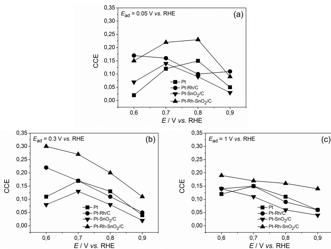
Fig. 46. Potentiodynamic EOR \text{CO}_2 current efficiency (CCE) values deduced from cyclic voltammeteries in 0.5 \text{ M H}_2\text{SO}_4 + 0.1 \text{ M EtOH} on Pt/C, Pt-Rh/C, Pt-SnO 2 /C and Pt-Rh-SnO 2 /C preceded by CA at E_{ad} = (a) 0.05, (b) 0.3 and (c) 1 V vs. RHE.
