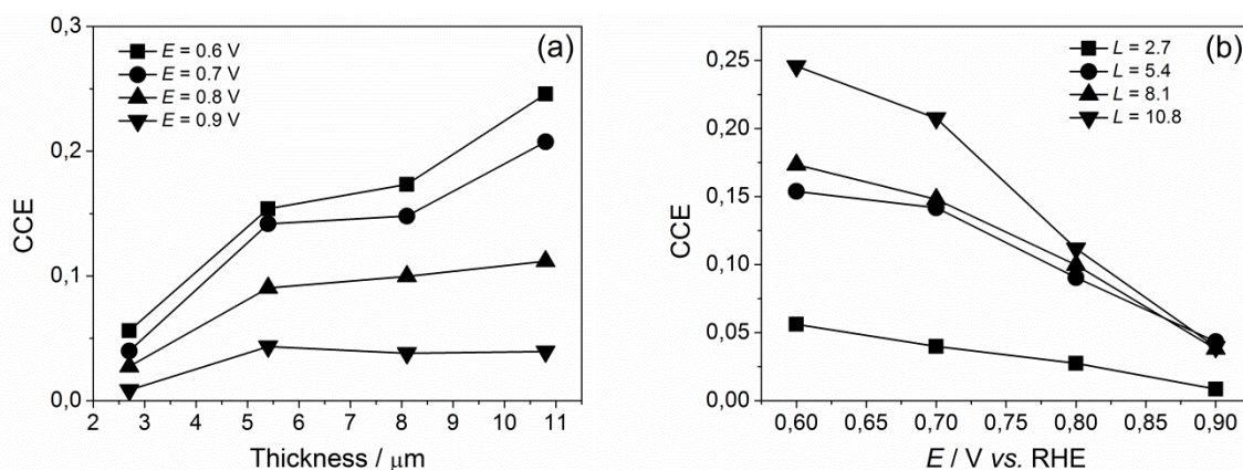
Fig. 16. Evolution of the EOR \text{CO}_2 current efficiency (CCE) against (a) the electrocatalyst thickness and (b) the applied potential calculated from cyclic voltammeteries run in 0.5\text{ M H}_2\text{SO}_4 + 0.1\text{ M EtOH} (represented in Fig. 15a) and corresponding MSCVs (Fig. 15b) on Pt/C.
