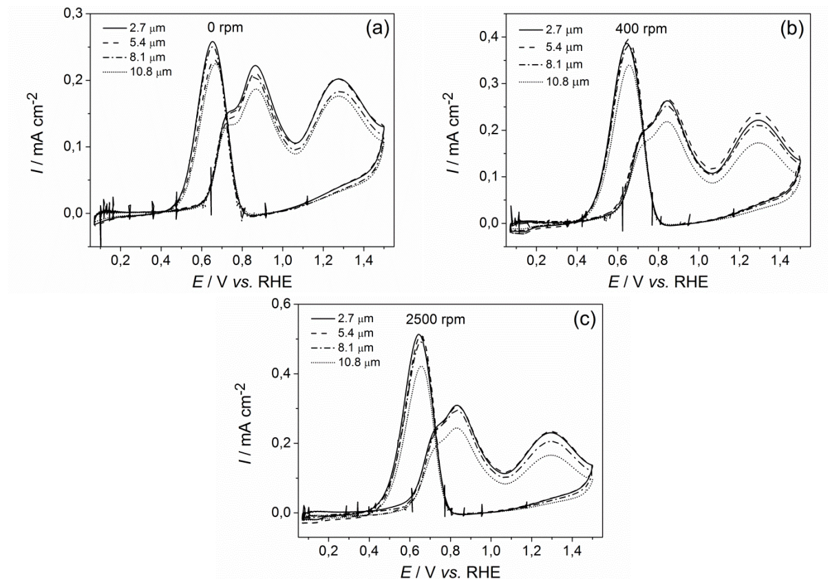
Fig. 17. CV in 0.5 M \text{H}_2\text{SO}_4 + 0.1 EtOH on Pt/C ( L = 2.7, 5.4, 8.1 and 10.8 \mu\text{m} ) on a RDE at different rotation speeds: \omega = (a) 0, (b) 400 and (c) 2500 rpm; v = 10 \text{ mV s}^{-1} ; T = 25^\circ\text{C} .
