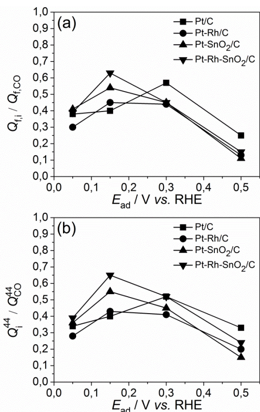
Fig. 70. Relative coverage of Pt/C, Pt-Rh/C, Pt-SnO 2 /C and Pt-Rh-SnO 2 /C electroactive surface by ethanol CO-like adsorbates (oxidizing at 0.4 V < E < 0.9 V vs. RHE) adsorbed at E_{ad} = 0.05, 0.15, 0.3 and 0.5 V vs. RHE deduced from (a) faraday charges and (b) ionic charges from the mass-to-charge signal m/z = 44 .
