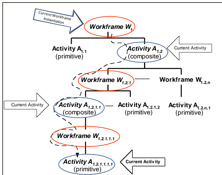
Figure 5.3 Workframe-Activity hierarchy
