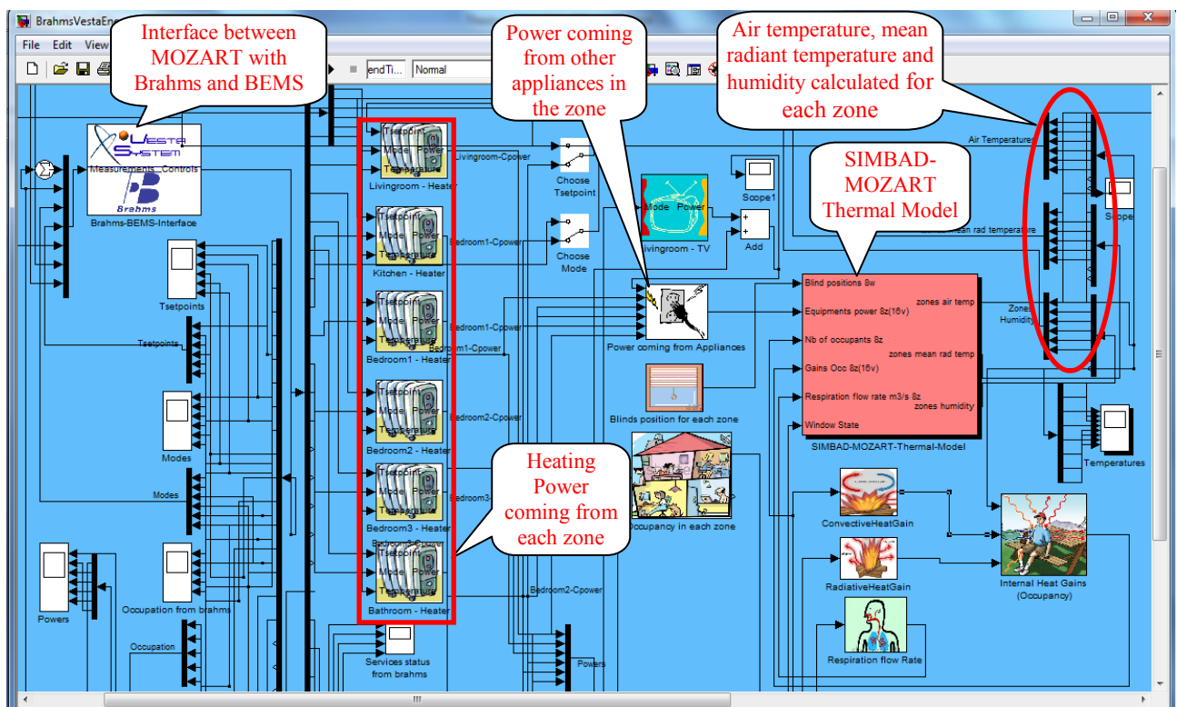
Figure 7.10 Co-simulation environment
