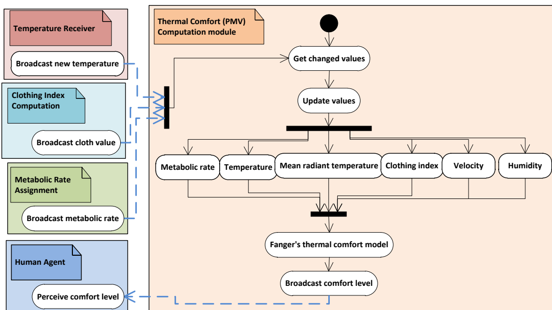
Figure 7.9 Thermal comfort (PMV) computation module
