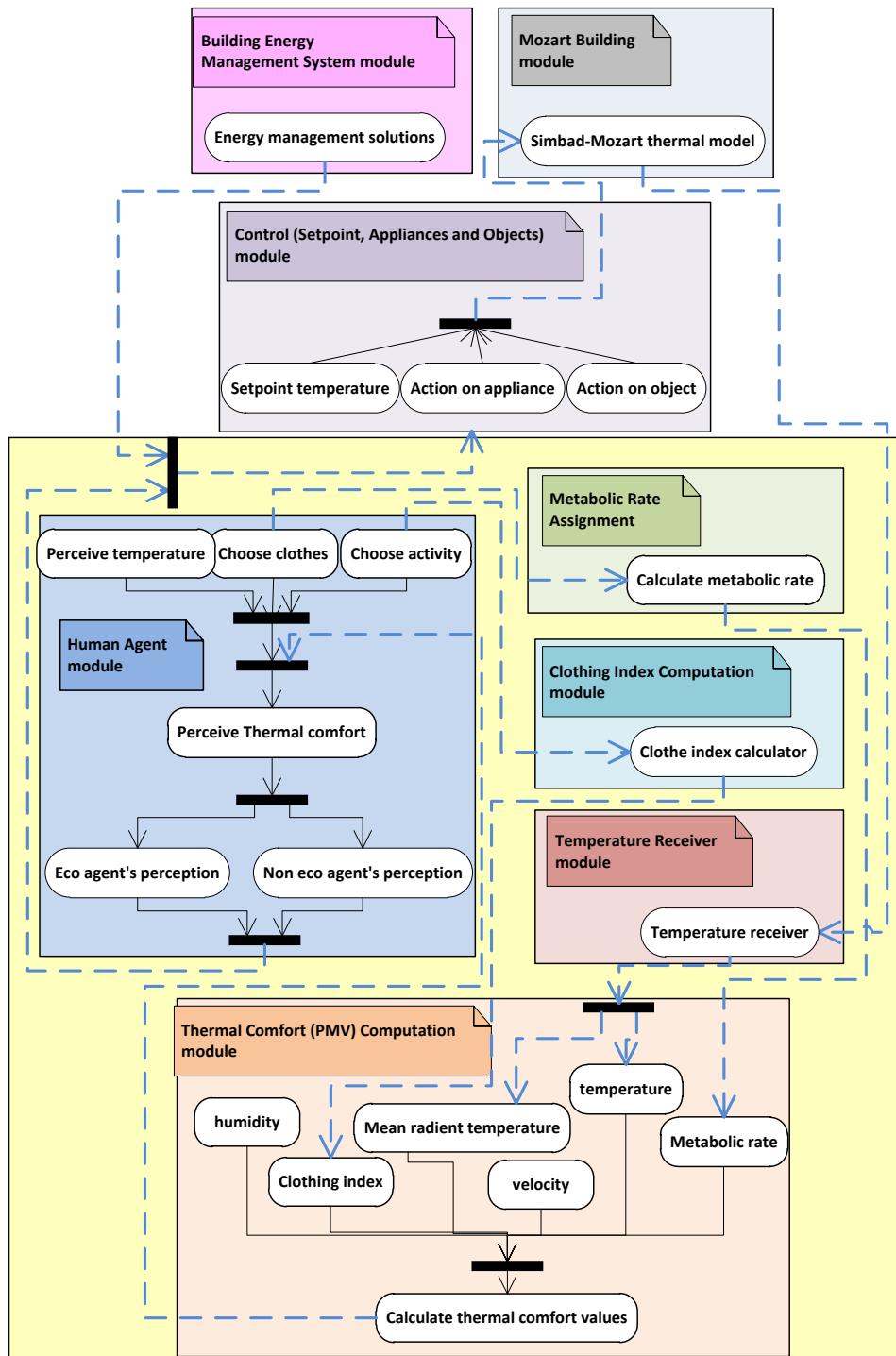
Figure 7.1 Co-Simulation between inhabitant’s behaviour, SIMBAD and BEMS
