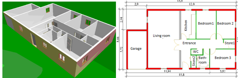
Figure 7.2 MOZART house plan
