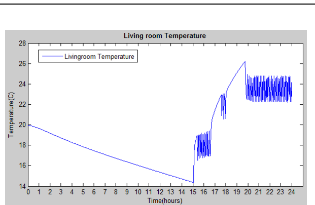
(b) Temperature controlled by agent and BEMS
