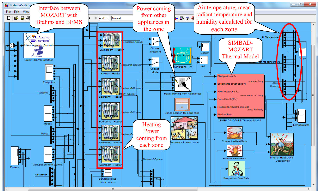
Figure 7.10 Co-simulation environment
