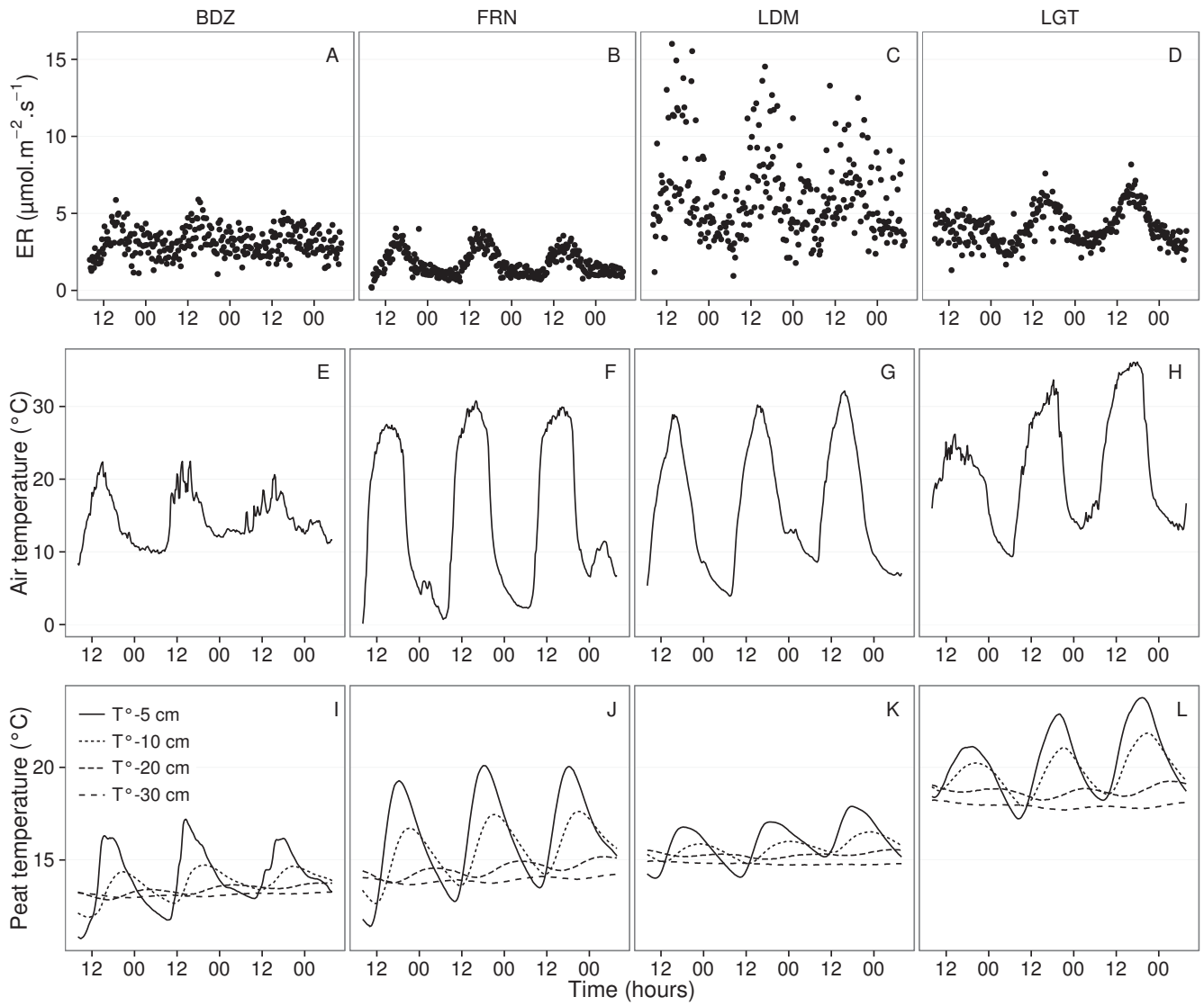
FIGURE 5.1 – Ecosystem Respiration (ER), air and peat temperature, in the 4 sites (Bernadouze : BDZ, Frasné : FRN, Landemarais : LDM, La Guette : LGT). All data points from all replicates are shown.
