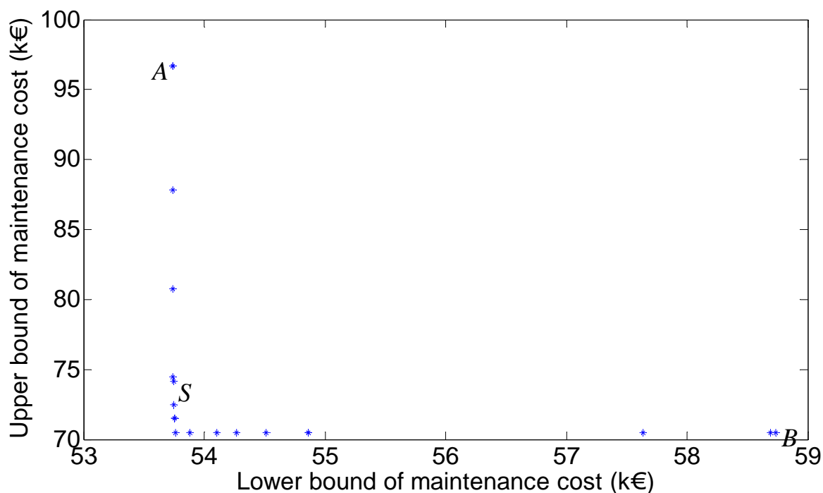
Fig. 7. The Pareto front obtained within the region [0, 100] \text{ k€} \times [0, 100] \text{ k€} .
