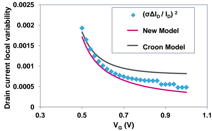
Figure II. 10: V_G > V_t ( V_G in the range of 0.5\text{--}1\text{V} , with V_t=0.36\text{V} ). Comparison between the new drain current mismatch model, the drain current mismatch model proposed by Croon and the measured drain current mismatch as a function of V_G (FD SOI transistors with W=1\mu\text{m}/L=0.1\mu\text{m} and V_D=50\text{mV} , R_{sd}=220\Omega ).
