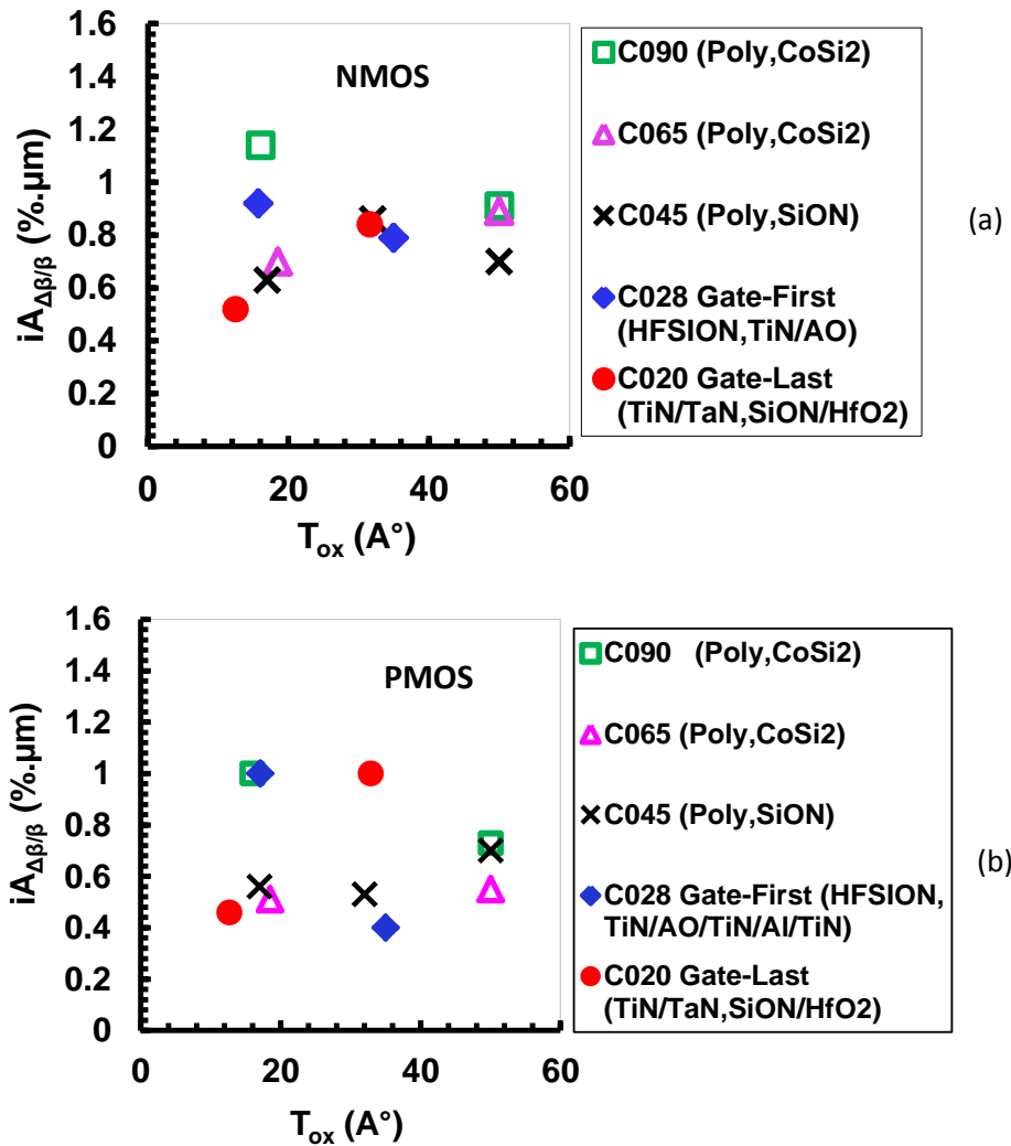
Figure V. 14: Trend of iA_{\Delta\beta/\beta} (%-\mu\text{m}) as a function of the oxide thickness T_{ox} (\text{\AA}) from 90nm ST Bulk technology to 20nm Gate-Last Bulk technology (a) for NMOS devices and (b) for PMOS devices.
