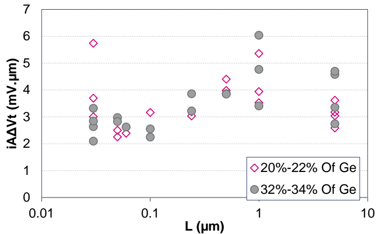
Figure IV. 16: Transistors with Pockets: Comparison of iA_{\Delta V_t} as a function of L between the minimum and the maximum considered percentages of Ge.
