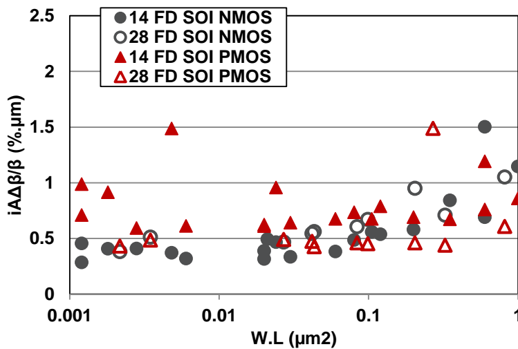
Figure VI. 8: Comparison of i\Delta\beta/\beta ( \%\cdot\mu\text{m} ) as a function of S ( \mu\text{m}^2 ) between NMOS and PMOS devices of the 28nm and 14nm FD SOI technologies.
