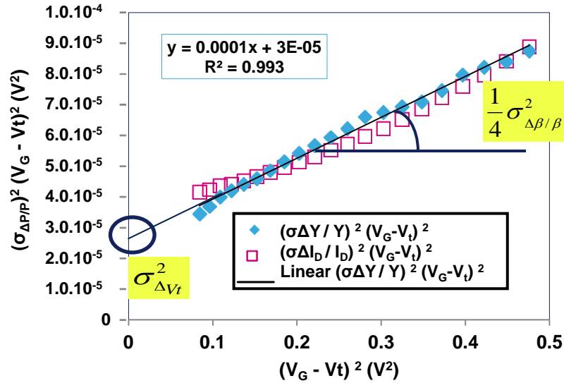
Figure II. 13: V_G > V_t ( V_G in the range of 0.6-1V, with V_t=0.31V ). Y function and drain current mismatch multiplied by (V_G - V_t)^2 and plotted as a function of (V_G - V_t)^2 (BULK transistors with W=10\mu\text{m}/L=0.03\mu\text{m} and V_D=50\text{mV} ).
