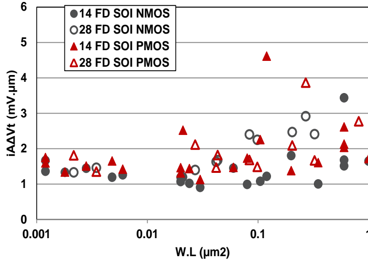
Figure VI. 7: Comparison of i\Delta V_t ( \text{mV}\cdot\mu\text{m} ) as a function of S ( \mu\text{m}^2 ) between NMOS and PMOS devices of the 28nm and 14nm FD SOI technologies.
