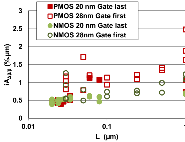
Figure V. 12: Comparison of iA_{\Delta\beta/\beta} (%. \mu m ) as a function of L ( \mu m ) between NMOS and PMOS devices of the 28nm Gate-First and 20nm Gate-Last technologies.
