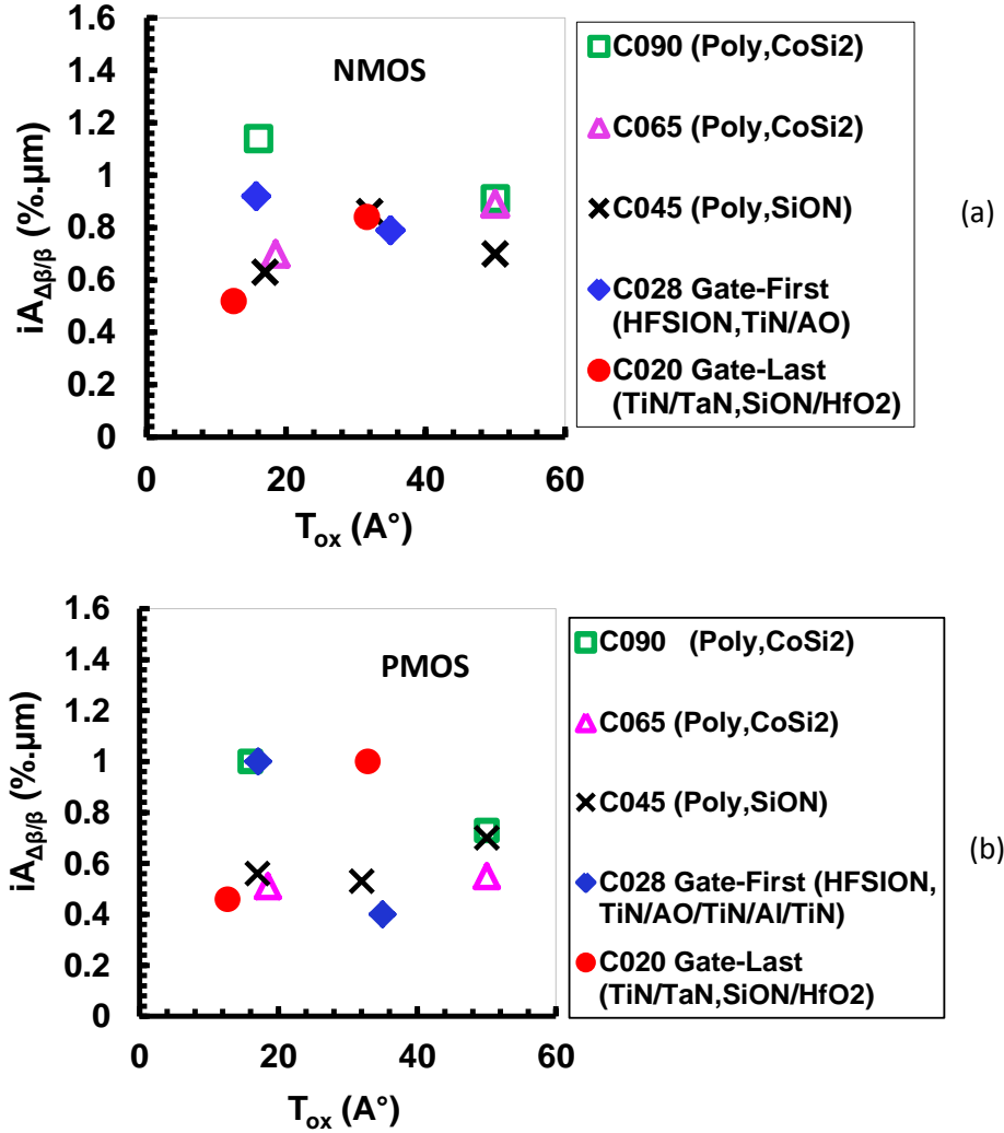
Figure V. 14: Trend of iA_{\Delta\beta/\beta} (%. \mu\text{m} ) as a function of the oxide thickness T_{ox} ( \text{\AA} ) from 90nm ST Bulk technology to 20nm Gate-Last Bulk technology (a) for NMOS devices and (b) for PMOS devices.
