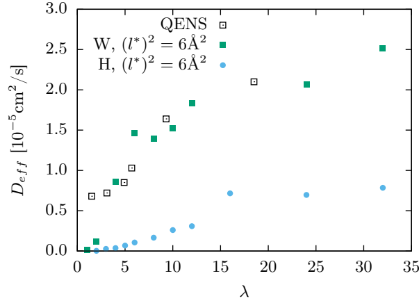
Figure 6.13: Effective diffusion coefficients of water and hydronium ions at a cutoff distance of 6\text{\AA}^2 . For comparison, the corresponding experimental values are also represented.
