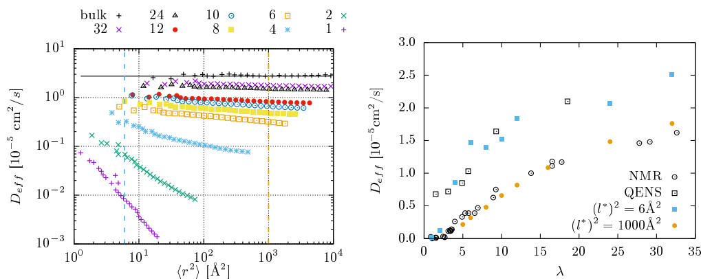
Figure 6.3: Left : The effective diffusion coefficient, D_{\text{eff}} , computed from Eq. (1.10), plotted parametrically against \langle r^2(t) \rangle . The solid black line is the result in the bulk for the considered water model, corresponding to D \simeq 2.74 \times 10^{-5} \text{ cm}^2/\text{s} . The dashed vertical lines, indicate the (squared) length scales \simeq 6 and \simeq 1000 \text{ \AA}^2 used to select the values of D_{\text{eff}} shown in the bottom panel, as discussed in the text. Right : The values for D_{\text{eff}} selected by the two verticals lines of the above panel are shown as closed symbols. We also show the diffusion coefficients obtained by PFG-NMR and QENS spectroscopy [119], which probe the dynamics on long and short length scales, respectively.
