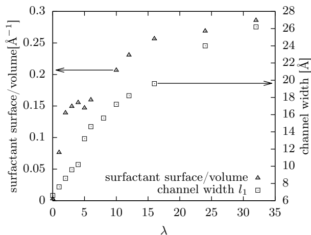
Figure 5.6: Variation with the water content, \lambda , of the average size of the self-assembled ionic channels and the extension of the generated hydrophobic/hydrophilic interfaces, normalised to the volume occupied by the surfactant macromolecules. Data for the confining size are similar to those reported in [156] and in the previous chapters, re-evaluated from the new system snapshots. The arrows indicate the axis relevant for each data set.
