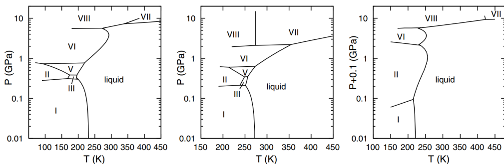
Figure 2.1: The phase diagram of water from experiment (centre) and computer simulations of TIP4P (left) and SPC/E (right) water models. Adapted from [14].
