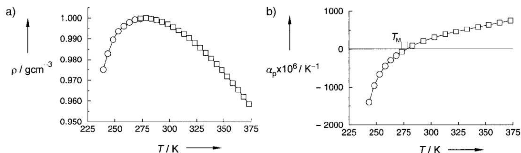
Figure 2.2: Structural anomalies of water. Temperature dependence of the density (a), and volume expansion coefficient (b) of water. Adapted from [16].
