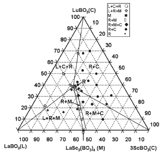
Fig. 2. Quasi-ternary phase diagram of LuBO_3 – LaBO_3 – ScBO_3 system; R, trigonal phase; C, solid solution of Lu_xSc_{1-x}BO_3 ; L, LaBO_3 ; M, monoclinic phase of LaSc_3(BO_3)_4 .
