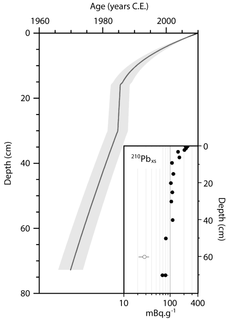
Figure 37. DTCI 2010 chronology. DTCI 2010 age model (dark line) based on ^{210}\text{Pb}_{\text{xs}} and associated age-model errors (grey area). The inset corresponds to the down core profile of ^{210}\text{Pb}_{\text{xs}} (error bars correspond to 1 SD).
