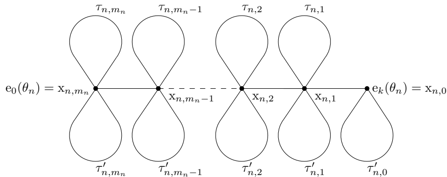
Figure 4.4 – Notation for the vertices and subtrees of \theta_n^{(k)} .
