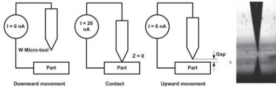
Fig. 2. Protocol for the adjustment of the gap.
