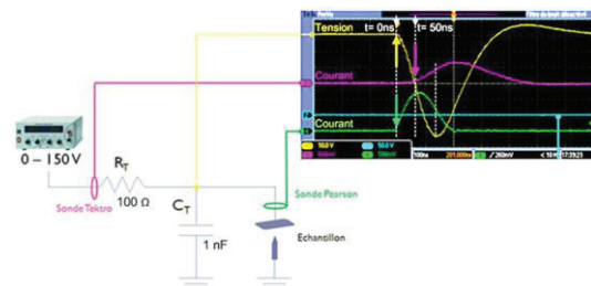
Fig. 10. Voltage drop (yellow), pulse current in the plasma (green) and current flowing out the power supply (violet) ( R_T = 100 \Omega , C_T = 1 \text{ nF} , gap = 3 \mu\text{m} , I_c = 1.3 \text{ A} , \Delta U = 65 \text{ V} ).
