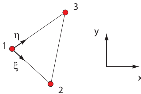
Figure 6.5: Triangular element
