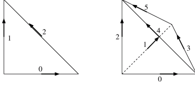
Figure 1.8: The Nedelec elements in 2D and 3D
