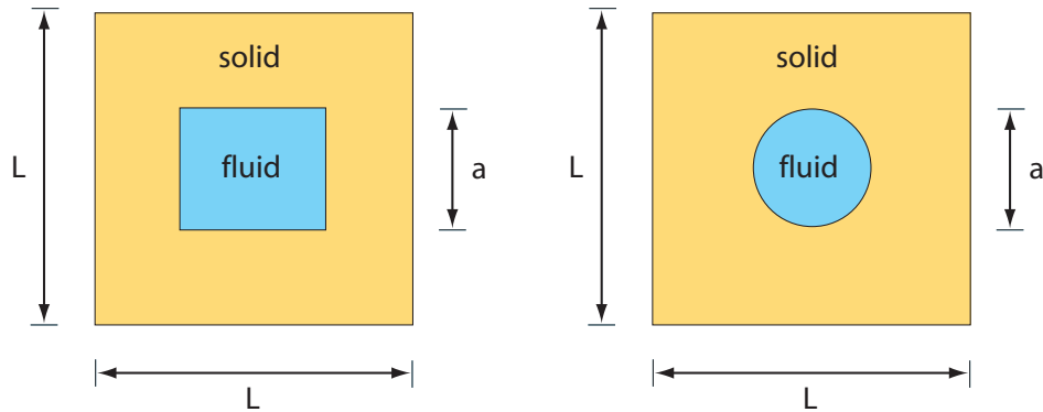
Figure 6.17: Definition of the unit cells for the flow through in a nano-porous solid containing squared or circular macropores.
