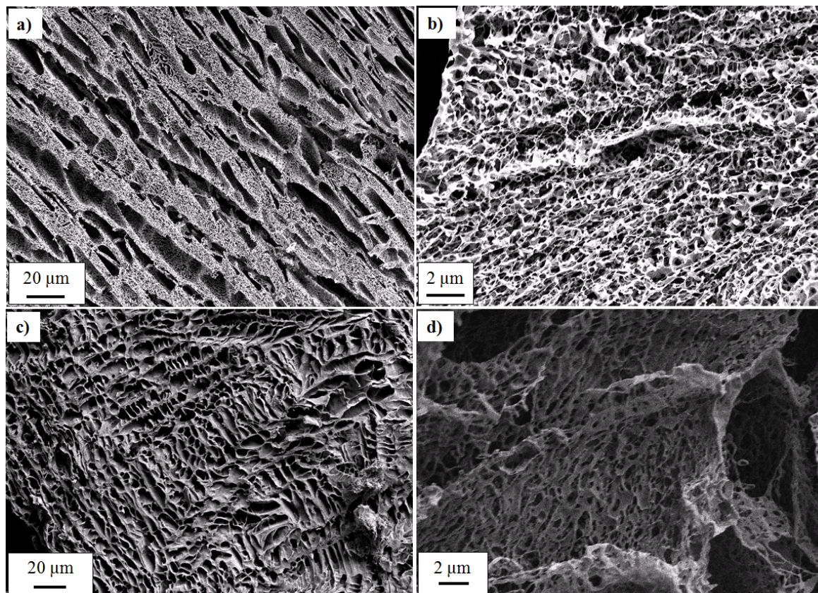
Figure 3.3: SEM micrographs of porous PHEMA samples prepared by TIPS at 2.5% (wt/v) of polymer concentration: (a), (b) cooling to -80^{\circ}\text{C} ; (c), (d) cooling to -196^{\circ}\text{C} . The co-solvent mixture contained 78/22 vol.% of water/dioxane.
