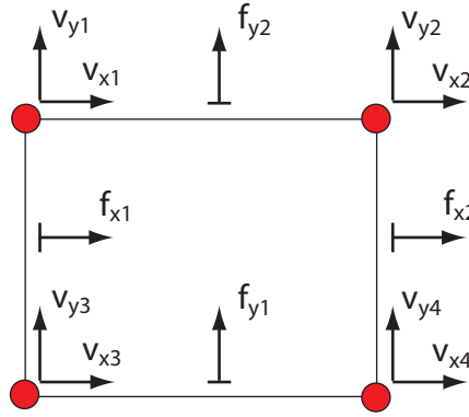
Figure 6.3: Degrees of freedoms of the Arbogast and Brunson rectangular element
