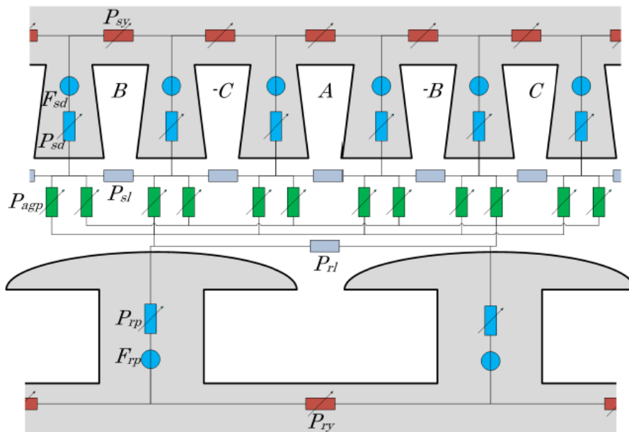
Fig.1. 24 Lumped element models applied to a synchronous generator [PETRICHENKO 07]
