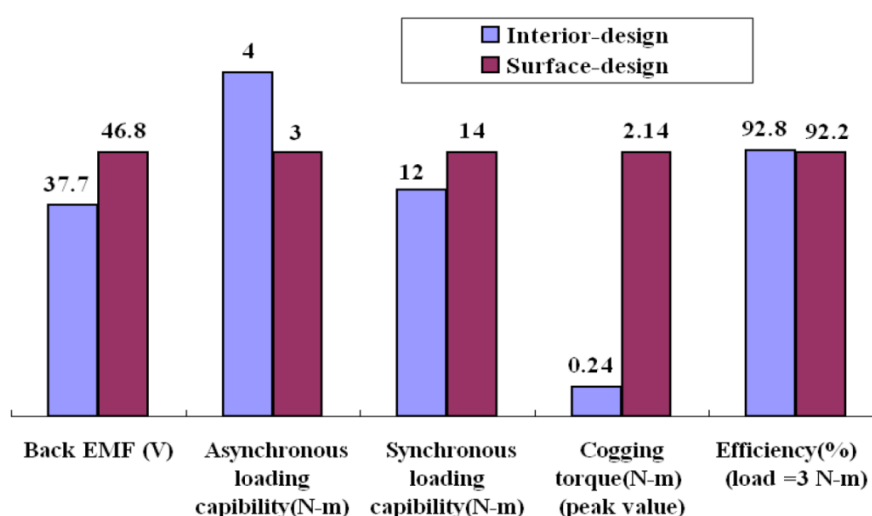
Fig.1. 18 Comparison of characteristics of two LSPMs of different rotor structures [HUANG 08]
