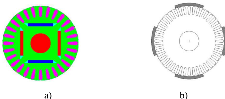
Fig.1. 16 Two rotor structures of line-start permanent magnet synchronous motor: (a) interior-magnet line-start permanent magnet synchronous motor; (b) surface-magnet line-start permanent magnet synchronous motor
