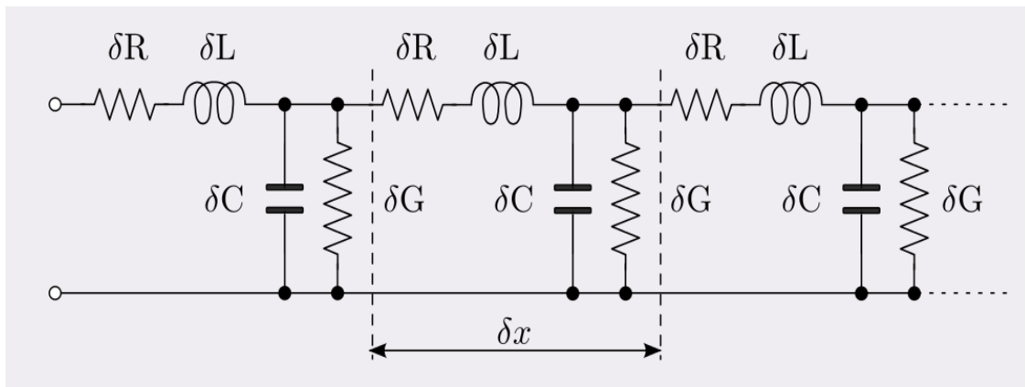
Fig.1. 23 Distributed element model applied to a transmission line
