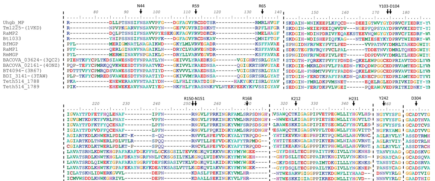
Figure 5 Sequence alignment of characterized GH130 enzymes. This alignment highlights the conservation of the catalytic and substrate-interacting residues among characterized GH130 enzymes, as well as family-specific loops.
