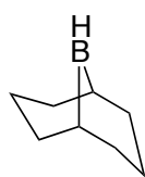
Figure 51 - 9-BBN.
