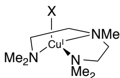
Figure 93 - [\text{Cu}^{\text{I}}(\text{PMDTA})(\text{NX})]^+ .
