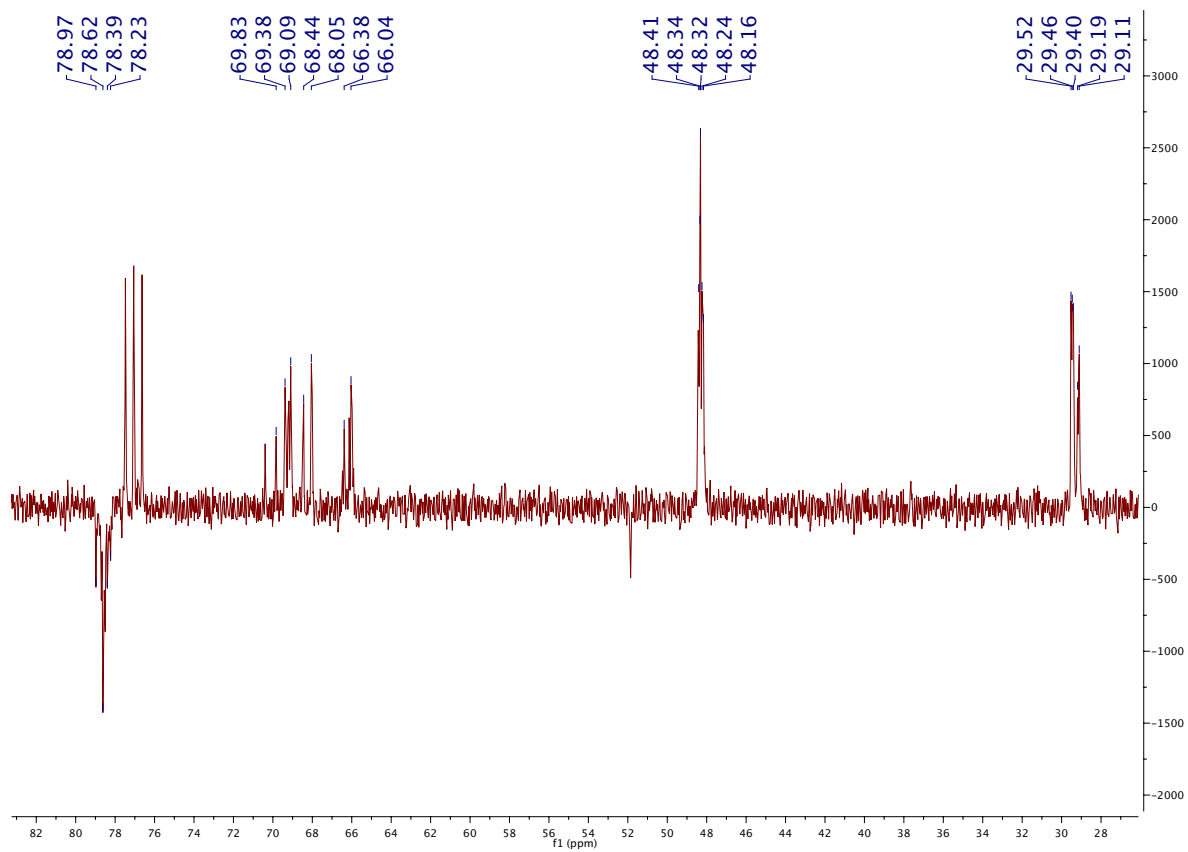
Figure 147 - Spectre RMN ^{13}\text{C} de 8c.
