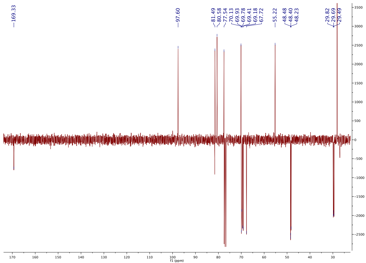
Figure 138 - Spectre RMN ^{13}\text{C} de 8a.
