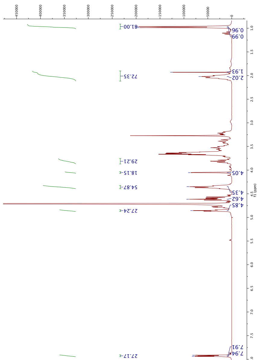
Figure 151 - Spectre RMN 1 H de 20a.
