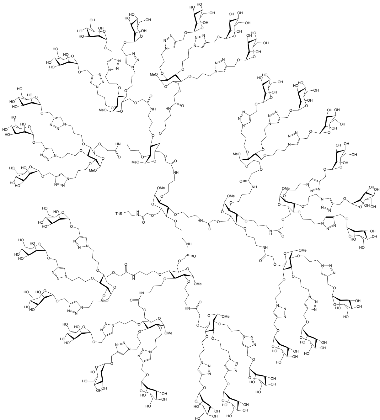
Figure 136 - Dend27Mannoses.
