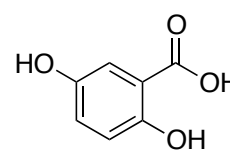
Figure 109 - DHB.
