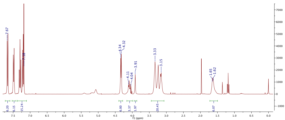
Figure 145 - Spectre RMN ^1\text{H} de 10b.
