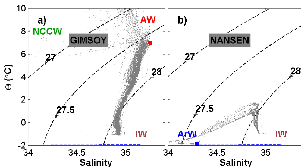
Fig. II.3 Potential temperature - Salinity Diagrams in August-September for the 1980-1985 period. (a) Gimsoy section (b) Nansen Basin. Red dot : ideal Atlantic Water, blue dot : ideal Arctic Water. Intermediate Arctic Waters : IW.
