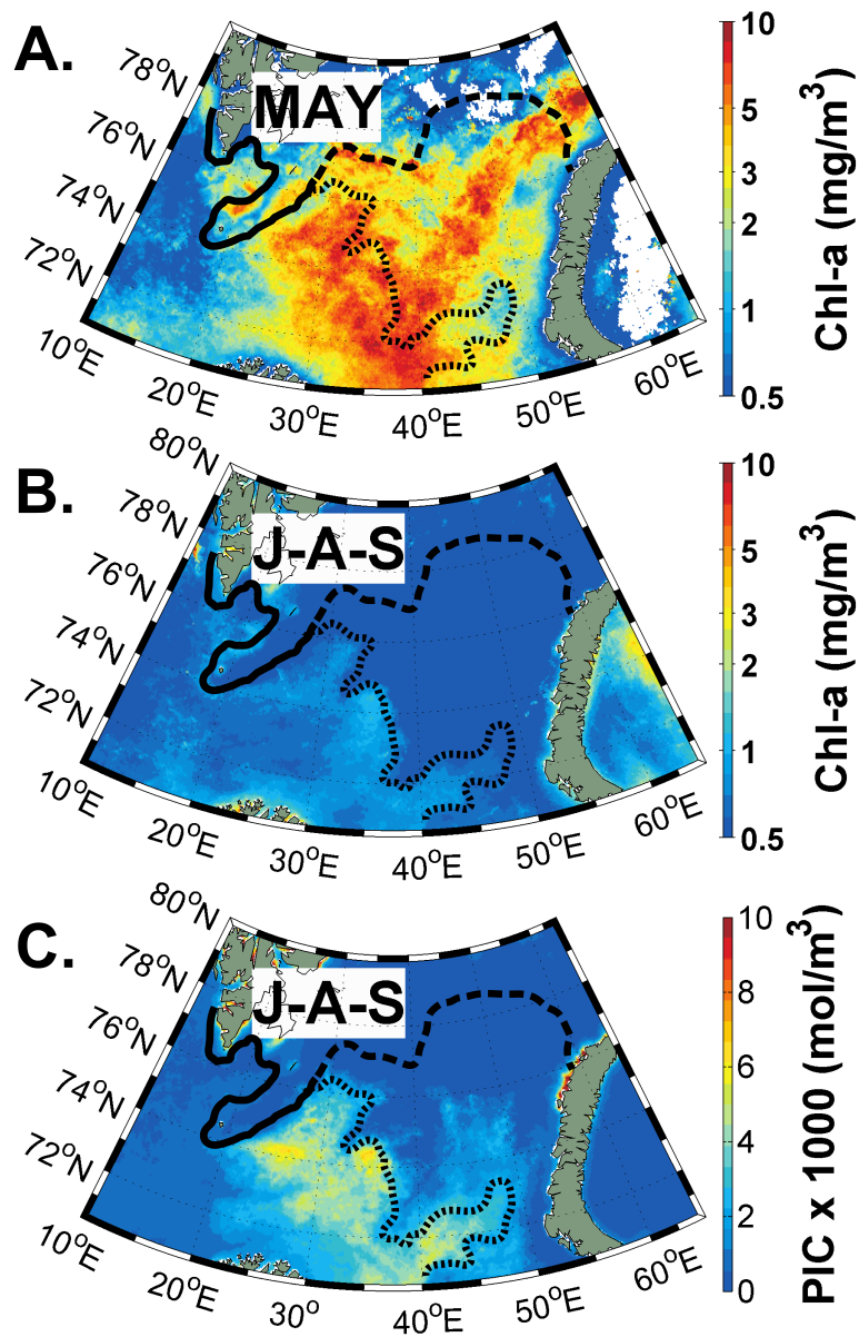
Fig. III.3 Climatology monthly maps of chl-a (mg/m 3 ) for (a) May and (b) July-August-September and (c) PIC (mol/m 3 ) (1997-2014) for July-August-September. The Polar Front is in solid line, the Southern Front in dotted line and the Northern Front in dashed line.
