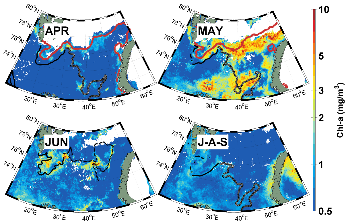
Fig. III.5 Maps of Chl-a ( \text{mg/m}^3 ) during April, May, June and July-August-September 2007. Red line is the Ice Edge, solid line is the Polar Front, dotted line is the Southern Front, dashed line is Northern Front.
