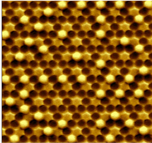
Figure F.14 Artificial Kagome Ising under applied field - Image 13
