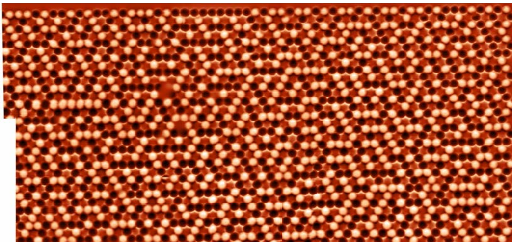
Figure E.10 Artificial Kagome Ising - MFM Image 10
