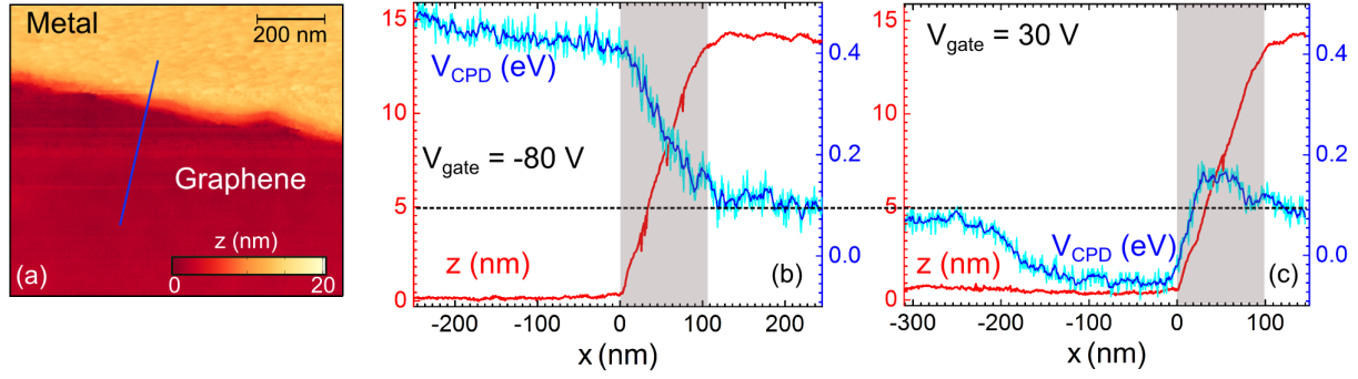
Figure 5.9: Change of V_{CPD} across the metal-graphene interface. (a) STM topograph of the metal-graphene interface. Imaging parameters: I_t = 50 pA, V_{bias} = 0.8 V, scan speed = 50 nm/s at 130 mK. (b) Change of V_{CPD} and height profile across the metal-graphene interface at high hole doping V_{gate} = -80 V \ll V_D^0 and (c) at low carrier concentration V_{gate} = 30 V \rightarrow V_D^0 . The grey window indicates the transition region between metal and graphene and the black dashed horizontal line runs along the V_{CPD} of the metal for a comparison between the two situations at high and low carrier doping.
