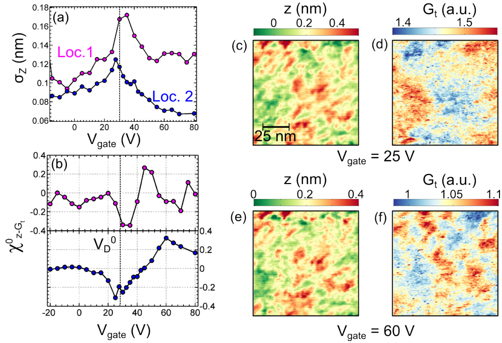
Figure 5.28: Change of (a) surface roughness \sigma_z and (b) 2D correlation coefficient between topography and the simultaneously acquired G_t(x, y) map \chi_{z-G_t}^0 [Eq.(5.4.2)] with V_{gate} for Location 1 (Figure 5.25) and 2 (Figure 5.26). (c) STM Topography and (d) the corresponding G_t(x, y) map for V_{gate} = 25 V (maximum negative correlation), for Location 2. (e) STM Topography and (f) the corresponding G_t(x, y) map for V_{gate} = 60 V (maximum positive correlation), for Location 2.
