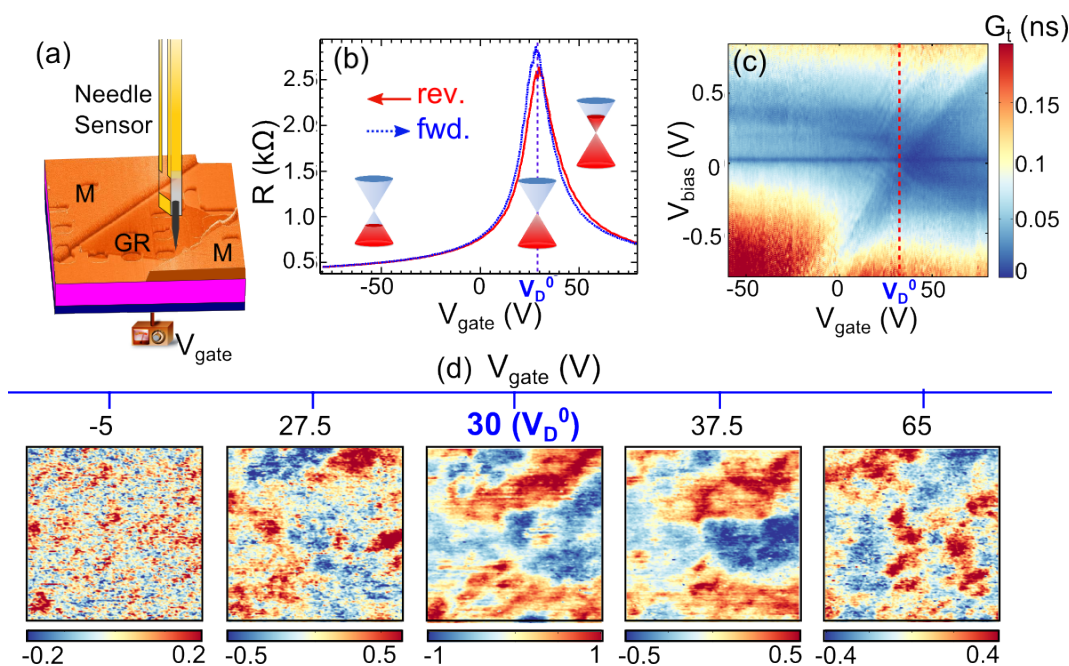
Figure 3: From macroscopic transport to charge disorder in graphene devices at various carrier concentrations. (a) Exfoliated graphene (GR) contacted with two isolated metal (M) contacts with a Needle sensor positioned on top: arrangement compatible for both transport and scanning probe microscopy. (b) Two-probe resistance as a function of V_{gate} . V_D^0 = 30 V gives the charge neutrality point. (c) Differential tunneling conductance G_t as a function of V_{bias} and V_{gate} . (d) DOS maps at different V_{gate} over an area of 100 \times 100 nm 2 .
