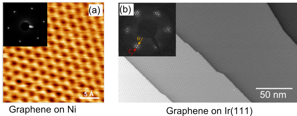
Figure 4.1: Graphene on metallic substrates. (a) Atoms resolved, constant current STM image of graphene on Ni(111) showing the perfect graphene lattice. Tunneling parameters: V_{bias} = 2 mV and I_t = 48 nA. The inset shows a LEED image obtained at 63 eV [111]. (b) STM topograph of graphene grown on Ir(111) at 1320 K. The moiré pattern due to lattice mismatch between graphene and the Ir substrate is clearly visible, extending over several Ir steps. Tunneling parameters: V_{bias} = 100 mV and I_t = 30 nA [112]. The inset shows the LEED pattern for graphene on Ir where additional intensity spots of the moiré are visible surrounding the graphene and Ir integer spots [113].
