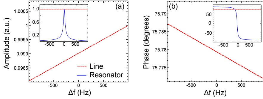
Figure 3.23: Contribution from the electrical line. (a) Amplitude of V_{out}^1/V_{exc} due to electrical line given by Eq.(3.3.6) as a function of \Delta f = f - f_0 ( C_p = 1 pF, R_{fb} = 22 k \Omega and the rest of the parameters are same as in Figure 3.20). Inset shows the simultaneous variation in the amplitude of the resonator response. (b) Phase of V_{out}^1/V_{exc} as a function of \Delta f . Inset shows the simultaneous variation in the phase of the resonator response.
