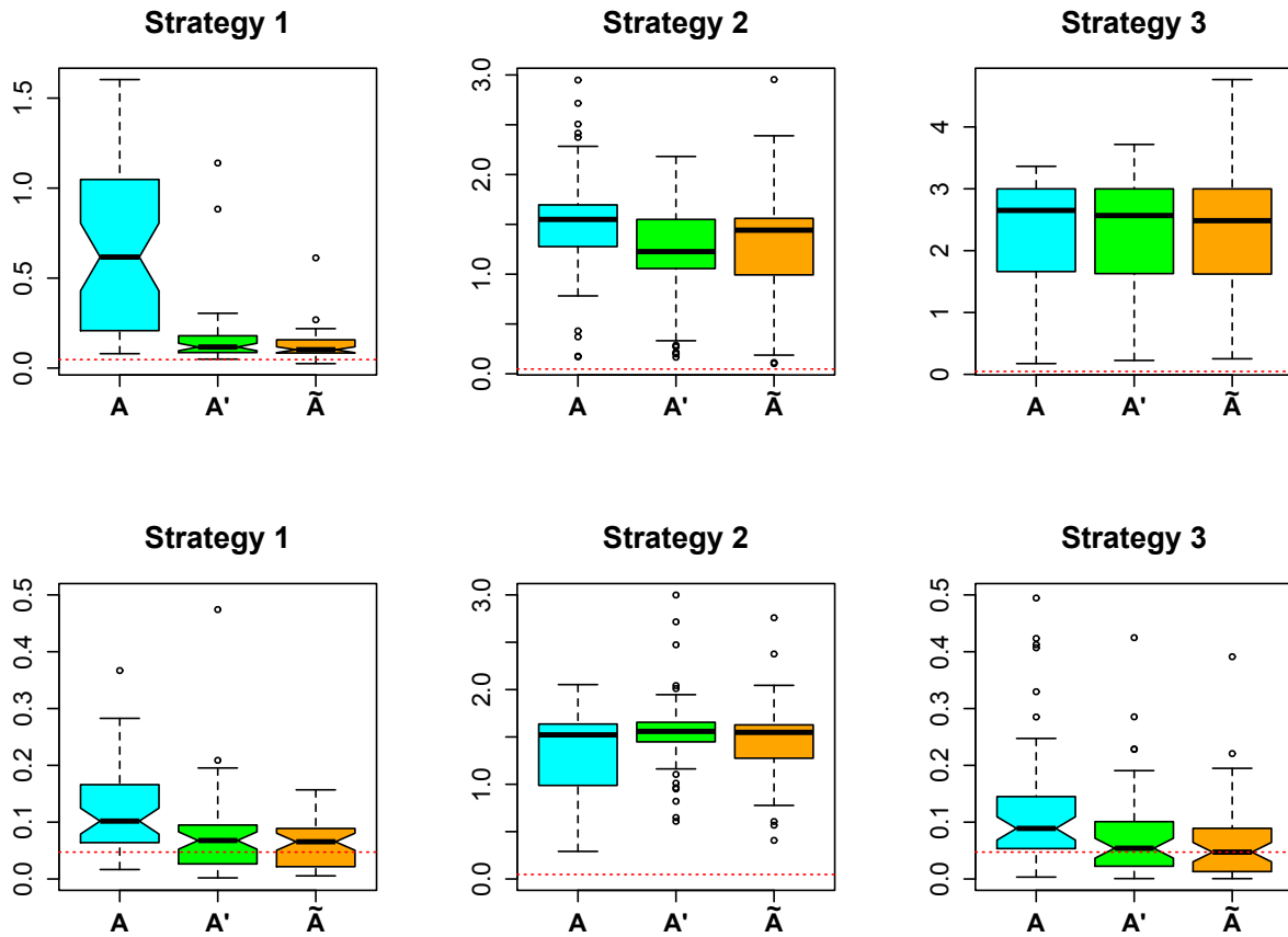
Figure 6.5 – Optimalty gap for the Hartman6 function with D = 25 over 50 runs with a budget of 250 evaluations, with k_y (top) and k_\Psi (bottom). For each strategy, matrices \mathbf{A} , \mathbf{A}' and \tilde{\mathbf{A}} are tested. The red dashed line indicates the best median performance, i.e. for strategy 3 with \tilde{\mathbf{A}} .
