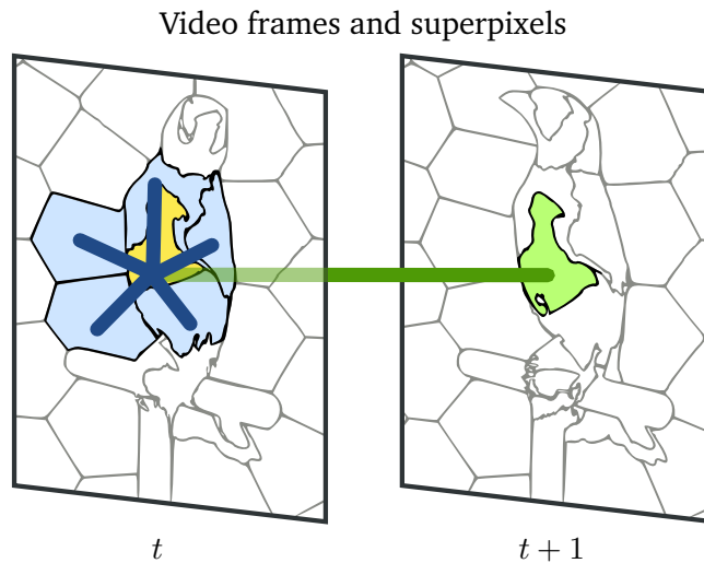
Fig. 6.2: Spatio-temporal graph of superpixels. For the yellow superpixel, spatial edges are shown in dark blue and temporal edges in dark green.
