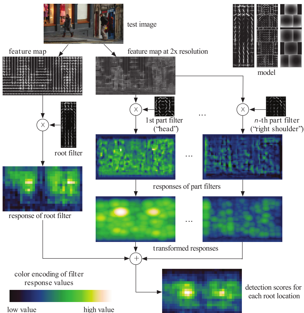
Fig. 3.2: Visualization of the efficient inference procedure for the deformable part model for object detection. Feature maps are extracted at a coarse and a fine resolution from the original image. Filter responses are computed over the entire feature maps using efficient convolution procedures. Filter response maps are then transformed using a generalized distance transform to incorporate the deformation costs. This produces maps which give the best possible part score contribution at each root part location. These maps are summed to produce the final scoremap, which gives detection scores at each possible object location and can be thresholded to produce a set of object detections. Figure from [Felzenszwalb et al. , 2013]
