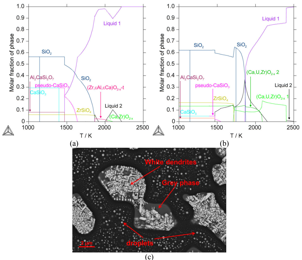
Figure 12: (a) Solidification path of Liquid 1= Al_{0.013}Ca_{0.065}Si_{0.269}Zr_{0.010}O_{0.643} ; (b) solidification path of Liquid 2= Al_{0.005}Ca_{0.011}Si_{0.249}U_{0.045}Zr_{0.028}O_{0.662} ; (c) microstructure observed in Transition zone
