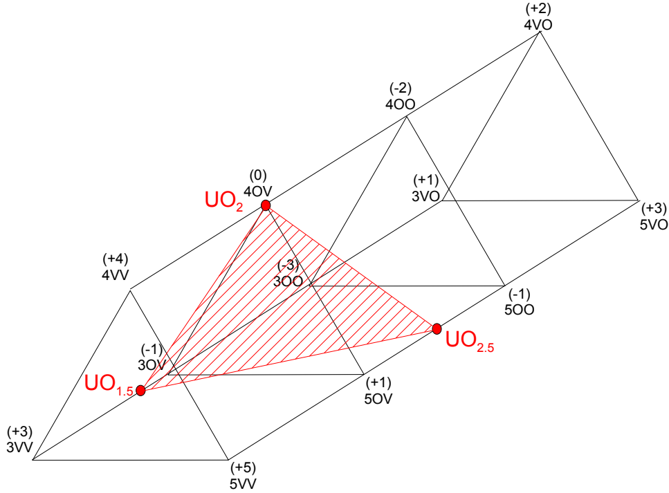
Figure 2: 3D representation of the three-sublattice model for the fcc UO_{2\pm x} phase. The red surface is the domain of composition where the phase is neutral
