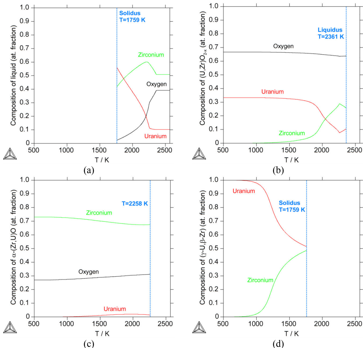
Figure 19: Composition of the phases appearing during the solidification of sample OUZr_1. (a) composition of the liquid; (b) composition of (U,Zr)O_{2-x} ; (c) composition of \alpha -Zr(O); (d) composition of (\gamma U-\beta Zr)
