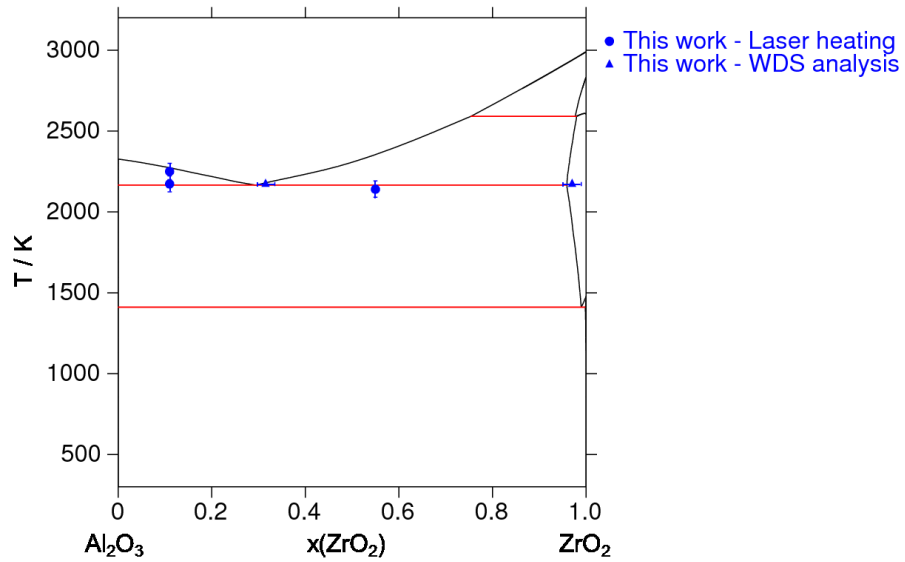
Figure 19: Comparison between current experimental results and calculated Al 2 O 3 -ZrO 2 phase diagram
