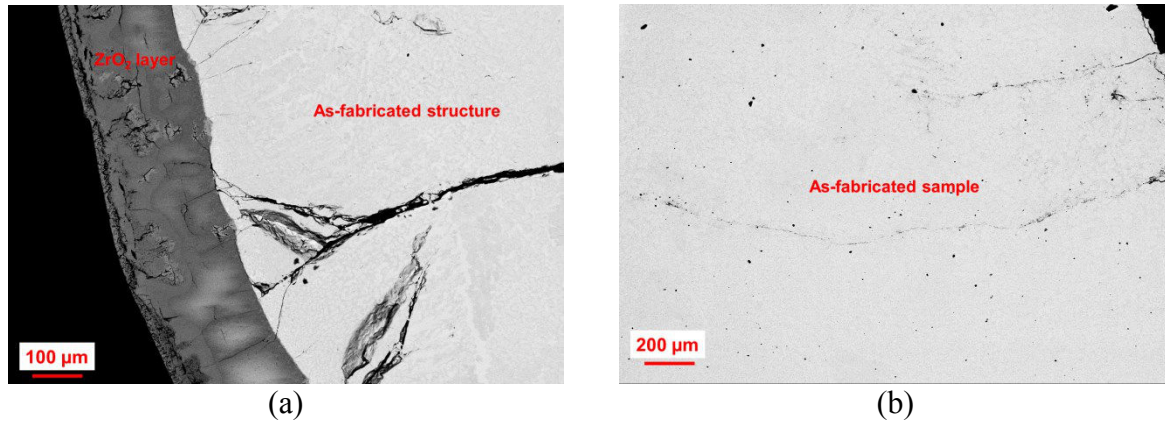
Figure 11: (a) BSE image of the microstructure of sample OFeZr_2 after a laser pulse sequence under air. A 150 μm thick ZrO 2 layer formed on the surface of the laser heated sample; (b) BSE image of sample OFeZr_2 as-fabricated by arc-melting
