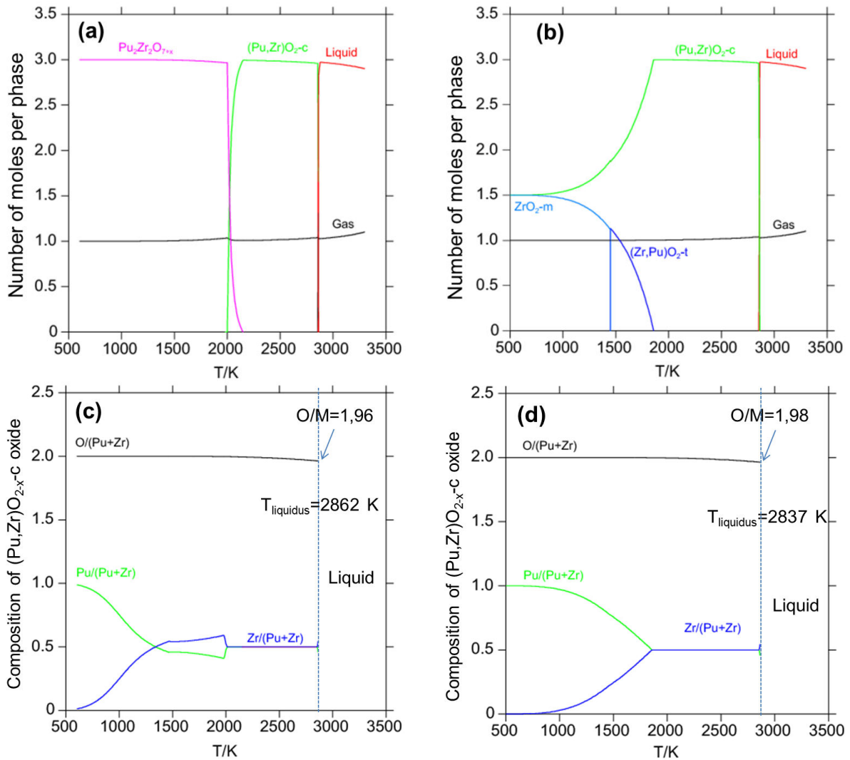
Figure 25: Calculated solidification paths on sample P50Z50. (a) Solidification path under Ar; (b) solidification path under air; (c) O/(Pu+Zr) ratio in the (\text{Pu,Zr})\text{O}_{2-x-c} phase during solidification as a function of temperature under Ar; (d) same as in (c) but obtained under air.
