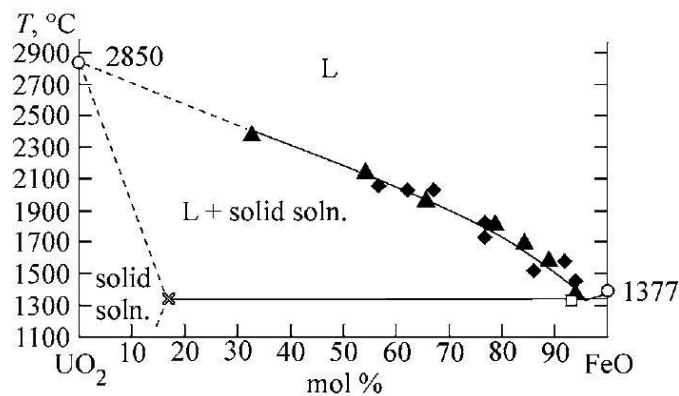
Figure 10: Tentative \text{UO}_2 - \text{FeO} phase diagram. Triangles are data from VPA IMCC, rhombuses are data obtained by using the Galakhov microfurnace, squares are DTA data and crosses are results of IMCC/XMSA [30]
