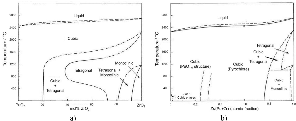
Figure 16: Tentative phase diagrams reported by Mardon et al. [39]. a) \text{PuO}_2\text{-ZrO}_2 section; b) \text{PuO}_{1.6}\text{-ZrO}_{2-x} section
