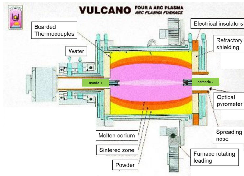
Figure 21: VULCANO furnace
