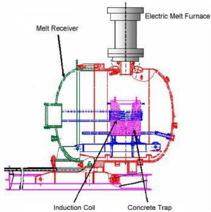
Figure 20: COTELS facility
