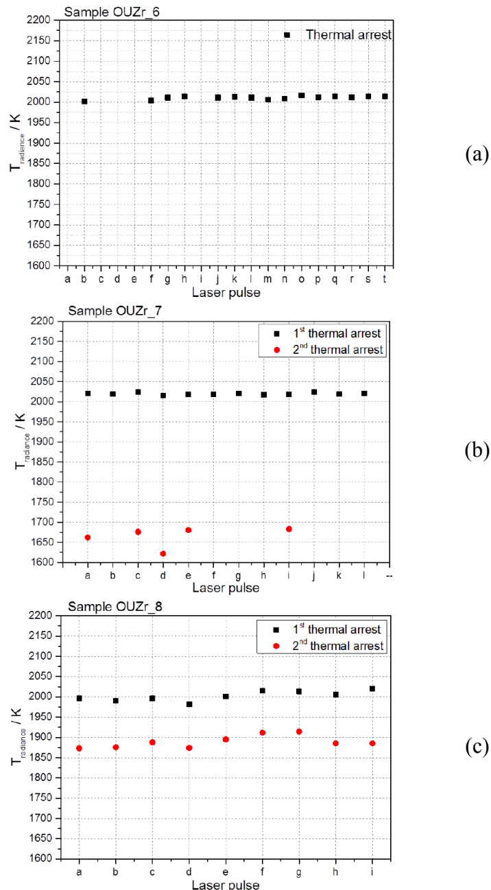
Figure 25: Summary of the experimental results obtained on samples OUZr_6, OUZr_7 and OUZr_8. The reported values are corrected only with the transmittance of the window. The reduced data dispersion in the three cases shows the excellent repeatability obtained during this experimental campaign
