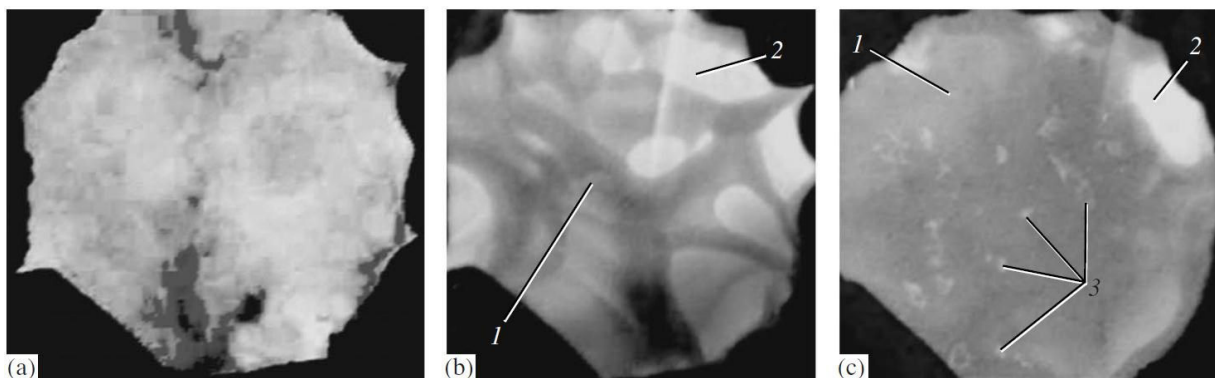
Figure 11: Image of the surface of the 50% \text{UO}_2 -50% \text{Fe}_2\text{O}_3 melt observed by Petrov et al. (a) 10 s, (b) 49 min and (c) 69 min after the beginning of the melting. With the label (1) is reported the lighter liquid, with (2) the main molten material. The label (3) refers to the gas bubbles climbing through the light liquid layer
