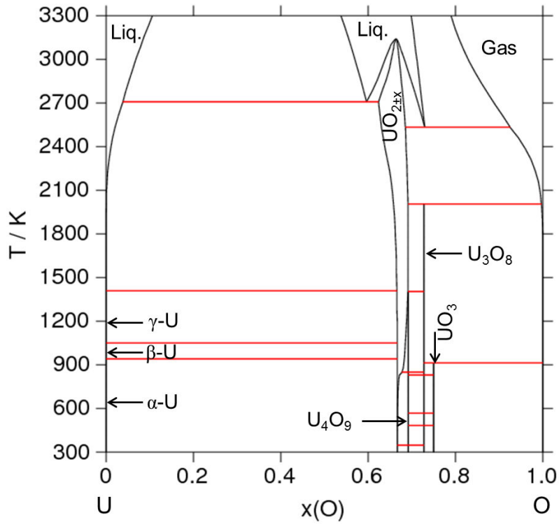
Figure 9: U-O phase diagram by Guéneau et al. [9]
