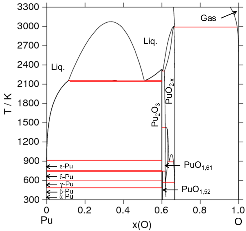
Figure 8: Pu-O phase diagram by Guéneau et al. [9]
