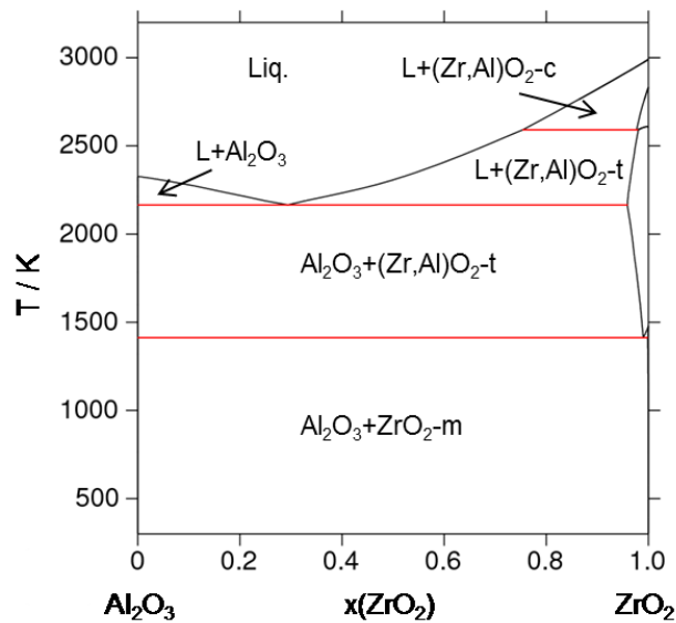
Figure 12: Calculated Al_2O_3 - ZrO_2 phase diagram [6]
