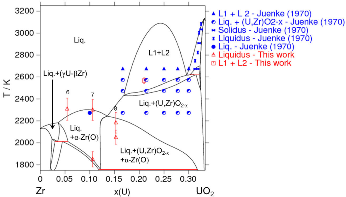
Figure 7: Calculated Zr- \text{UO}_2 isopleth section. The reported experimental data are from Juenke & White [14]. The L1+L2 reported for this work is referred to the heat treatment result obtained on sample OUZr_3
