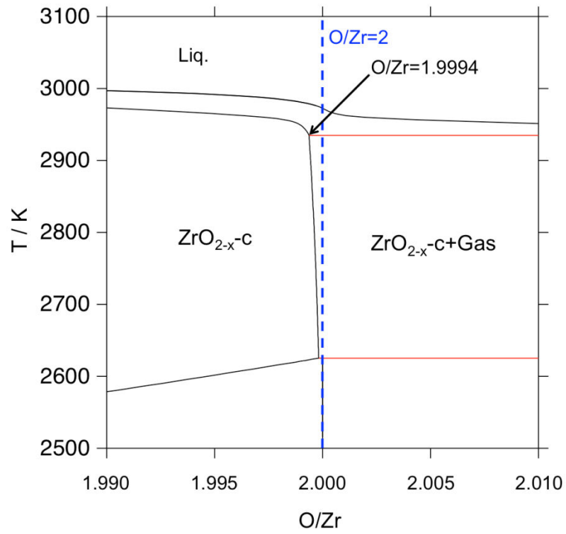
Figure 11: High temperature Zr-O phase diagram centred on O/Zr=2
