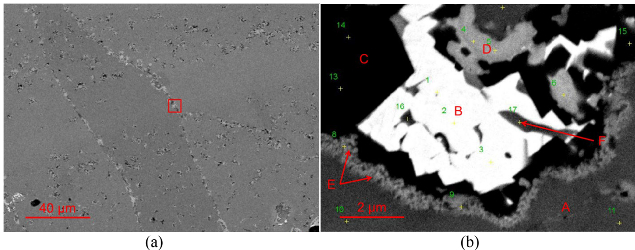
Figure 28: (a) BSE image of the solidified oxide Liquid 2; (b) close up on the white precipitates along the mixed oxide (U,Zr)O 2-x grain boundaries. Six phase are identified and analysed by WDS (A-F in the figure)
