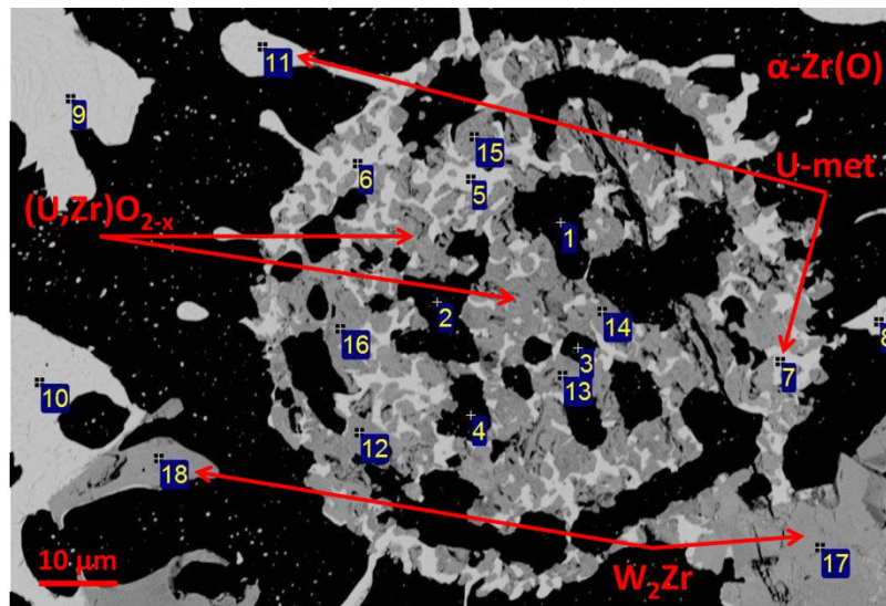
Figure 15: Oxide droplet solidified within the quenched metallic liquid. The EDS results on the reported spectra (1-18) are presented in Table 9.
