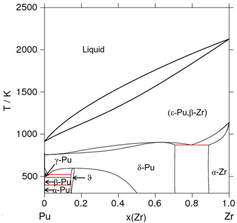
Figure 5 Pu-Zr phase diagram by Kurata [5]
