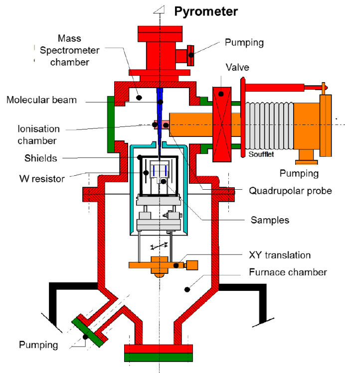
Figure 3: Scheme of the furnace employed for the heat treatments
