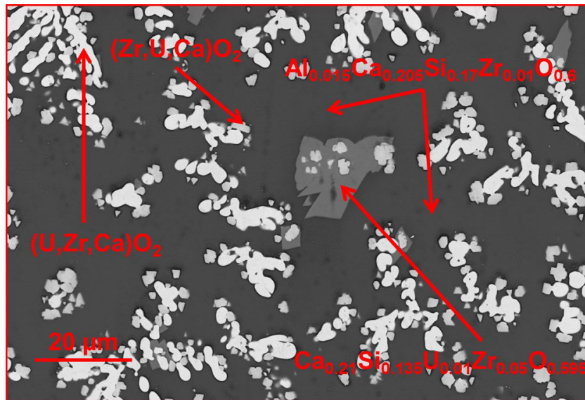
Figure 3: Larger view of the red square in Figure 2b. Three phases are identified: dendrites of (U,Zr,Ca)O_2 , the light grey phase is a mixture (Ca,Si,Zr,\epsilon U,O) and the dark grey phase is a mixture of (Ca,Si,\epsilon Al,\epsilon Zr,O) , probably a quenched liquid
