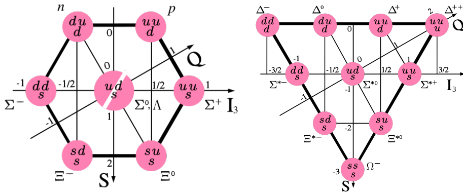
Figure 1.2: Left: the J^P = 1/2^+ baryon octet. Right: the J^P = 3/2^+ baryon decuplet, showing the S = -3 baryon \Omega^- at the bottom of the decuplet.
