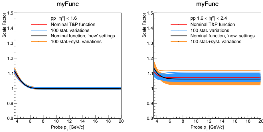
Figure 6.15: 100 variations of the \varepsilon^{data} part of C^{TNP} ( pp collisions), using alternate tag-probe settings (orange) and using standard settings (blue). The blue curves make up for a statistical uncertainty of the procedure, while orange curves take also a systematic uncertainty into account.
