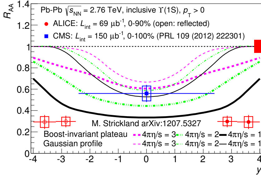
Figure 7.10: PbPb nuclear modification factor R_{AA} in PbPb collisions at \sqrt{s_{NN}} = 2.76 TeV, as a function of Y rapidity, taken from [5]. Data from CMS publication using 2010 pp data [4] and ALICE [5]. The data is plotted against a potential model for quarkonium suppression described in [142].
