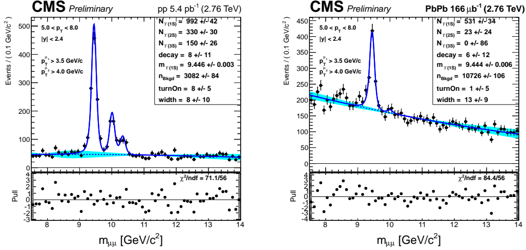
Figure A.3: Same as Figure A.1 in the bin p_T [GeV/c] ∈ [5 – 8].
