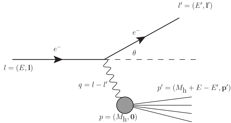
Figure 1.3: Deep inelastic e^-p scattering. A photon is exchanged and a hadronic final state X is formed.
