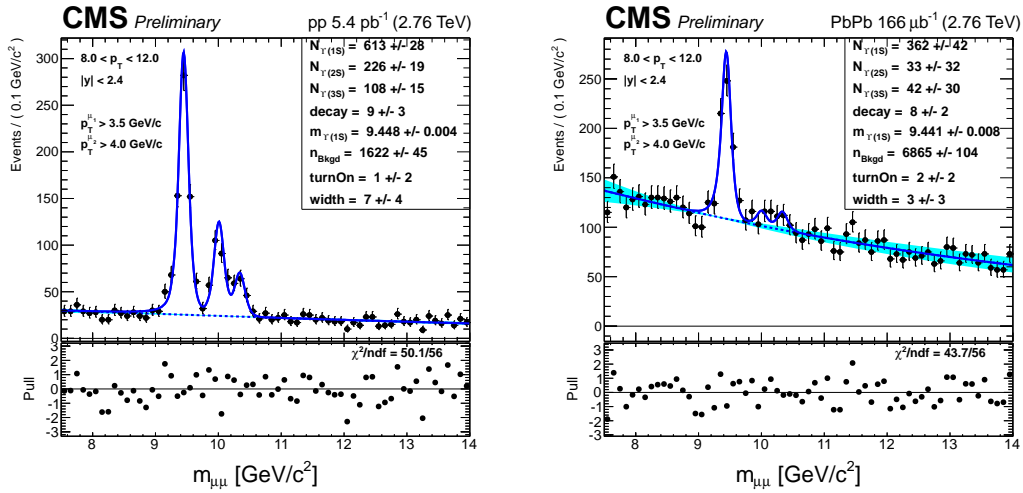
Figure A.4: Same as Figure A.1 in the bin p_T [GeV/c] ∈ [8 – 12].
