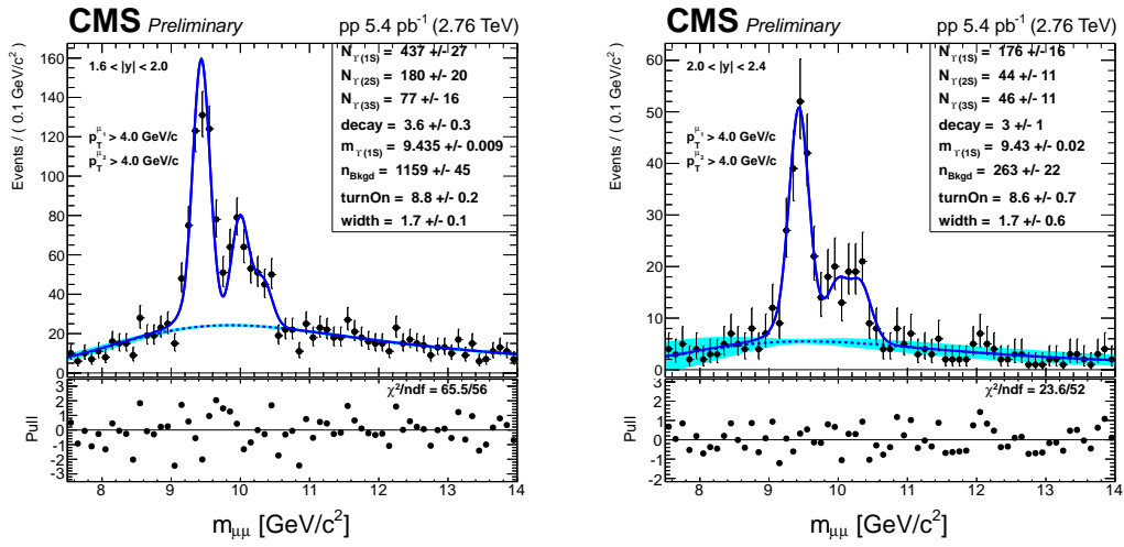
Figure A.23: Fits to the pp dataset with the tight muon p_T cut applied, for the extraction of the pp \Upsilon(2S) and \Upsilon(3S) cross sections in fine bins of rapidity. Left: y \in [1.6-2.0] . Right: y \in [2.0-2.4] .
