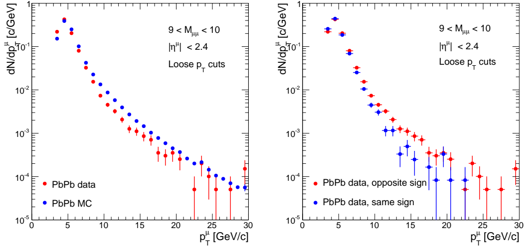
Figure 6.5: Single muon p_T distributions. Muons come from dimuon pairs in the mass region of the \Upsilon , 9 < M < 10 \text{ GeV}/c^2 . In both panels, red symbols represent the muon p_T distribution in PbPb collisions. On the left panel, muons from generated \Upsilon are in blue. On the right, muons from same-charge pairs are in blue.
