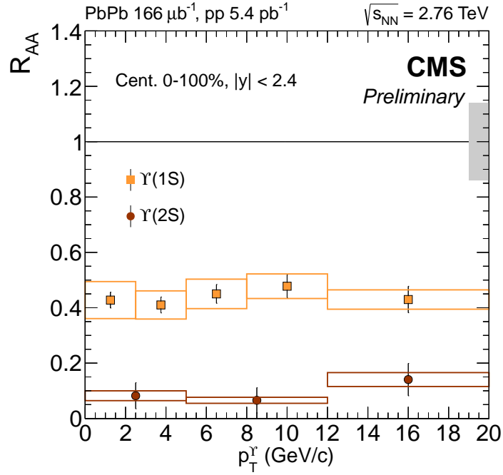
Figure 7.6: PbPb nuclear modification factor of \Upsilon(1\text{S}) and \Upsilon(2\text{S}) in PbPb collisions at \sqrt{s_{\text{NN}}} = 2.76 \text{ TeV} , as a function of the \Upsilon transverse momentum. The gray error bar at unity is the global systematic uncertainty due to pp tracking efficiency and luminosity.
