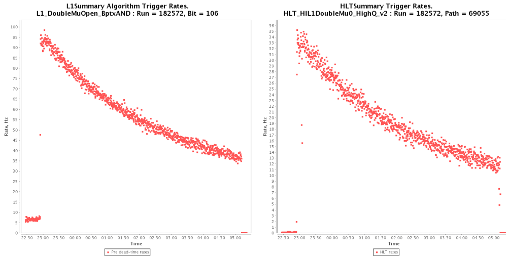
Figure 4.2: Rates of the open dimuon trigger in the 2011 PbPb run. Left: rate of L1_DoubleMuOpen_BptxAND ; Right: rate of HLT_HIL1_DoubleMu0_HighQ .
