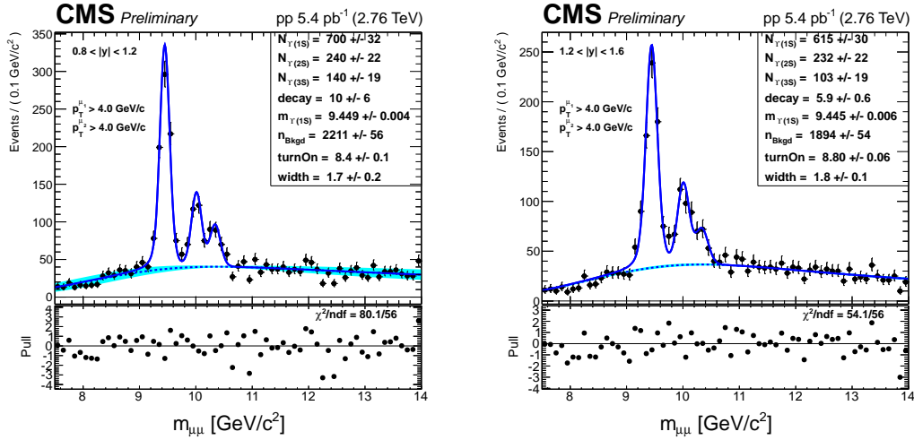
Figure A.22: Fits to the pp dataset with the tight muon p_T cut applied, for the extraction of the pp \Upsilon(2S) and \Upsilon(3S) cross sections in fine bins of rapidity. Left: y \in [0.8, 1.2] . Right: y \in [1.2, 1.6] .
