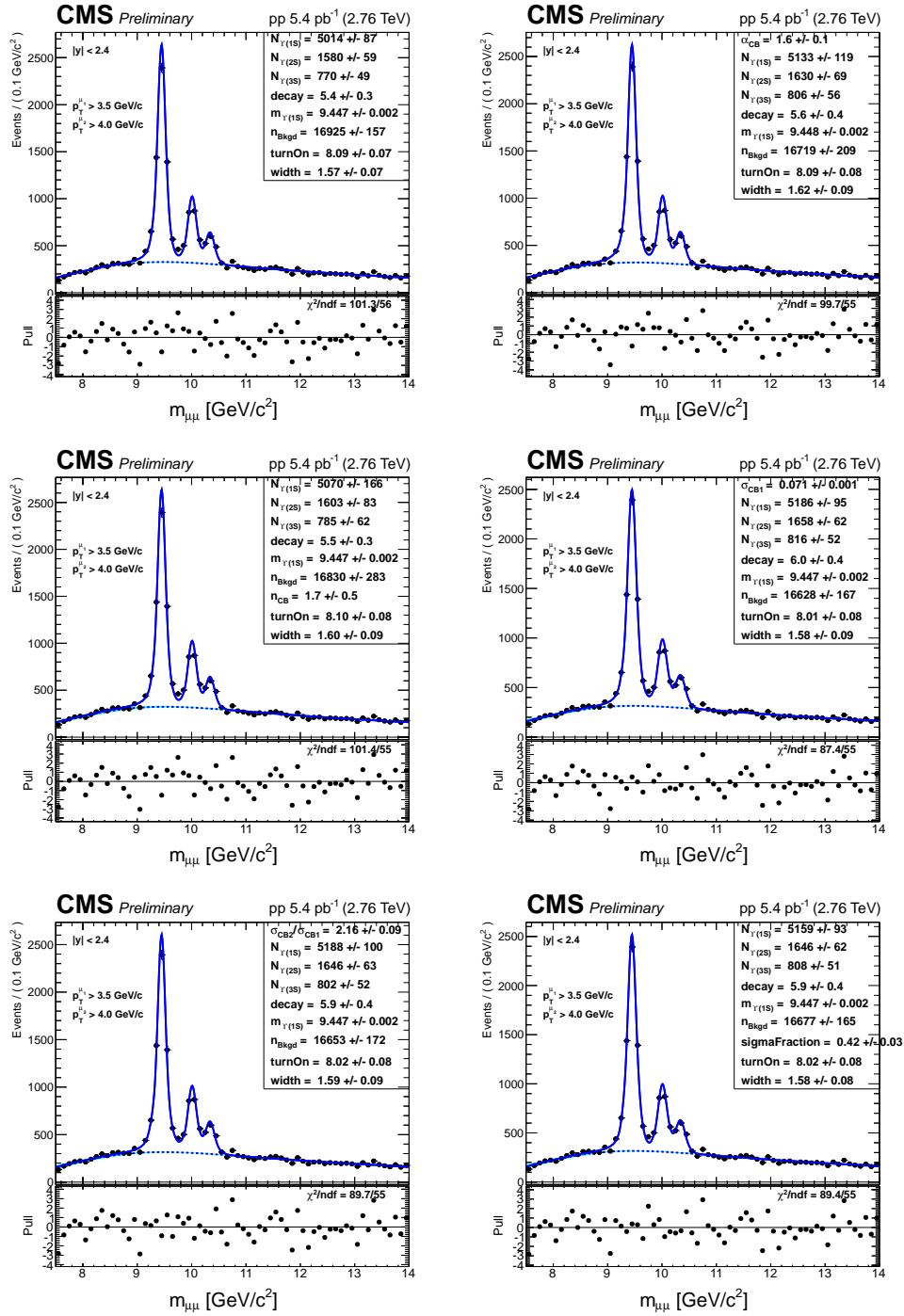
Figure A.27: Fit Variations of the all-integrated pp data, cases where the signal shape was varied.
