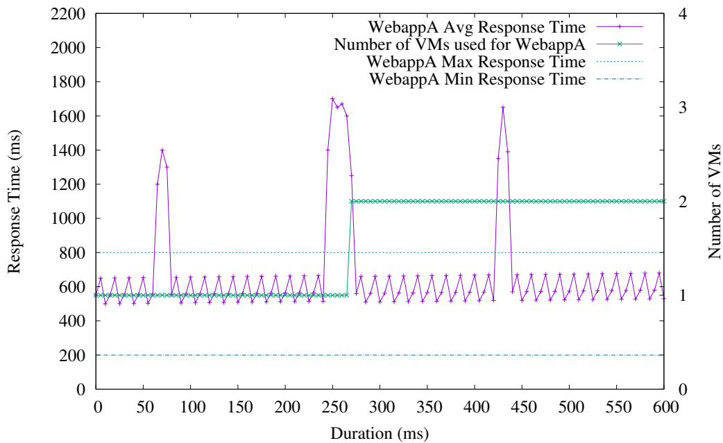
Figure 7.6: Autonomous responses with fluctuation of average response time of WebappA using MFS algorithm
