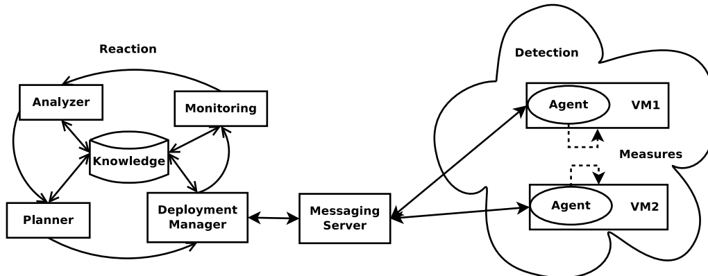
Figure 6.6: Roboconf autonomic loop for elasticity
