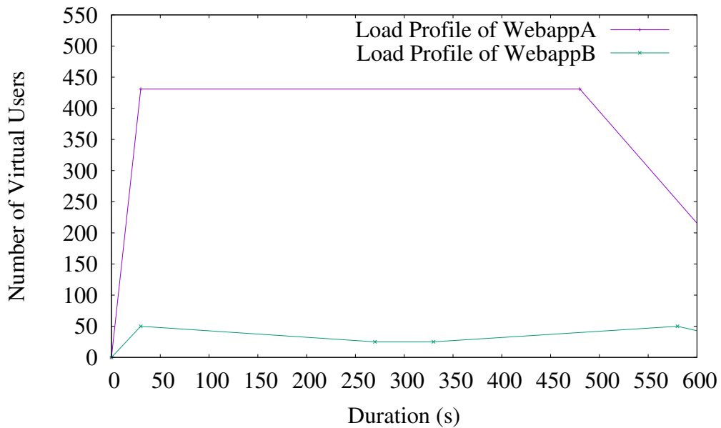
Figure 7.2: CLIF load profiles of the WebappA and WebappB
