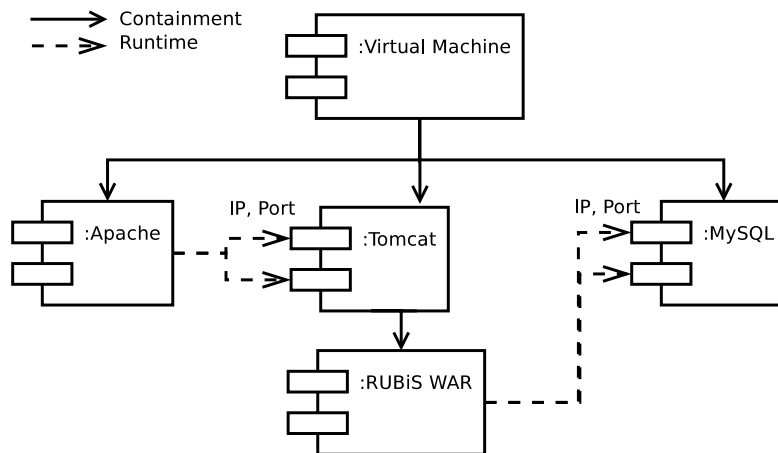
Figure 5.2: Illustration of a fine-grained description of components
