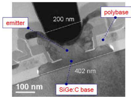
FIGURE 1.26: SEM SiGe BiCMOS9MW / Performances [37, 38]
