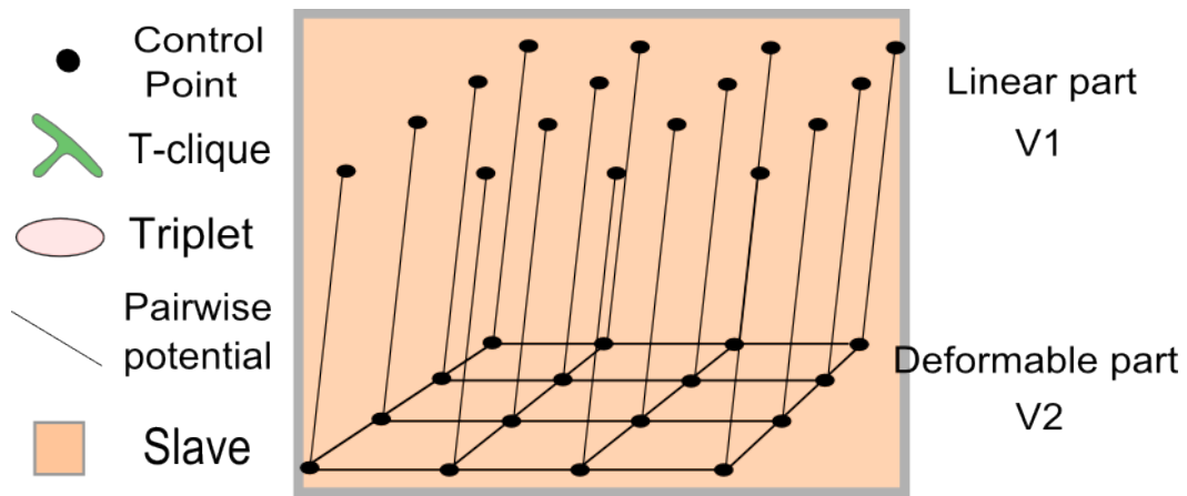
Figure 4.5: The deformable slave contains all the pairwise potentials of the graph. We send a message from the nodes only linked by an edge (containing the data term), then we can solve the problem using Fast-PD because the other pairwise, the smoothing term, is submodular.
