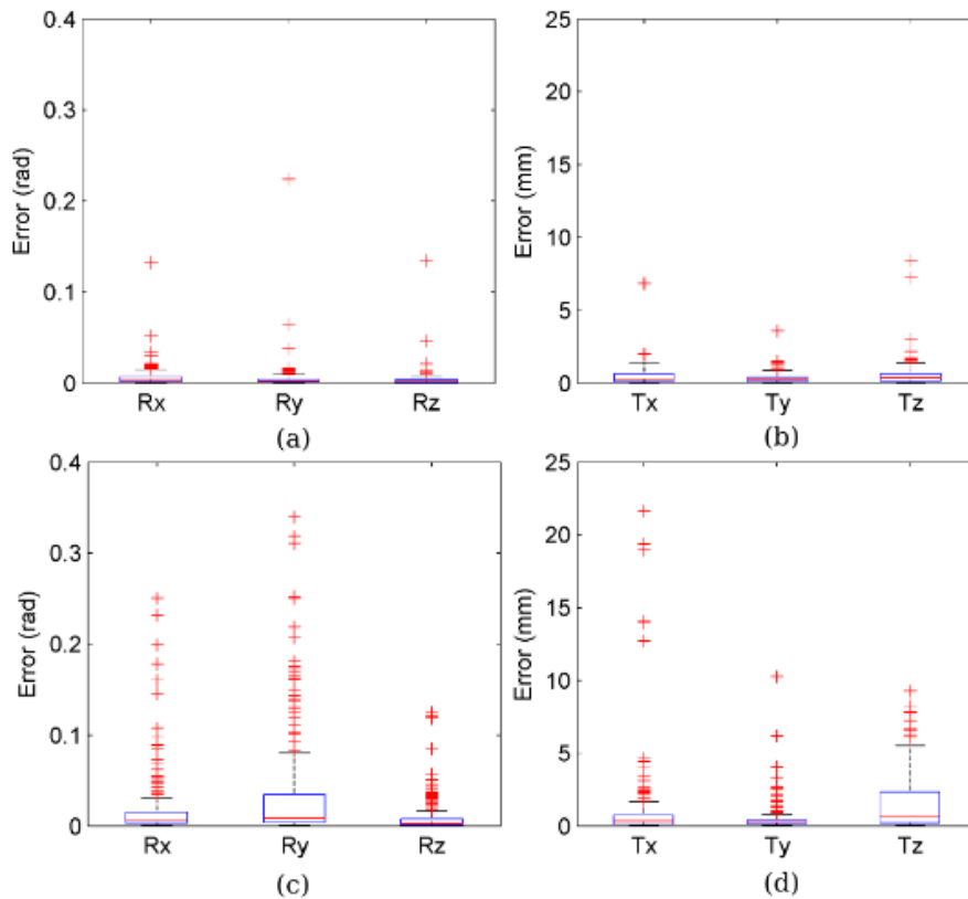
Figure 5.2: (a) and (b) Error estimation of the plane parameters for the method described here. (c) and (d) Error estimation for the method presented in [37] for the same dataset with equivalent setup.
