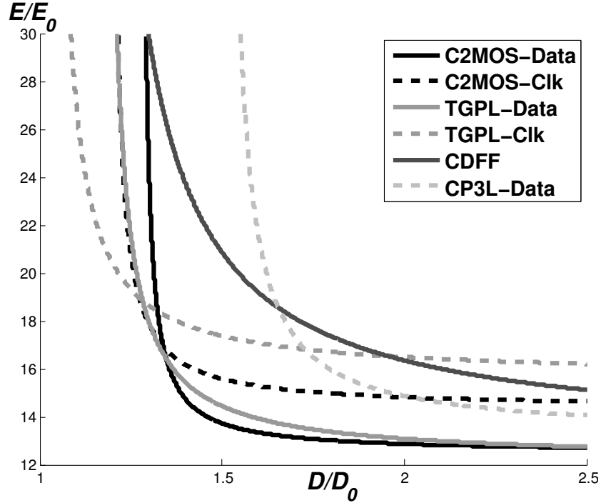
Figure D.11: CEE: V_{dd} = 1.0V , V_{dds}=G_{nds}=0V , \alpha_{sw} = 0.15 , T_{clk} = 40FO4 , corner TT, température 70^\circ C .
