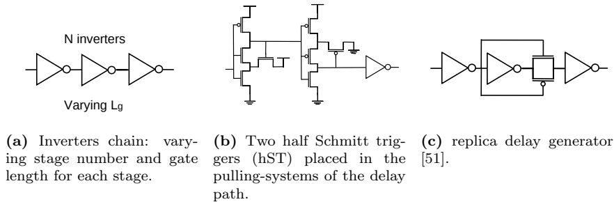
Figure 3.6: Delay generator architectures used for the comparison.
