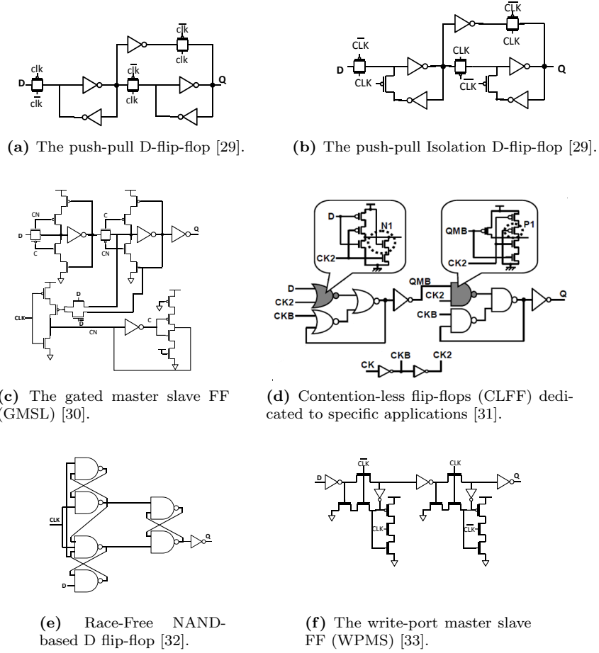
Figure 1.7: Novel master-slave architectures proposed in the literature.
