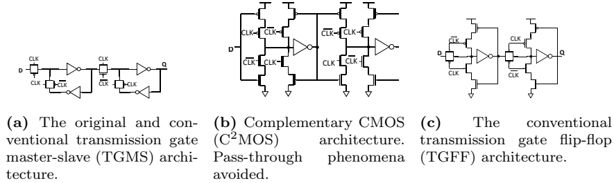
Figure 1.6: Conventional master-slave architectures. TGFF gives the best tradeoff between speed performances and pass-through phenomena.
