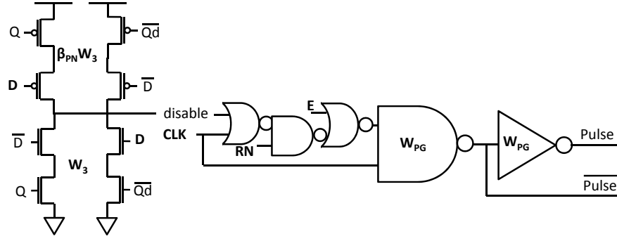
(a) The conditional pulse generator (current-starved circuitry not shown for clarity).
