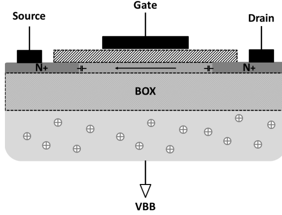
Figure 1.4: FDSOI transistor (NMOS version).
