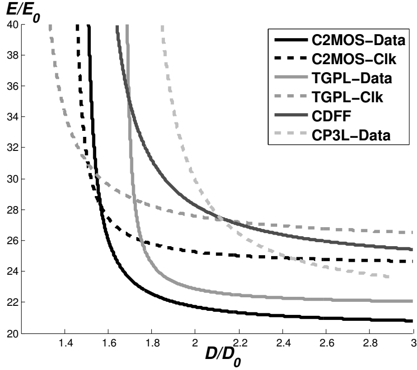
Figure D.12: CEE: V_{dd} = 0.35V , V_{dds}=G_{nds}=0V , \alpha_{sw} = 0.15 , T_{clk} = 40FO4 , corner TT, température 25^{\circ}C .
