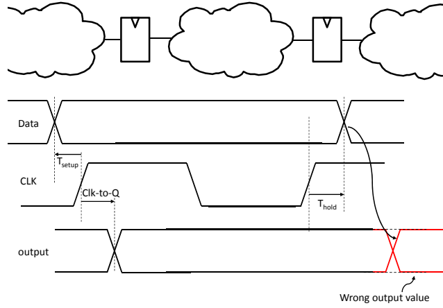
Figure 1.5: The flip-flop principle and its figures of merit.
