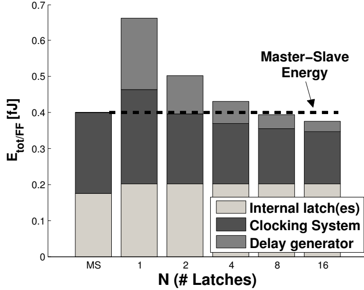
Figure 4.6: The energy per FF with the number of latches sharing a PG. Bars represent the proportions of the energy consumed in the delay generator, the clocked part ( CLK and Pulse signals), and the latch alone. V_{dd}=1V , minimum driving strength (X1), T_{clk} = 40FO4 , \alpha_{sw} = 15\% .
