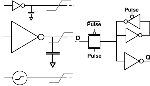
Figure 2.1: Three different configurations providing identical input slopes when the transmission gate is closed.
