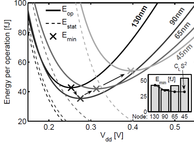
Figure 1.3: Minimum energy point increases with further technological node because of the higher variability [2].
