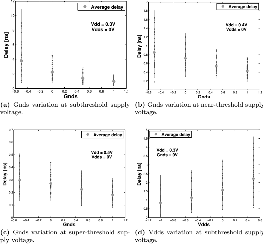
Figure 2.18: Evolution of measured delays with VDDs and GNDS.
