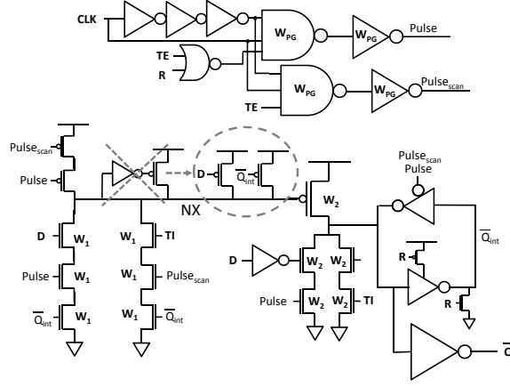
Figure A.1: Two-stages single-edge CDFF.
