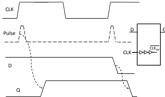
Figure 1.12: The pulse-triggered flip-flop principle. During the pulse period, the flip-flop behaves essentially like a level-sensitive latch.
