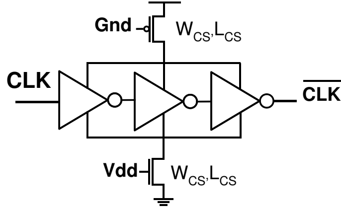
Figure 3.2: Proposed current starved (CS) delay generator architecture [70].
