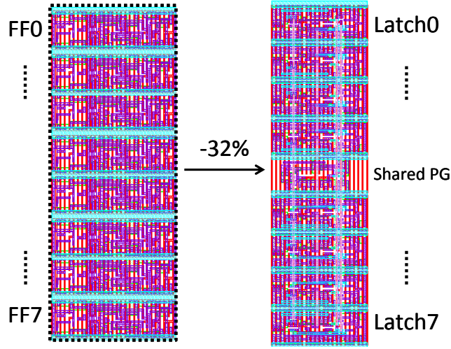
Figure 4.7: Pulse-triggered FF architecture shows a lower area per FF than master-slave. The block of 8 pulsed-FF (right) has 32% less area than 8 MS FFs, at the expense of the M3 layer utilization.
