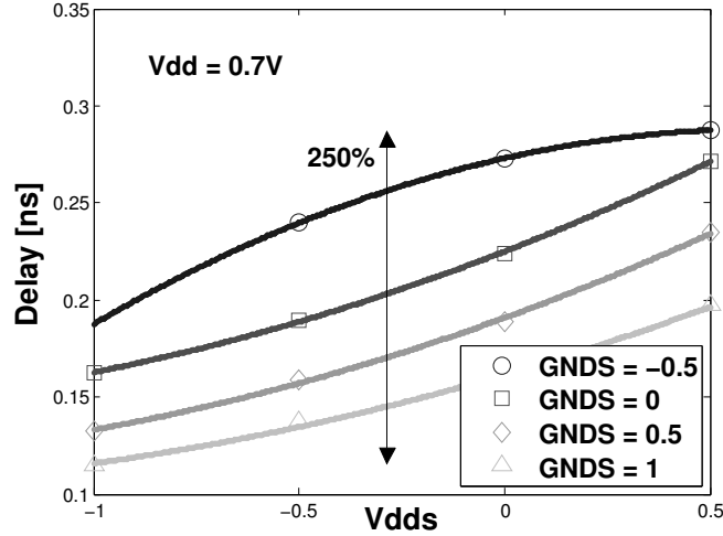
Figure 2.17: Vdds variation and GNDS at intermediate supply voltage. A variation of 250% is achieved with the back biasing.
