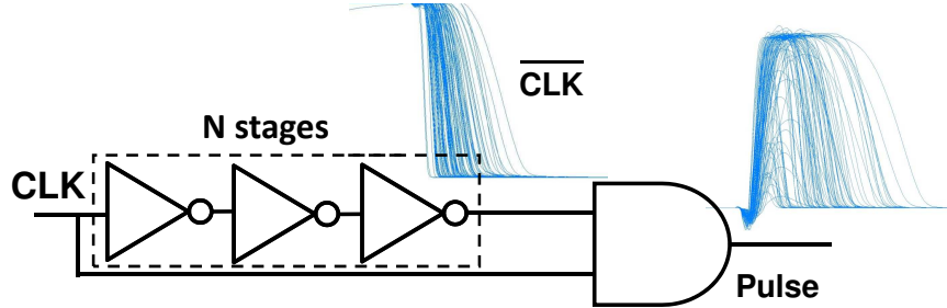
(a) Variability issues in ultra-low-voltage pulse generator.
