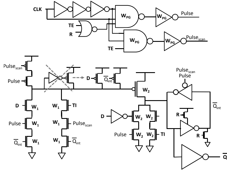
Figure 2.8: Scannable and resettable version of the two-stages single-edge CDFD from figure 1.17d
