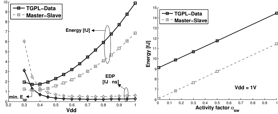
(a) Evolution of the average energy per cycle ( \alpha_{sw} = 15\% ) and the EDP with the supply voltage. (b) Evolution of the average energy per cycle with the data switching activity factor.
