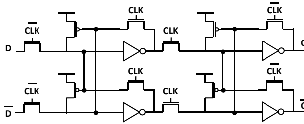
Figure 1.9: Improved MS-based differential structure [34].
