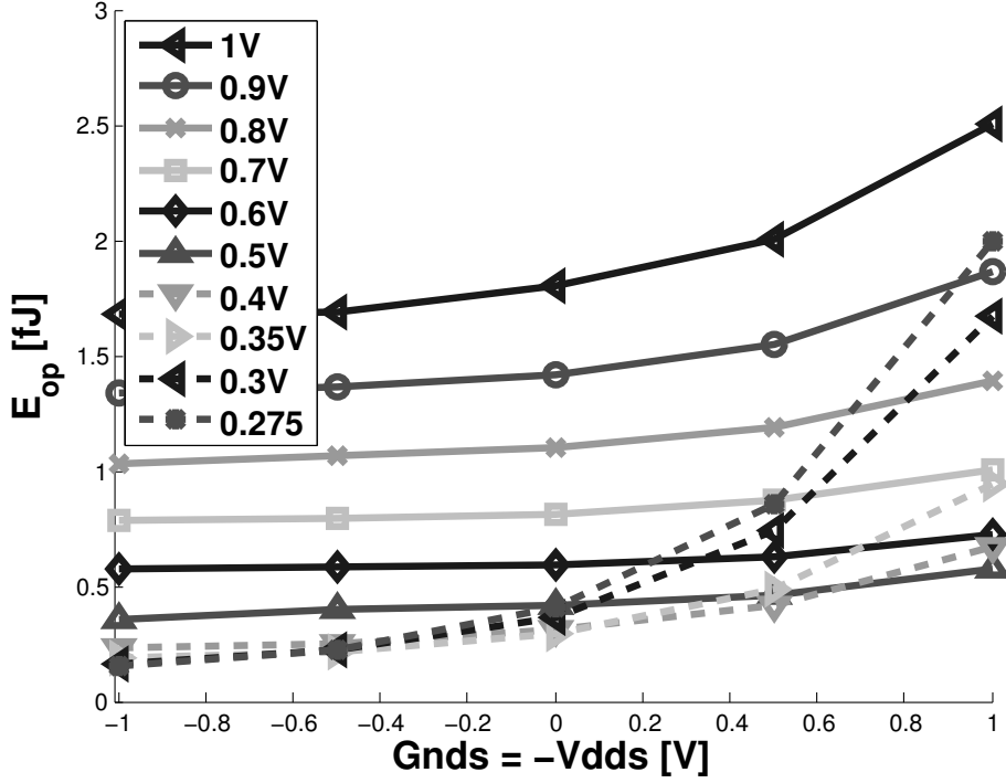
Figure 4.10: Energy per operation function of the supply voltage and the back biasing ( \alpha_{rate} = 15\% , T_{clk} = 40FO4 , corner TT, temp. = 25^\circ\text{C} ).
