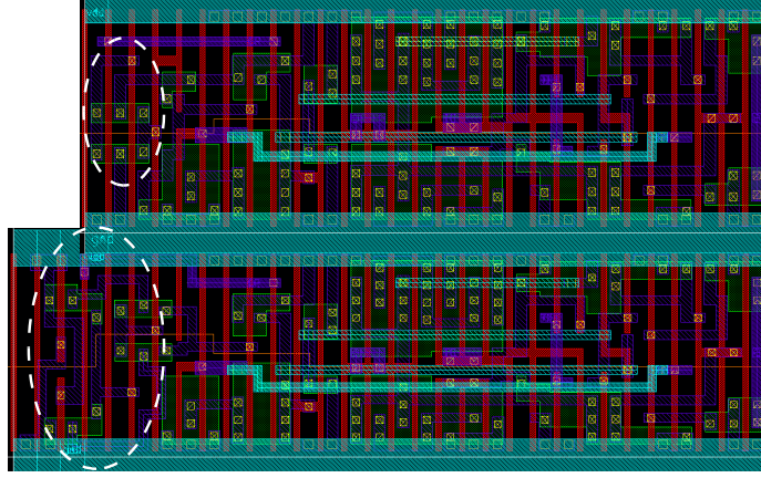
Figure 3.9: Layout of TGPL-Data (minimum EDP and driving strength) with the conventional DG (above) and the current-starved-like DG (below). An overhead of three fingers is paid for an impressive increase of robustness.
