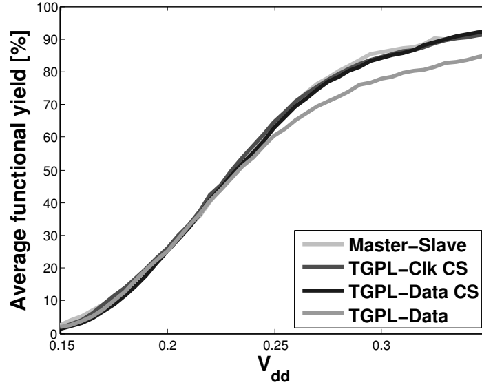
Figure 3.15: Yield average over the whole (vdds,gnds) space. The explicit pulsed-FFs presents, now, the same robustness as Master-Slave topology.
