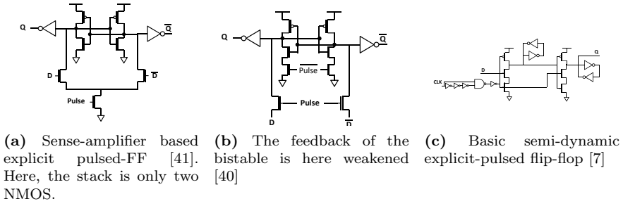
Figure 1.16: Differential and semi-dynamic architectures of explicit pulsed-FF.
