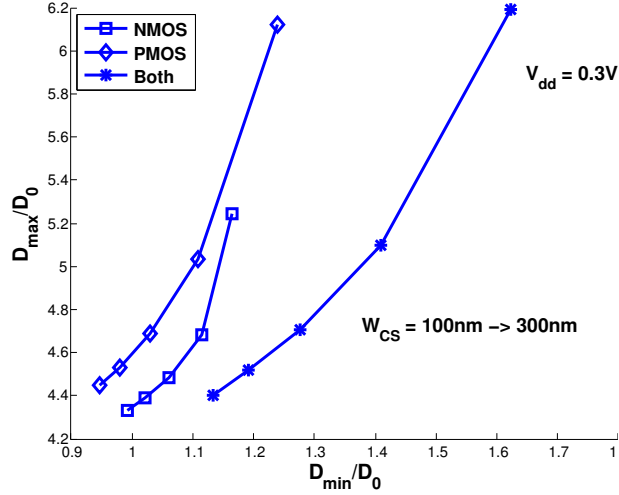
Figure 3.5: Minimum and maximum delays ( T_{del, \pm 3\sigma} ) and energy consumption function of the size of the current-starving transistor(s). NMOS-only exhibits a lower timing variability than PMOS-only.
