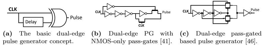
Figure 1.19: Dual-edge pulse generators.
