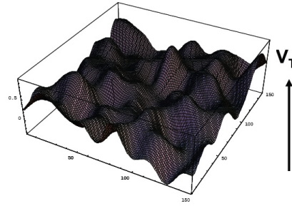
Figure 1.2: Discrete threshold voltage distribution in the transistor channel [13].
