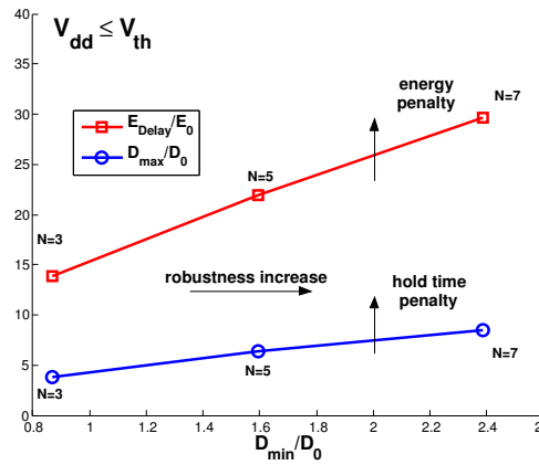
(b) The energy dissipation and the maximum delay ( \mu + 3\sigma ) versus the minimum delay ( \mu - 3\sigma ) of an inverters chain ( N = 3, 5 and 7 )
