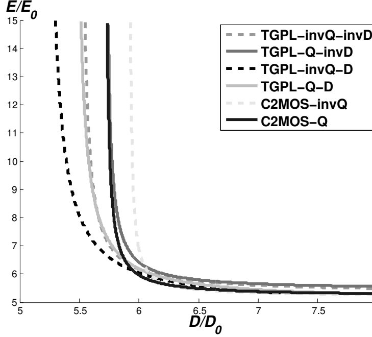
Figure 4.4: Energy-Delay with several different XOR ( V_{dd} = 1V , driving strength X1, \alpha_{sw} = 0.15 , T_{clk} = 40FO4 , temperature 70^\circ C ).
