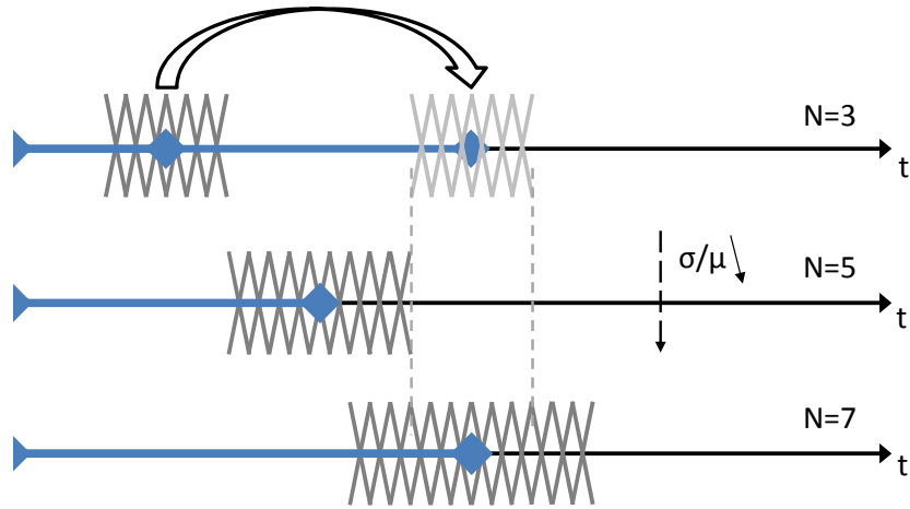
Figure 3.3: The current-starved delay generator architecture provides a translation without expansion of the delay window in the time line. In other words, it increases the average delay without noticeably increasing the dispersion.
