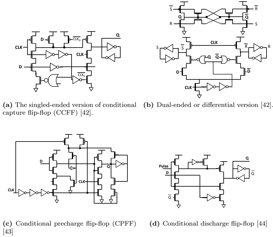
Figure 1.17: Other conditional techniques.
