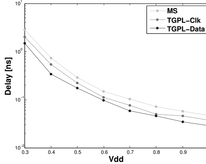
Figure 2.16: Measured delays from 0.3V to 1V in nominal case ( V_{DDS}=G_{NDS}=0V ). Clk-to-Q delay is lower for TGPL-Data than for TGPL-Clk, contrary to the D-to-Q delay ( T^\circ = 80^\circ C ).
