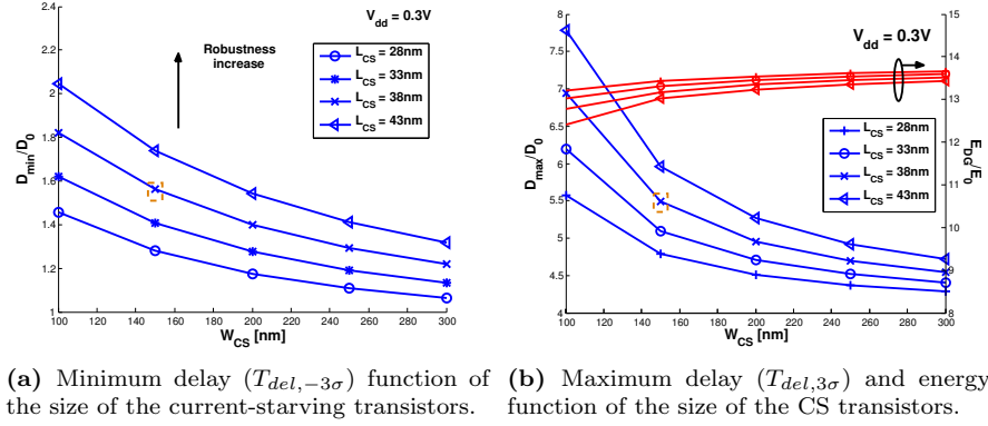
Figure 3.4: Impact of sizing on the delay generators figures of merit.
