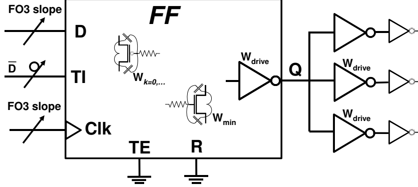
Figure B.1: Testbench used to characterize FFs with layout parasitics included.
