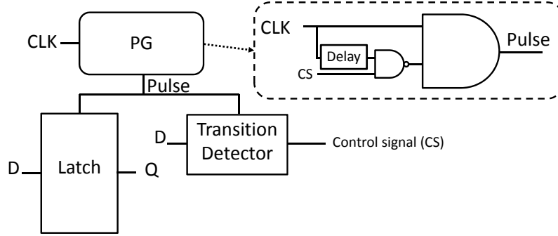
Figure 1.22: Example of implementation of the time-borrowing technique in explicit pulse-triggered flip-flop.
