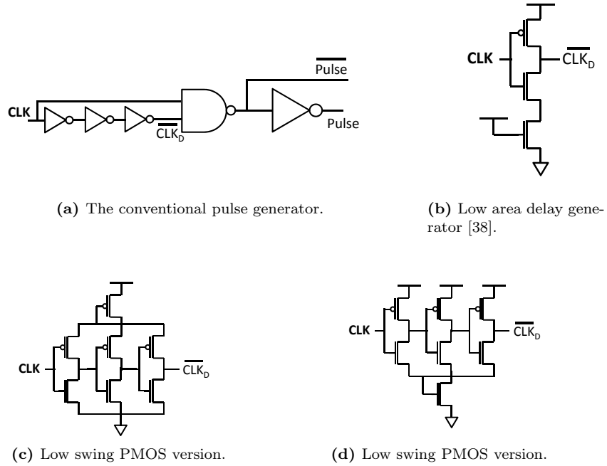
Figure 1.14: Pulse generators dedicated for pulsed-FFs in the state of the art. In 1.14c and 1.14d, transistors in diode mode lead to a lower swing, thus energy consumption, in the delay generator [39].
