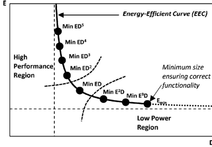
Figure 2.10: Extraction of energy-efficient curve (EEC) [67]: from the corresponding energy consumptions ( E ) and propagation delays ( D ) of the design points given by the W_k , we plot them in the E - D space and interpolate those points by a hyperbole.
