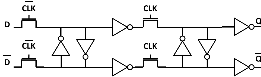
Figure 1.8: The differential flip-flop principle (master-slave-based).
