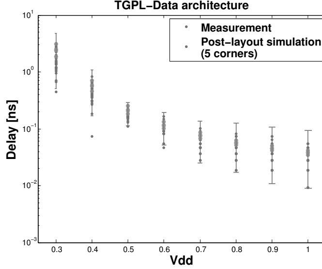
Figure 2.15: Measured delays of TGPL-Data from 0.3V to 1V with the expected 3\sigma range computed from 63 chips ( V_{DDS}=G_{NDS}=0V ). Gray dots are the results of post-layout simulations in the five process corners ( T^\circ = 80^\circ C ).
