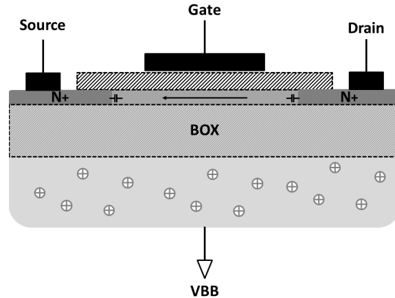
Figure D.1: Le transistor FDSOI (version NMOS).
