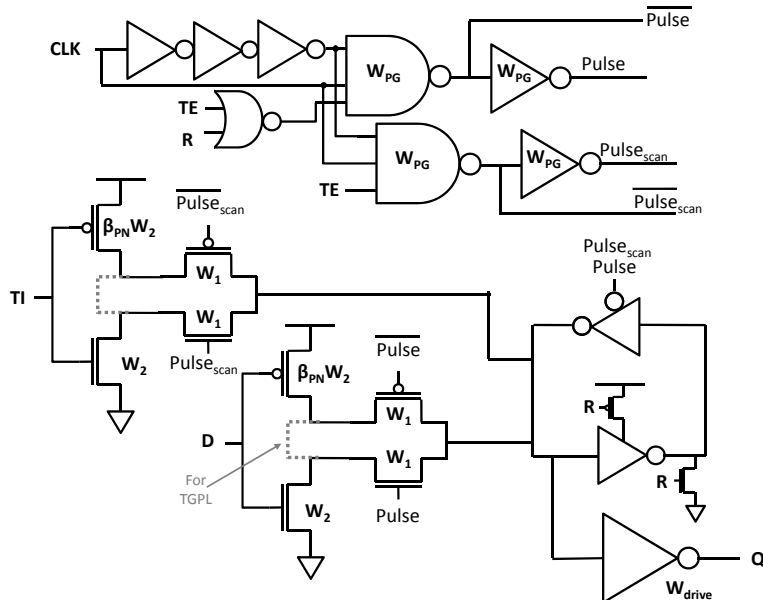
Figure 2.7: One-stage TGPL-Clk and C 2 MOS-Clk (respectively with and without the dotted wire) FF.s, two variants of the TGPL architecture from figure 1.15.
