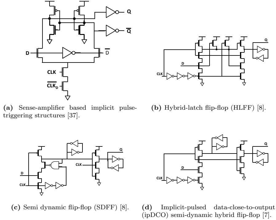
Figure 1.13: Differential and semi-dynamic implicit pulse-triggered flip-flops.
