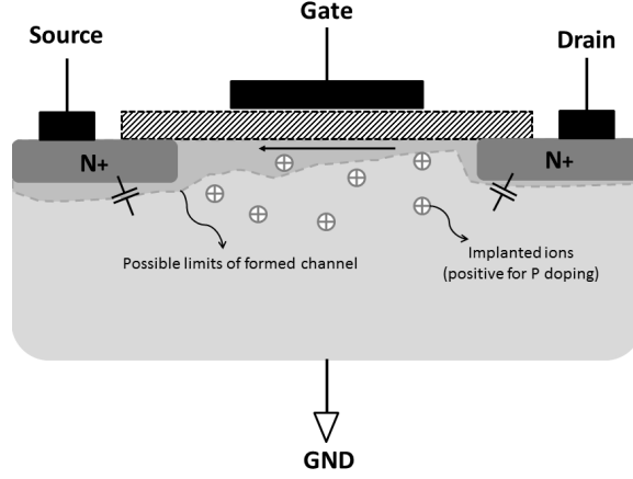
Figure 1.1: Conventional Bulk transistor (NMOS).
