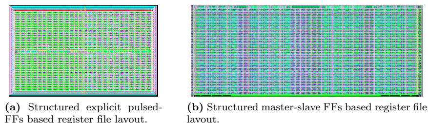
Figure 4.8: Layout comparison led to a 14% saving in area.
