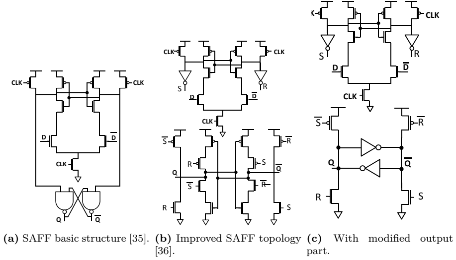
Figure 1.10: Differential sense-amplifier based flip-flops.
