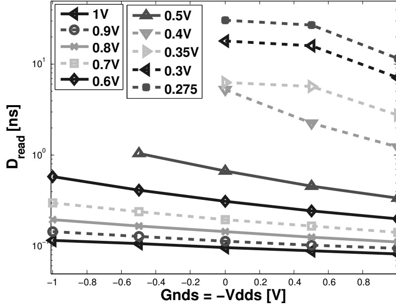
Figure 4.11: Evolution of the register file delay with back biasing.
