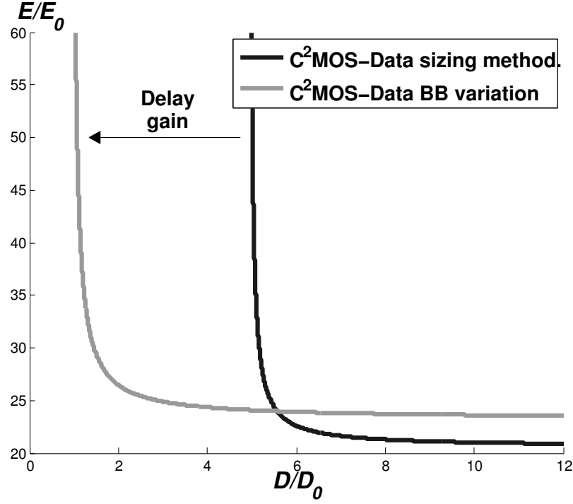
Figure 2.14: EECs of the C 2 MOS-Data architecture extracted from the sizing methodology and from a applied back biasing ( V_{dd} = 0.35V , driving strength X1, \alpha_{sw} = 0.15 , T_{clk} = 40FO4 , temperature 25^{\circ}C ).
