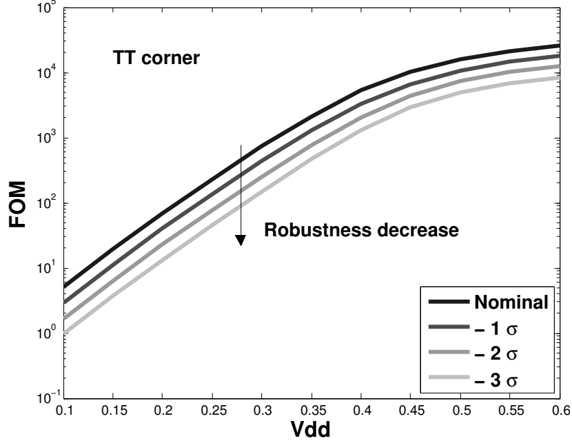
Figure 3.12: At ULV, the degradation of the FOM ( \frac{I_{on}}{I_{off}} ratio) leads to a degraded output logic level.
