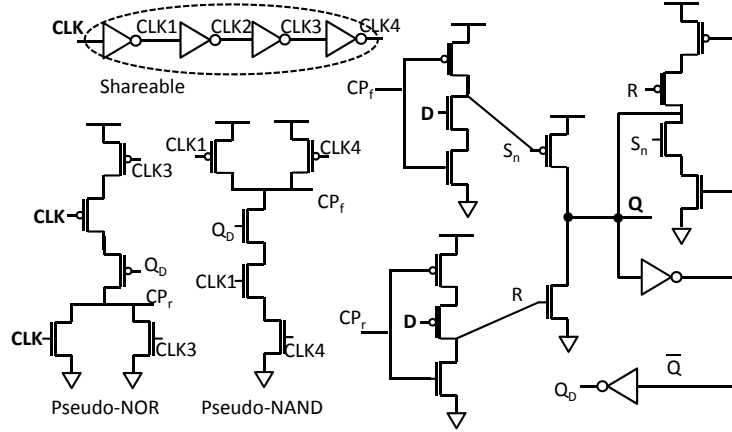
Figure 1.21: Conditional push-pull pulsed latch ( CP^3L ) [49]. The lowest EDP of the literature.
