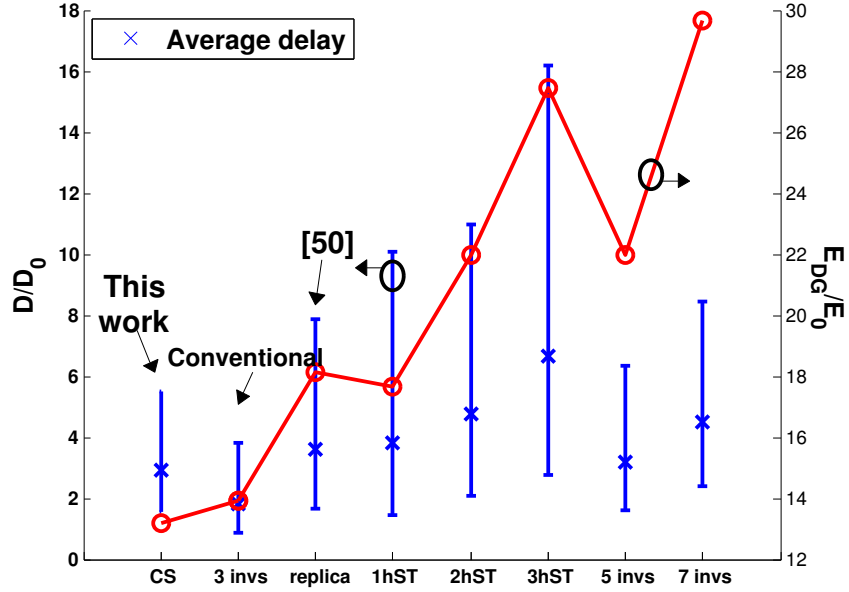
Figure 3.8: Comparison of energy and delay performances in subthreshold regime ( V_{dd} = 0.3V ) for different DG architectures.
