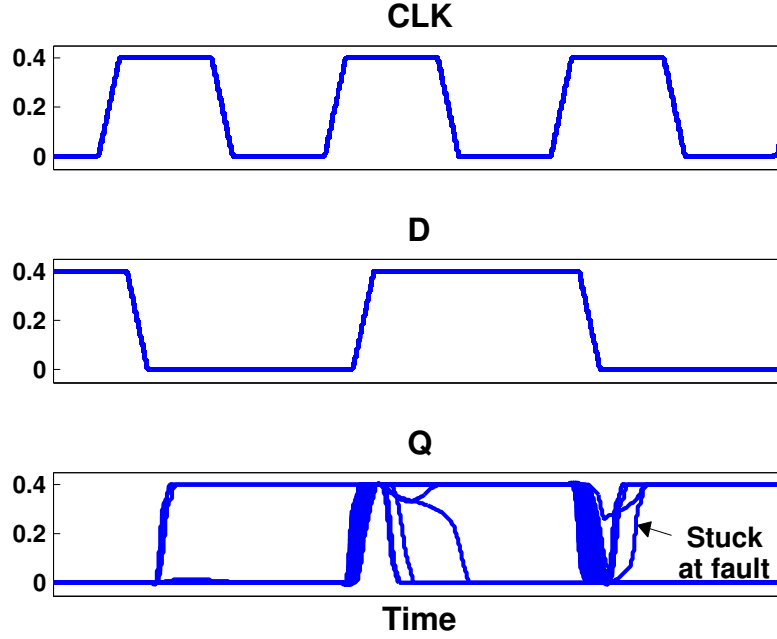
Figure A.3: Monte-Carlo simulations exhibit the weak robustness of ACPL architecture to transistor variability (corner FS, temp. = 25°C, V_{dd} = 0.4V).
