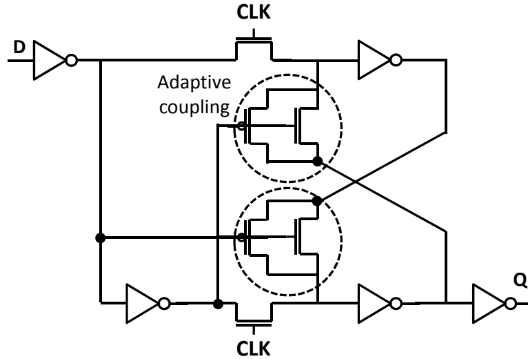
Figure A.2: As a reminder, the pulse-triggered version of the ACFF, the adaptive coupling pulse latch (ACPL). Even the basic architecture without additional functionalities is not functional at ultra-low-voltage.
