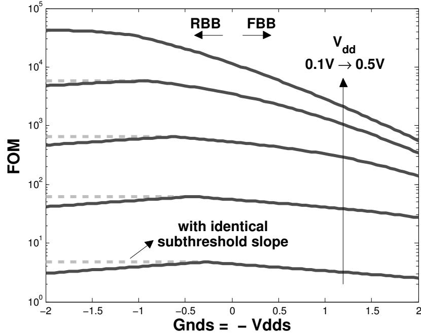
Figure 3.14: Strong FBB increases the speed but decreases the robustness. In 28nm FDSOI technology, the non-identical subthreshold slopes cause a robustness decrease also for RBB.
