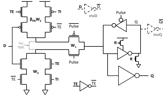
(b) The C 2 MOS-XOR latch with additional inverters for \bar{D} and \bar{Q_d} signals.
