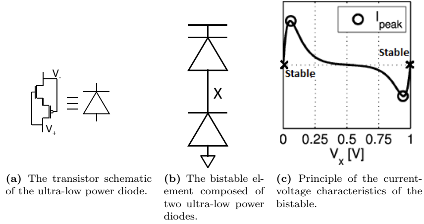
Figure 2.2: Ultra-low power static bistable element [59].
