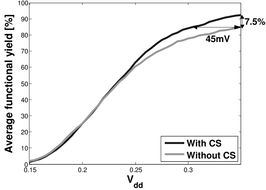
Figure 3.16: The current-starved (CS) delay generator provides a notable gain for the yield.
