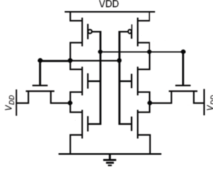
Figure 2.3: The half Schmitt trigger bistable [61].
