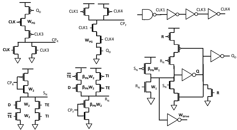
Figure 2.9: CP 3 L-Data, scannable and resettable version of the two-stages negative-edge triggered CP 3 L from figure 1.21.
