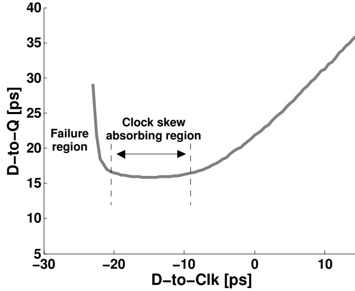
Figure 4.1: Timing regions and characteristics for TGPL flip-flop (nominal voltage).
