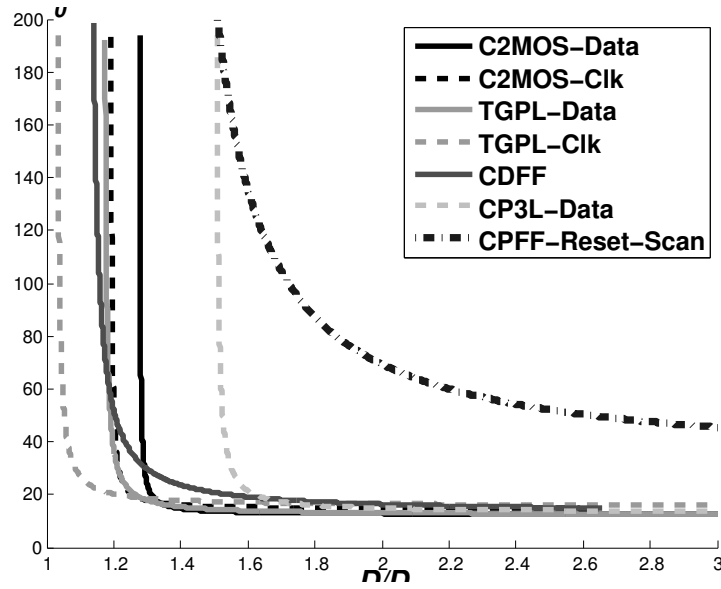
Figure A.5: EECs with CPFF architecture (driving strength X1, V_{dd} = 1.0V ; \alpha_{sw} = 0.15 , T_{clk}/FO4 = 40 , corner TT, temperature 70^\circ ). Additional transistors lead to a very poor E - D performances.
