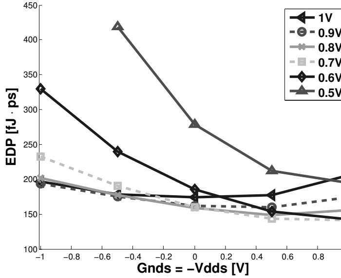
Figure 4.12: Evolution energy-delay product (EDP) with V_{dd} and back bias.
