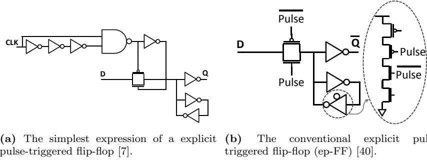
Figure 1.15: The basic structures of explicit pulse-triggered flip-flop.
