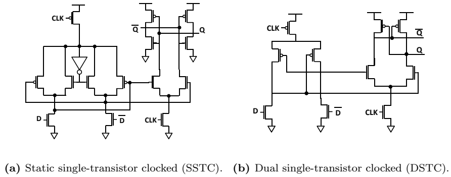
Figure 1.11: Differential master-slave flip-flops [35].
