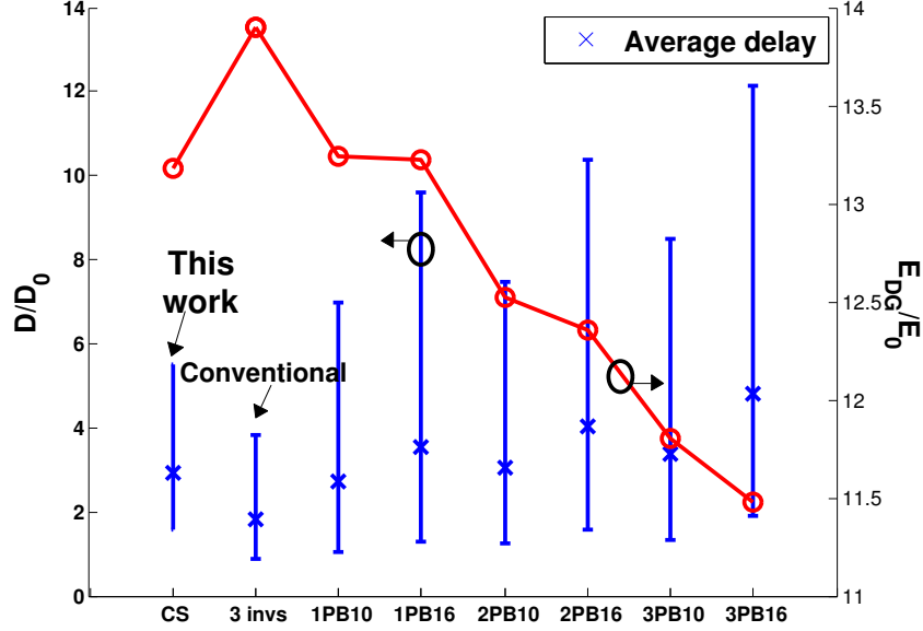
Figure 3.7: Comparison of energy and delay performances in subthreshold regime ( V_{dd} = 0.3V ). The name indicates the poly bias and the number of stages getting this PB.
