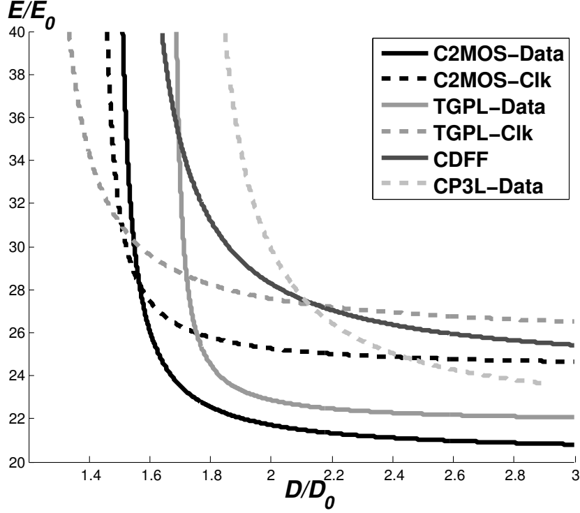
Figure 2.12: EEC: V_{dd} = 0.35V , v_{dds}=gnds=0V , \alpha_{sw} = 0.15 , T_{clk} = 40FO4 , corner TT, temperature 25^\circ C .
