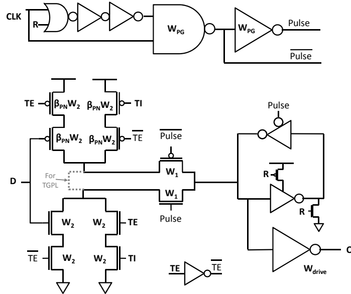
Figure 2.6: One-stage TGPL-Data and C 2 MOS-Data (with and without the dotted wire, respectively) FFs, two variants of the TGPL architecture from figure 1.15.
