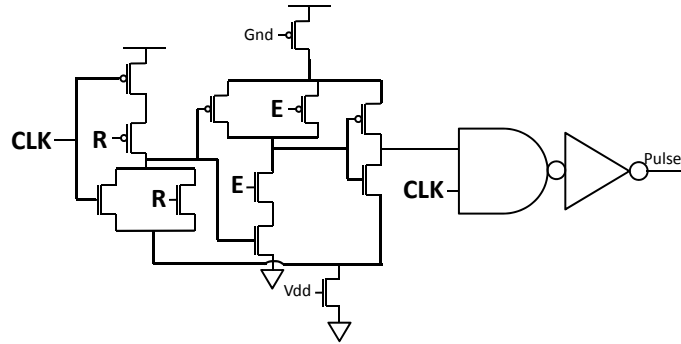
Figure 3.18: (Re)Set and Enable current-starved pulse generator.
