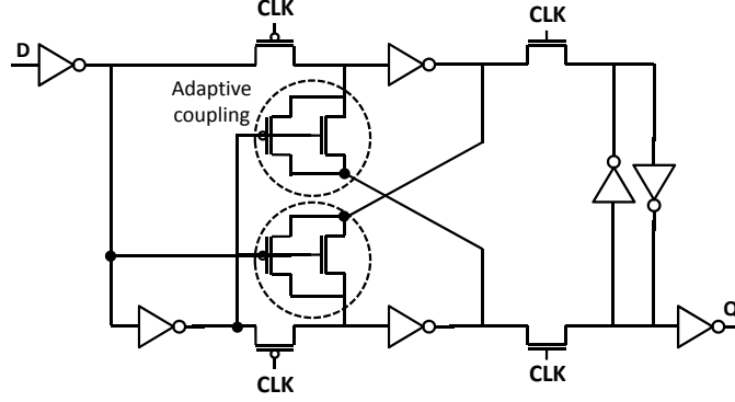
Figure 1.20: Adaptive-coupling flip-flop [48]. Thanks to the elementary clock load, this architecture exhibits the lowest energy consumption among the flip-flop literature.
