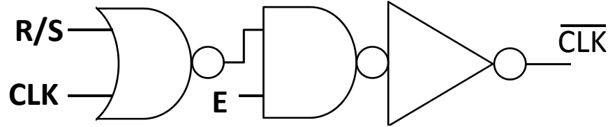
Figure 3.17: (Re)Set and Enable functionalities are easily implemented in the pulse generator.
