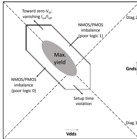
Figure 3.11: Schematic behaviour of the yield in the vdds-gnds space.
