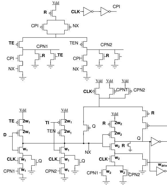
Figure A.4: R-S CPFF architecture.
