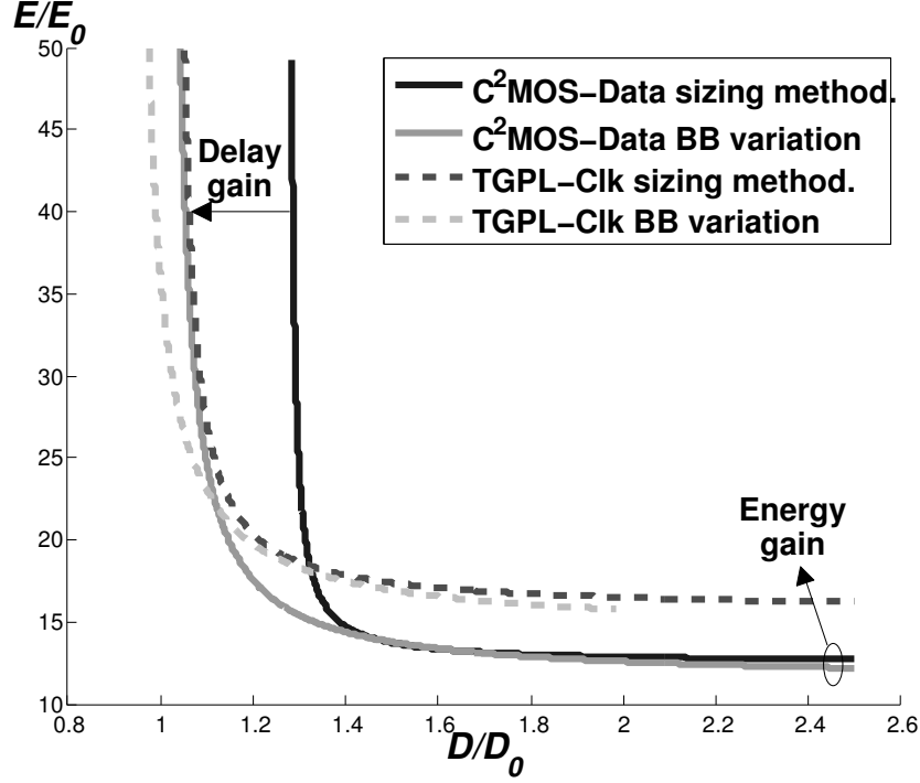
Figure 2.13: EECs of the C 2 MOS-Data and TGPL-Clk architectures extracted from the sizing methodology and from a applied back biasing ( V_{dd} = 1V , vdds/gnds range = \pm 1V , \alpha_{sw} = 0.15 , T_{clk} = 40FO4 , temperature 70^\circ C ). Back biasing technique provides better performances than sizing methodology.
