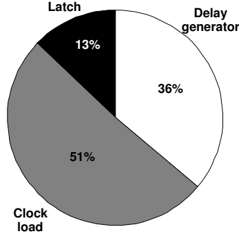
Figure 4.2: Repartition of the energy dissipation in C^2 MOS architecture (minimum EDP sizing). Corner TT, nominal voltage (1V), temperature = 70°C.
