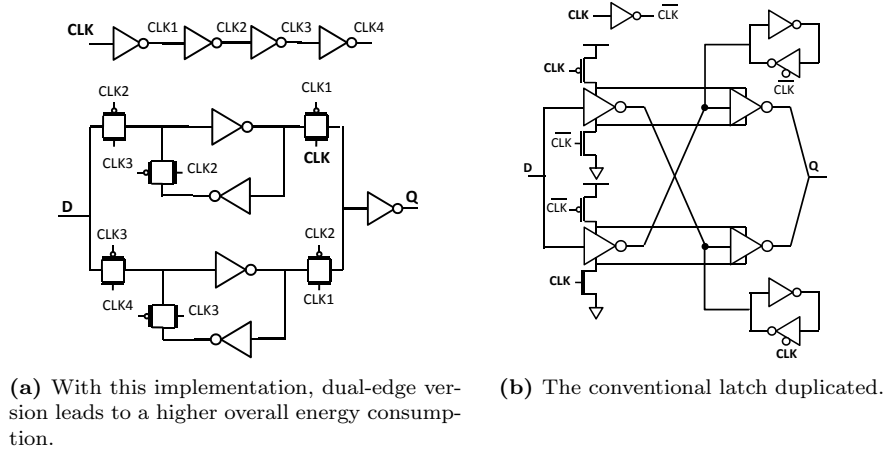
Figure 1.18: A basic implementation of the dual-edge property [7].
