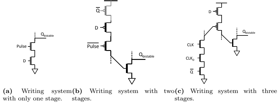
Figure 2.5: Schematic principle of the writing system with many stages. Only the pull-down part is shown.
