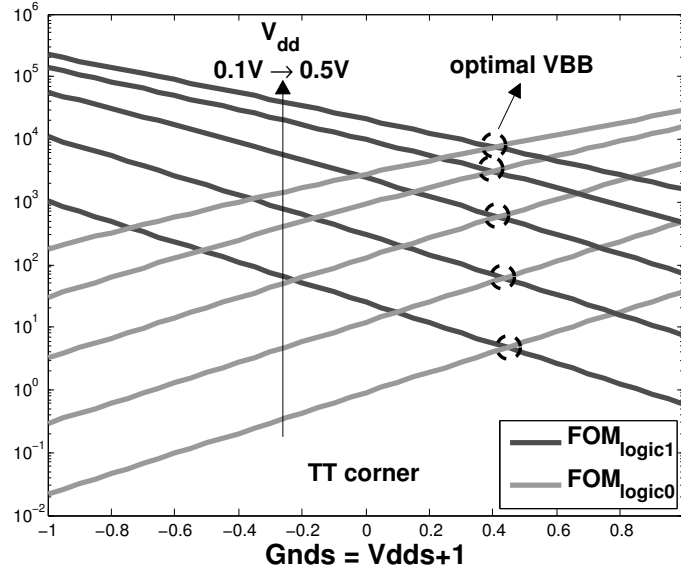
Figure 3.13: For V_{dds} and G_{nds} values evolving in the same way, an optimal point is found near the middle of the diagonal 2 (Fig. 3.11).
