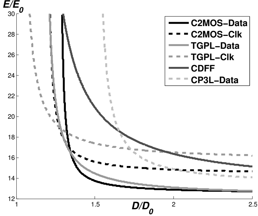
Figure 2.11: EEC: V_{dd} = 1.0V , v_{dds}=gnds=0V , \alpha_{sw} = 0.15 , T_{clk} = 40FO4 , corner TT, temperature 70^{\circ}C .
