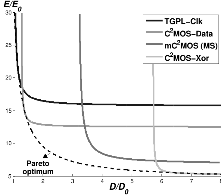
Figure 4.5: EECs for the four interesting architectures at V_{dd} = 1V (driving strength X1, \alpha_{sw} = 0.15 , T_{clk} = 40FO4 , temperature 70^\circ C ). The dashed curve is only there to illustrate the Pareto optimum idea.
