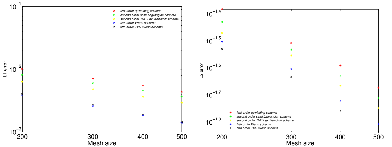
Figure 5.15: L^1 and L^2 errors evolution in log-log scale for a Square Pulse initial condition with the pressure-mediated proliferation model. \gamma_0 = 0.78 \text{ day}^{-1} ; \Pi_c = 0.0026 \text{ r.i} (ri: relative unit)
