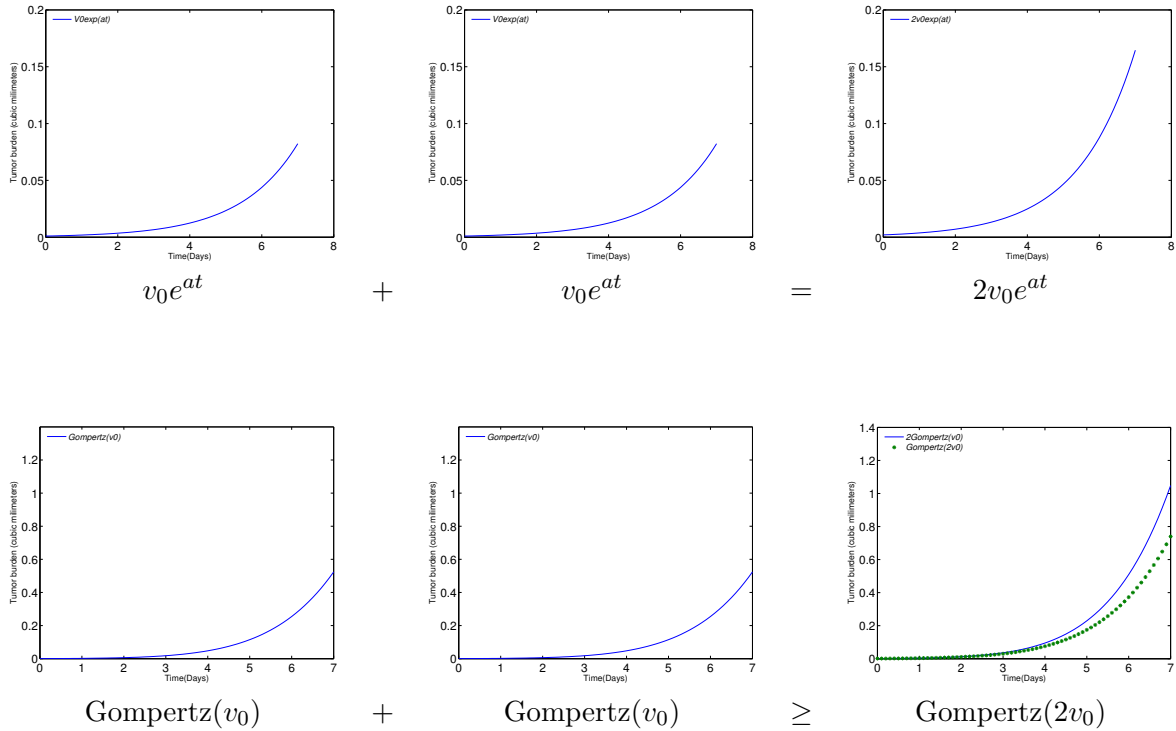
Figure 7.1: Top: two tumors growing under an exponential law lead to the same final total volume than one tumor with the same initial total volume; Bottom: two tumors growing under a Gompertz law lead to a larger final volume than one tumor with the same initial total volume
