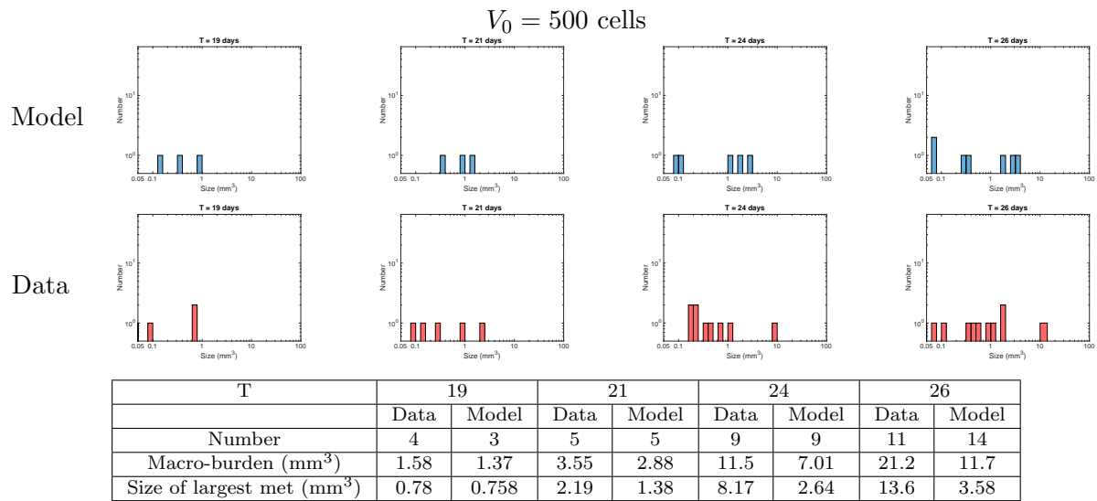
Figure A.3: Time course of the macro-metastases size distribution for different initial metastatic sizes. Top to down: simulation of the mathematical formalism of the standard theory (i.e. dissemination and independent growth of the resulting tumor foci), using the parameter values inferred from the total metastatic burden data (total GFP signal in the lungs) using four different initial numbers of initiating metastatic cells. The results are compared to observations of macro-metastases numbers and sizes in one mouse on MRI data.
