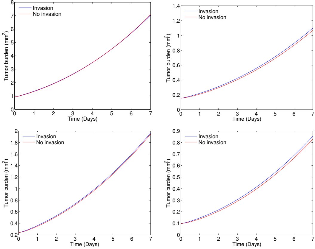
Figure 7.8: Comparison between the model with and without cellular diffusion (invasion) using the pressure mediated proliferation law (7.6). The parameters were retrieved from the fits on MRI data presented in Fig 5.16.
