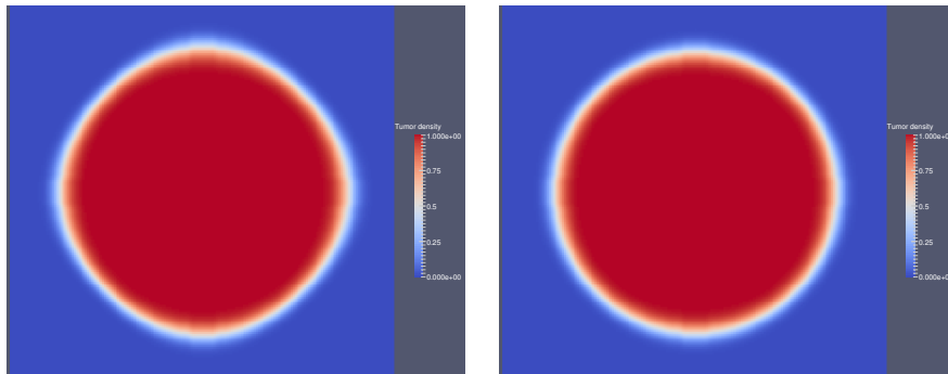
Figure 5.14: Simulation results for the tumor final distribution: final time T = 1\text{day} , \gamma_0 = 0.67\text{day}^{-1} , Mesh size 200 \times 200 . Left: k = 1 , Right: k = 1 in the included circle, k = 1000 outside.
