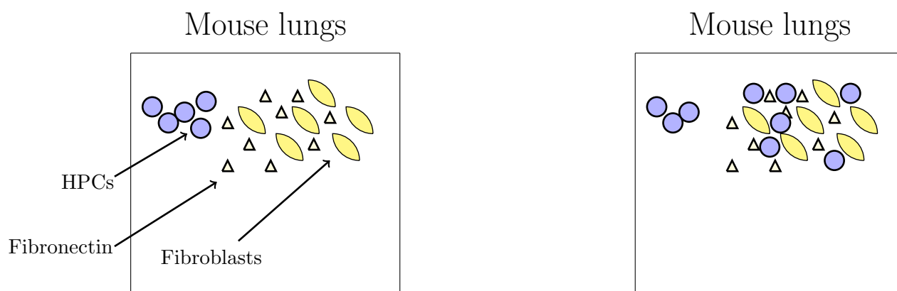
Figure 8.11: Second step of the premetastatic niche formation: HPCs adhere to the premetastatic niche thanks to fibronectin expression.
