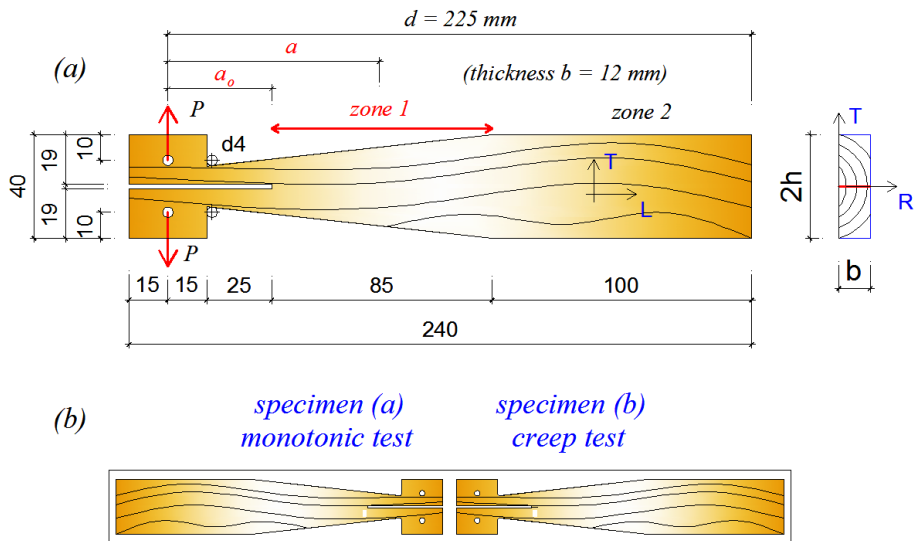
Figure 3.1: (a) Dimension of mTDCB specimen, (b) cutting position of mTDCB specimens for the 2 fracture tests
