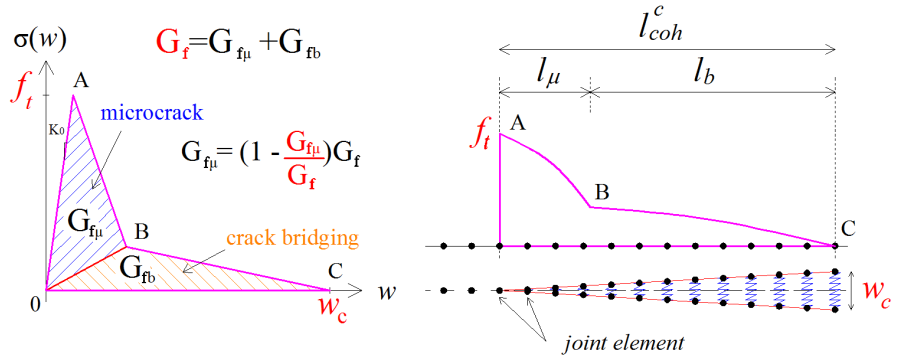
Figure 3.13: Bi-linear softening function in cohesive zone model
