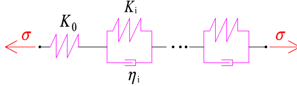
Figure 1.8: Generalized Kelvin Voigt model
