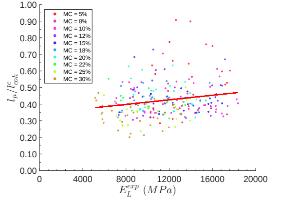
(f) Relation between l_\mu/l_{coh}^c and E_L^{exp}
