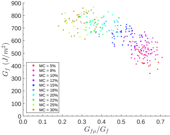
(d) Relation between G_f and G_{f\mu}/G_f
