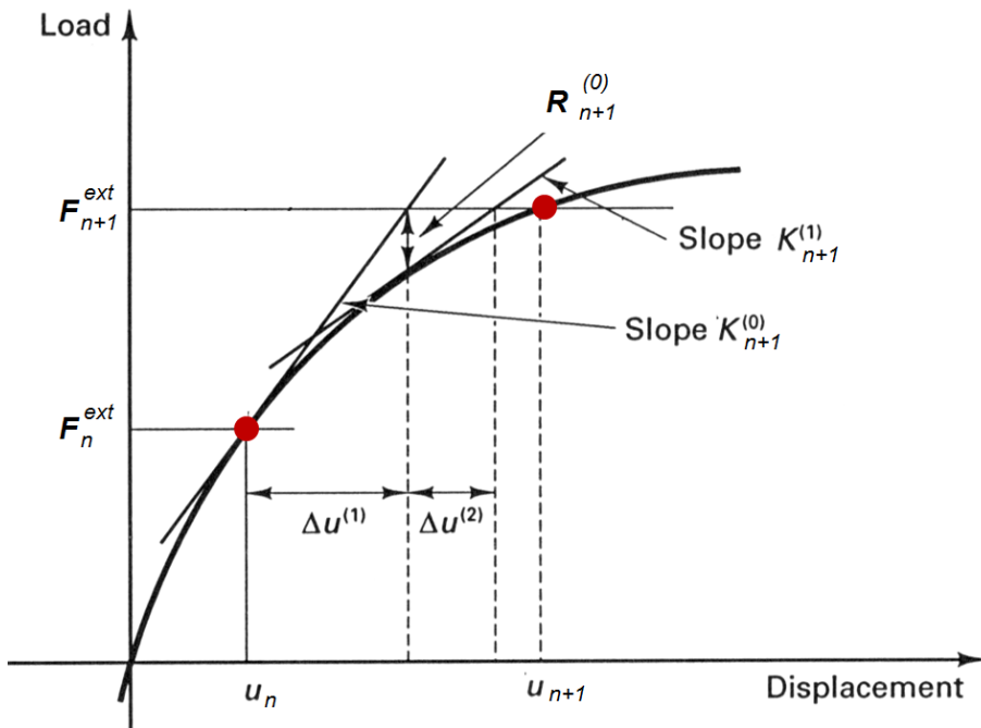
Figure 5.13: Newton-Raphson algorithm for Non-Linear Finite Element solution
