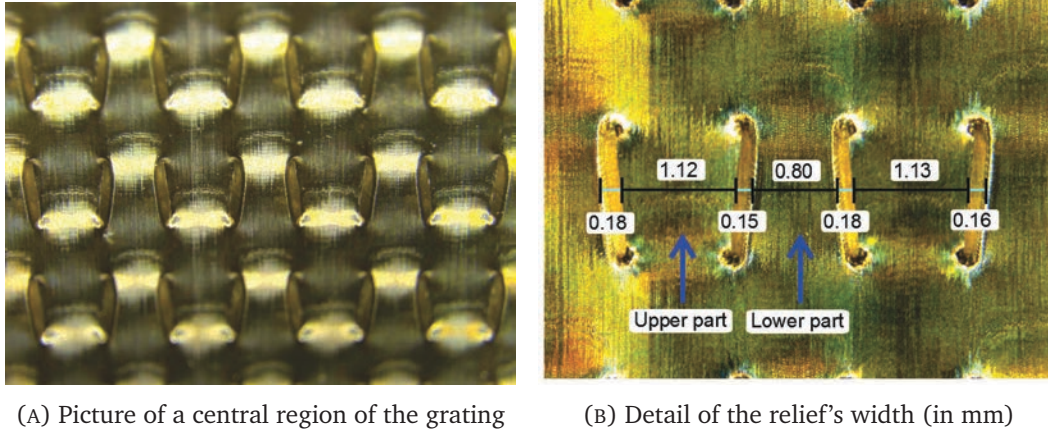
FIGURE 5.27: Picture of the reflective phase grating taken with a microscope
