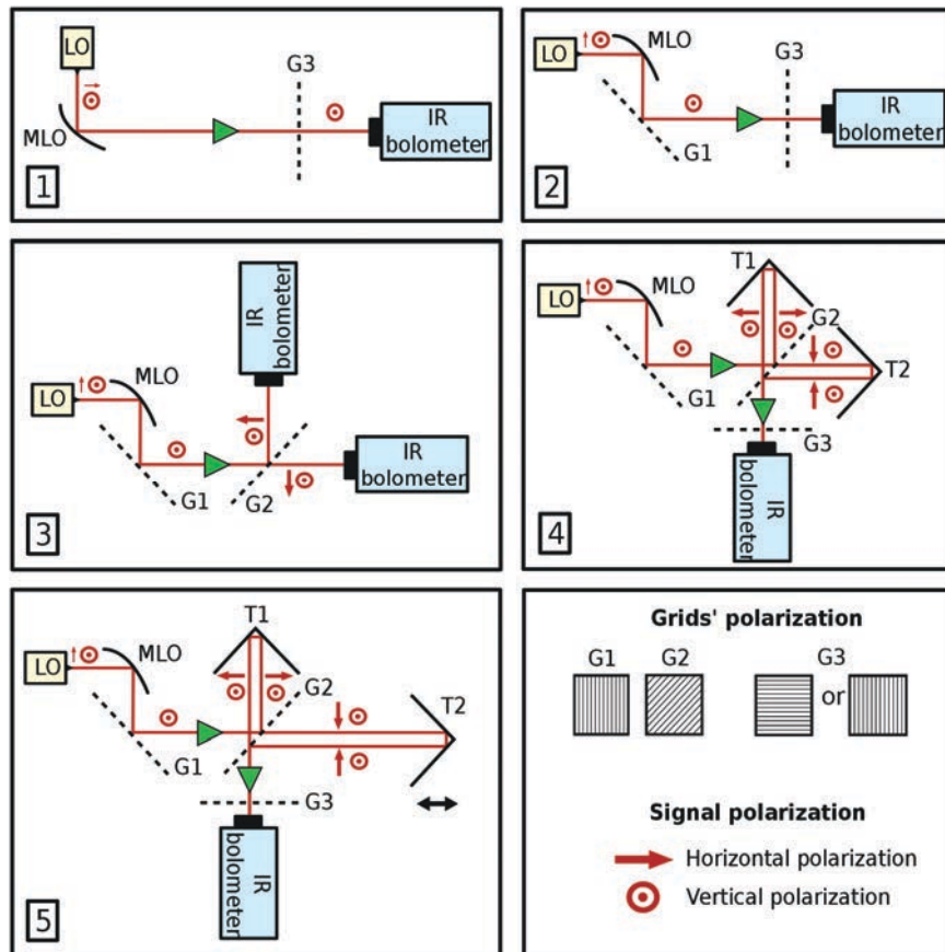
FIGURE 4.23: Consecutive steps of the MPI assembly
