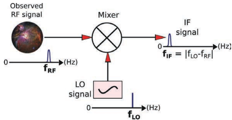
FIGURE 2.2: Principle of the heterodyne detection
