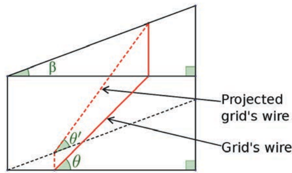
FIGURE 4.6: Projected inclination angle of the MPI grid's wires
