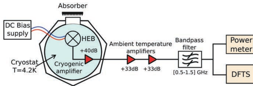
FIGURE 3.12: Set-up of the experiment to measure the stability of the cryogenic amplifier and the HEB bias supply
