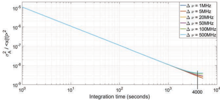
FIGURE 3.11: Spectral Allan variance for different spectral distances
