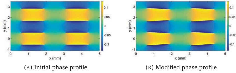
FIGURE 5.22: Modification of the phase profile to compensate the power disparity between the 4 beams
