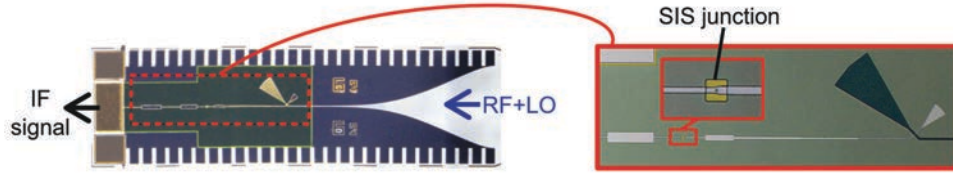
FIGURE 2.7: Picture of a SIS mixer (Credits: Faouzi Boussaha)
