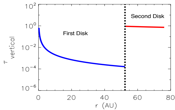
FIGURE 6.4: The vertical optical depth at 10 μm of wavelength versus the radius for the two-components disk model. The dashed line shows the transition between the two components.
