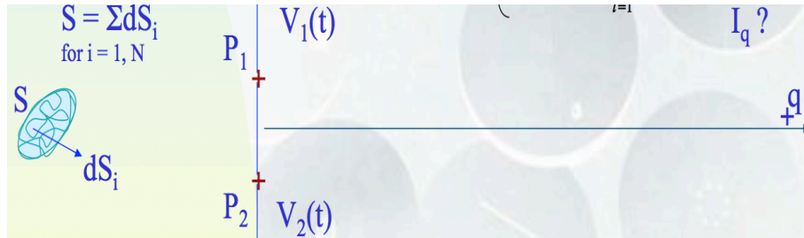
FIGURE 2.14: A scheme of the extended source with two similar pinholes. Credit: talk of J. Surdej in VLTI school.
