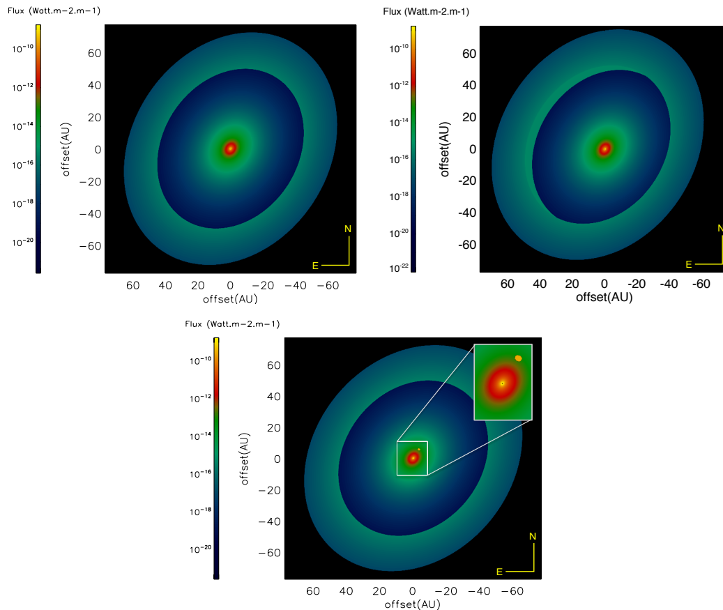
FIGURE 6.9: The synthetic image of MWC480 at \lambda=10 \mu\text{m} . Top-Left: Two-component disk model, Top-Right: Two-component disk model with wall, Bottom: Two-component disk model with clump.
