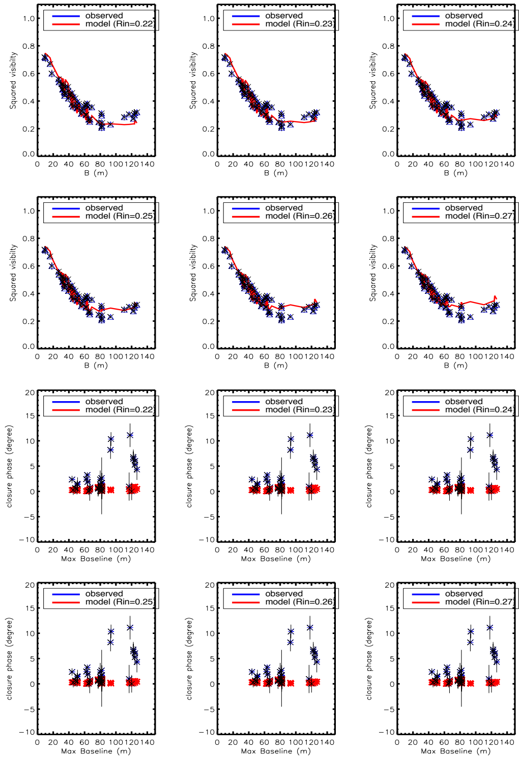
FIGURE 4.9: Top: Visibilities versus baseline for different inner radii of the inner disk and bottom: Closure phase versus Maximum baseline for different inner radii of the inner disk at \lambda=1.656 \mu\text{m} .
