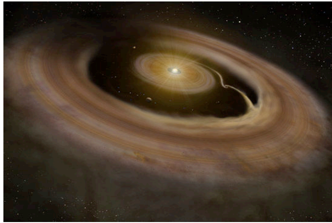
FIGURE 1.14: A pre-transitional disk around young star, 2MASS J16042165-2130284. Credit: The Graduate University for Advanced Studies, Japan.
