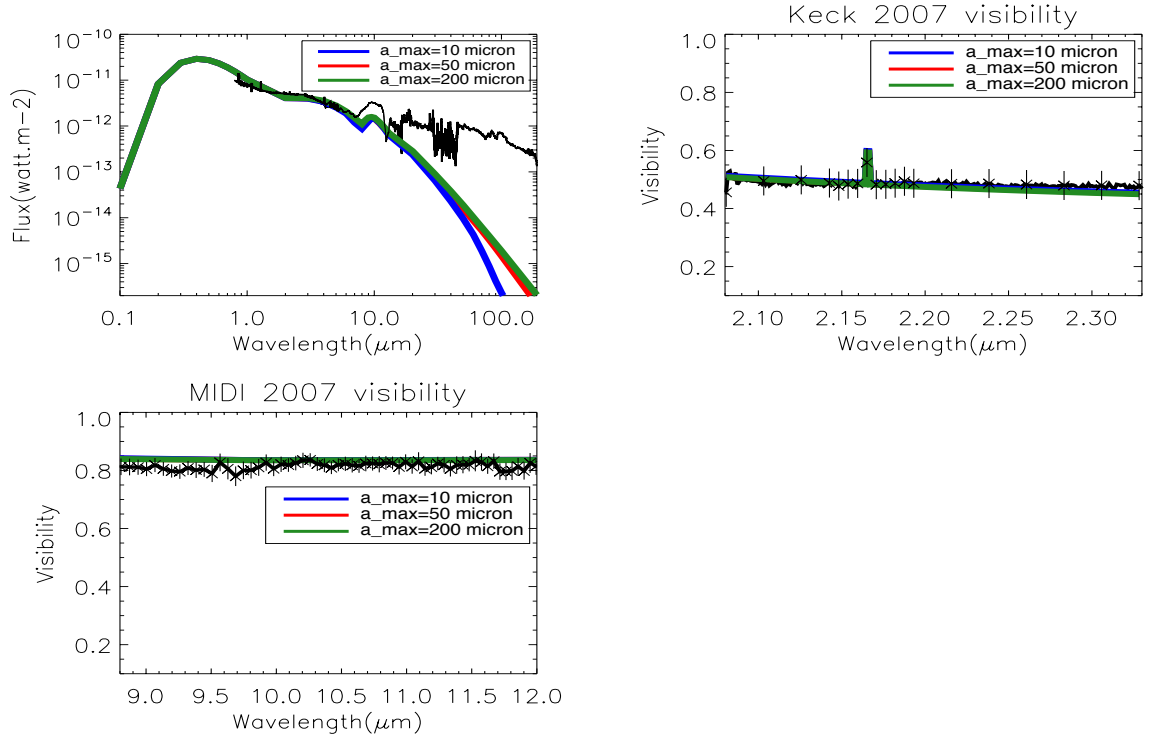
FIGURE 5.3: One-component disk model. The effect of the maximum grain size ( a_{max} = 10 \mu\text{m} , a_{max}=50 \mu\text{m} and a_{max}= 200 \mu\text{m} ) is compensated by an adjustment of the dust mass: M_{dust}=2.4 \times 10^{-11} M_{\odot} , M_{dust}=0.5 \times 10^{-10} M_{\odot} and M_{dust}=10^{-10} M_{\odot} , respectively. The black solid lines in plots represents the observational data. For the SED, SpeX and BASS data for 0.8-14 \mu\text{m} and ISO data in 1998 for 15–200 \mu\text{m} . MIDI uncorrelated spectrum between 8–13.5 \mu\text{m} .
