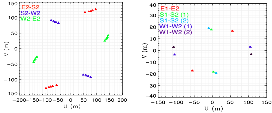
FIGURE 3.1: (u,v) coverage obtained for the observations of 51 Oph in the continuum (left) and the in the H\alpha line (right).
