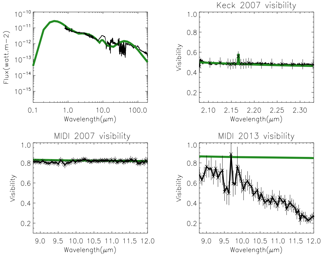
FIGURE 6.2: The two-component disk model for a maximum grain size of 200 μm. See caption of Fig. 5.6 of Chapter 5.
