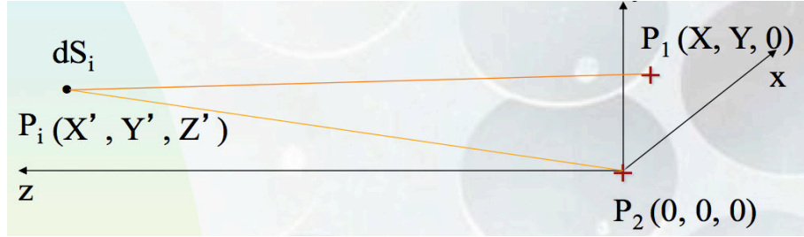
FIGURE 2.15: A schematic of the extended source with two similar pin hols. Credit: talk of J. Surdej in VLTI school.
