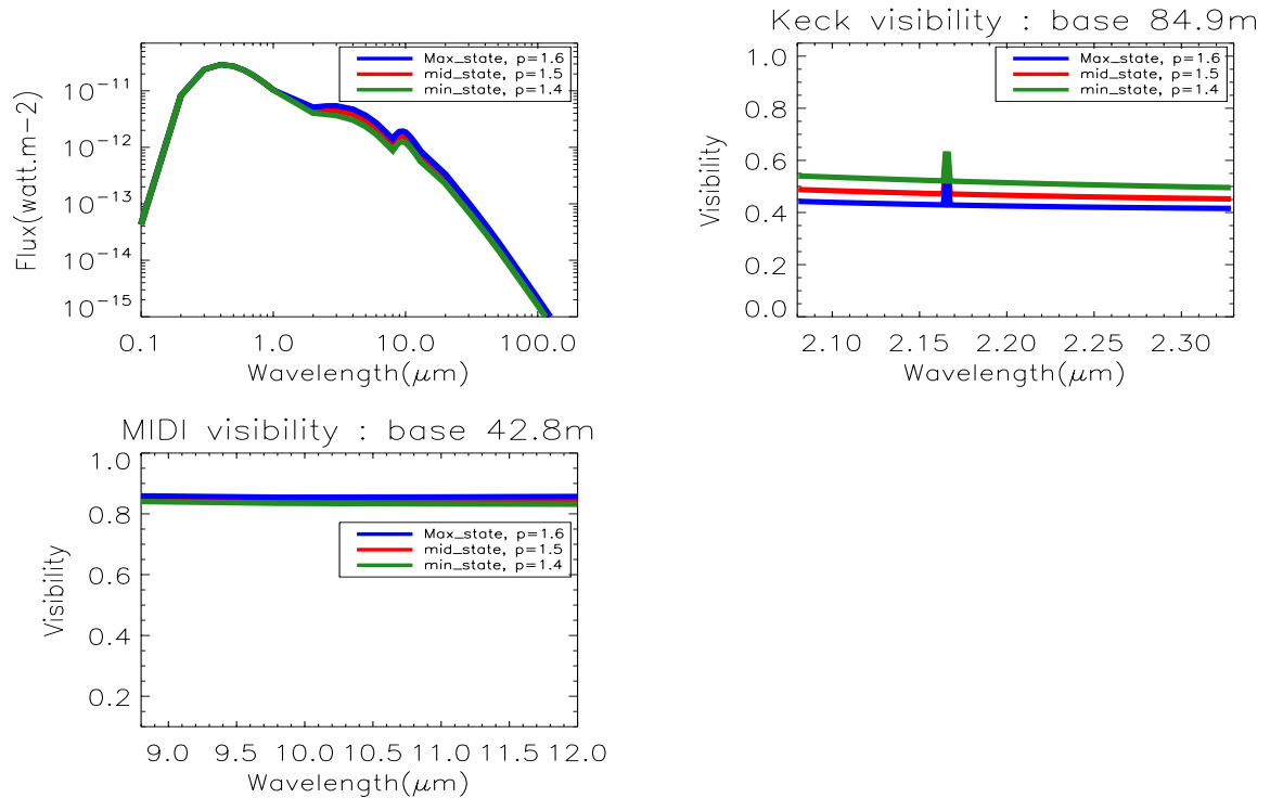
FIGURE 5.4: The effect of variability of the star in the near-IR in different brightness state for the maximum grain size of 200 \mu\text{m} in one-component disk model .
