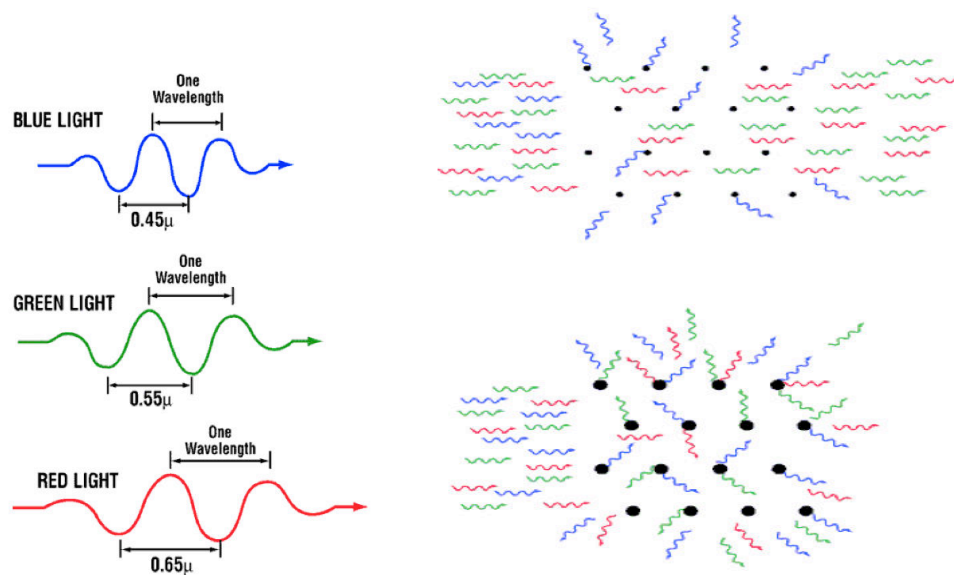
FIGURE 1.8: Left: three different incident light with different wavelength, i.e., blue: 0.45 \mu\text{m} ; green: 0.55 \mu\text{m} and red: 0.65 \mu\text{m} . Right-top: Scattering process for three different incident wavelength (left part of figure) and for small grains much smaller than the wavelength of incident light following Rayleigh scattering. Right-bottom: Scattering process for three different incident wavelength (left part of figure) and for larger grain sizes comparable to the wavelength of incident light following Mie theory (Mie 1908).
