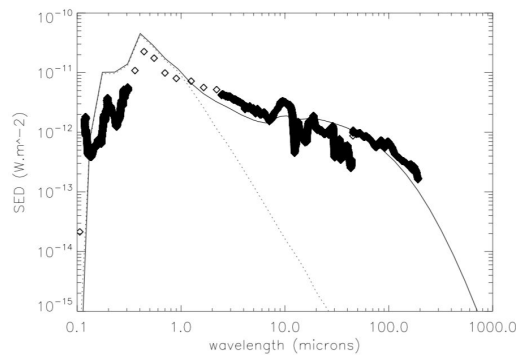
FIGURE 5.9: The plot of SED for a two-layer disk model including a mid-plane component. The bolded black line is observed data and thin black line is the best model.
