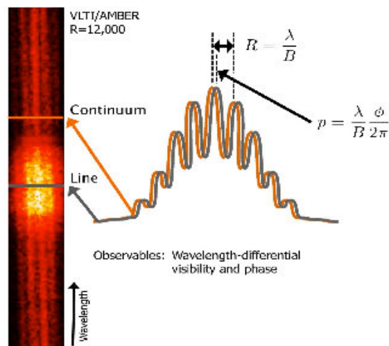
FIGURE 2.19: Spectro-interferometry uses spectrally dispersed interferograms (such as the VLTI/AMBER R = 12,000 interferogram from Kraus et al. (2011) shown here) in order to detect phase differences between the continuum emission and the emission within a spectral line. In first-order expansion, this differential phase \phi correspond to the photocenter offset p between the continuum- and line- emitting region. Credit: Kraus et al. (2011)
