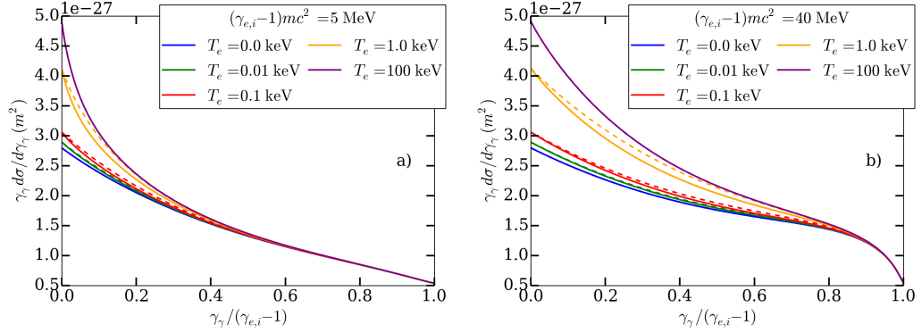
Figure 3.6: Cross section \gamma d\sigma_{\gamma\gamma}^{RE-WYD} (solid line) and \gamma d\sigma_{\gamma\gamma}^{RE-r} (dashed line) for different plasma temperatures (and consequently different degrees of ionization) for two initial electron energies 5 MeV (a) and 40 MeV (b) in silver.
