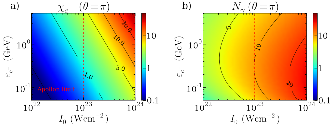
Figure 4.4: (a) Approximated electron quantum parameter \chi_{e^-} as a function of the laser intensity and the electron energy. (b) Number of photons of energy up to 1 MeV produced during a laser period by an electron. The red dashed line corresponds to the expected maximum intensity of the Apollon laser.
