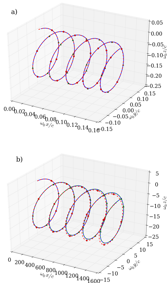
Figure 6.4: Particle trajectories in a circular plane wave calculated with the scheme of J. P. Boris (red dashed line), J. L. Vay (green dashed line) and analytically (blue) with 50 points per laser period and laser amplitudes of a_0 = 0.1 (a) and a_0 = 10 (b).
