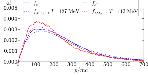
Figure 9.13: Corresponding electron f_{e^-} (red) and positron f_{e^+} (blue) distributions and comparison with the best-fitting Maxwell-Jüttner distributions f_{MJ} (dashed lines)
