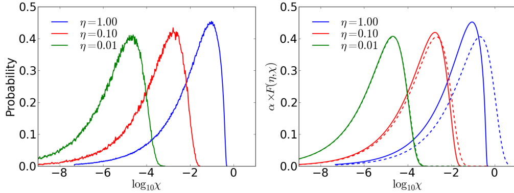
Figure 6.10: Photon distributions in \log_{10}(\chi_\gamma^f) : comparison between the simulations (a) and the synchrotron emissivity F(\chi_{e^-}, \chi_\gamma) (b) in the classical regime (dashed lines) and the quantum regime (solid lines). The factor of normalization is \alpha = \int_0^\infty F(\chi_{e^-}, \chi_\gamma) d\chi_\gamma .
