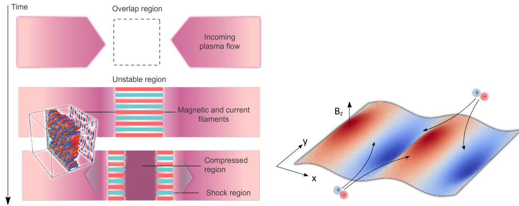
Figure 9.1: Schematic of the Weibel instability in the collision of two electron-positron pair plasmas.
