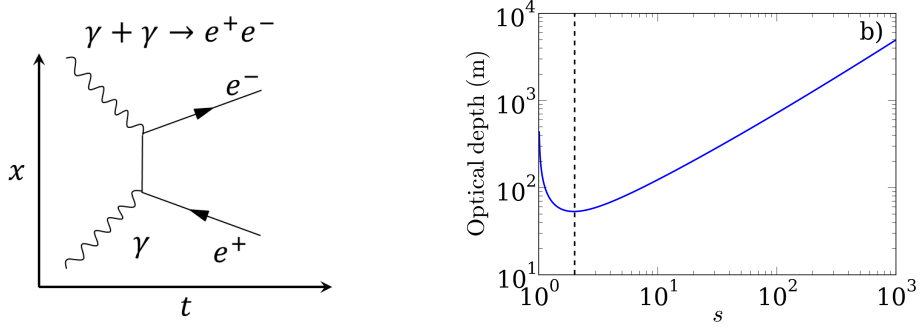
Figure 4.1: (a) - Feynman diagram of the photon-photon Breit Wheeler pair conversion. (b) - Optical depth as a function of the parameter s for a photon propagating in a cloud of photons of density n_c . The black dashed line corresponds to s = 2 .
