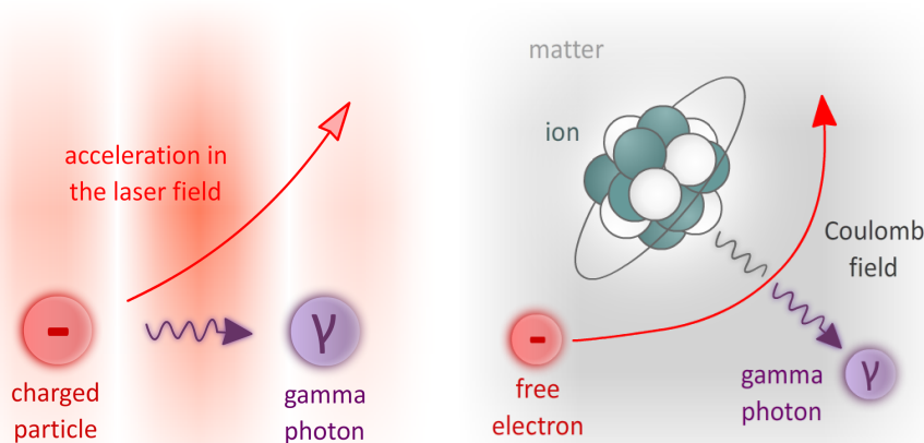
Figure 1.3: Scheme of the nonlinear Compton Scattering (a) and the Bremsstrahlung (b) emission processes.
