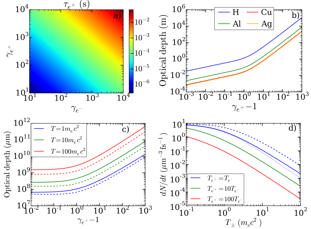
Figure 4.8: (a) - Lifespan of a positron of energy \gamma_{e^+} propagating in a mono-energetic cloud of electrons at \gamma_{e^-} at the critical density n_{e^-} = n_c . (b) - Optical depth (m) to pair annihilation in hydrogen, aluminium, copper and silver. (c) - Annihilation distance (optical depth) of a positron propagating in a Maxwellian plasma at temperature T_{\pm} = 1, 10, 100m_e c^2 . The dashed lines correspond to the case of the head-on collision of a particle with a counter-streaming cloud of electrons with energy \gamma_{e^-} = T_{e^-} . (d) - Annihilation rate in \mu\text{m}^{-3}\text{fs}^{-1} inside a Maxwellian pair plasma of temperature ratio T_{e^+}/T_{e^-} = 1, 10, 100 . Again, the dashed line corresponds to the collision of two mono-directional counter-streaming pair plasmas at similar energy \gamma = T_{\pm} . The dotted line corresponds to the collision with an angle of 0.01 rad of two beams of energy \gamma = T_{\pm} .
