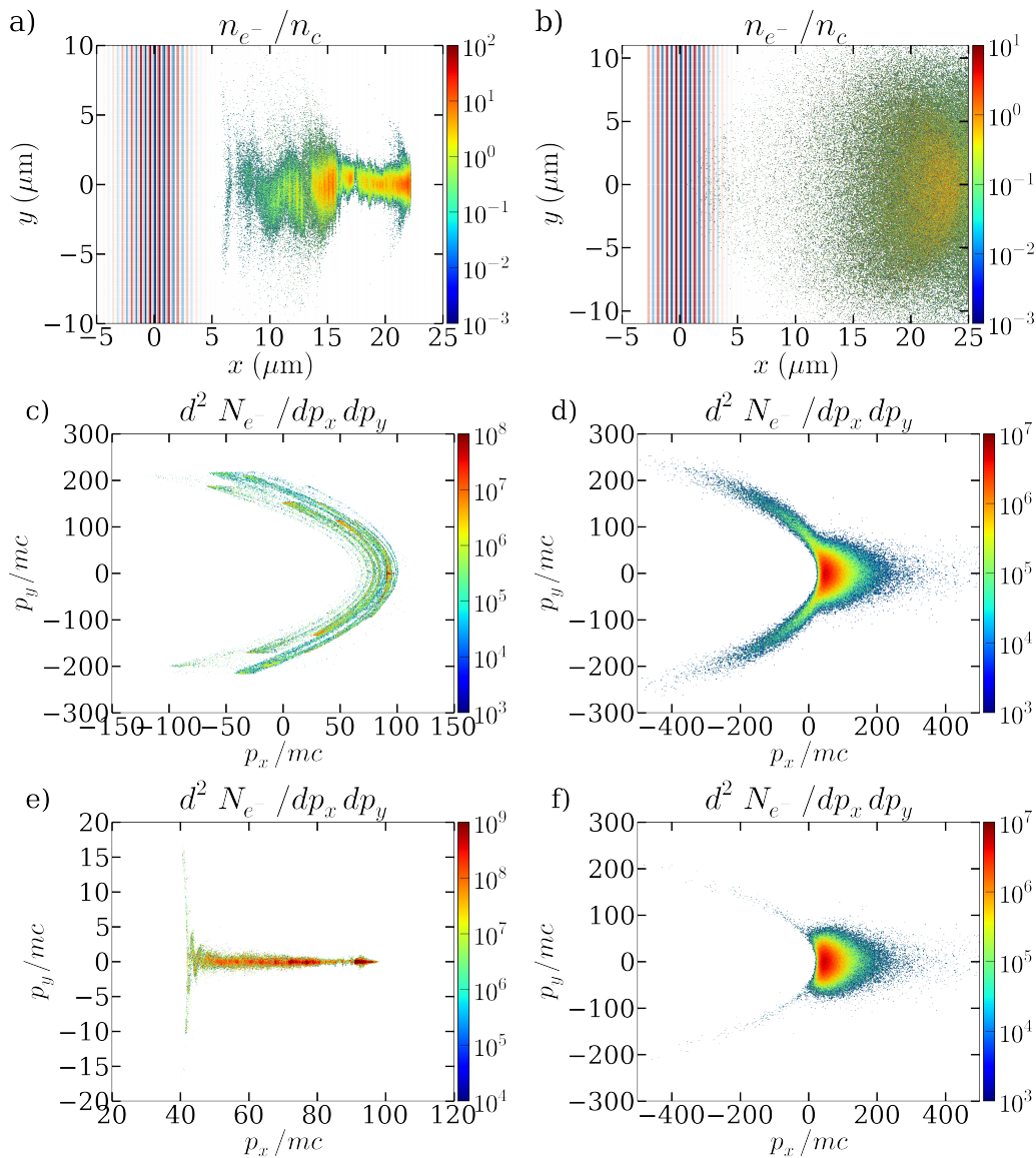
Figure 8.19: Electron density projection n_{e^-} from the initial beam on the plane x - y after the laser interaction ( t = 147 fs) with the Sokolov radiation friction model (a) and the quantum discontinuous description (b). Electron momentum phase space p_x - p_y at time of the maximum average angular divergence \theta_{xy} ( t = 126 fs) with the Sokolov radiation friction model (c) and the quantum discontinuous description (d). Electron momentum phase space p_x - p_y after the laser interaction with the Sokolov radiation friction model (e) and the quantum discontinuous description (f). Note that the x -axis and the colormap scales are changed in each figure.
