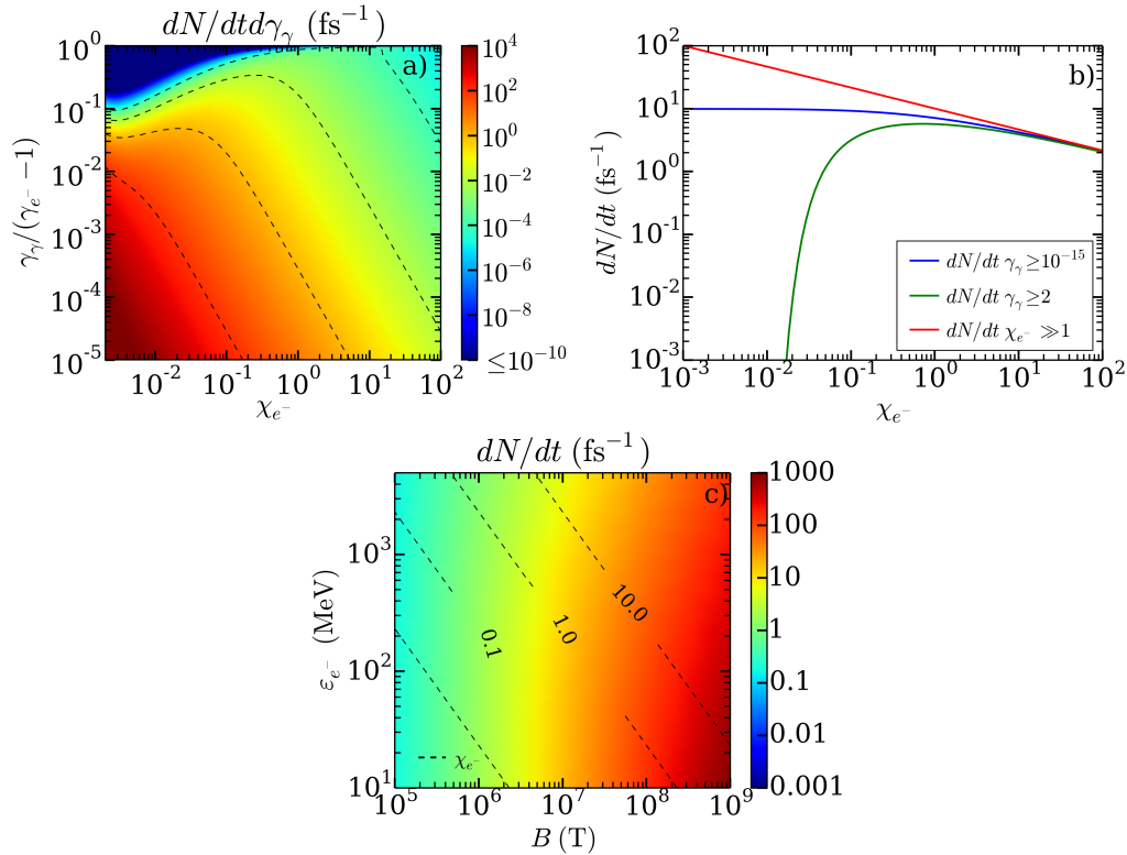
Figure 2.1: (a) - Energy-differential photon emission rate \frac{d^2N_{Cs}}{dtd\gamma_\gamma} (Eq. 2.7) as a function of the electron quantum parameter \chi_{e^-} and the ratio of the photon energy over the emitting electron kinetic energy. The dashed contours correspond to 10^{-4} , 10^{-2} , 10^0 and 10^2 . (b) - Photon emission rate \frac{dN_{Cs}}{dt} given by numerical integration of Eq. 2.7 for photon of energies above 1 MeV (blue curve), above 10^{-15}\gamma_{e^-}m_e c^2 (green curve) and the asymptote limit in the high- \chi region (red curve) as a function of the quantum parameter (here, the electron energy varies whereas the field is set at B = 5.5 \times 10^6 T). (c) - Photon emission rate in a constant magnetic field as a function of the magnetic field amplitude B and the electron energy \varepsilon_{e^-} . The dashed contour lines represent the electron quantum parameter parameter \chi_{e^-} .
