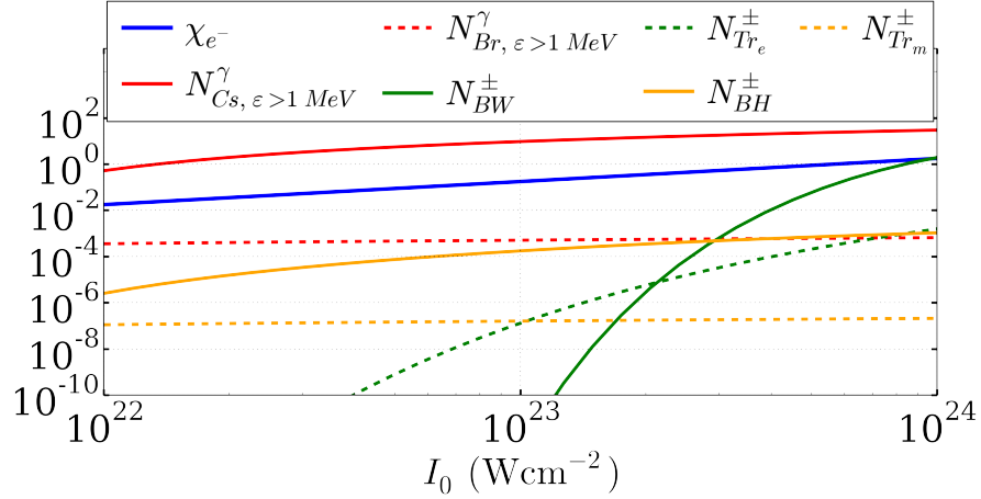
Figure 7.11: Electron quantum parameter \chi_{e^-} (blue), number of \gamma -photons generated via the nonlinear Compton scattering N_{Cs}^\gamma (red), via the Bremsstrahlung N_{Br}^\gamma (dashed red), number of pairs generated via the nonlinear Breit-Wheeler N_{BW}^\pm (green), via the electromagnetic Trident N_{Tr,e}^\pm (green dashed), via the Bethe-Heitler (orange) and the matter Trident (dashed orange) during a laser period T_l from a single electron as a function of the laser normalized amplitude a_0 .
