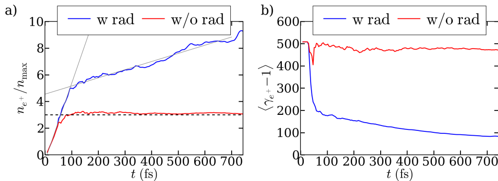
Figure 9.25: (a) - Time-evolution of the positron compression rate R = n_{e^+}/n_{\max} at the center of the domain in the radiative (blue) and the non-radiative case (red). The black dashed line represents the threshold of R = 3 . (b) - Time-evolution of the average positron kinetic energy at the center of the domain in the radiative (blue) and the non-radiative case (red).
