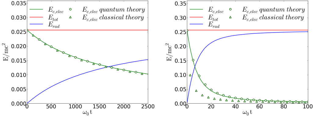
Figure 6.11: Evolution of the electron kinetic energy \varepsilon_{k,e^-} , radiated energy \varepsilon_{rad} and total energy \varepsilon_{tot} for \chi_{e^-} = 0.01 (a) and \chi_{e^-} = 1 (b). The simulation results are compared to the theory in the classical (triangle markers) and quantum regime (circle markers).
