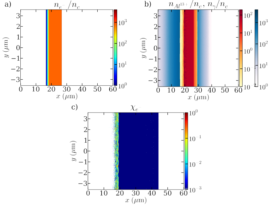
Figure 7.2: a) - Initial target configuration showing the electron density n_e/n_c . b) - Ion density n_{\text{Al}^{13+}}/n_c and photon density n_\gamma/n_c at time t = 159 fs. c) - The electron quantum parameter \chi_{e^-} at time 159 fs.
