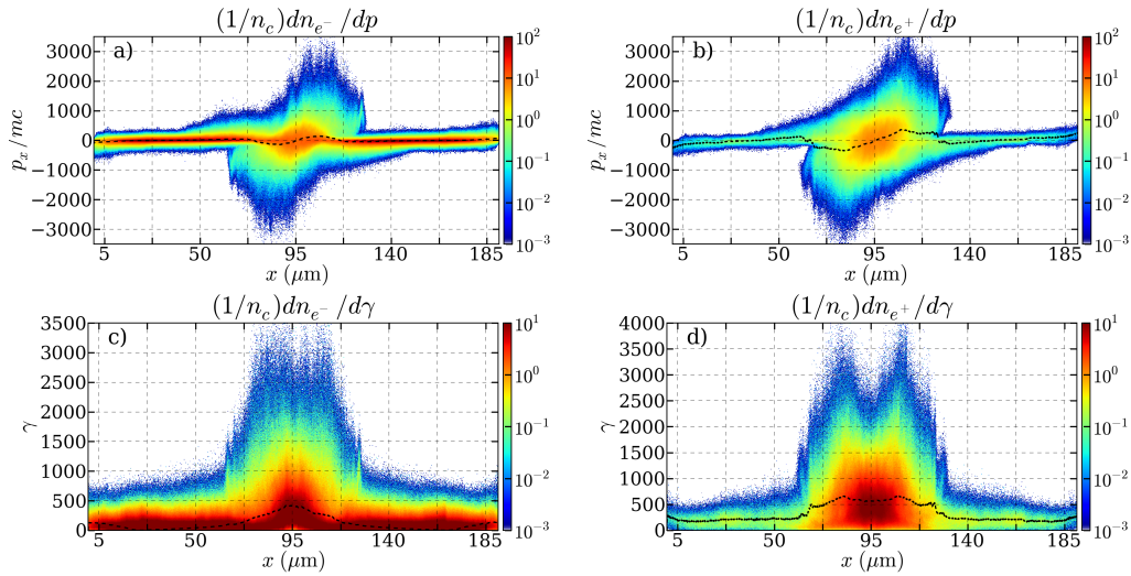
Figure 9.21: Electron (a) and positron (b) x - p_x phase spaces at the time t = 491 fs for the pair flow collision without radiation losses. Electron (c) and positron (d) x - \gamma phase space in the similar conditions.
