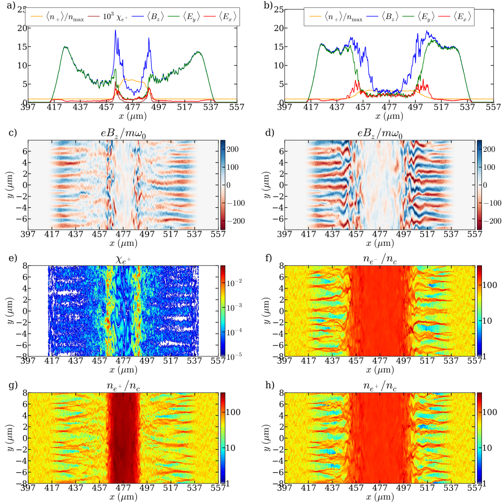
Figure 9.26: y -averaged positron density n_{e^+} , positron quantum parameter \chi_{e^+} , magnetic |B_z| and electric fields, |E_x| and |E_y| , in the radiative (a) and non-radiative (b) cases. Magnetic field |B_z| with (c) and without (d) radiation losses. (e) - Positron quantum parameter \chi_{e^+} for the radiative case. (f) - Electron density showing the filaments and the compressed structure in the non-radiative case. Positron density in the radiative (g) and the non-radiative case (h) in the overlapping region. All of the figures correspond to time t = 214 fs ( 405\omega_0^{-1} ).
