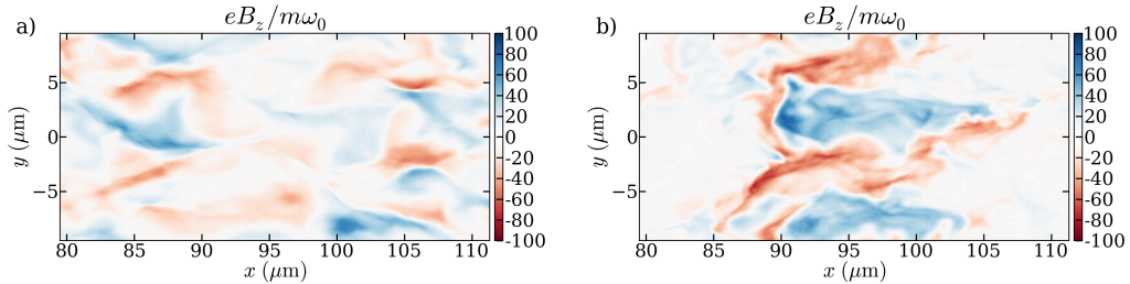
Figure 9.29: Magnetic field B_z in the overlap region t = 594 fs (a) and time t = 802 fs (b) during the ion collision.
