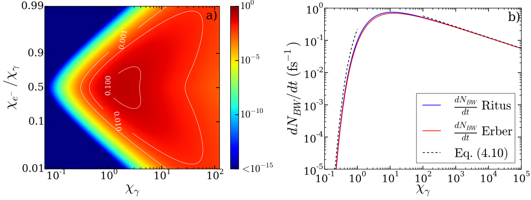
Figure 4.3: (a) - Normalized pair creation energy distribution given by Eq. 4.6. (b) - Normalized total pair production distribution. The blue curve is a plot of Eq. 4.7. The red one is the Erber approximation given by Eq. 4.9. Black curves are asymptotic approximations.
