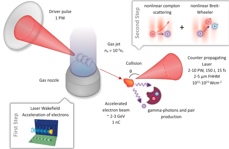
Figure 8.1: Scheme of the all-optical configuration studied in this chapter. Strong-field QED emission of \gamma -photons and the decay into pairs is studied in an all-optical scheme by the collision of a LWFA electron bunch with a counter-propagating extremely intense laser.
