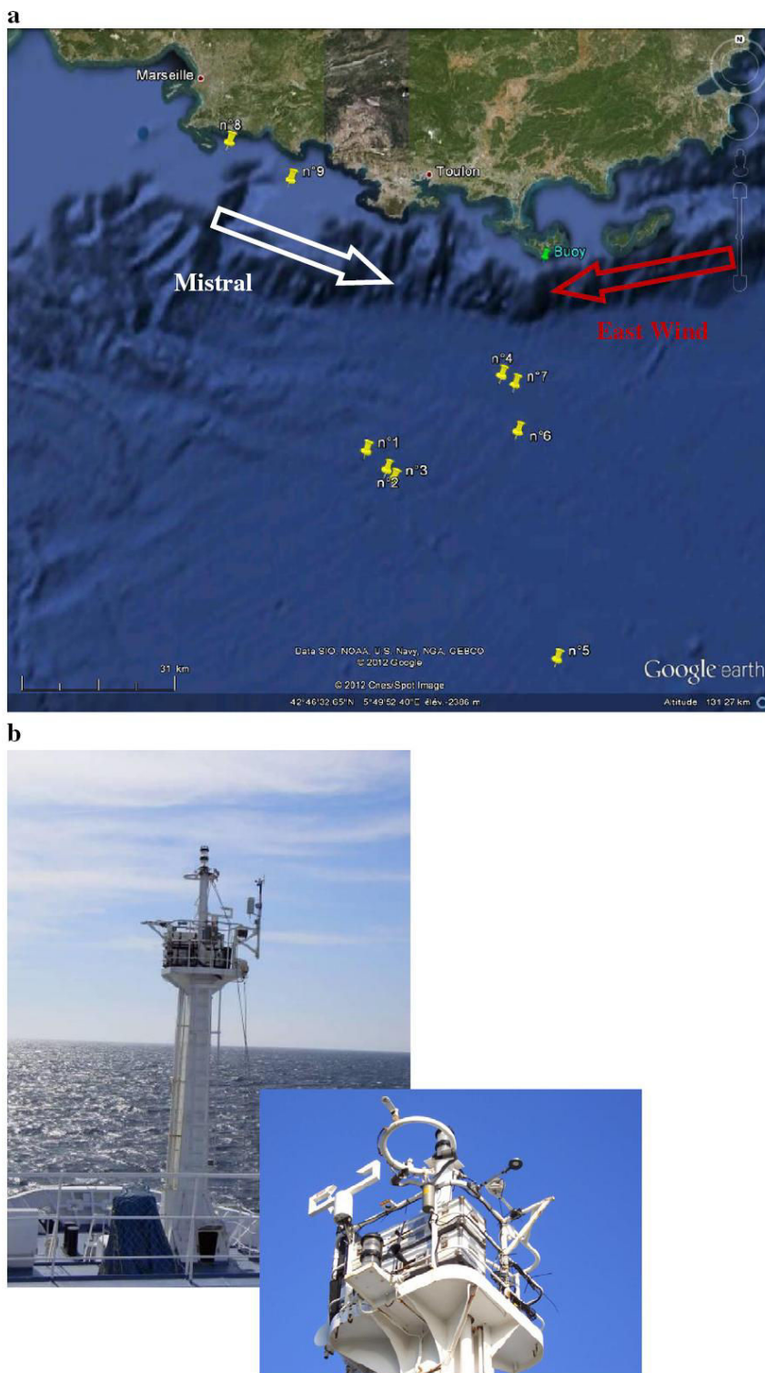
Fig. 1. a: The yellow pins show the locations of the aerosol size distribution samplings made on board of the “Atalante” from the 18 to the 28 May 2008. Each location is numbered from 1 to 9. The green pin shows the location of the buoy. b: The mast of the ship Atalante equipped with the two particle measuring systems and meteorological sensors at an elevation of 10 m height.
